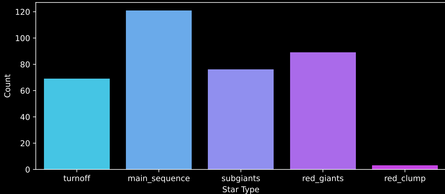
Gaia Cluster: [FSR_0336] Count plot of Star Type
