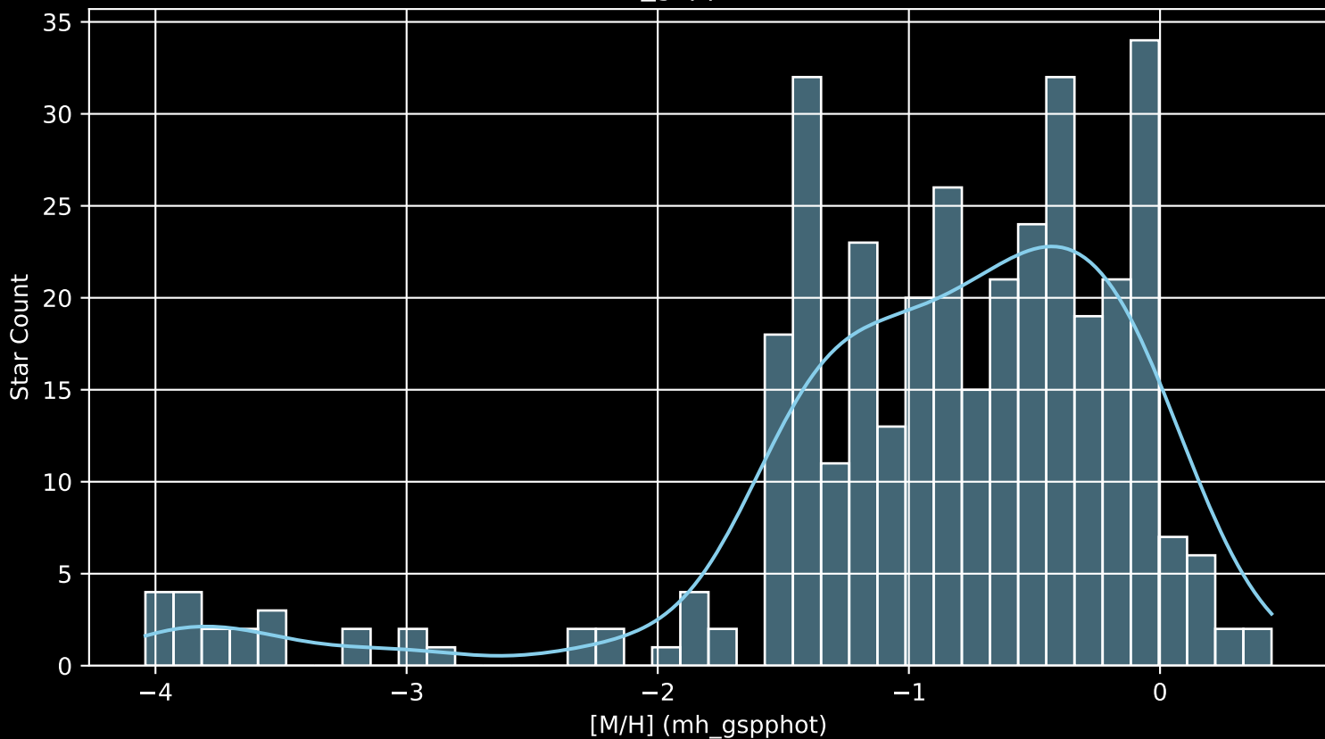
Gaia Cluster: [FSR_0336 [M/H] (mh_gspphot) (n= 357)
