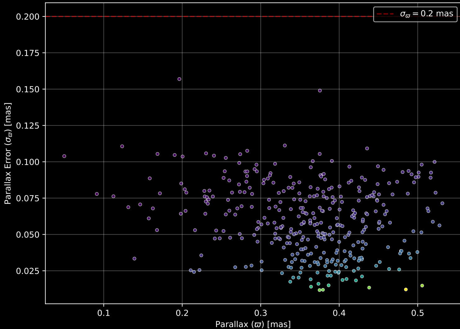
Gaia Cluster: [FSR_0336] Parallax Quality (n= 358)
