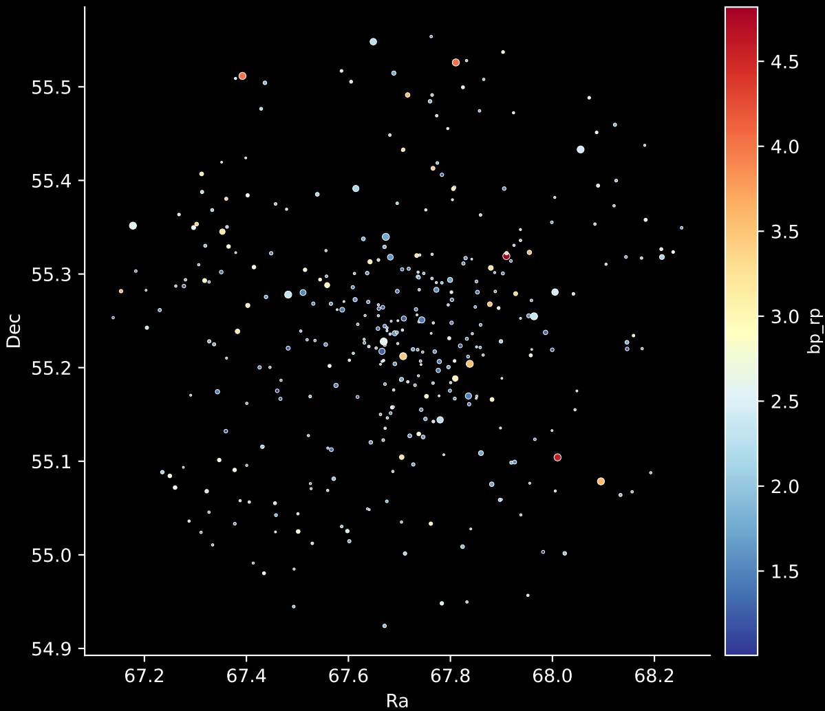
Gaia Cluster: [FSR_0336] Stars: 358
