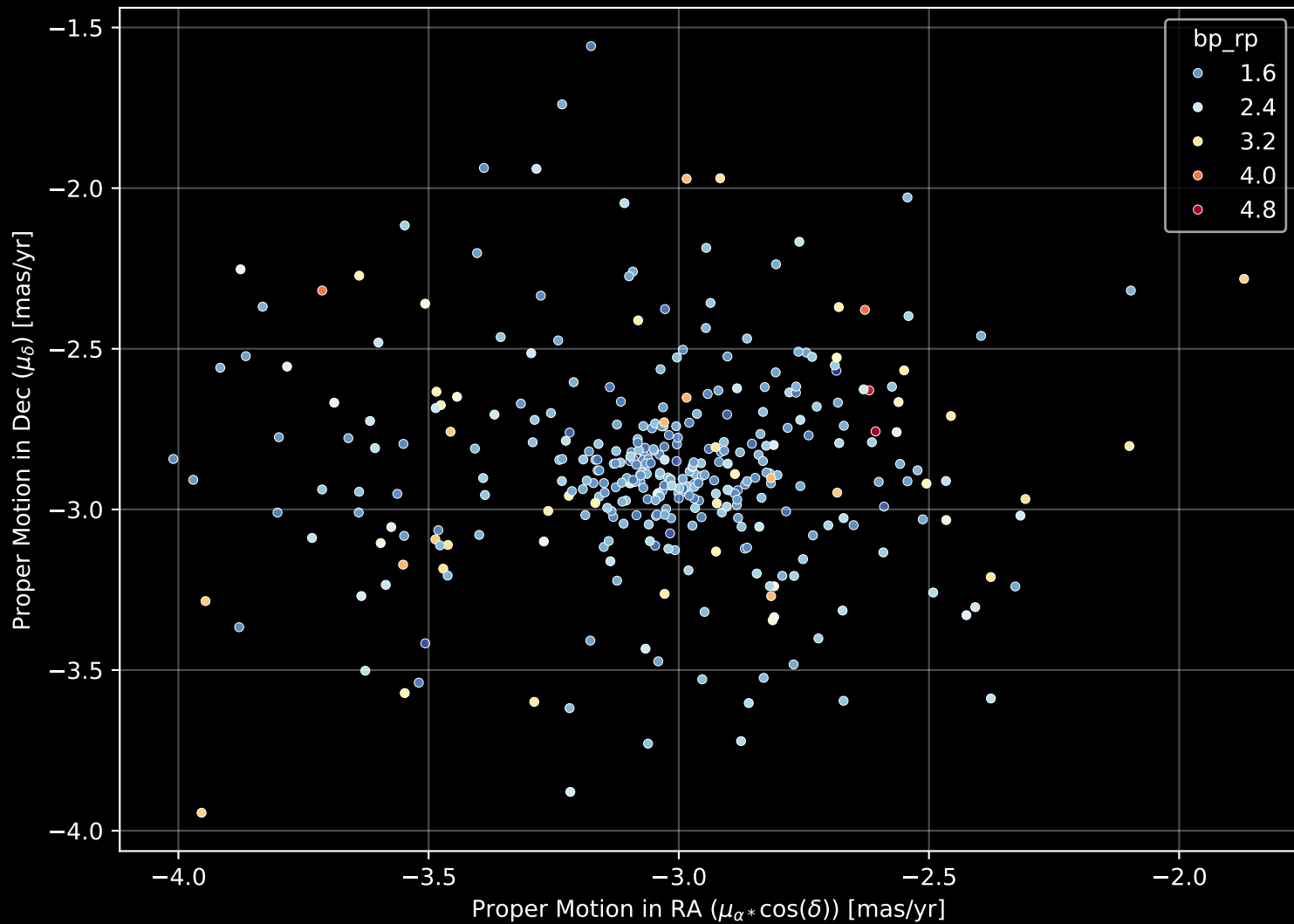
Gaia Cluster: [FSR_0336] Proper Motion Diagram (n= 358)
