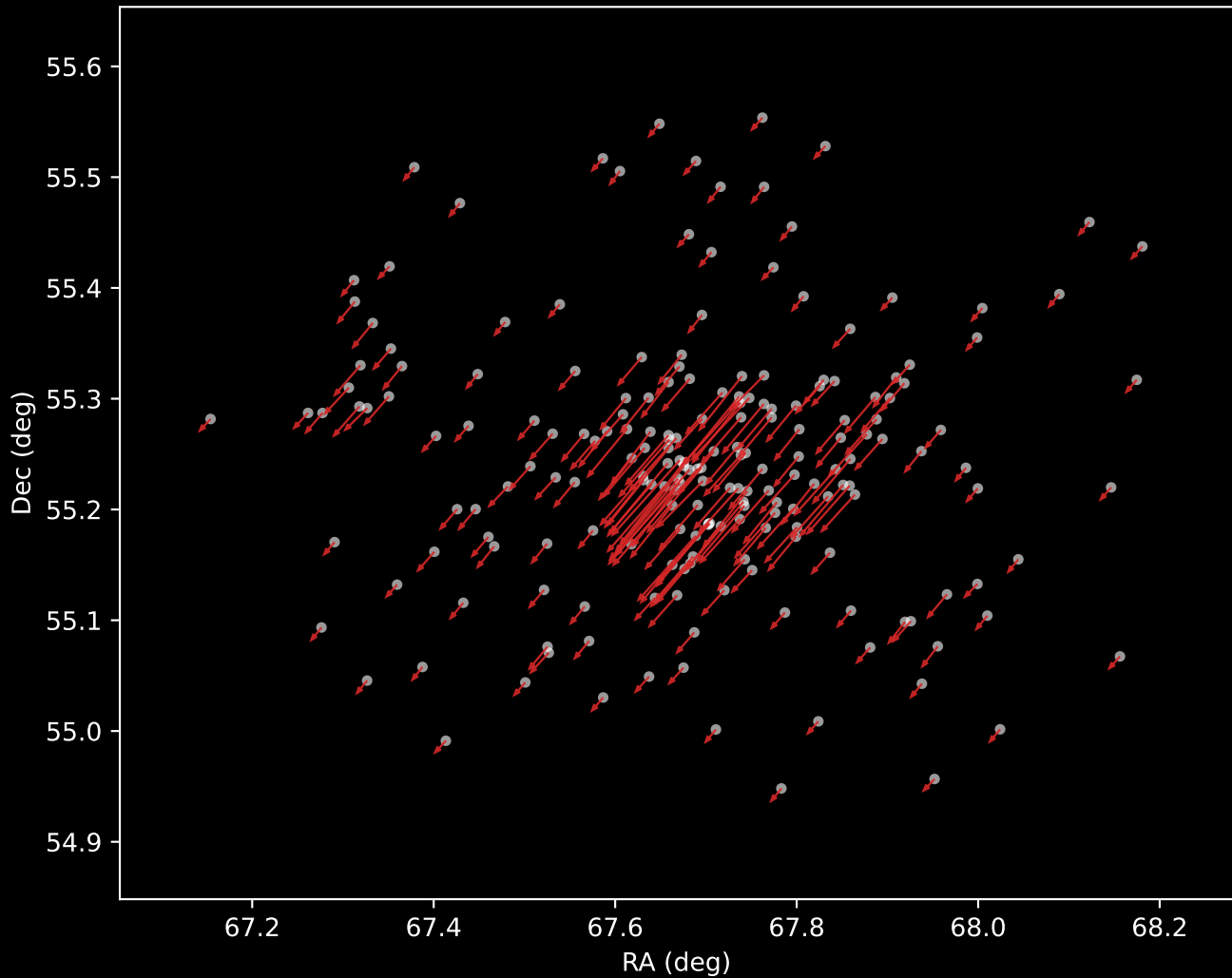
Gaia DR3 Cluster 6 Proper Motion Vectors (n=203)
