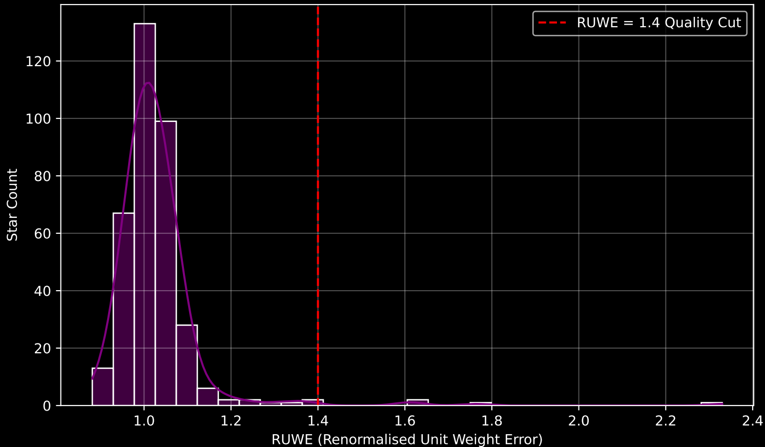
Gaia Cluster: [FSR_0336] RUWE Distribution (n= 358)
