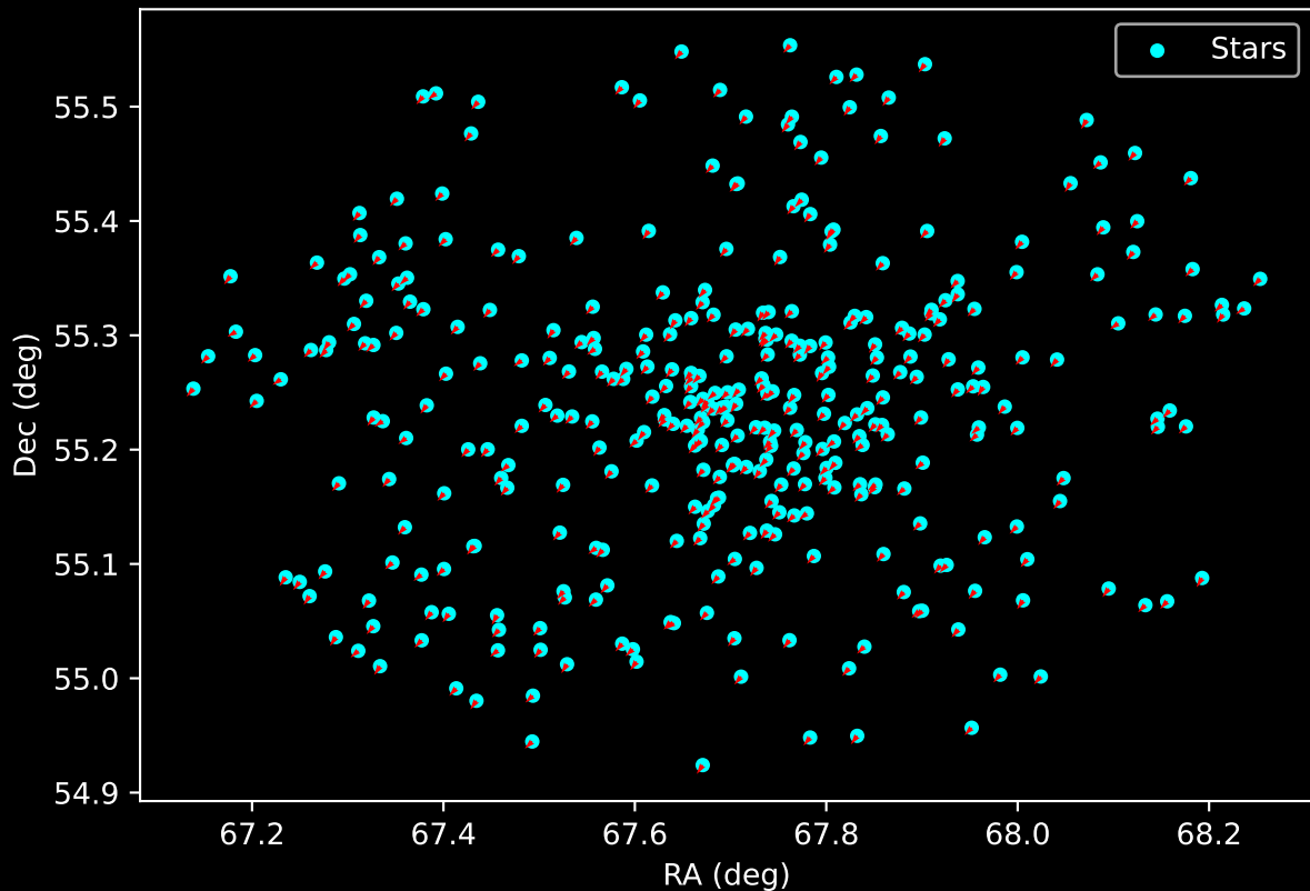
Gaia Cluster: [FSR_0336] Proper Motion Vectors for Gaia Star Field (n= 358)
