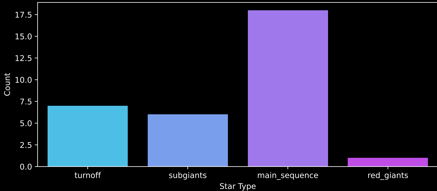
Gaia Cluster: [FSR_0385] Count plot of Star Type
