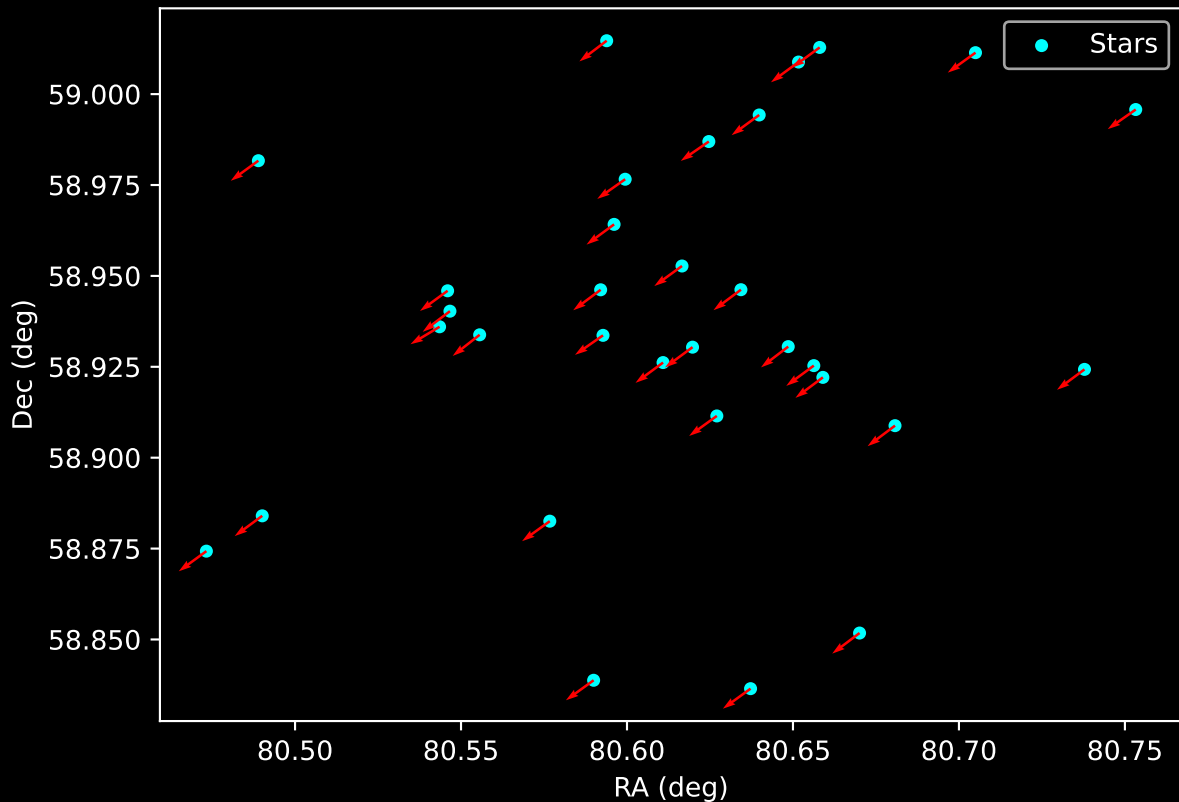
Gaia Cluster: [FSR_0385] Proper Motion Vectors for Gaia Star Field (n= 32)
