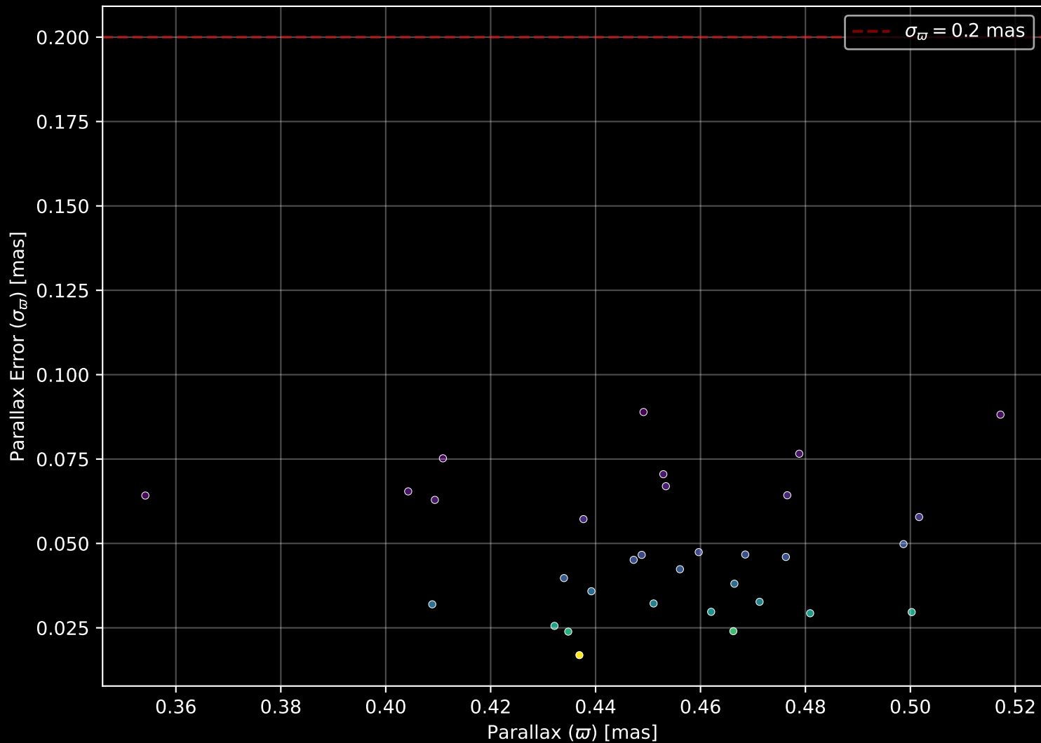
Gaia Cluster: [FSR_0385] Parallax Quality (n= 32)
