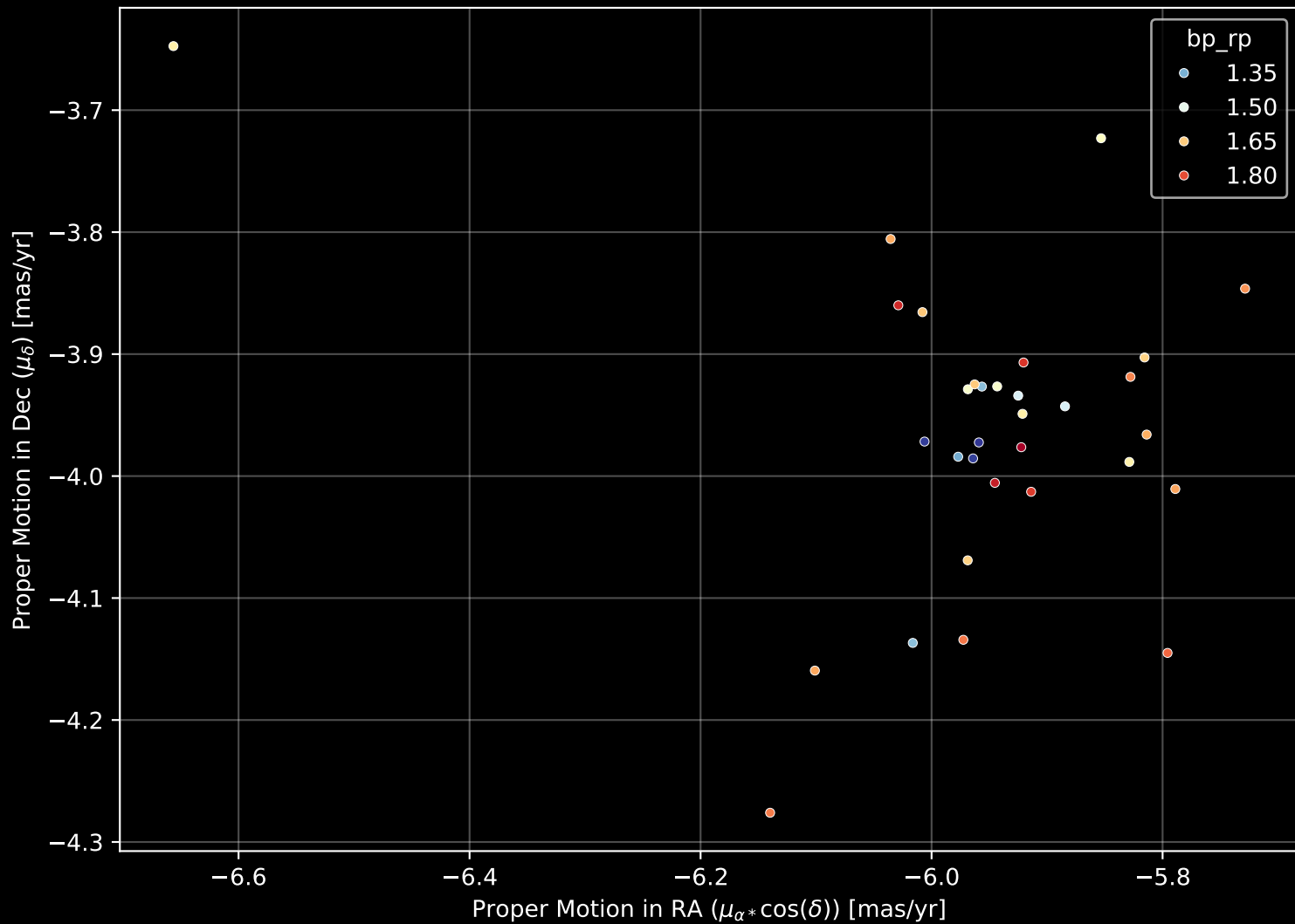
Gaia Cluster: [FSR_0385] Proper Motion Diagram (n= 32)
