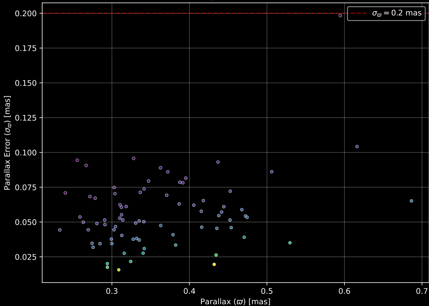
Gaia Cluster: [FSR_0448] Parallax Quality (n= 78)
