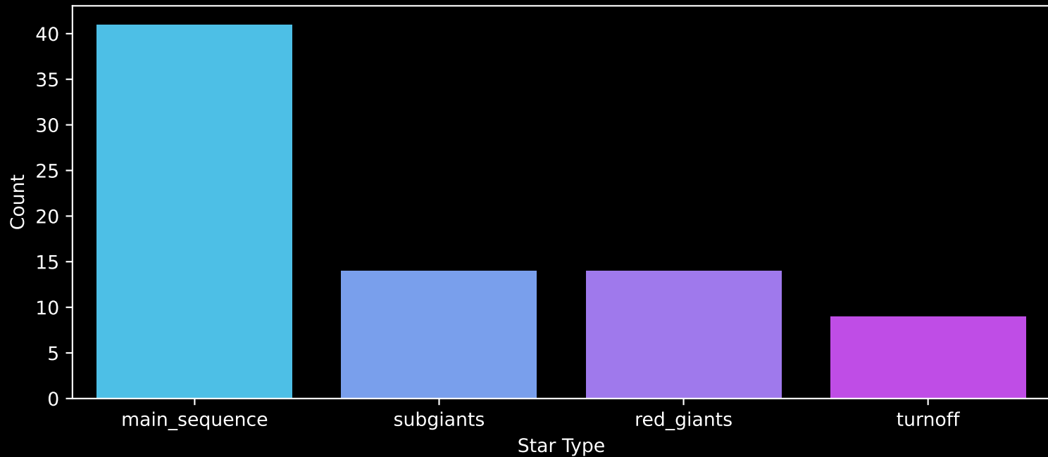
Gaia Cluster: [FSR_0448] Count plot of Star Type
