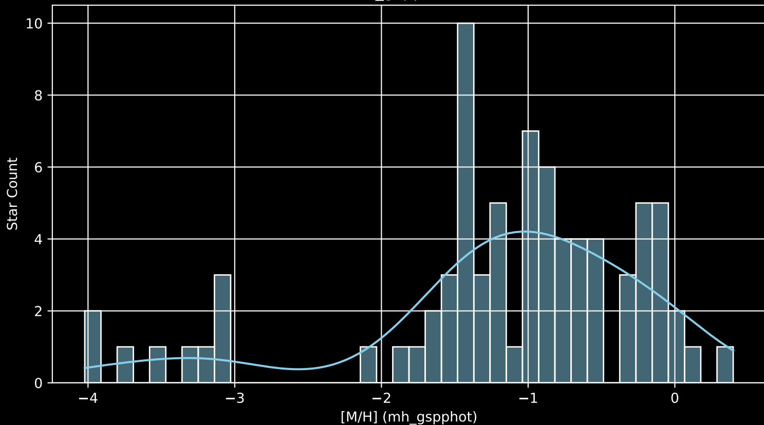
Gaia Cluster: [FSR_0448 [M/H] (mh_gspphot) (n= 78)
