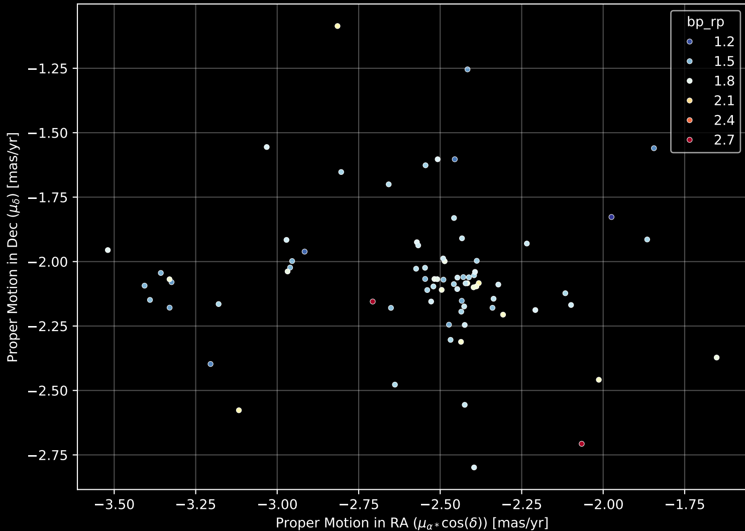
Gaia Cluster: [FSR_0448] Proper Motion Diagram (n= 78)
