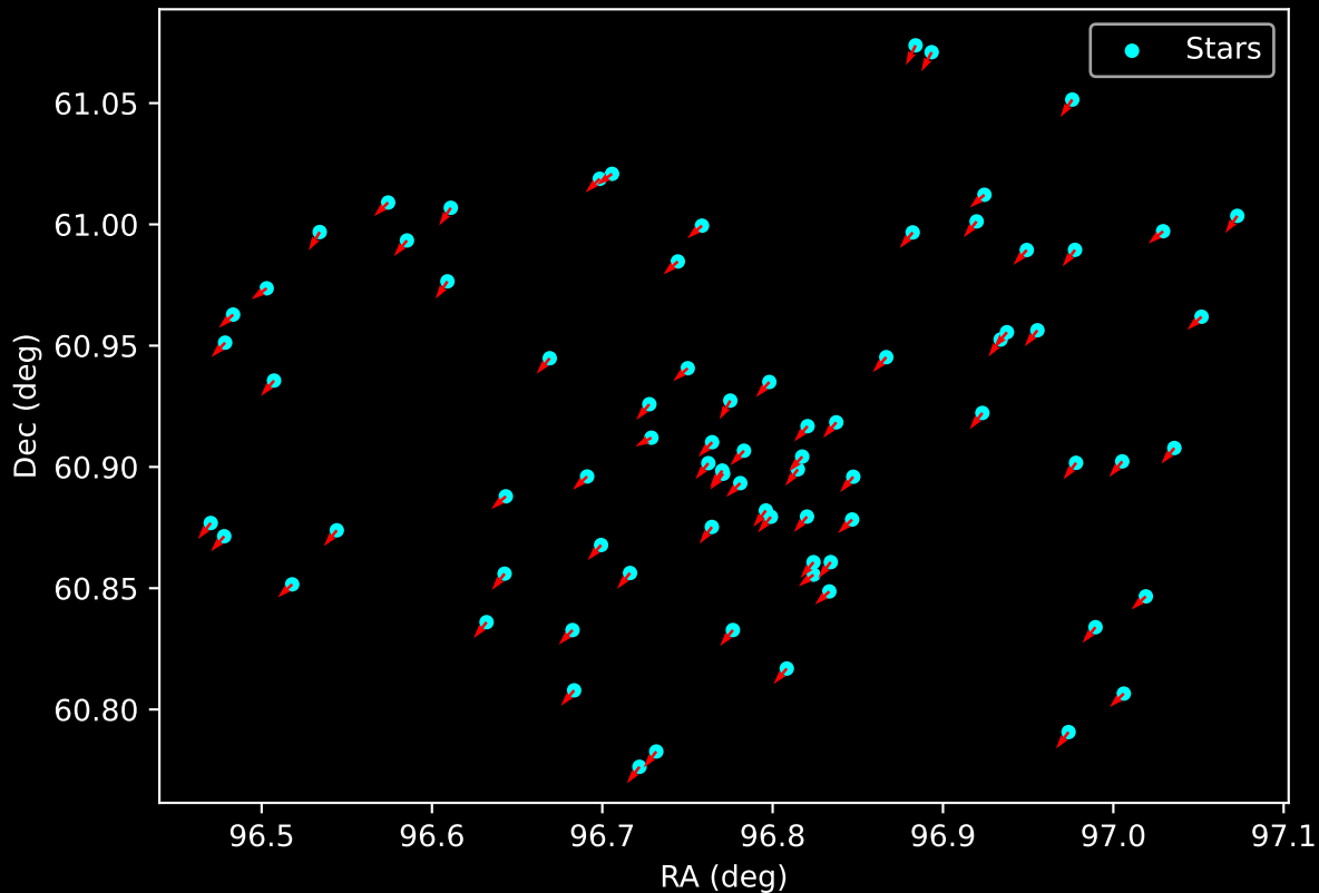
Gaia Cluster: [FSR_0448] Proper Motion Vectors for Gaia Star Field (n= 78)
