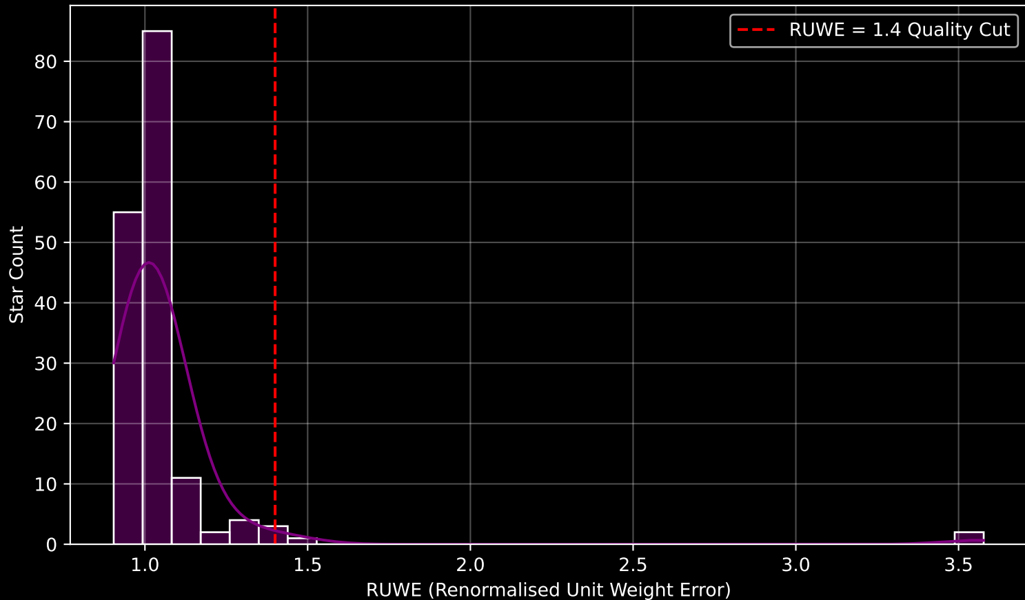
Gaia Cluster: [FSR_0496] RUWE Distribution (n= 163)
