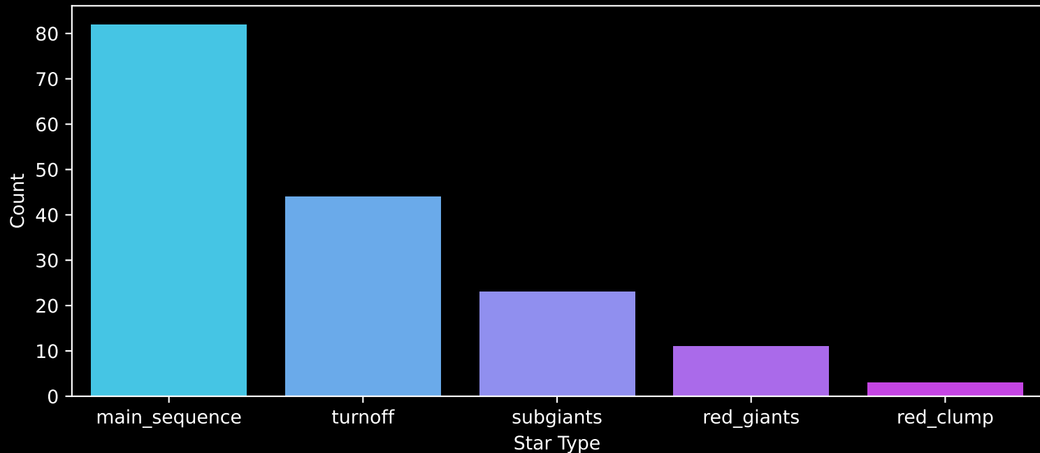
Gaia Cluster: [FSR_0496] Count plot of Star Type
