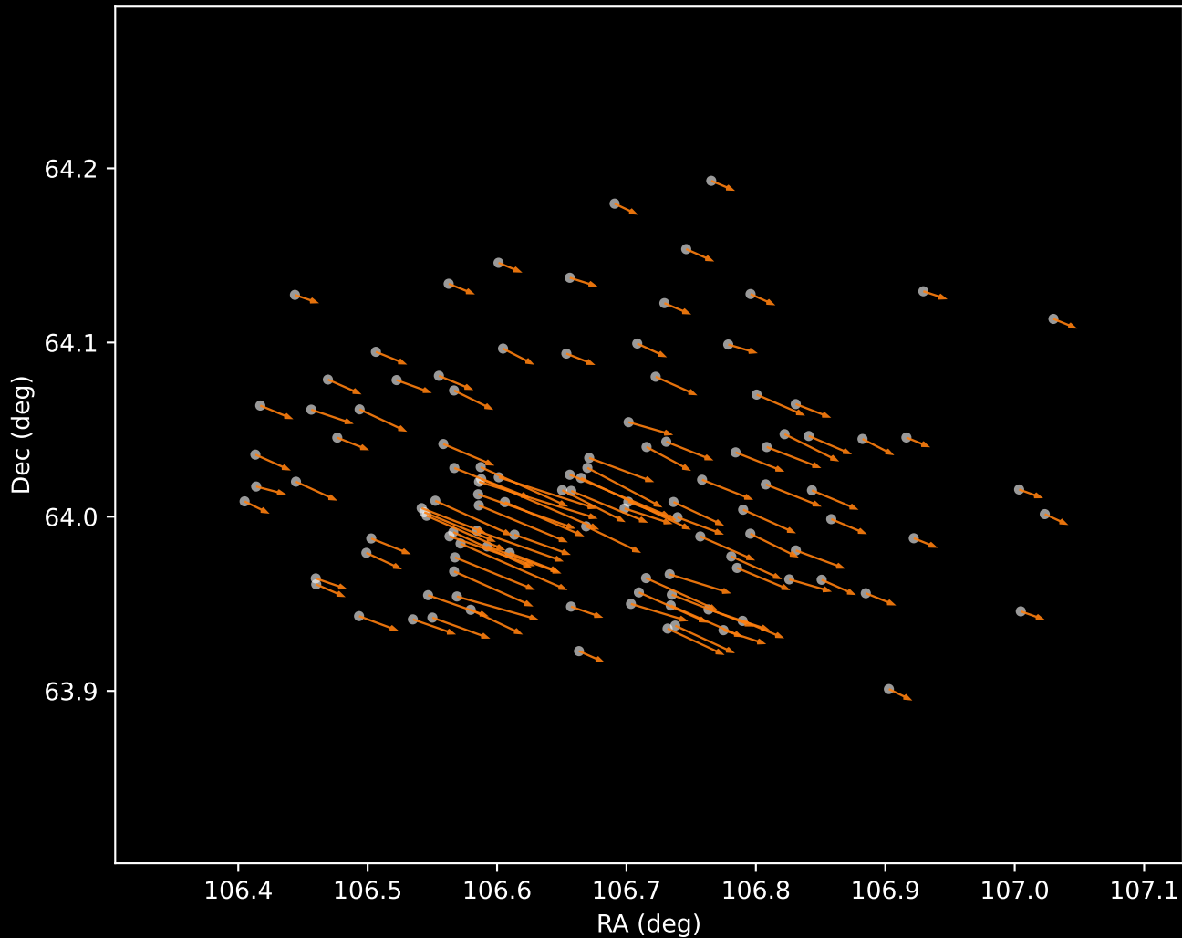
Gaia DR3 Cluster 2 Proper Motion Vectors (n=114)
