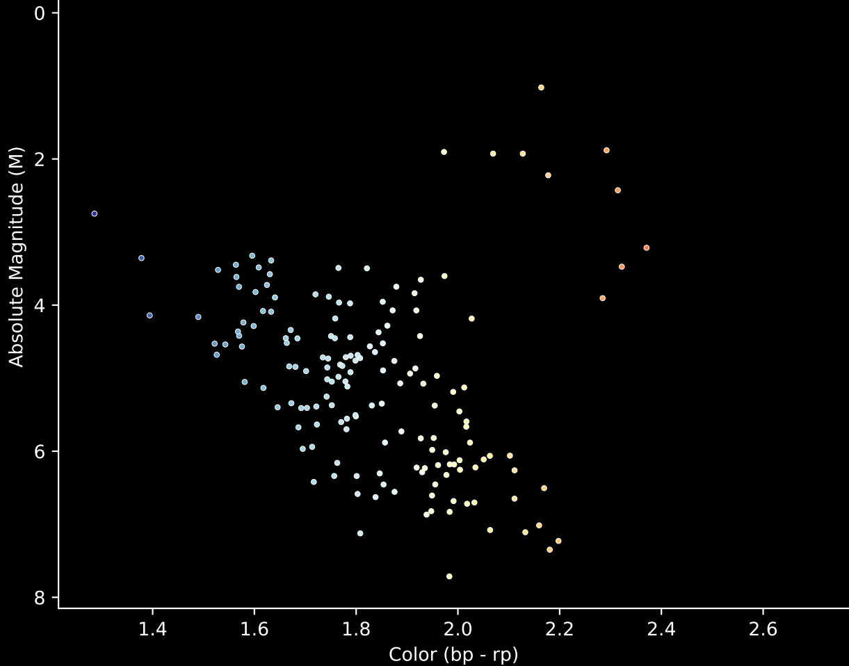
Gaia Cluster: [FSR_0496] Stars (n= 163) Hertzsprung-Russell Diagram
