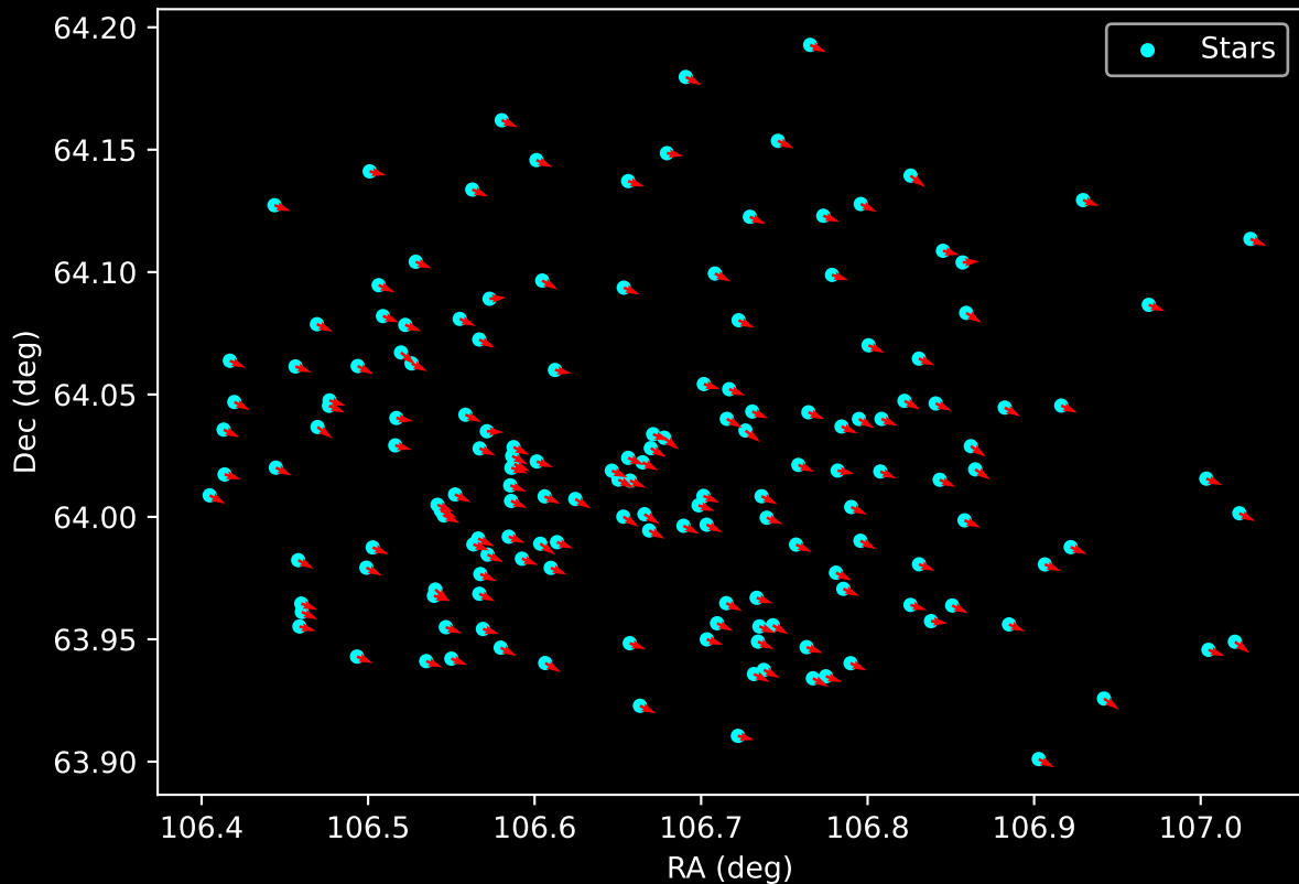
Gaia Cluster: [FSR_0496] Proper Motion Vectors for Gaia Star Field (n= 163)
