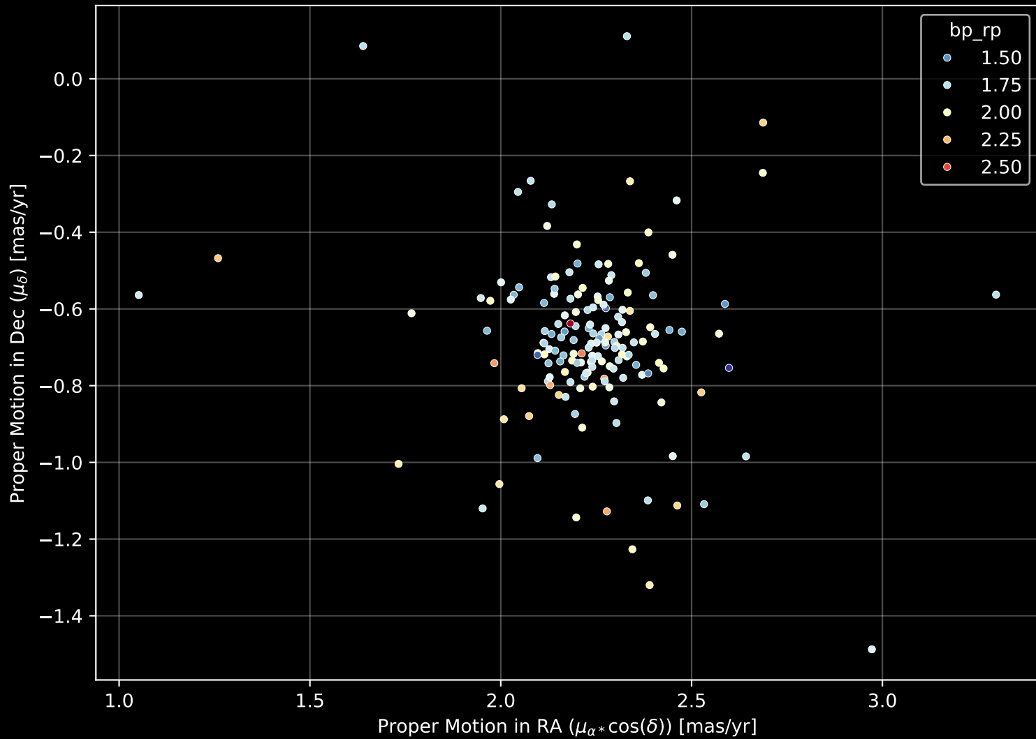
Gaia Cluster: [FSR_0496] Proper Motion Diagram (n= 163)
