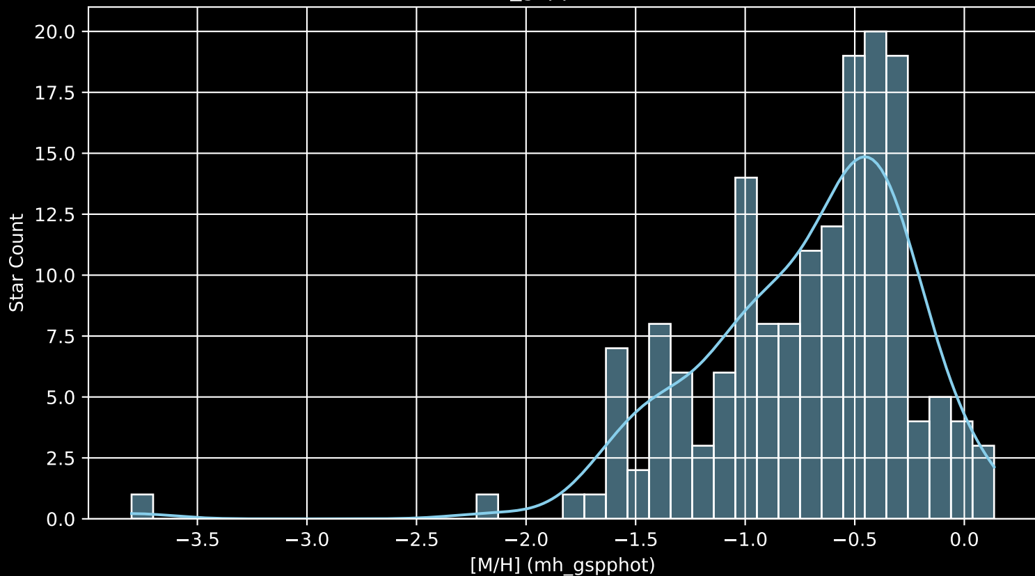
Gaia Cluster: [FSR_0496 [M/H] (mh_gspphot) (n= 163)
