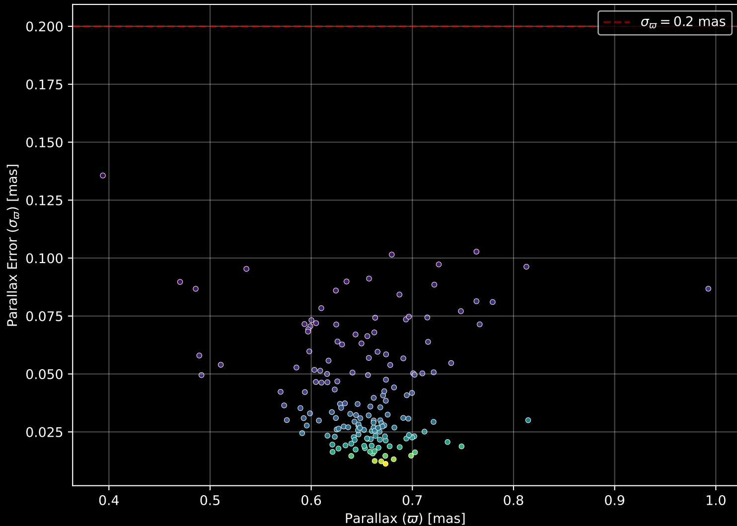
Gaia Cluster: [FSR_0496] Parallax Quality (n= 163)
