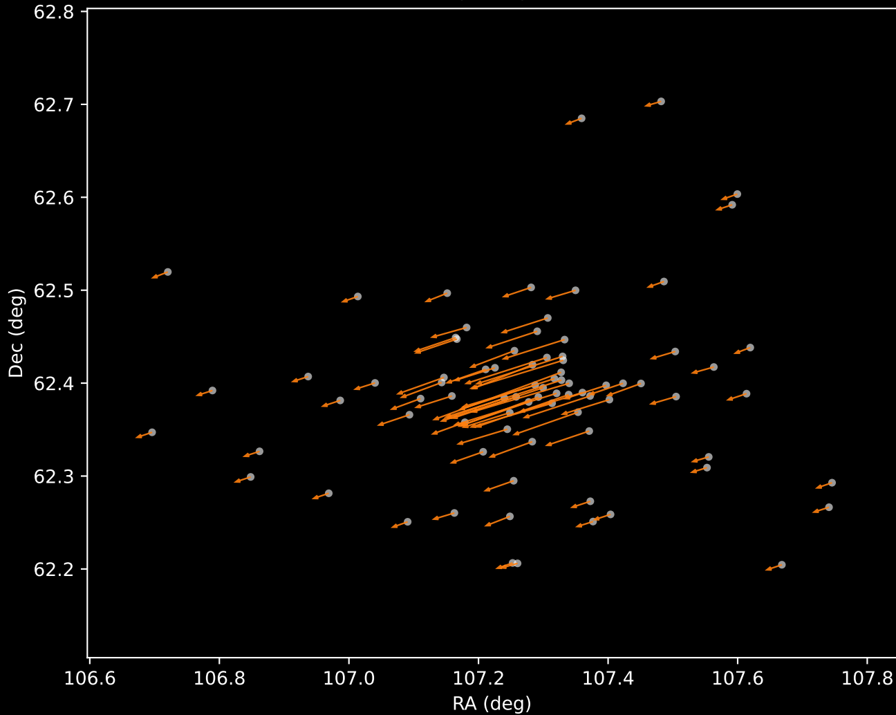
Gaia DR3 Cluster 2 Proper Motion Vectors (n=81)
