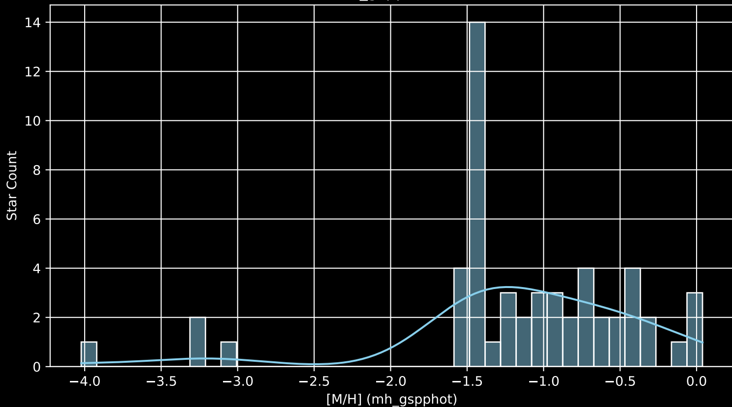
Gaia Cluster: [FSR_0524 [M/H] (mh_gspphot) (n= 54)
