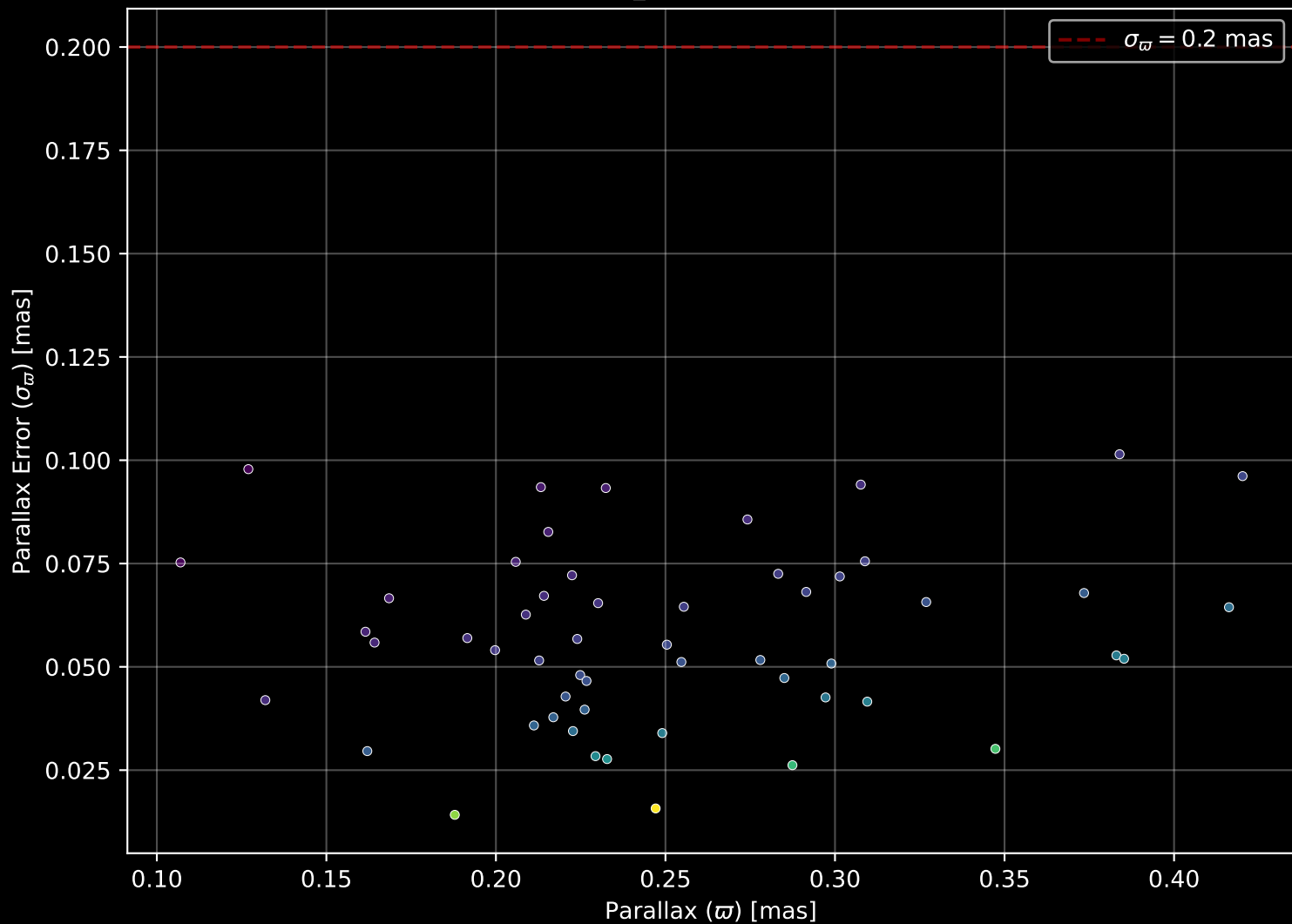
Gaia Cluster: [FSR_0524] Parallax Quality (n= 54)
