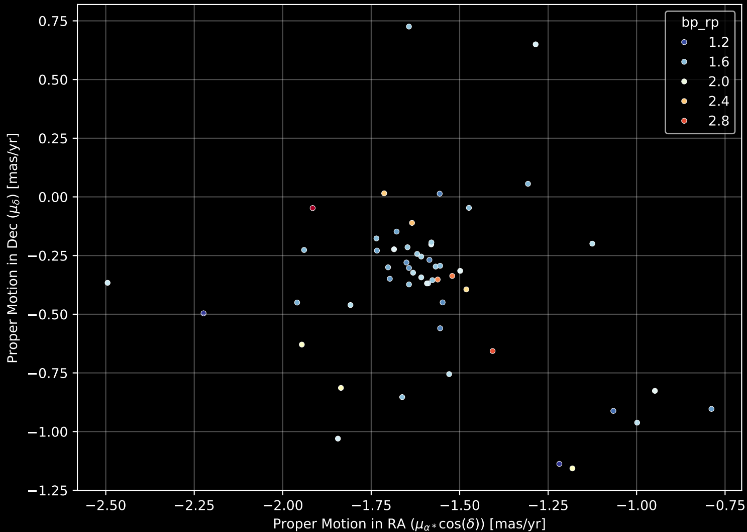
Gaia Cluster: [FSR_0524] Proper Motion Diagram (n= 54)
