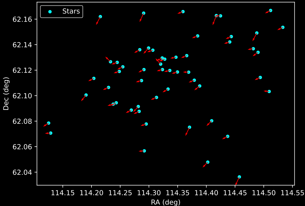
Gaia Cluster: [FSR_0524] Proper Motion Vectors for Gaia Star Field (n= 54)
