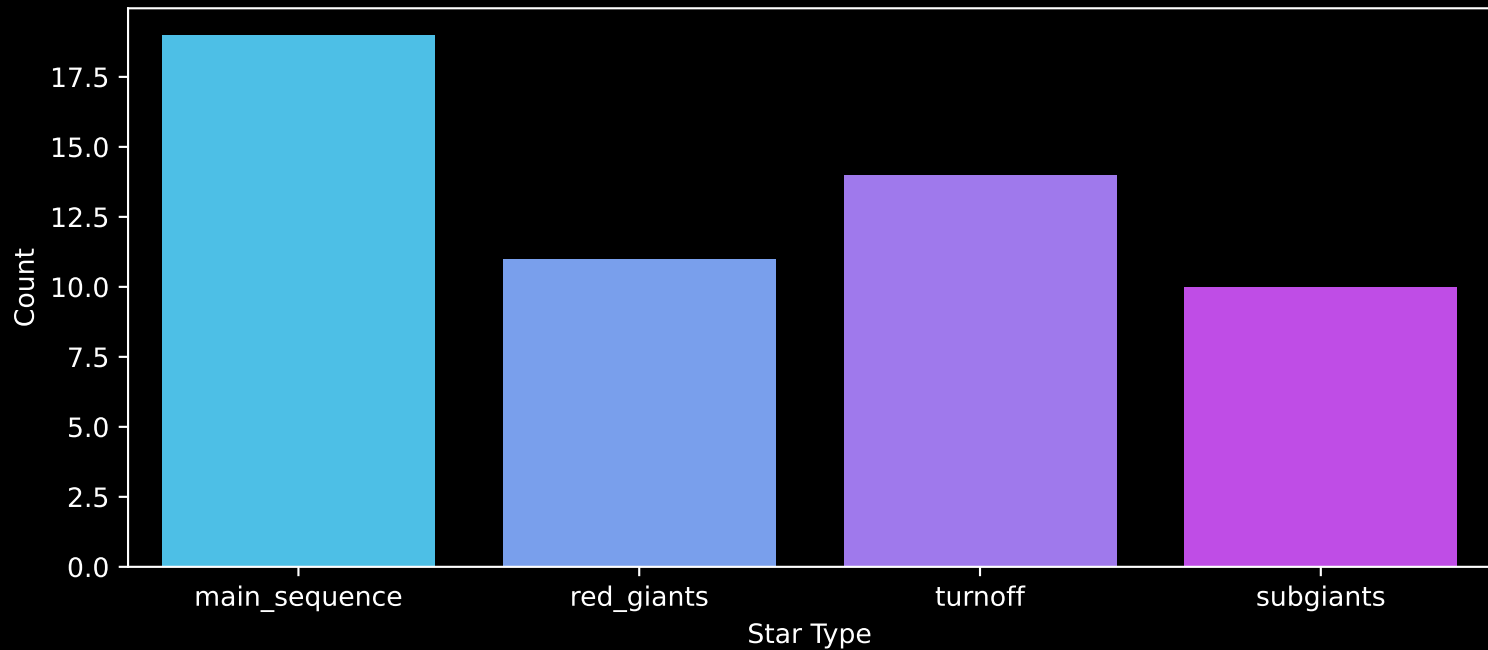
Gaia Cluster: [FSR_0524] Count plot of Star Type
