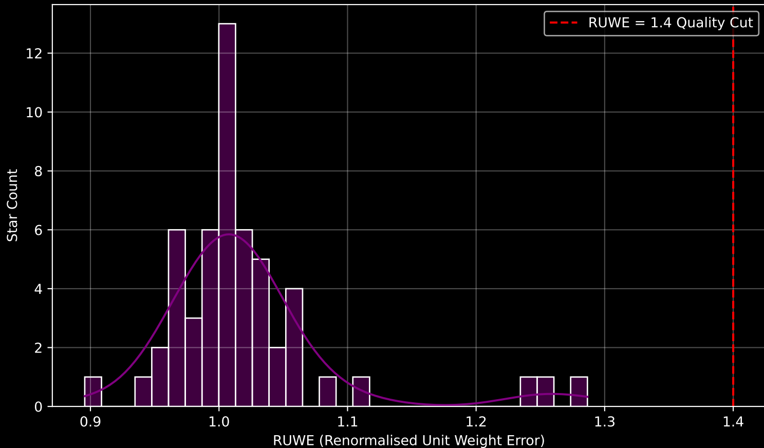
Gaia Cluster: [FSR_0524] RUWE Distribution (n= 54)
