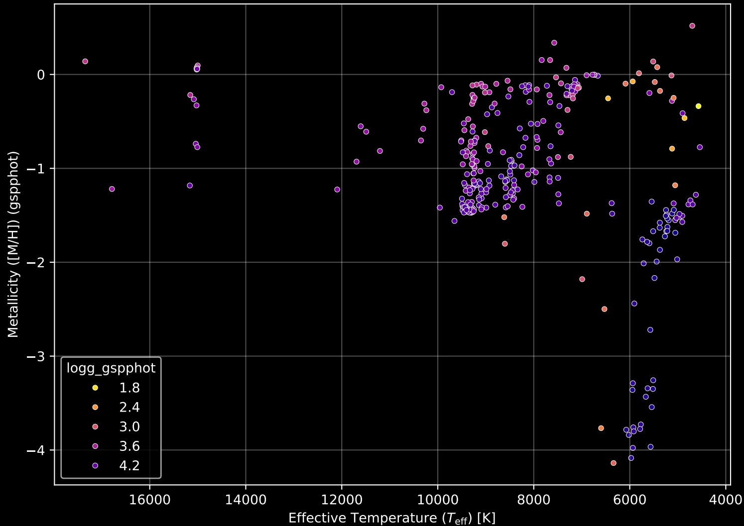
Gaia Cluster: [FSR_0542] Stellar Population Parameters (n= 324)
