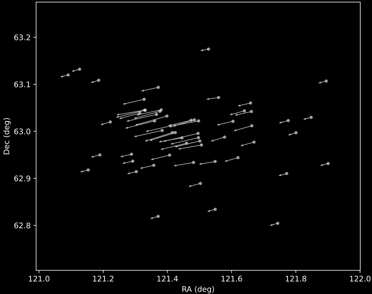
Gaia DR3 Cluster 15 Proper Motion Vectors (n=56)
