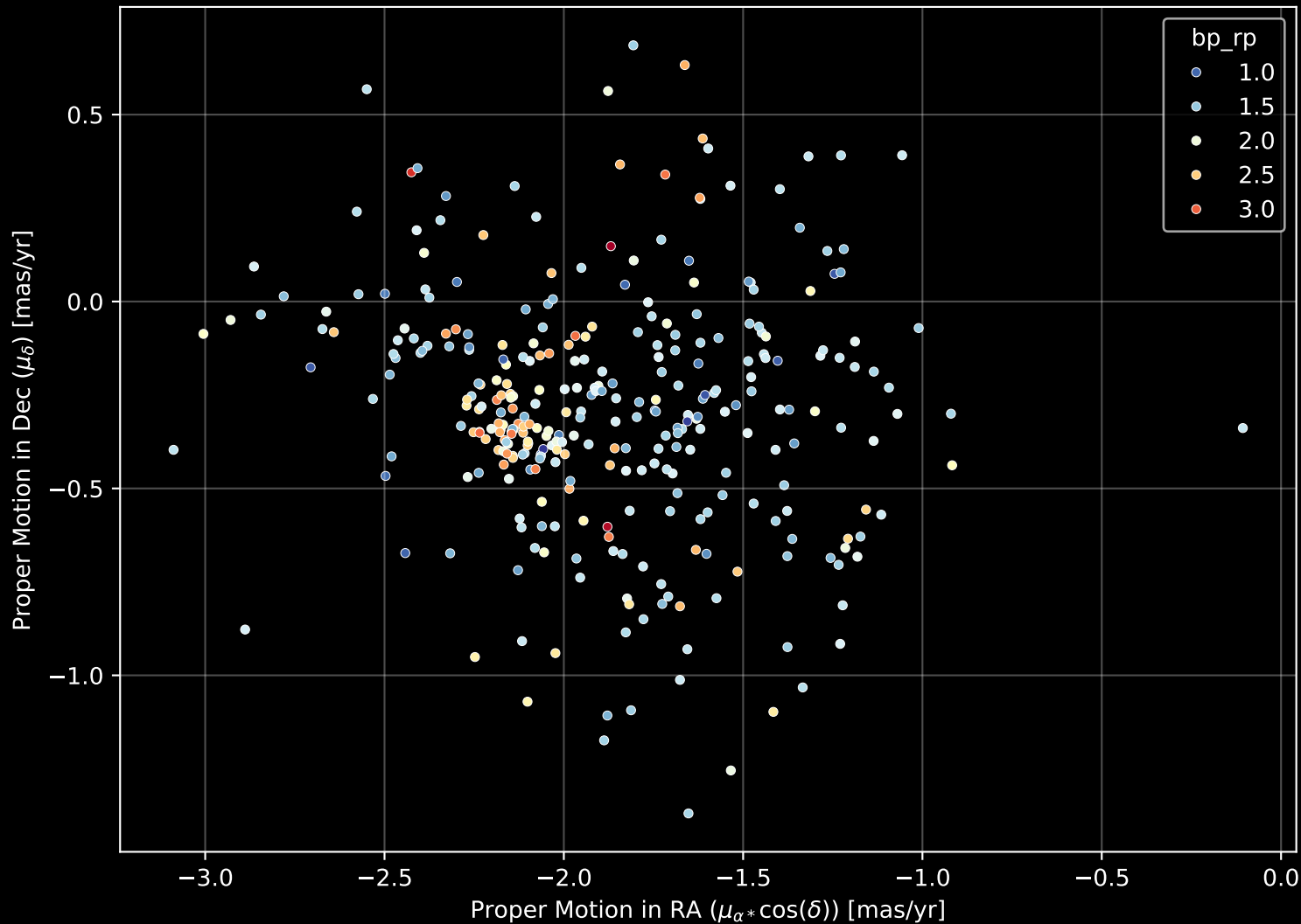
Gaia Cluster: [FSR_0542] Proper Motion Diagram (n= 324)
