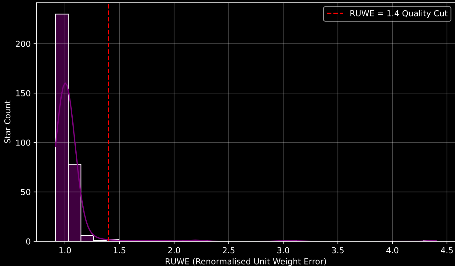
Gaia Cluster: [FSR_0542] RUWE Distribution (n= 324)
