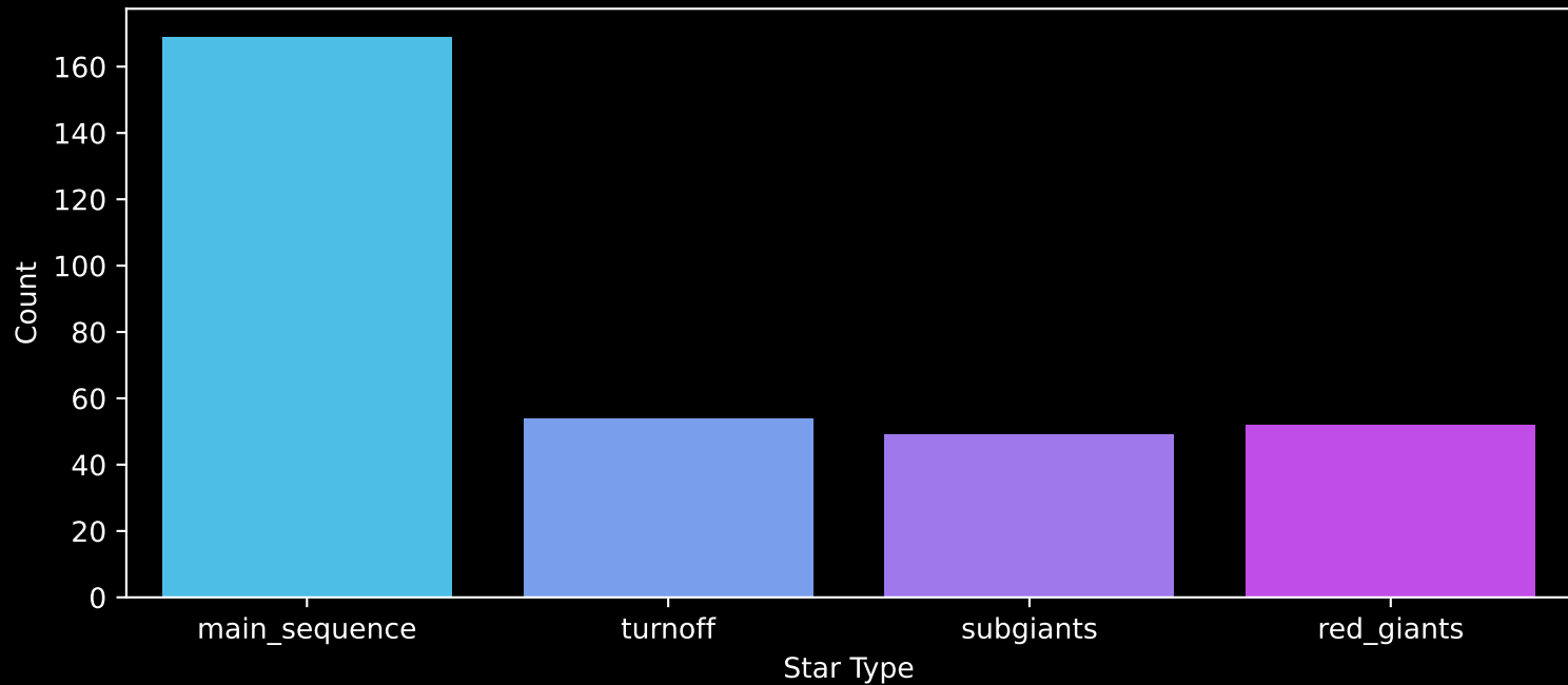
Gaia Cluster: [FSR_0542] Count plot of Star Type
