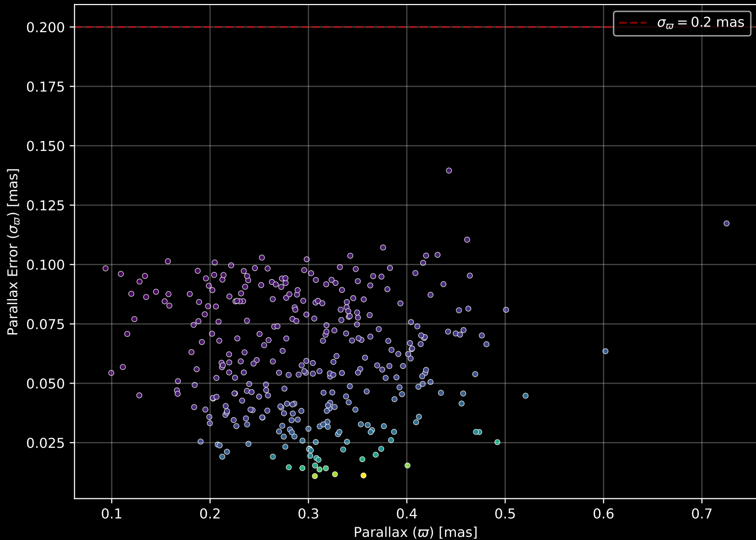
Gaia Cluster: [FSR_0542] Parallax Quality (n= 324)
