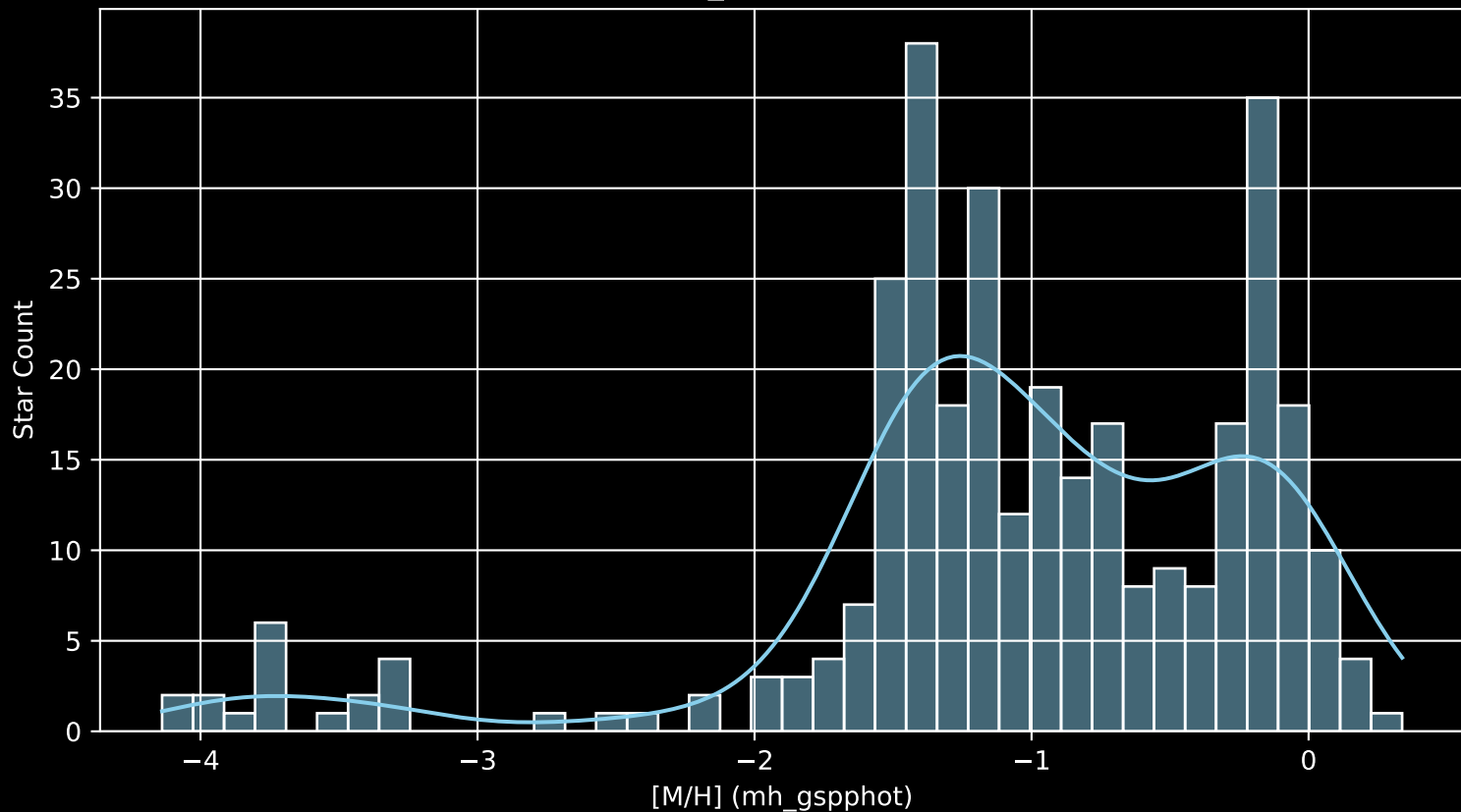
Gaia Cluster: [FSR_0542 [M/H] (mh_gspphot) (n= 323)
