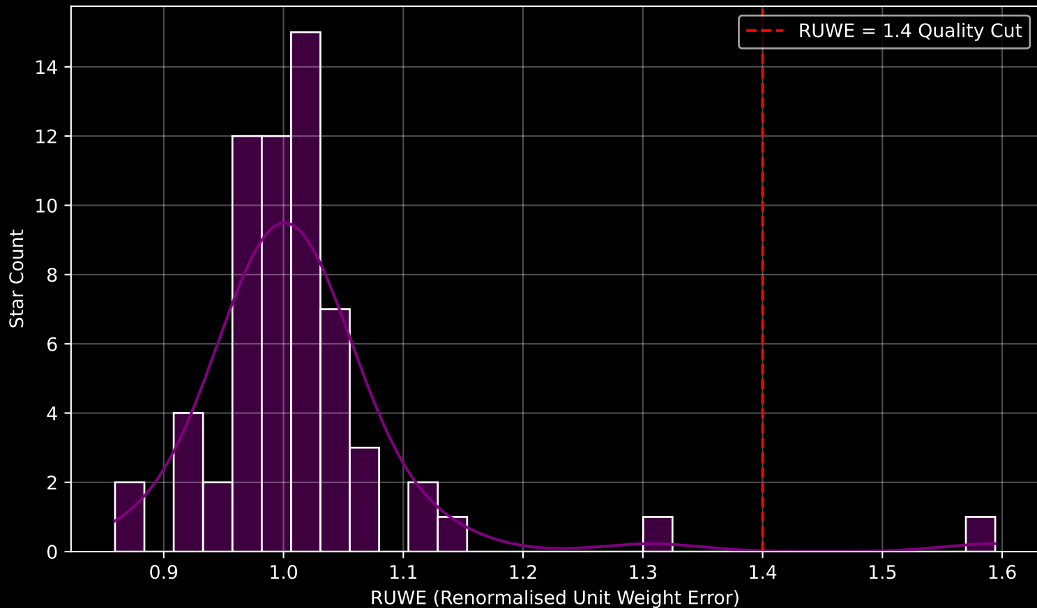
Gaia Cluster: [FSR_0551] RUWE Distribution (n= 62)
