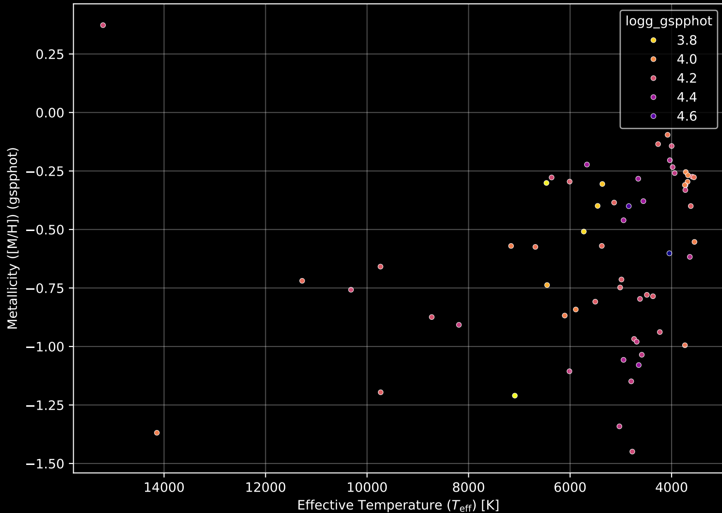
Gaia Cluster: [FSR_0551] Stellar Population Parameters (n= 62)
