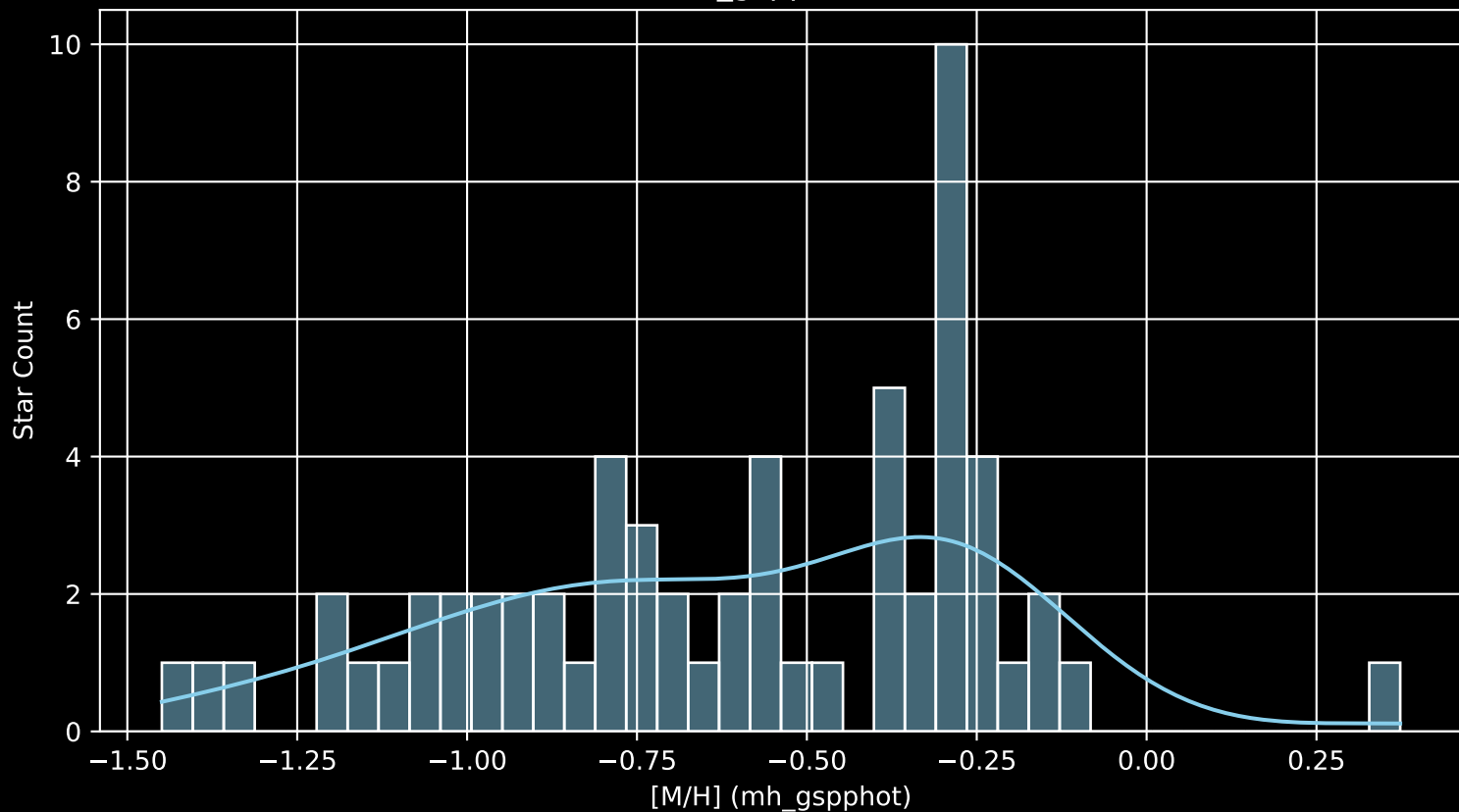
Gaia Cluster: [FSR_0551 [M/H] (mh_gspphot) (n= 62)
