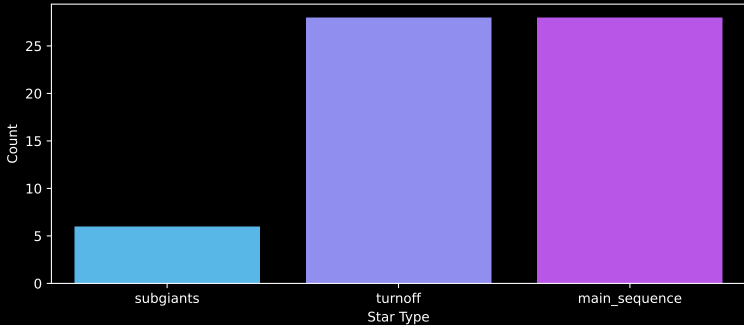
Gaia Cluster: [FSR_0551] Count plot of Star Type
