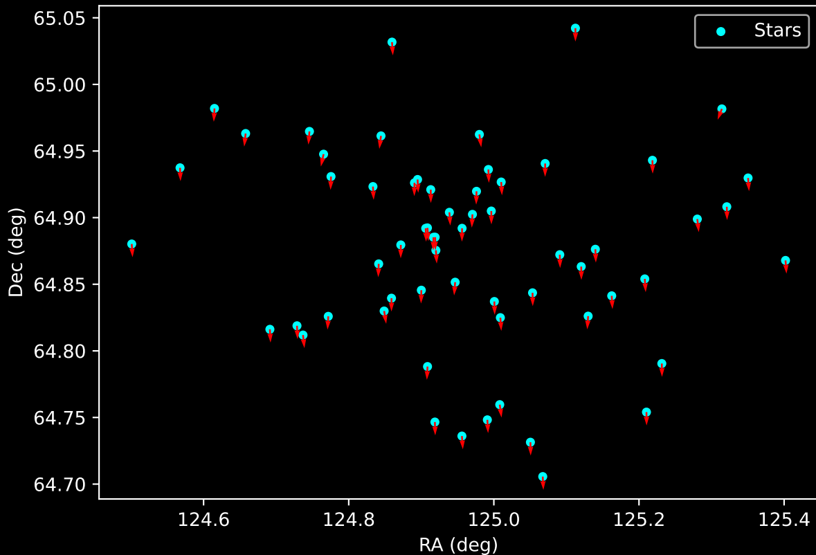
Gaia Cluster: [FSR_0551] Proper Motion Vectors for Gaia Star Field (n= 62)
