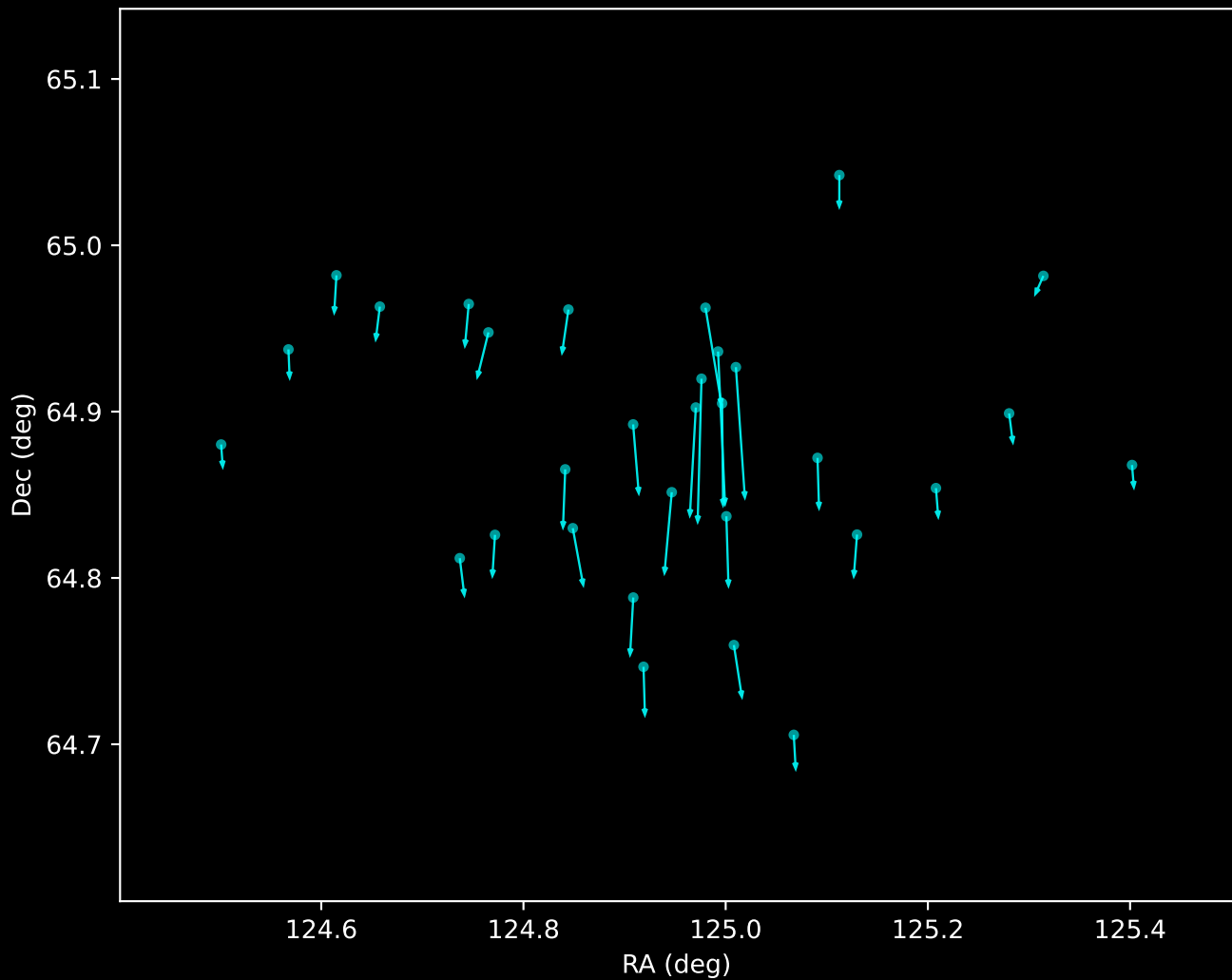
Gaia DR3 Noise Stream Proper Motion Vectors (n=31)
