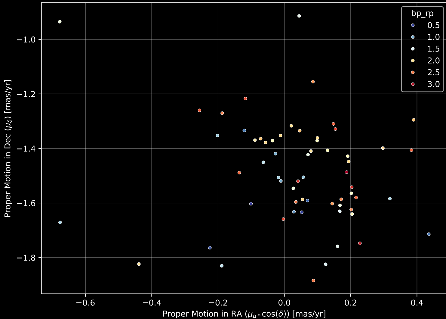
Gaia Cluster: [FSR_0551] Proper Motion Diagram (n= 62)
