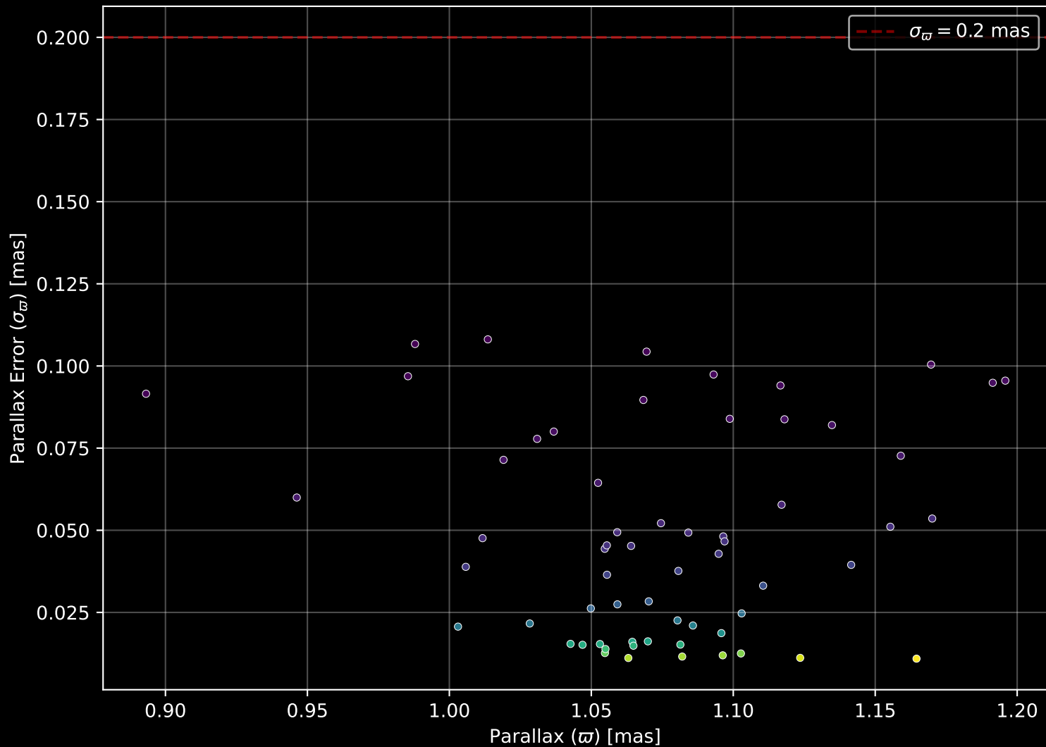
Gaia Cluster: [FSR_0551] Parallax Quality (n= 62)
