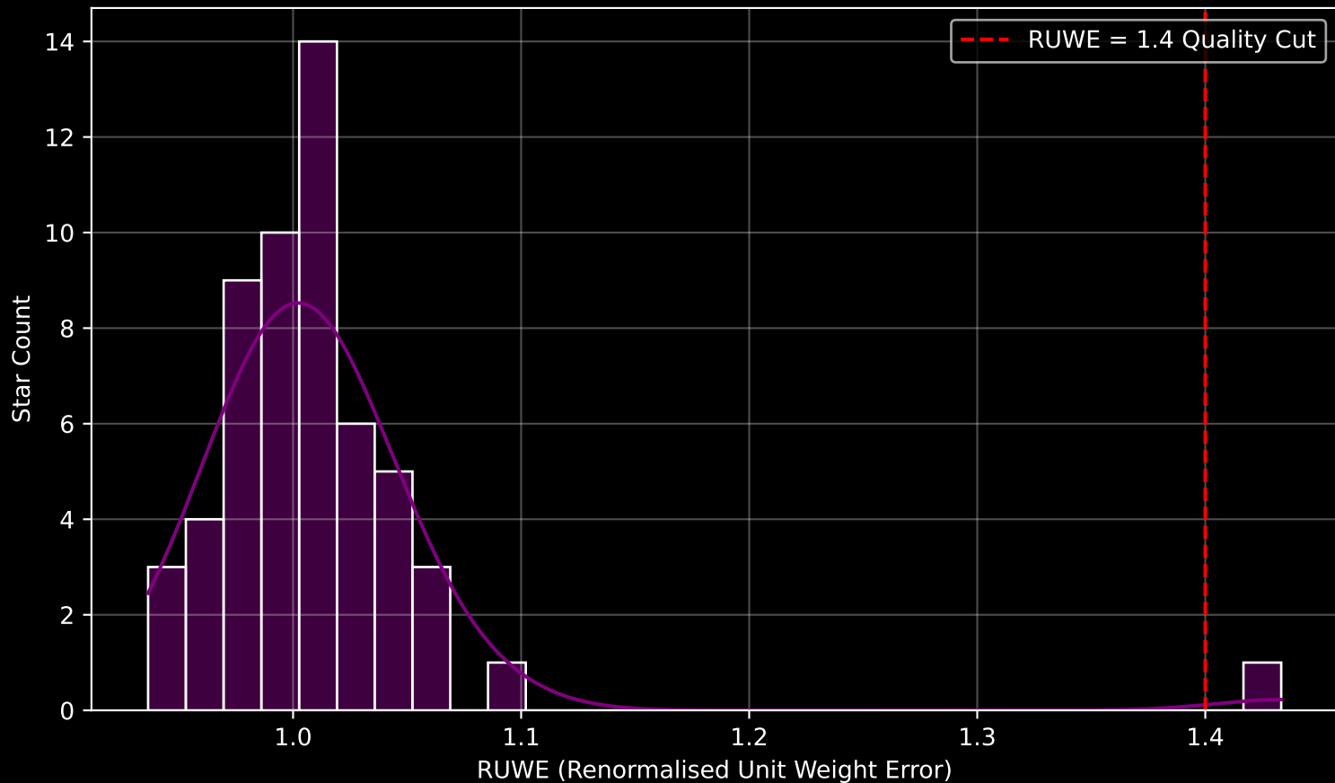
Gaia Cluster: [FSR_0553] RUWE Distribution (n= 56)
