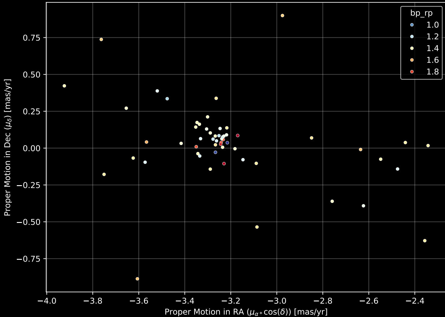
Gaia Cluster: [FSR_0553] Proper Motion Diagram (n= 56)
