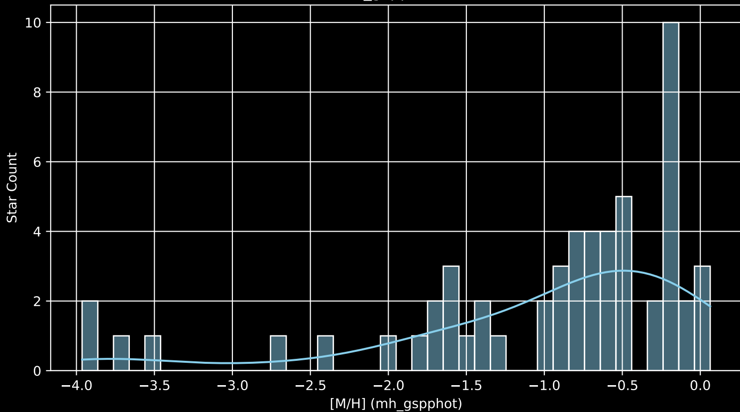
Gaia Cluster: [FSR_0553 [M/H] (mh_gspphot) (n= 56)
