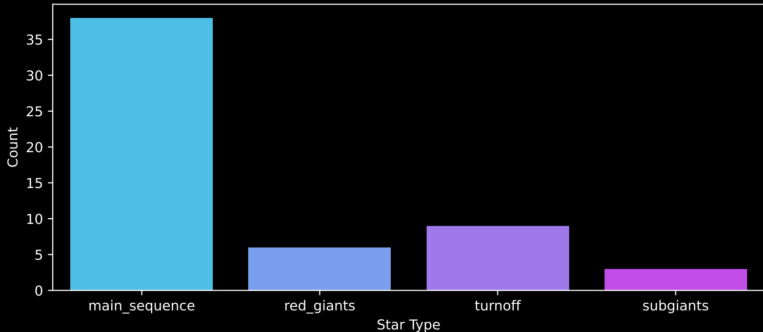
Gaia Cluster: [FSR_0553] Count plot of Star Type
