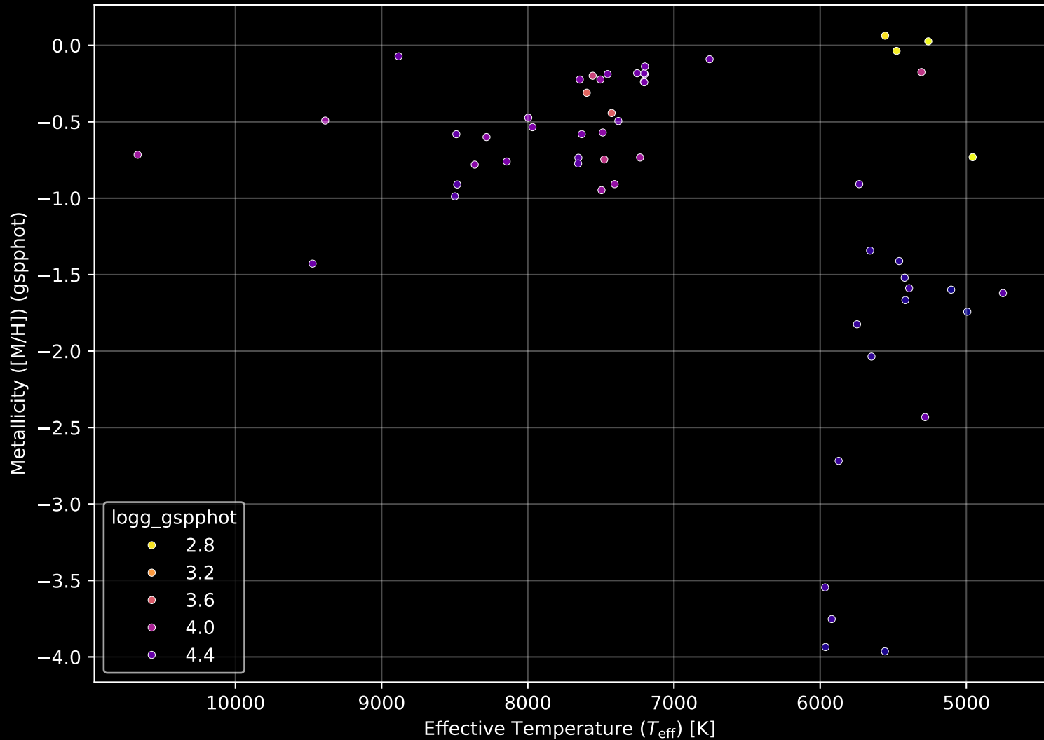
Gaia Cluster: [FSR_0553] Stellar Population Parameters (n= 56)
