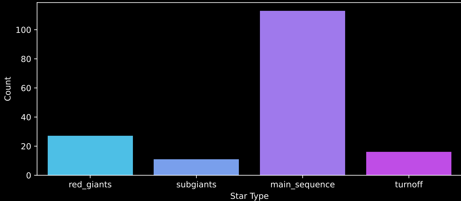
Gaia Cluster: [FSR_0558] Count plot of Star Type
