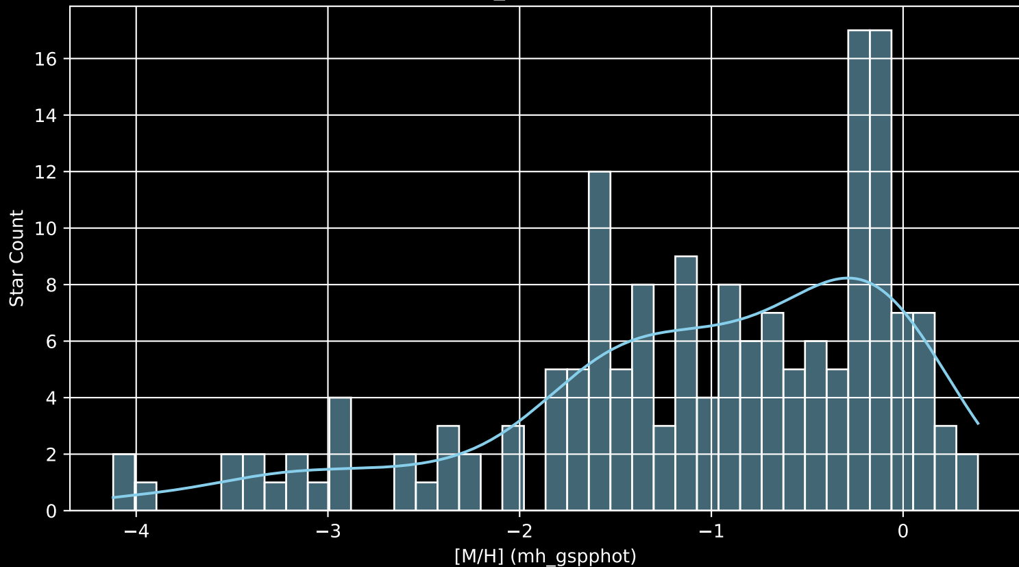
Gaia Cluster: [FSR_0558 [M/H] (mh_gspphot) (n= 167)
