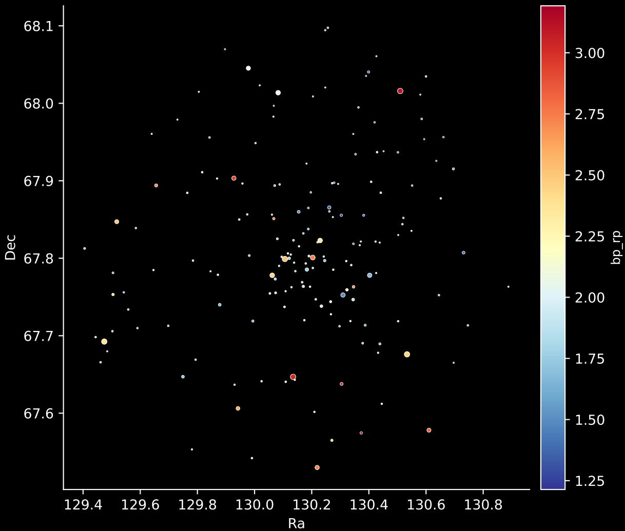
Gaia Cluster: [FSR_0558] Stars: 167
