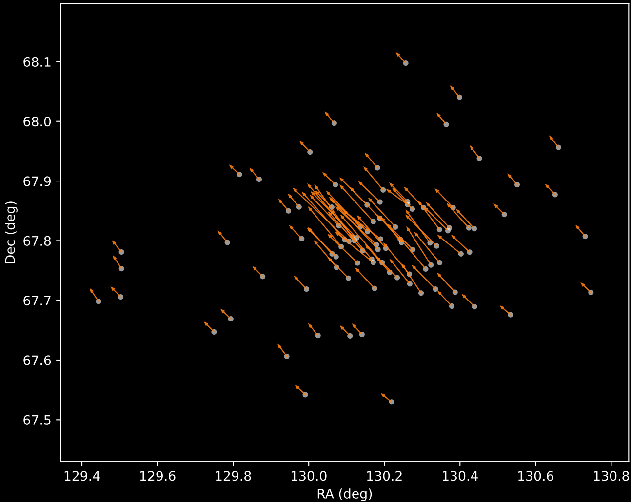
Gaia DR3 Cluster 2 Proper Motion Vectors (n=94)
