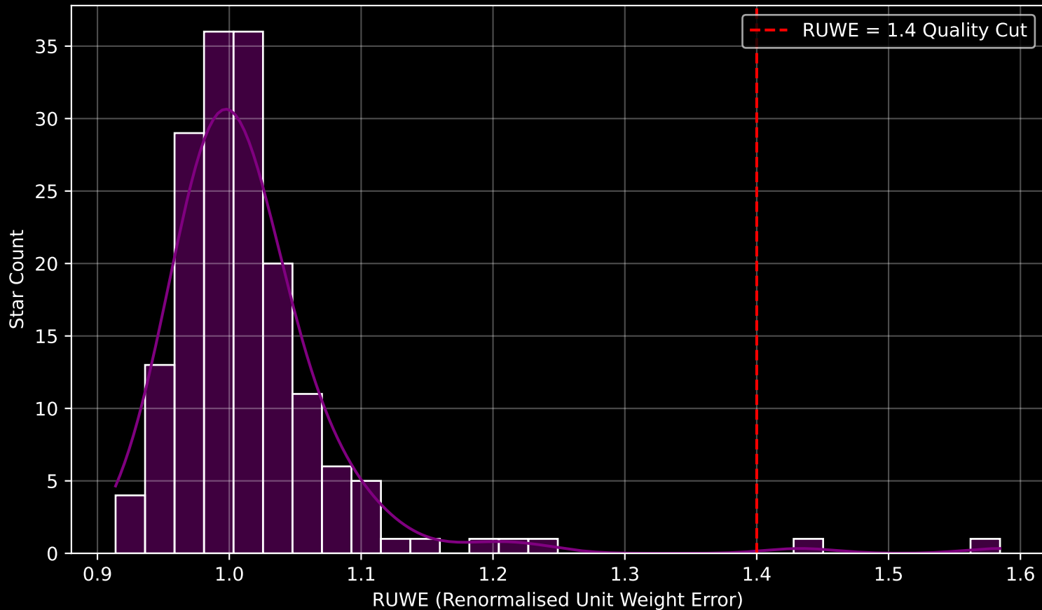
Gaia Cluster: [FSR_0558] RUWE Distribution (n= 167)
