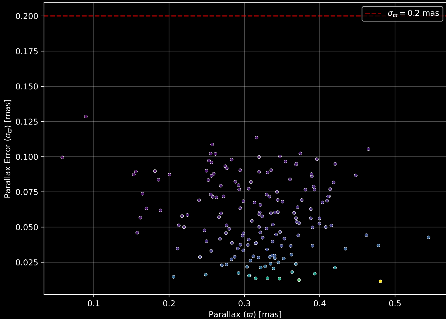
Gaia Cluster: [FSR_0558] Parallax Quality (n= 167)
