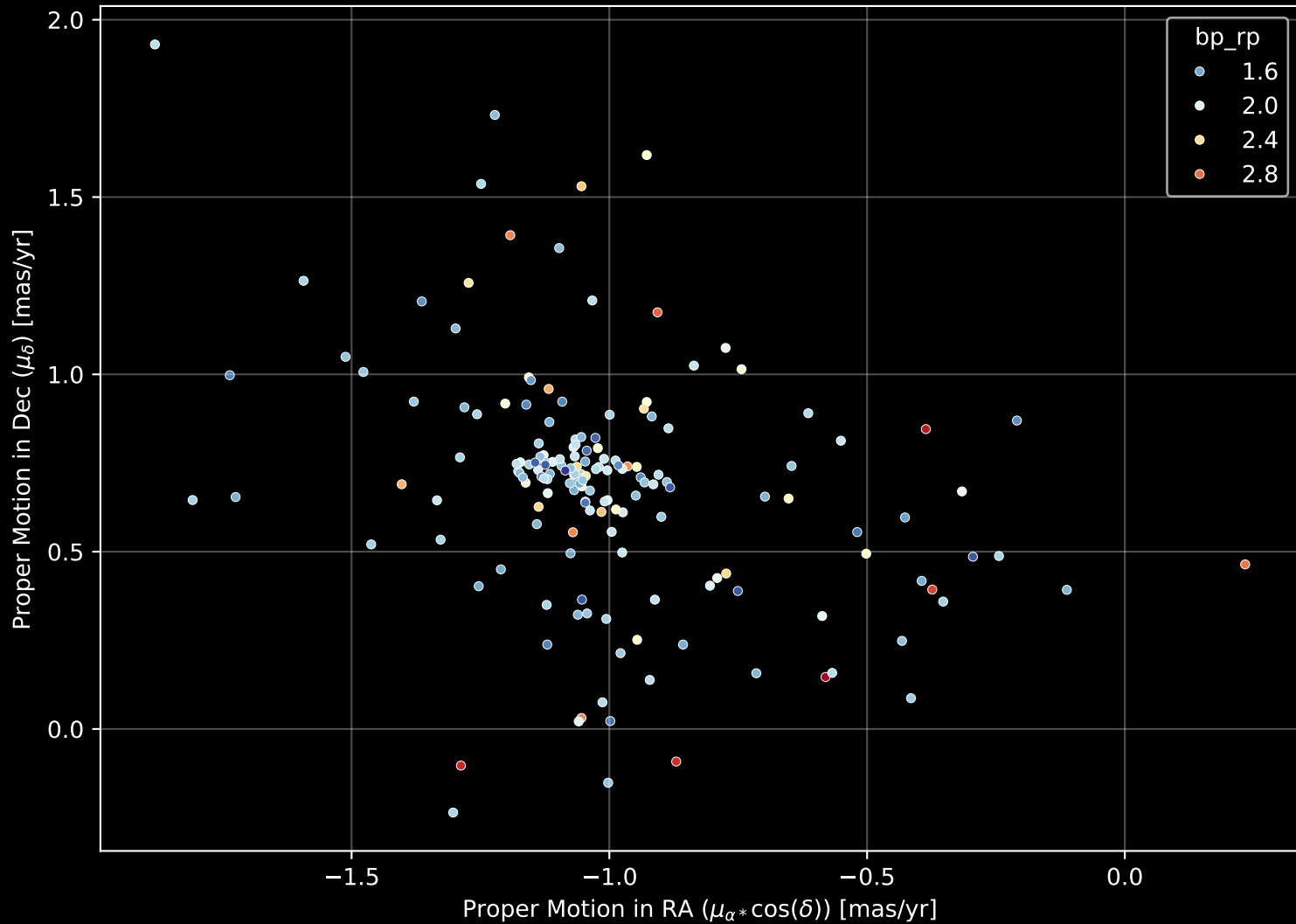
Gaia Cluster: [FSR_0558] Proper Motion Diagram (n= 167)
