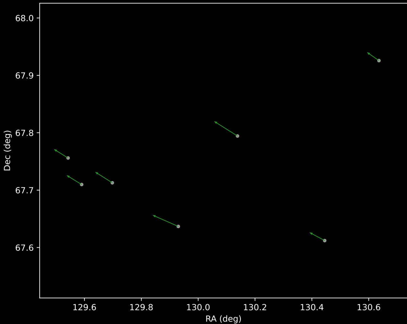
Gaia DR3 Cluster 4 Proper Motion Vectors (n=7)
