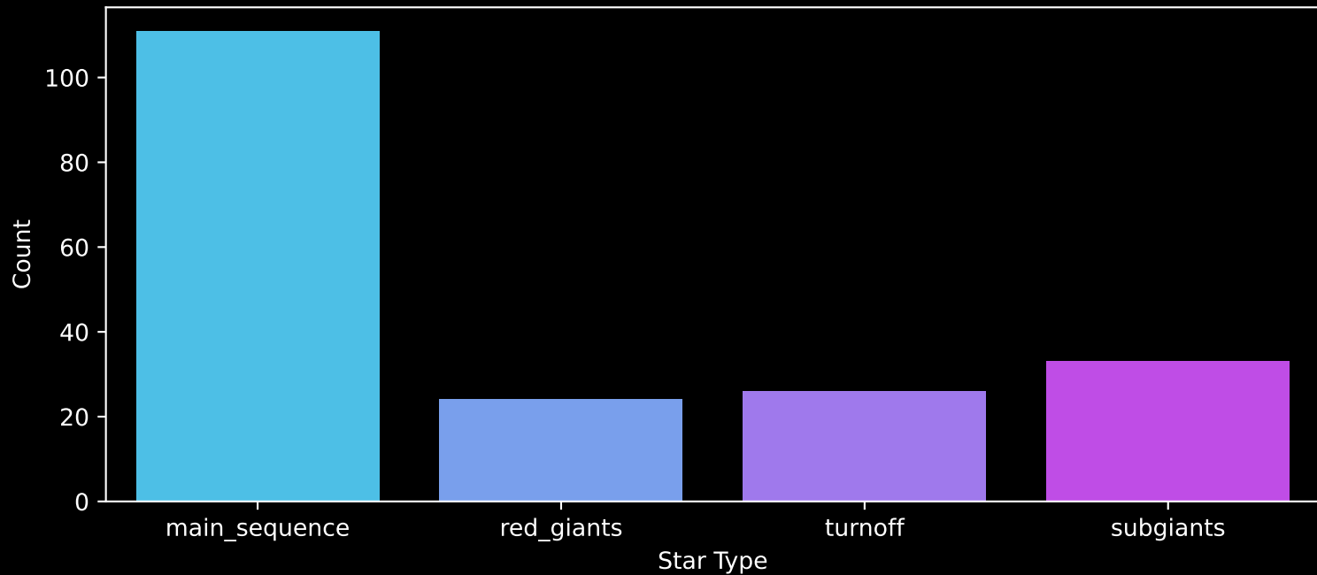
Gaia Cluster: [FSR_0826] Count plot of Star Type
