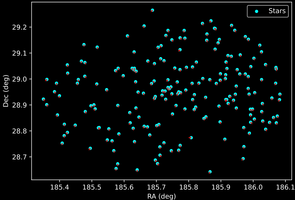
Gaia Cluster: [FSR_0826] Proper Motion Vectors for Gaia Star Field (n= 194)
