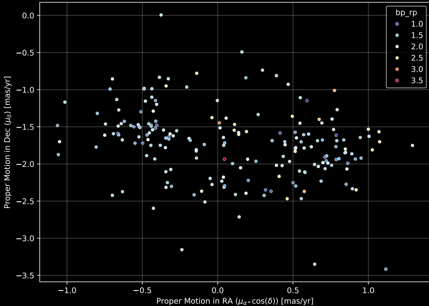
Gaia Cluster: [FSR_0826] Proper Motion Diagram (n= 194)
