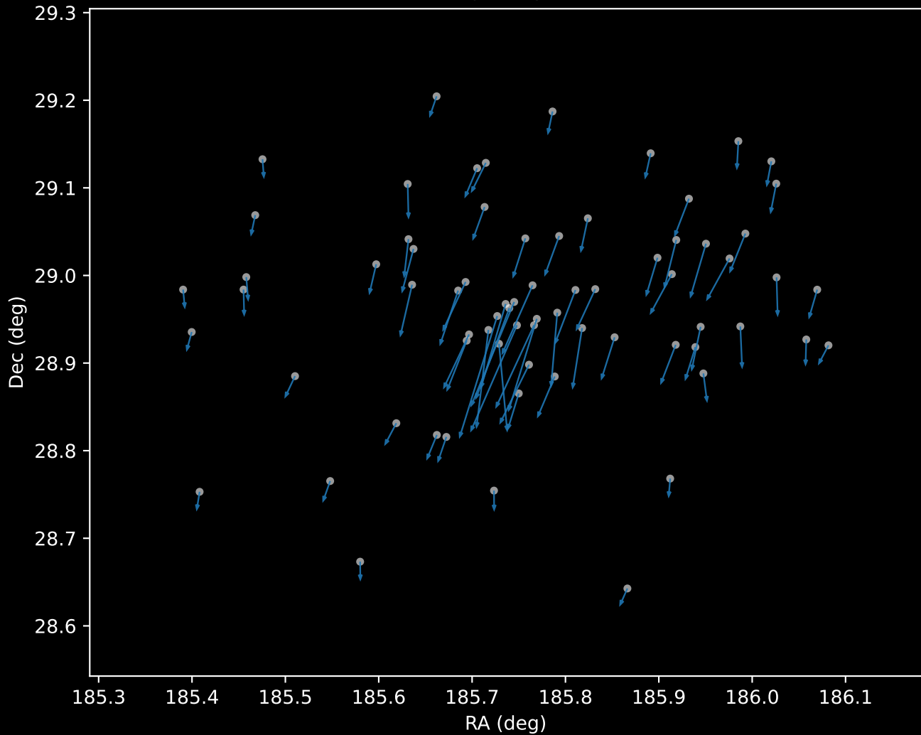
Gaia DR3 Cluster 0 Proper Motion Vectors (n=71)
