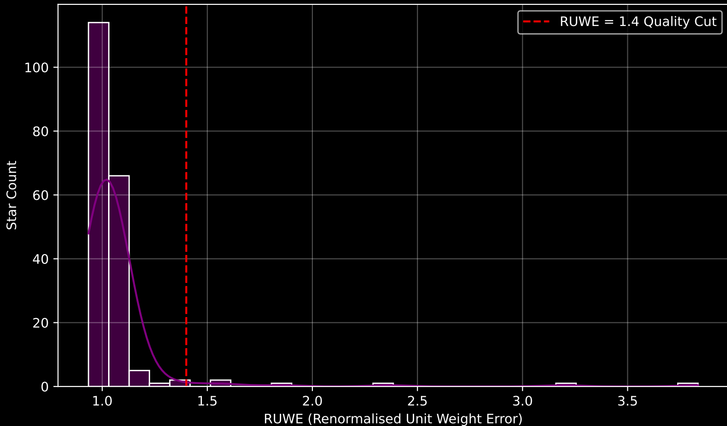
Gaia Cluster: [FSR_0826] RUWE Distribution (n= 194)
