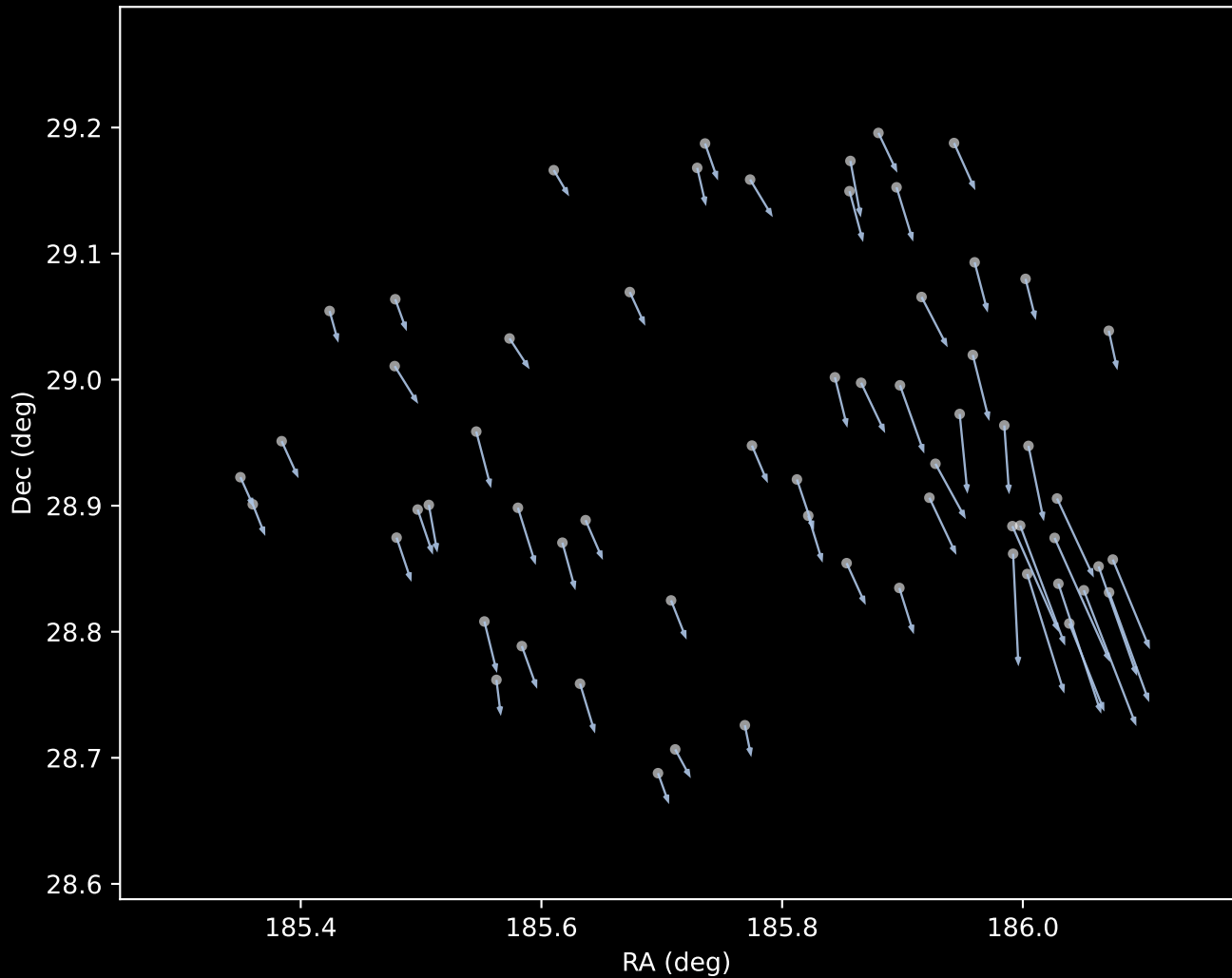
Gaia DR3 Cluster 1 Proper Motion Vectors (n=62)
