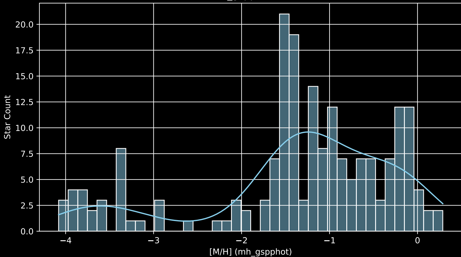
Gaia Cluster: [FSR_0826 [M/H] (mh_gspphot) (n= 192)
