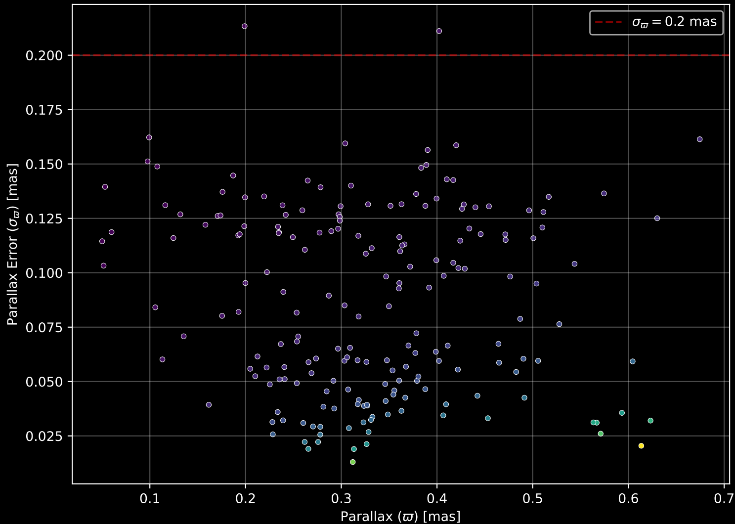
Gaia Cluster: [FSR_0826] Parallax Quality (n= 194)
