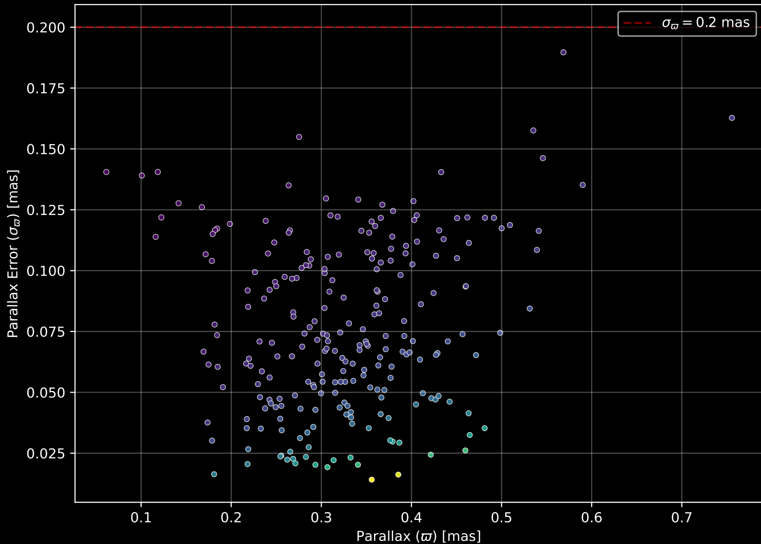
Gaia Cluster: [FSR_0852] Parallax Quality (n= 240)
