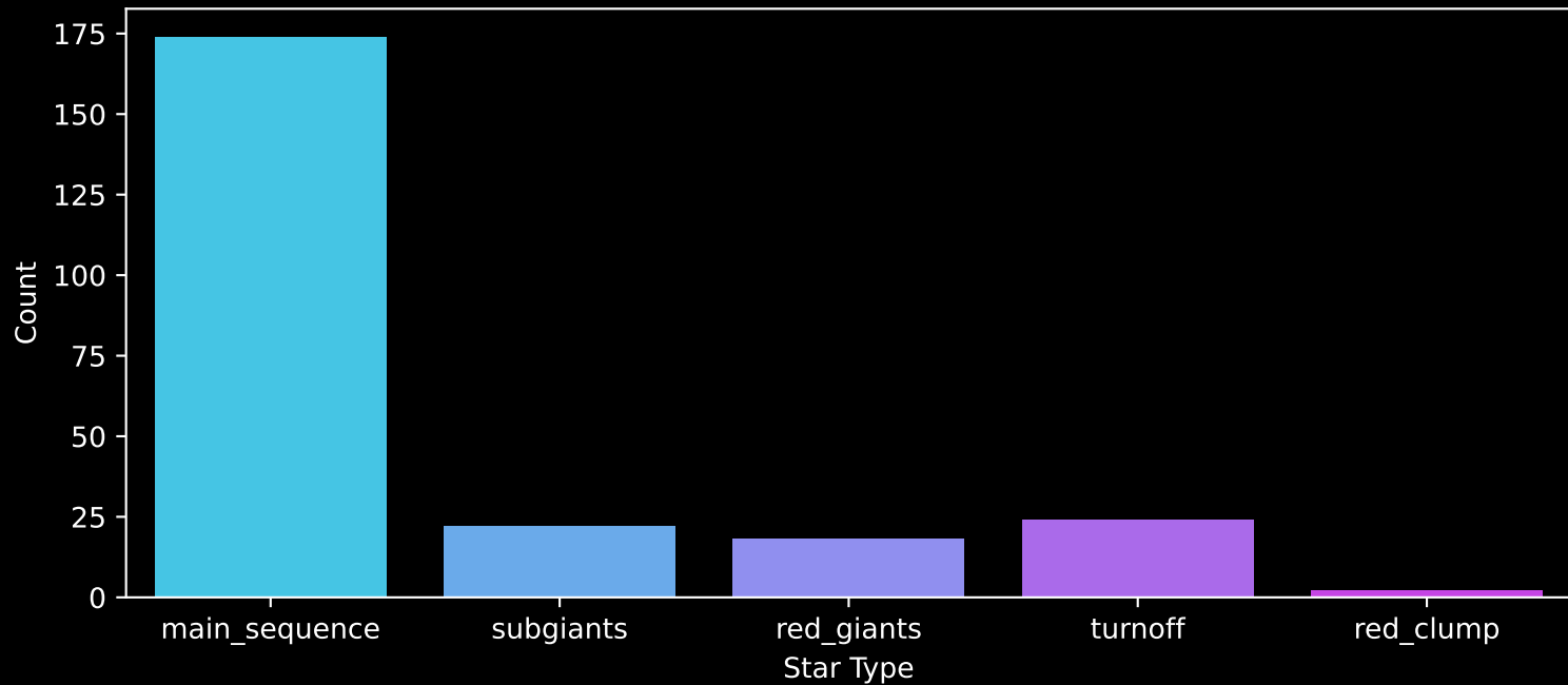
Gaia Cluster: [FSR_0852] Count plot of Star Type
