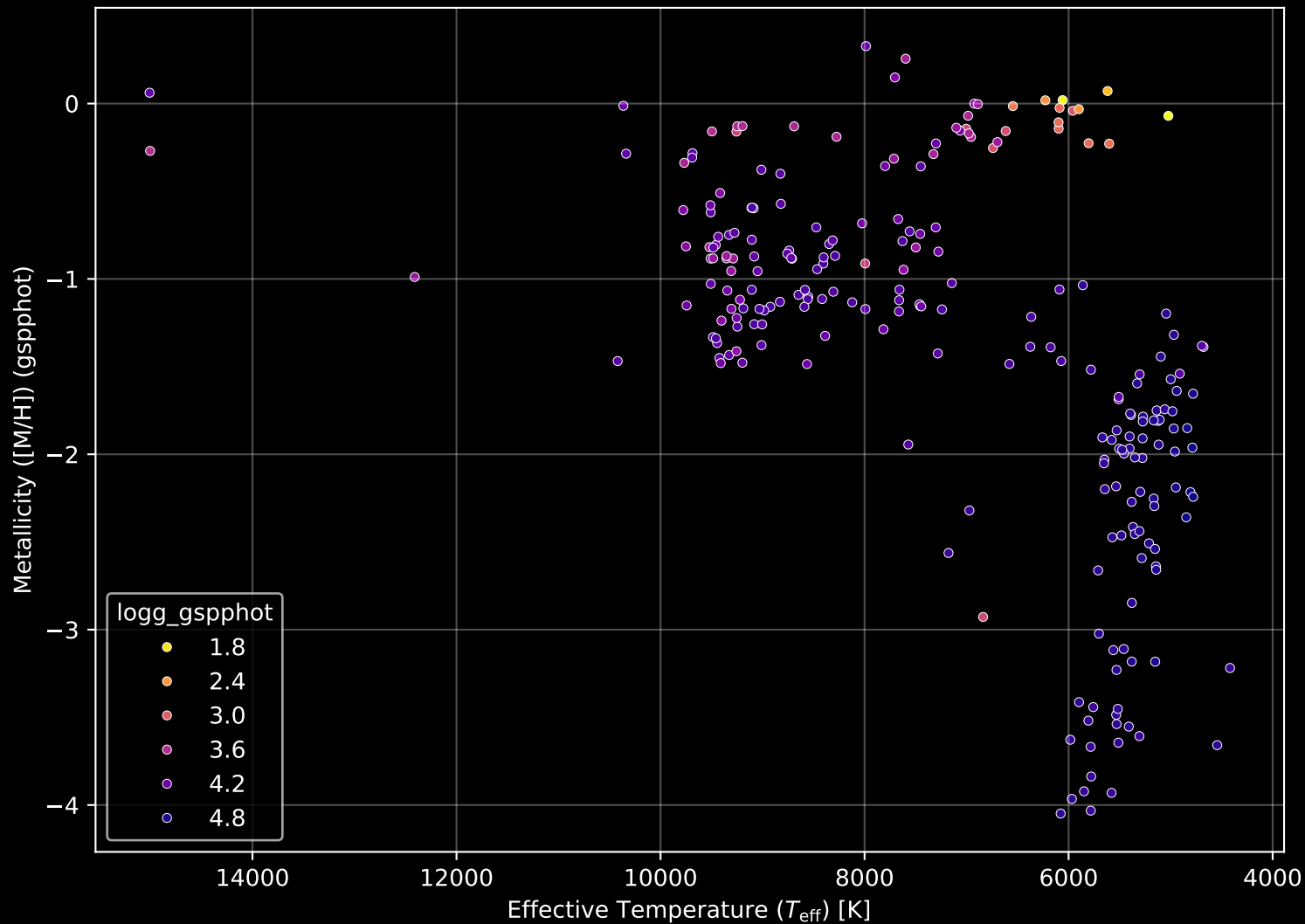
Gaia Cluster: [FSR_0852] Stellar Population Parameters (n= 240)
