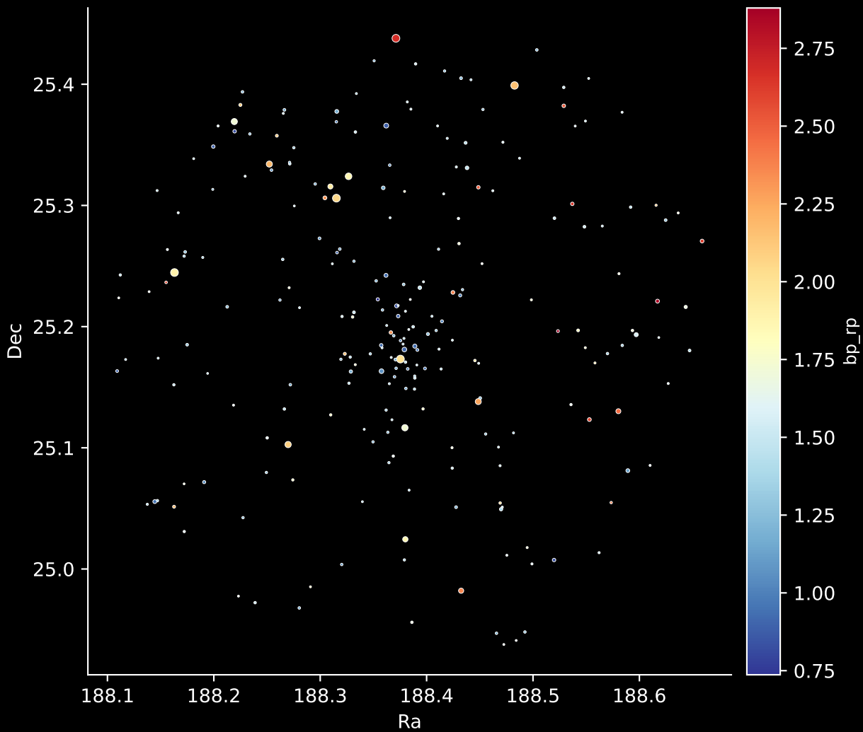
Gaia Cluster: [FSR_0852] Stars: 240
