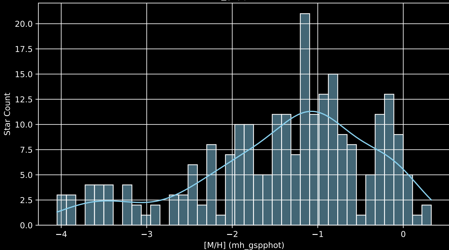
Gaia Cluster: [FSR_0852 [M/H] (mh_gspphot) (n= 240)
