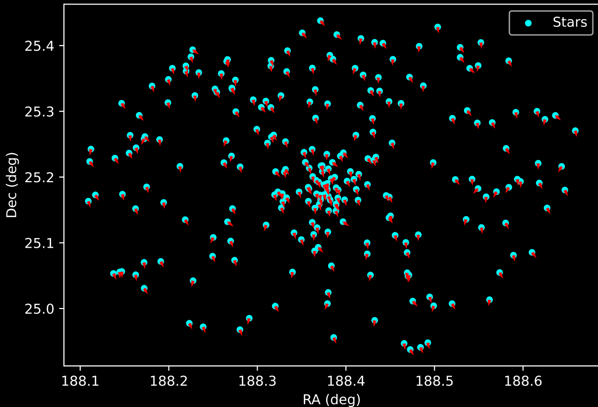
Gaia Cluster: [FSR_0852] Proper Motion Vectors for Gaia Star Field (n= 240)
