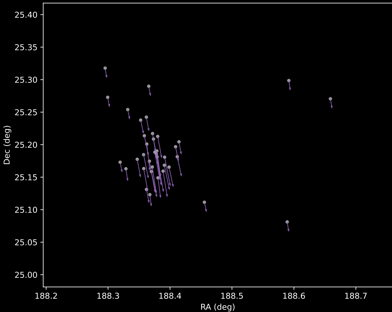
Gaia DR3 Cluster 8 Proper Motion Vectors (n=37)
