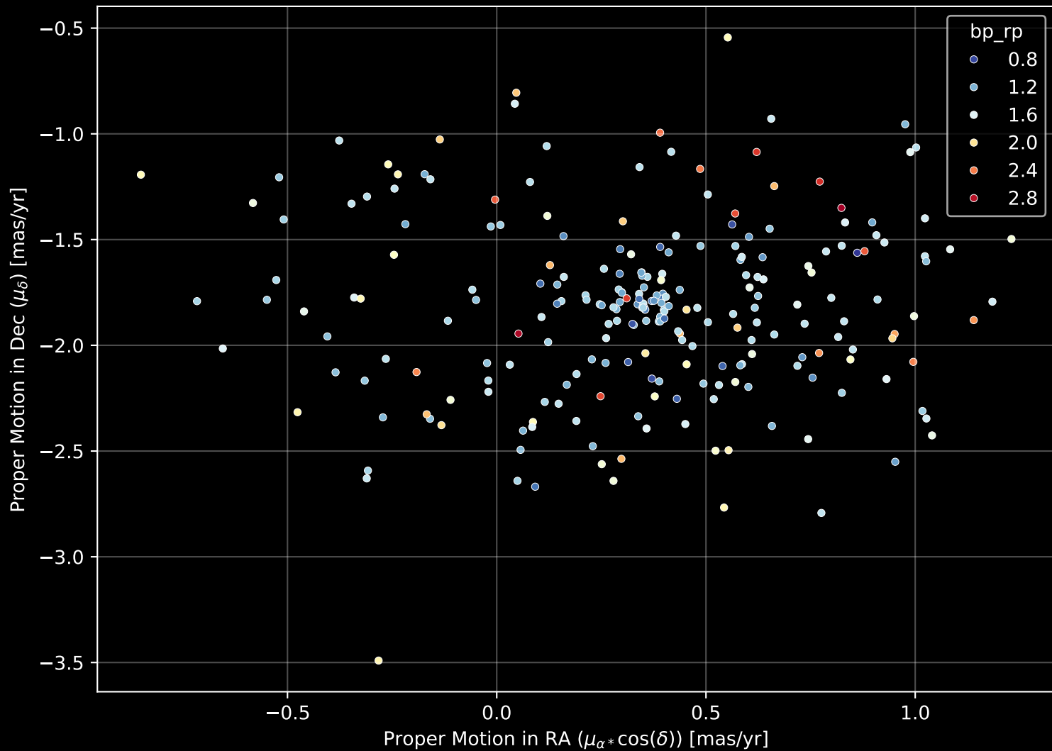
Gaia Cluster: [FSR_0852] Proper Motion Diagram (n= 240)
