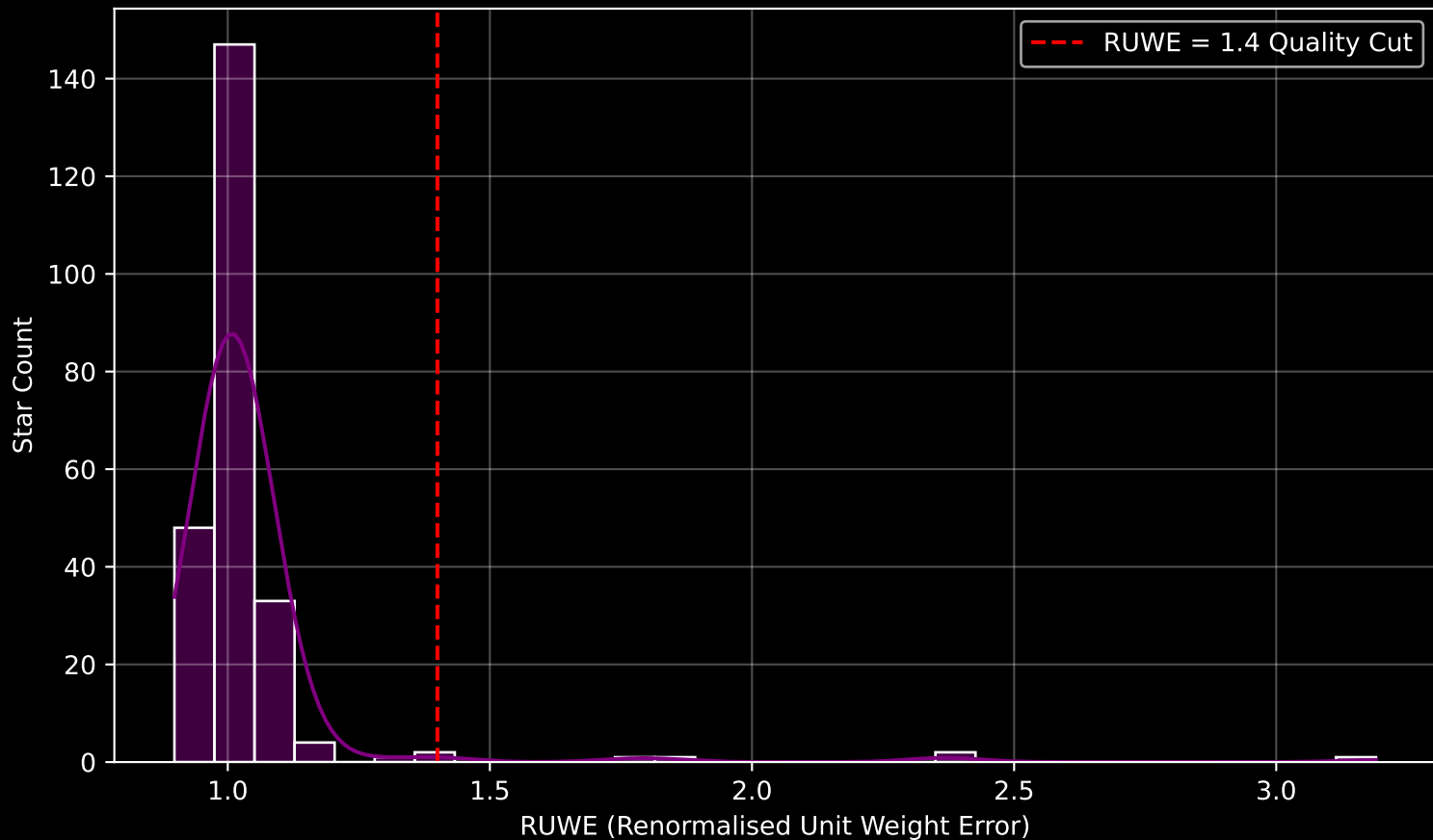
Gaia Cluster: [FSR_0852] RUWE Distribution (n= 240)
