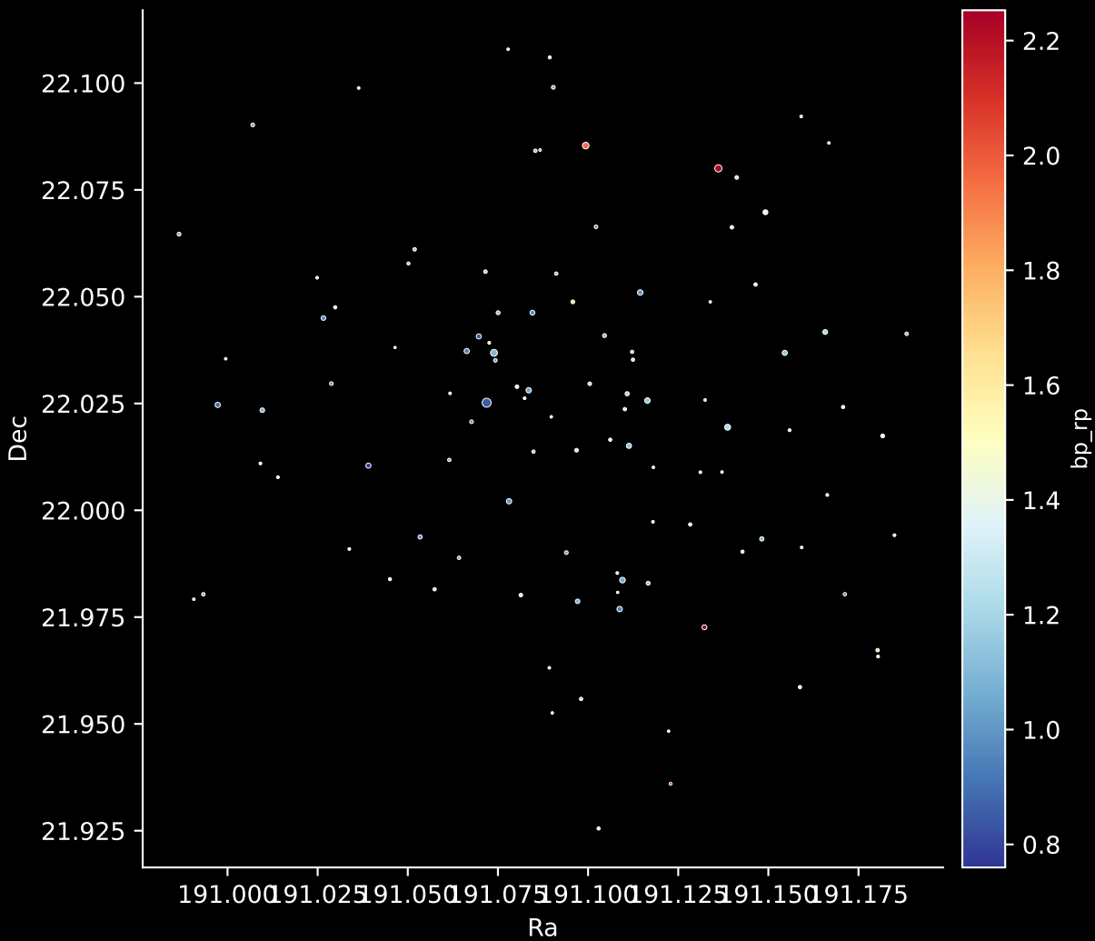
Gaia Cluster: [FSR_0883] Stars: 106
