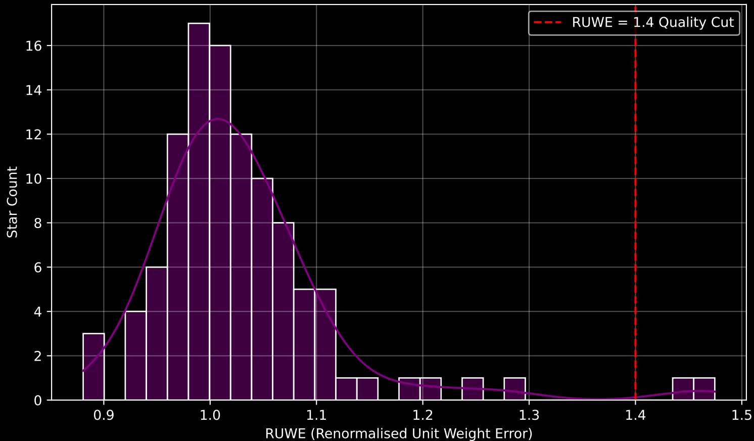
Gaia Cluster: [FSR_0883] RUWE Distribution (n= 106)
