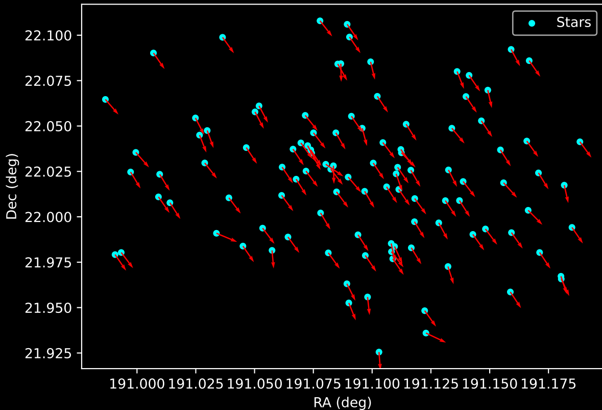
Gaia Cluster: [FSR_0883] Proper Motion Vectors for Gaia Star Field (n= 106)
