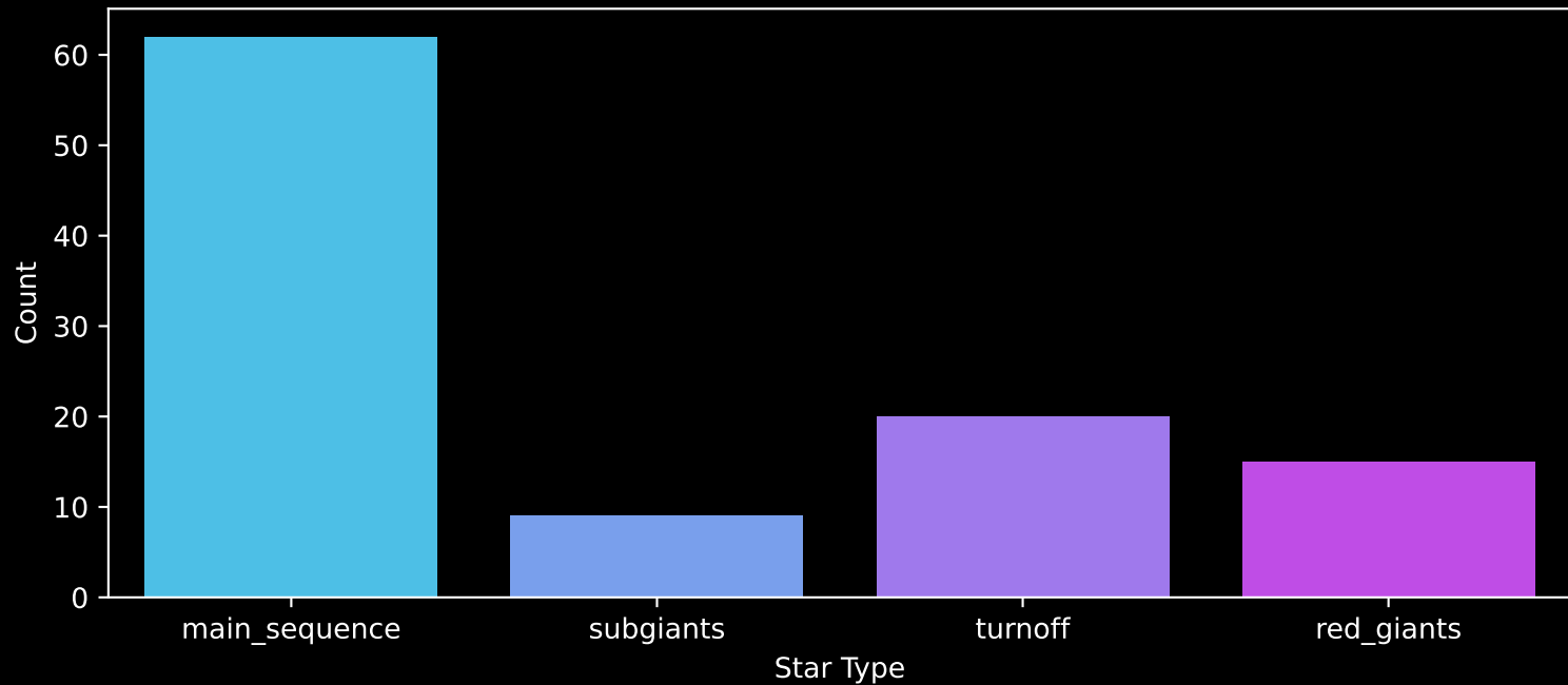
Gaia Cluster: [FSR_0883] Count plot of Star Type
