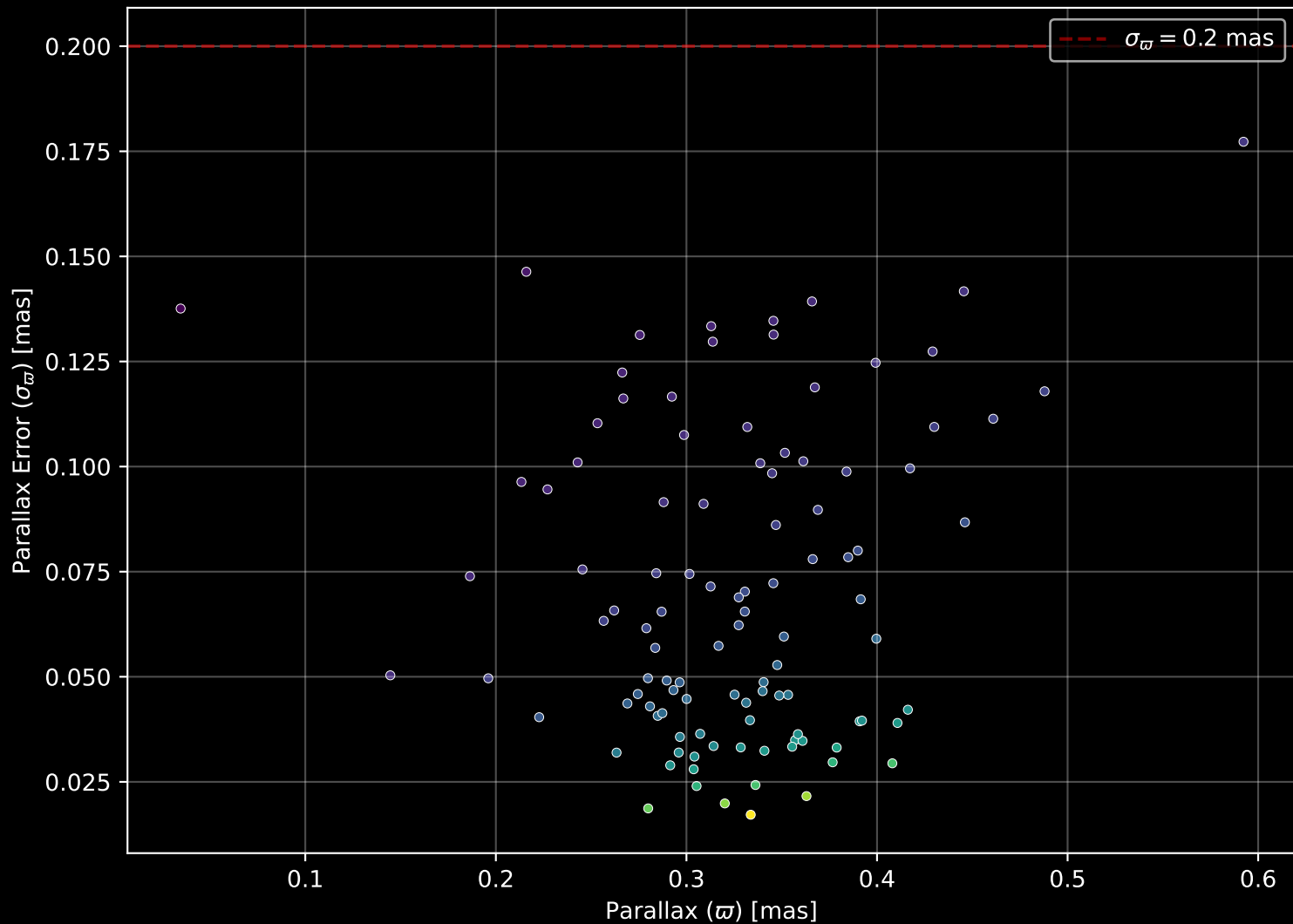
Gaia Cluster: [FSR_0883] Parallax Quality (n= 106)
