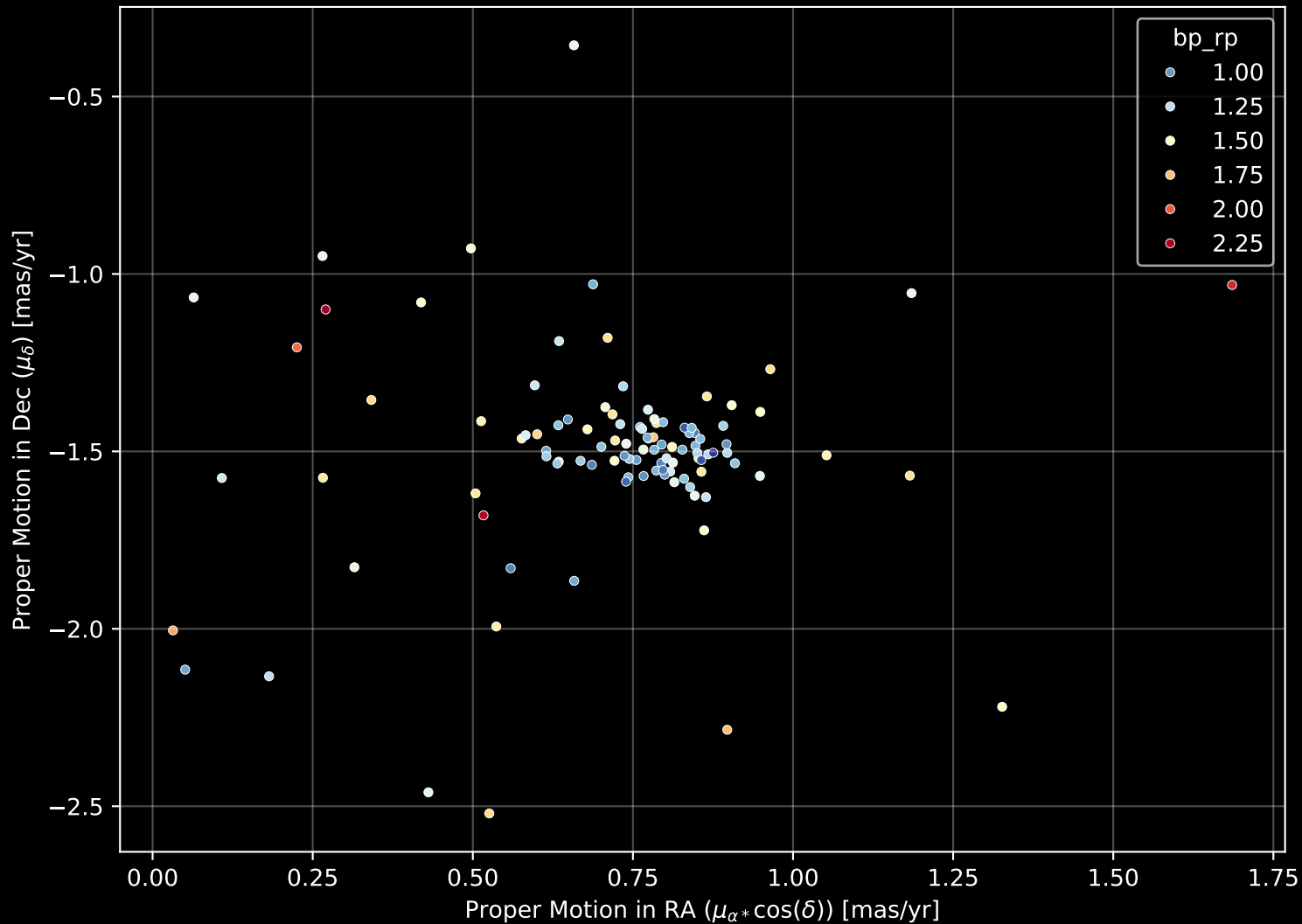
Gaia Cluster: [FSR_0883] Proper Motion Diagram (n= 106)
