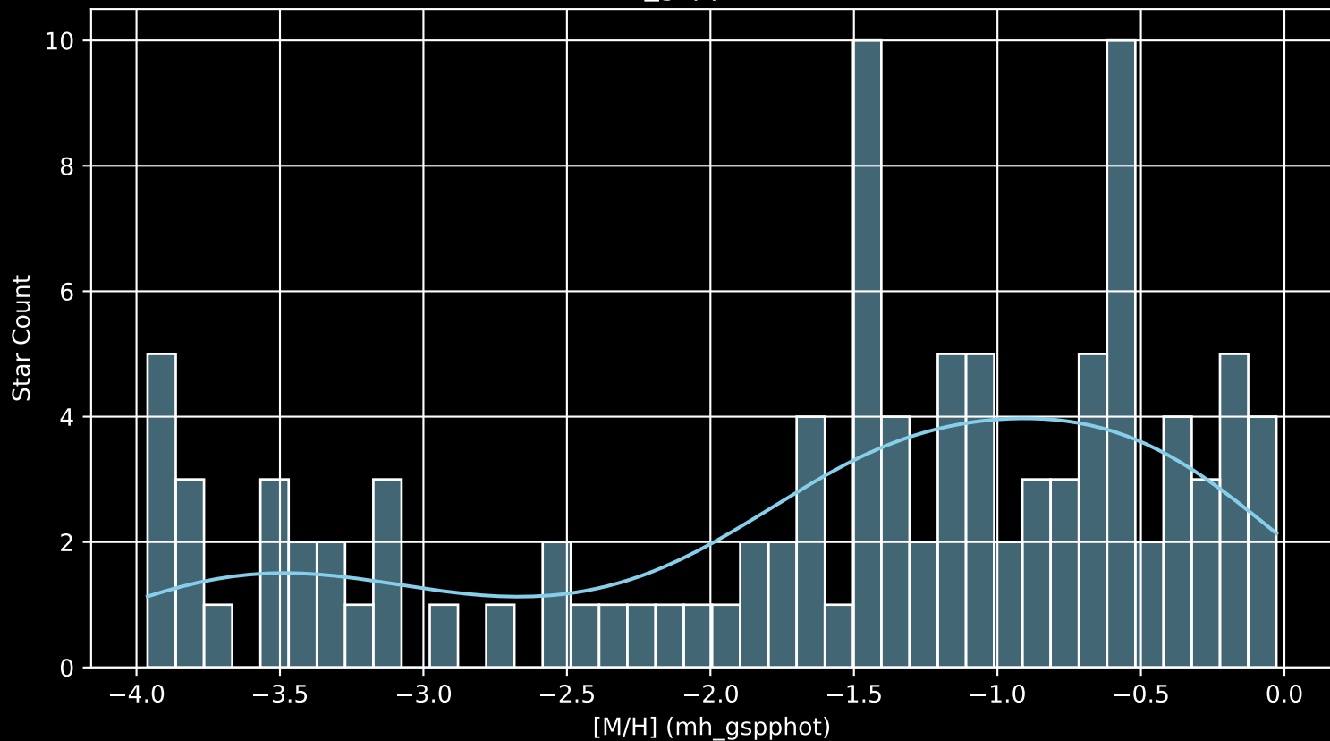
Gaia Cluster: [FSR_0883 [M/H] (mh_gspphot) (n= 106)
