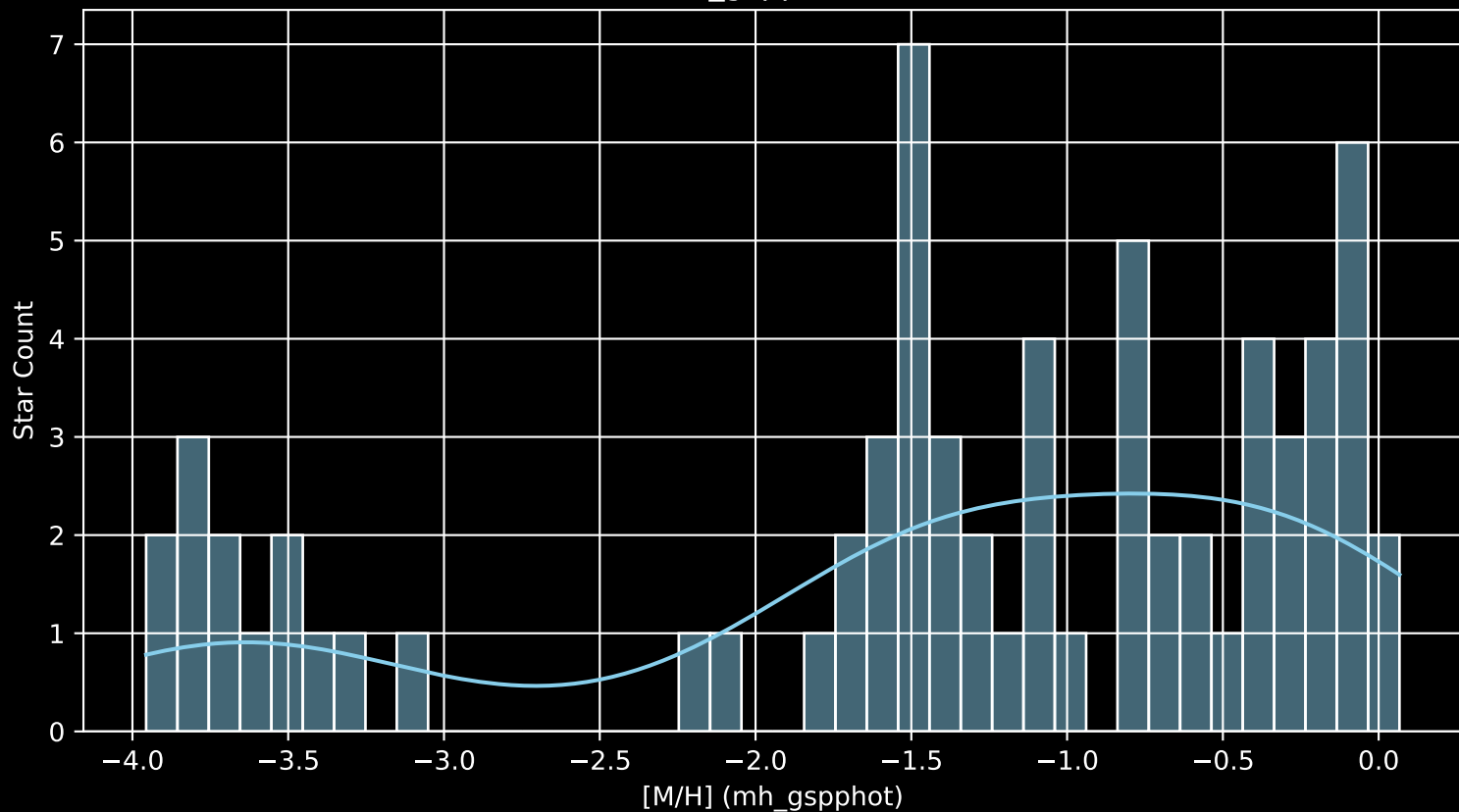
Gaia Cluster: [FSR_0921 [M/H] (mh_gspphot) (n= 68)
