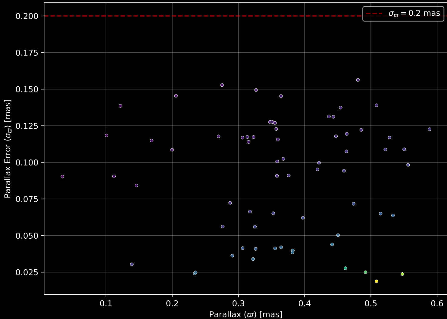
Gaia Cluster: [FSR_0921] Parallax Quality (n= 68)
