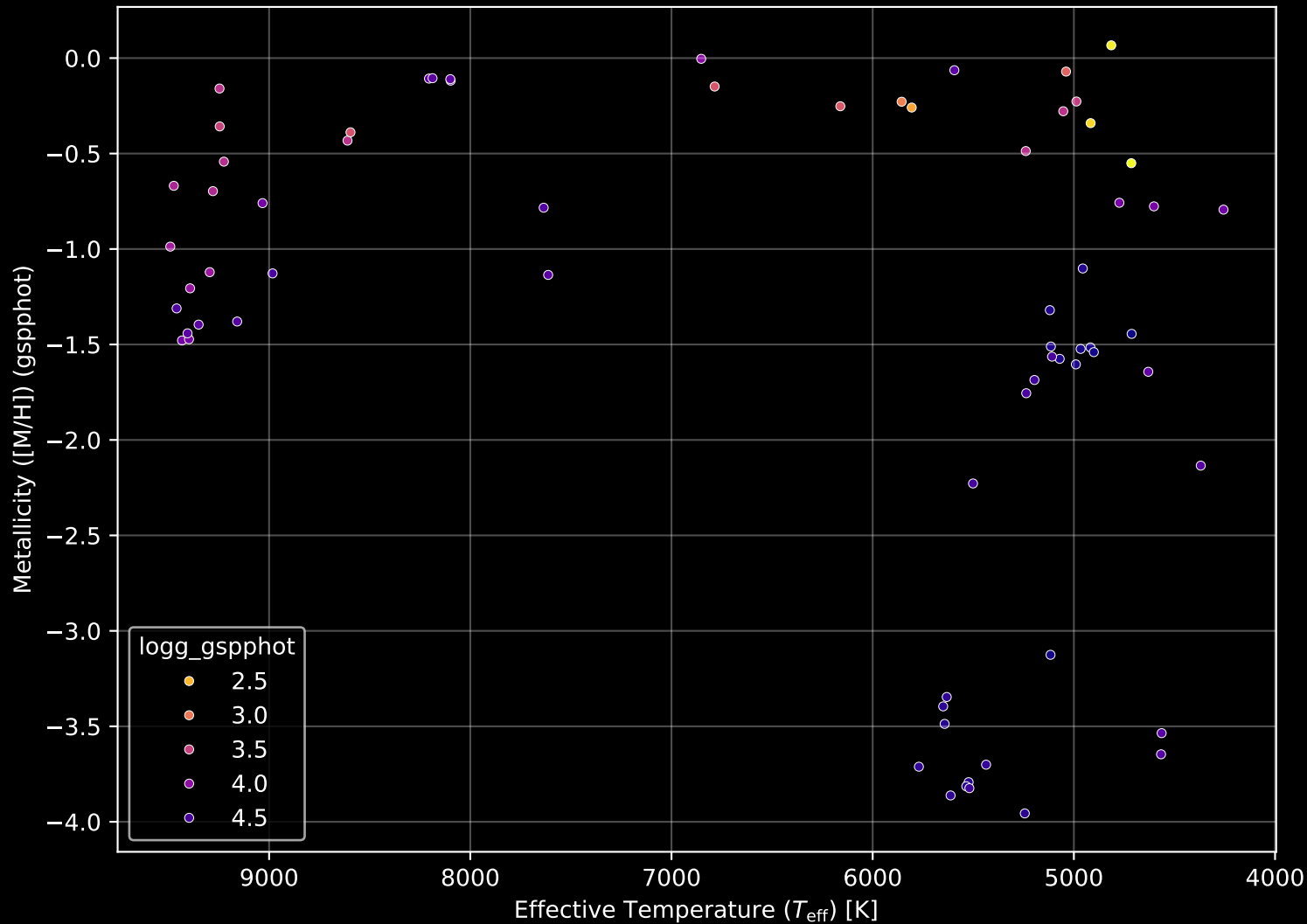
Gaia Cluster: [FSR_0921] Stellar Population Parameters (n= 68)
