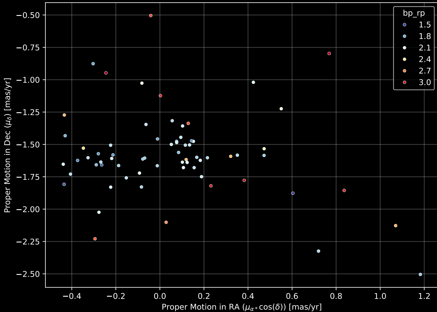
Gaia Cluster: [FSR_0921] Proper Motion Diagram (n= 68)
