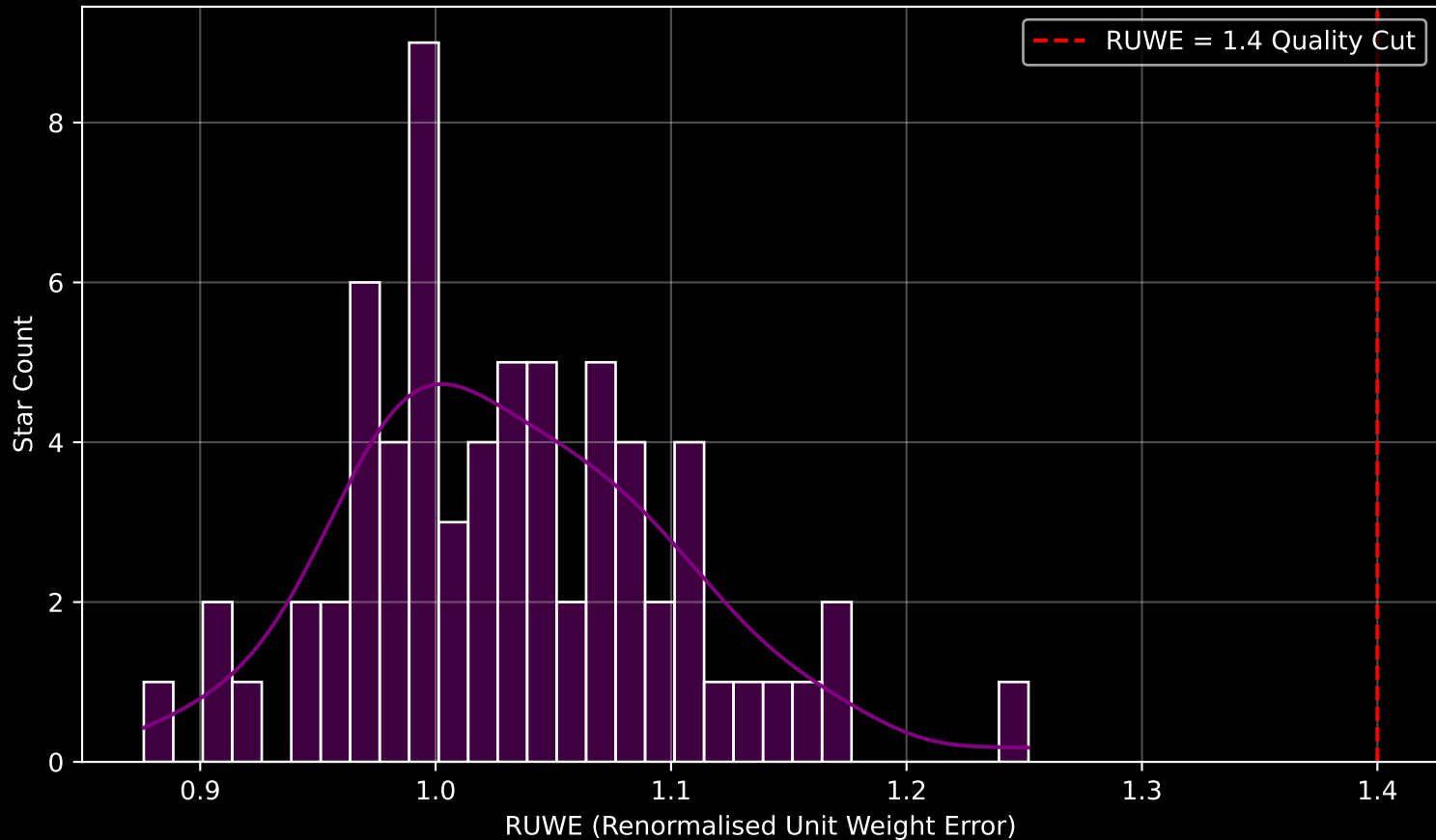
Gaia Cluster: [FSR_0921] RUWE Distribution (n= 68)
