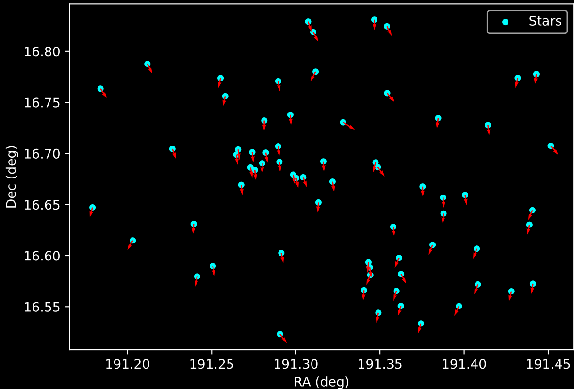
Gaia Cluster: [FSR_0921] Proper Motion Vectors for Gaia Star Field (n= 68)
