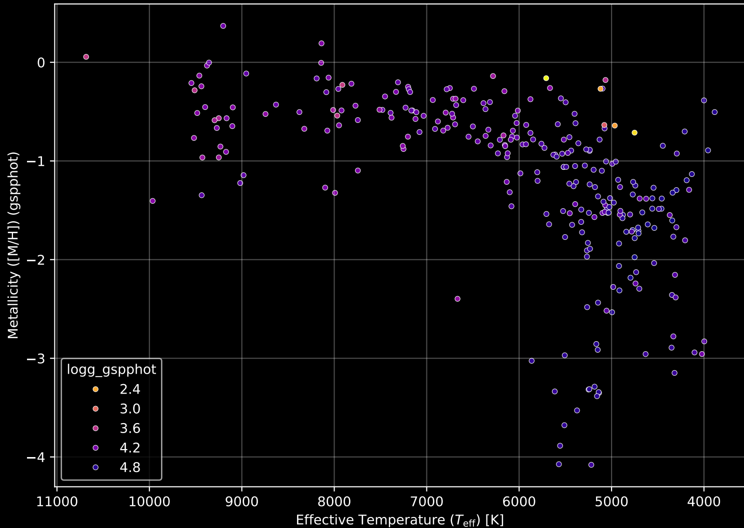
Gaia Cluster: [FSR_0951] Stellar Population Parameters (n= 277)
