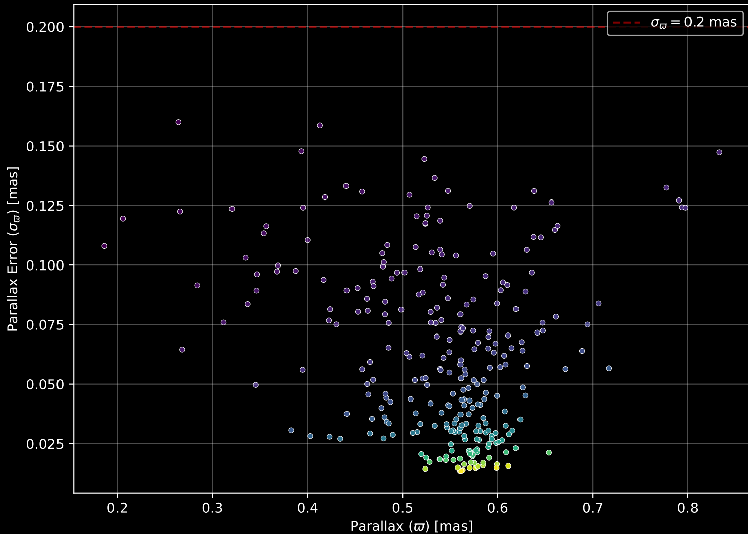
Gaia Cluster: [FSR_0951] Parallax Quality (n= 277)
