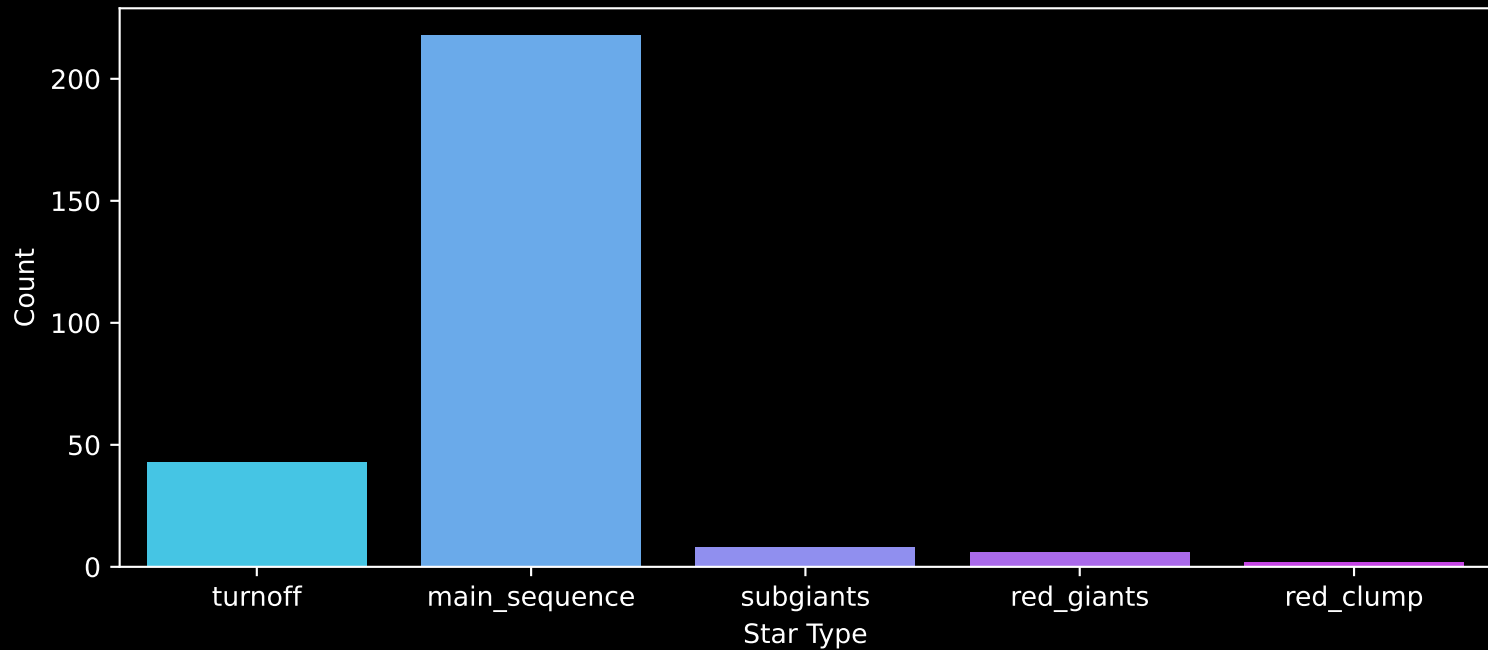
Gaia Cluster: [FSR_0951] Count plot of Star Type
