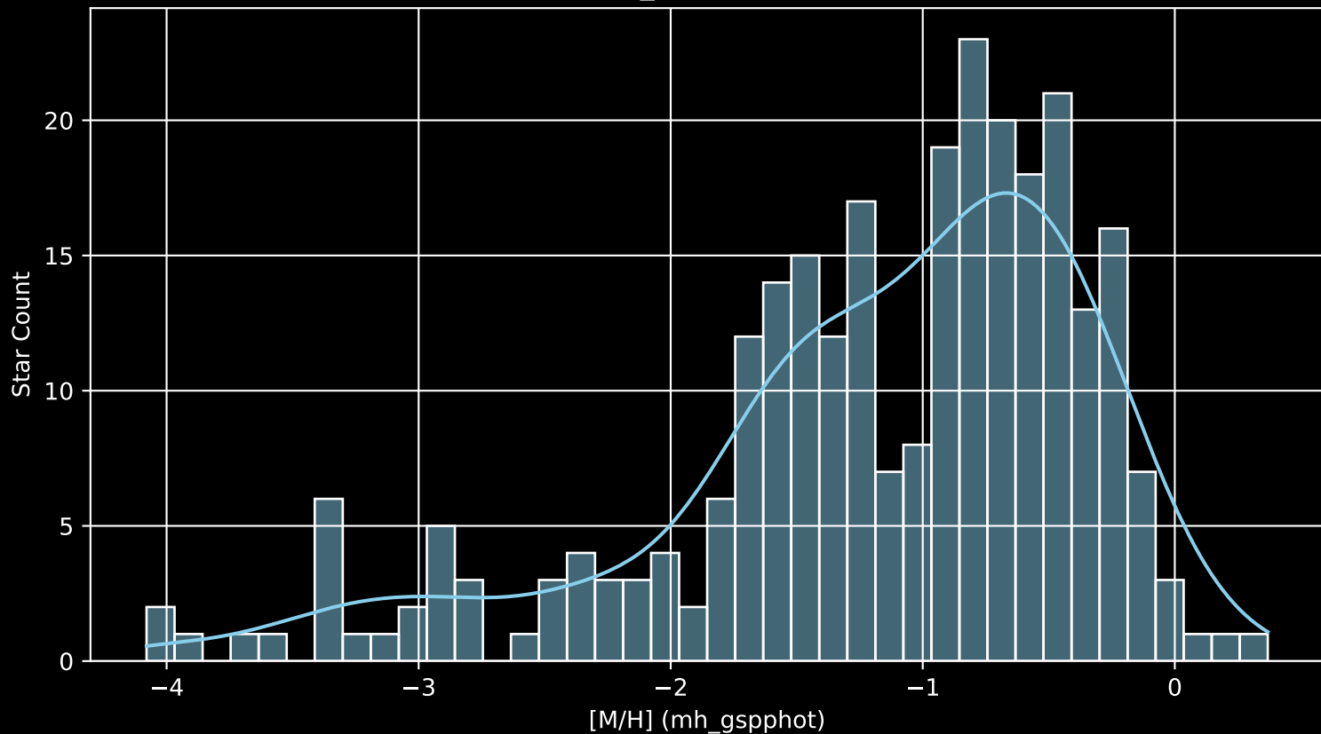
Gaia Cluster: [FSR_0951 [M/H] (mh_gspphot) (n= 277)
