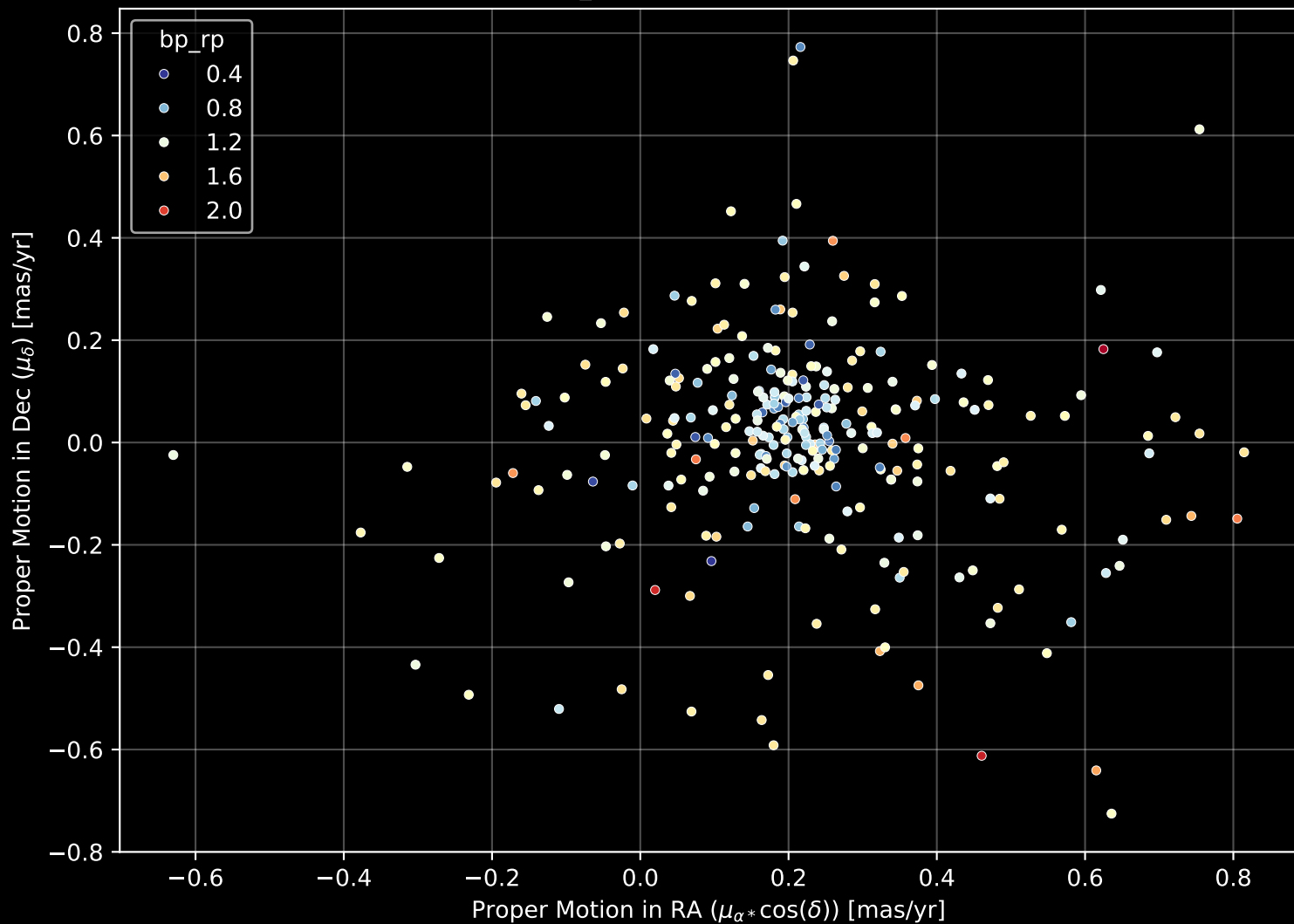
Gaia Cluster: [FSR_0951] Proper Motion Diagram (n= 277)
