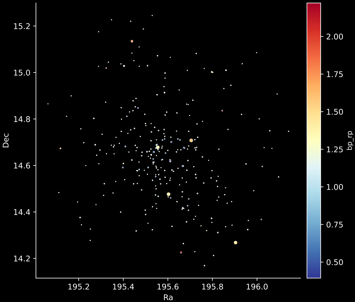
Gaia Cluster: [FSR_0951] Stars: 277
