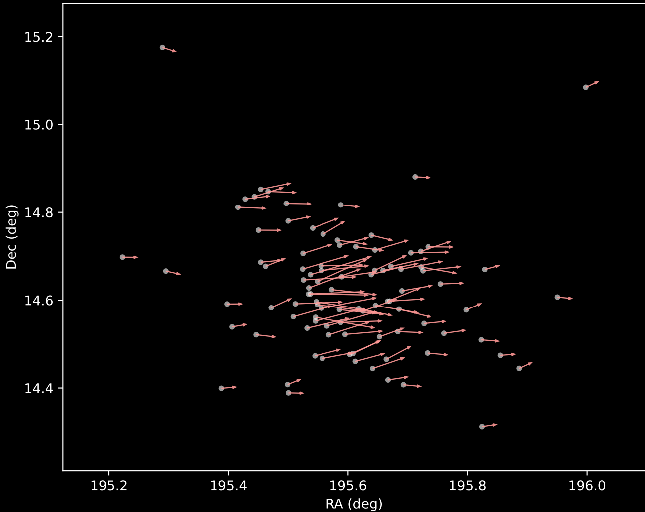
Gaia DR3 Cluster 7 Proper Motion Vectors (n=94)
