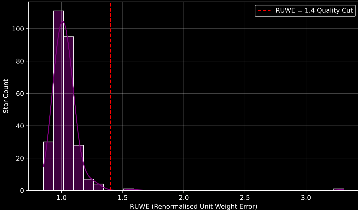
Gaia Cluster: [FSR_0951] RUWE Distribution (n= 277)
