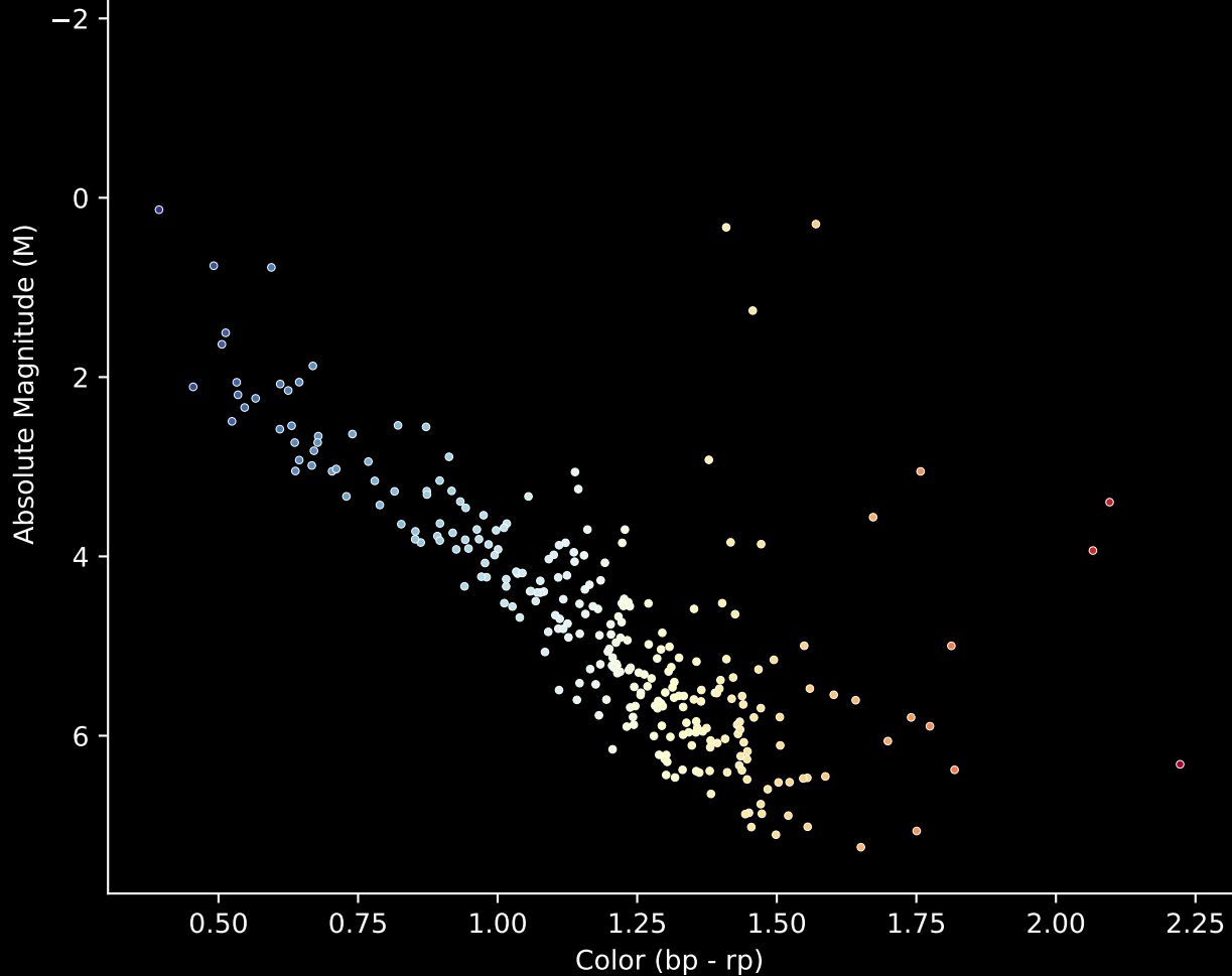
Gaia Cluster: [FSR_0951] Stars (n= 277) Hertzsprung-Russel Diagram
