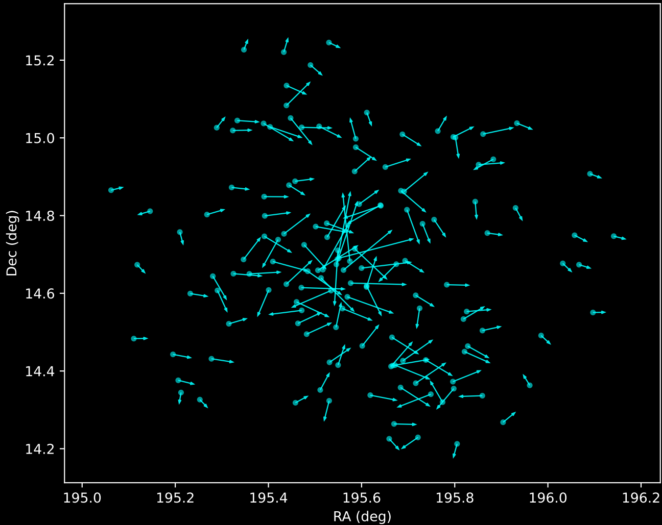
Gaia DR3 Noise Stream Proper Motion Vectors (n=138)
