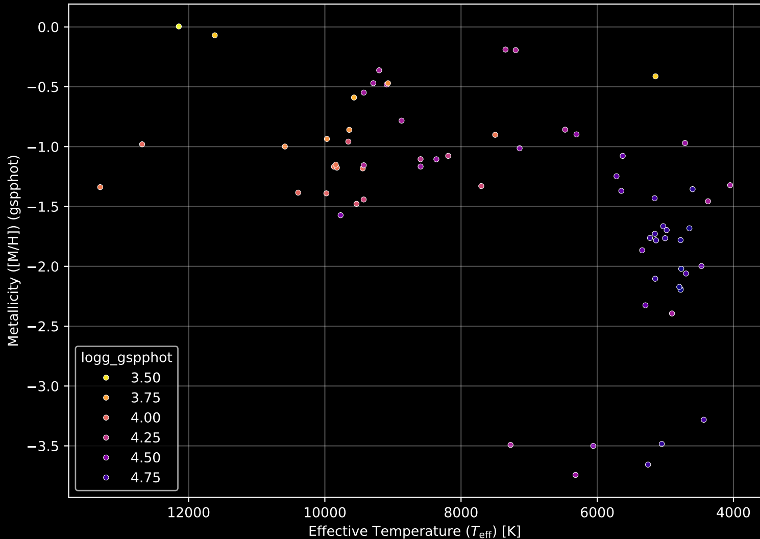
Gaia Cluster: [FSR_0968] Stellar Population Parameters (n= 69)
