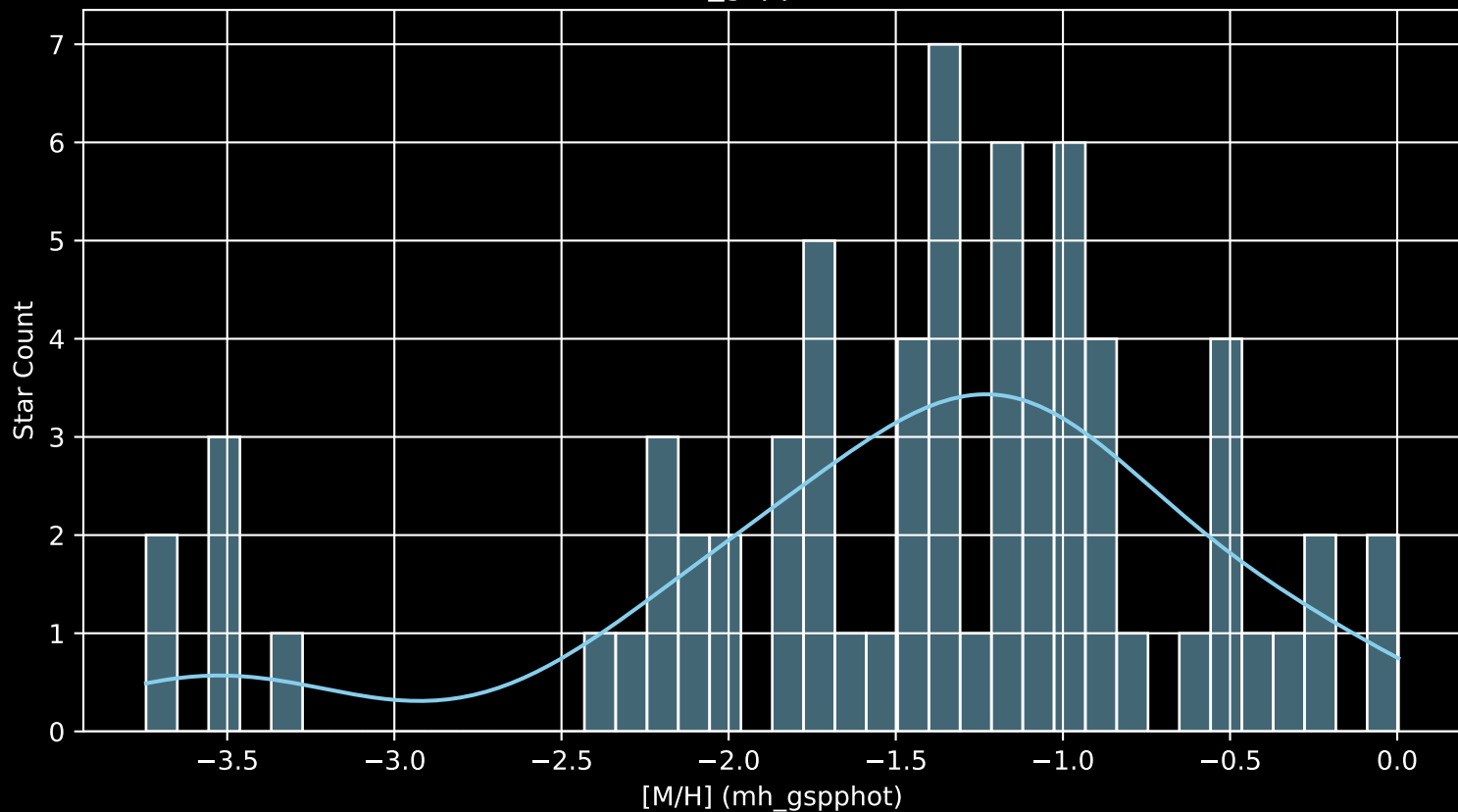
Gaia Cluster: [FSR_0968 [M/H] (mh_gspphot) (n= 69)
