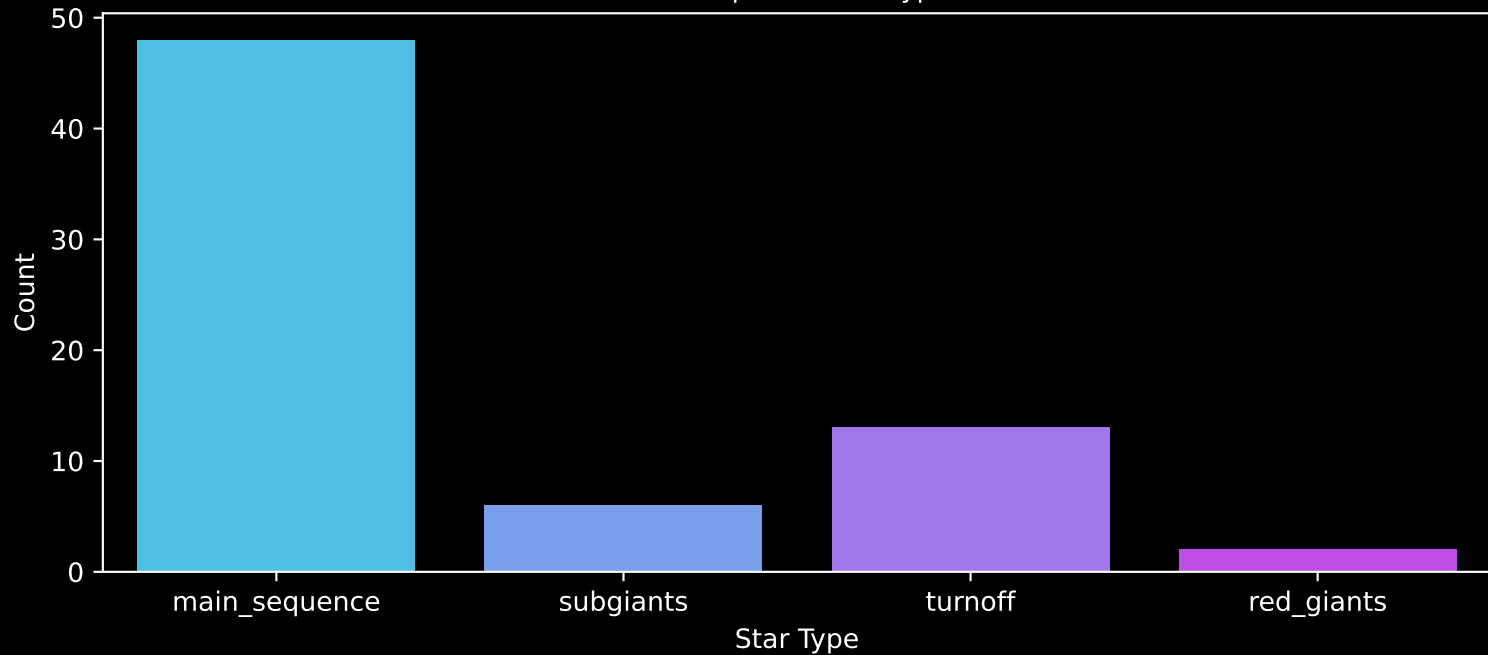
Gaia Cluster: [FSR_0968] Count plot of Star Type
