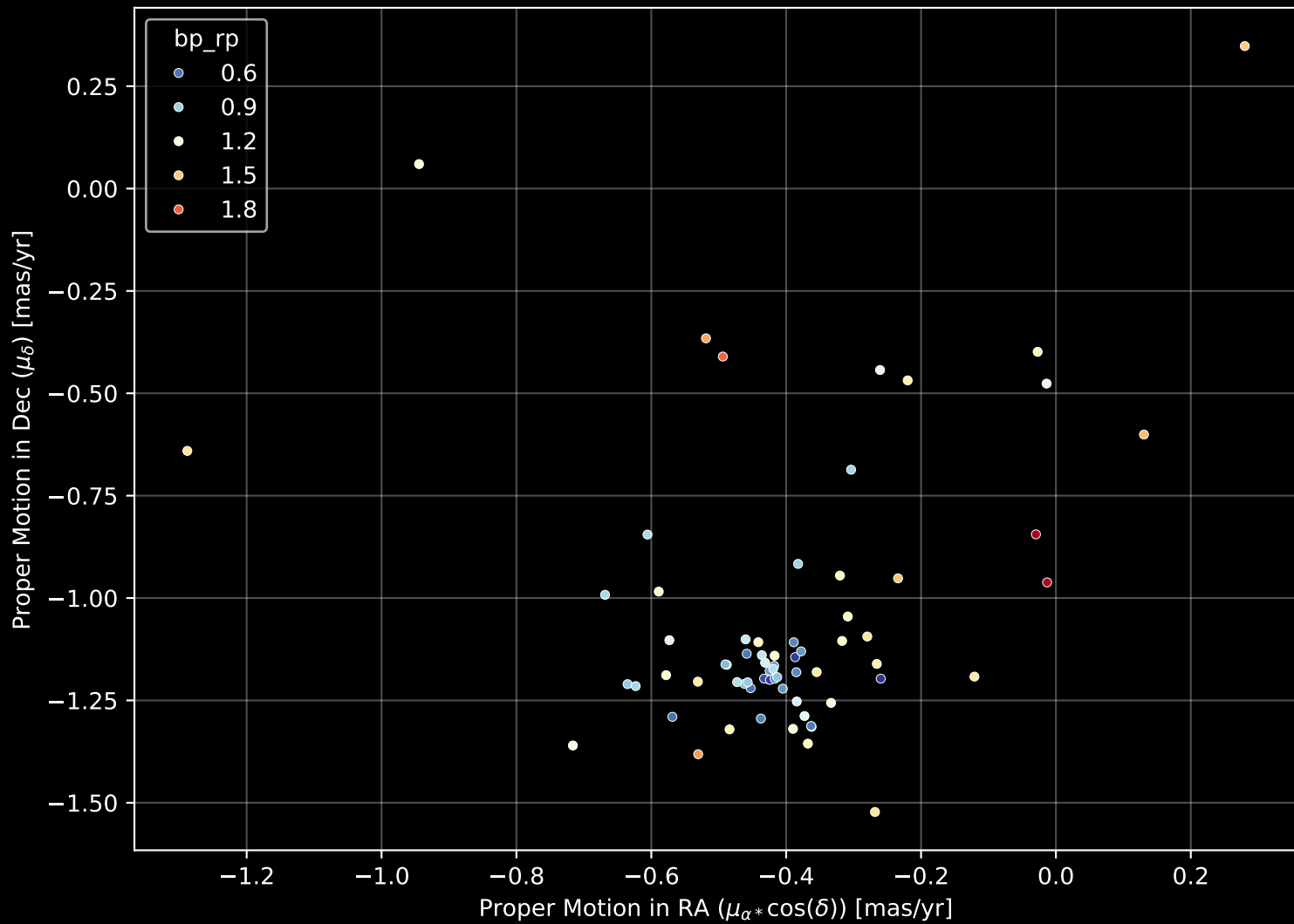
Gaia Cluster: [FSR_0968] Proper Motion Diagram (n= 69)
