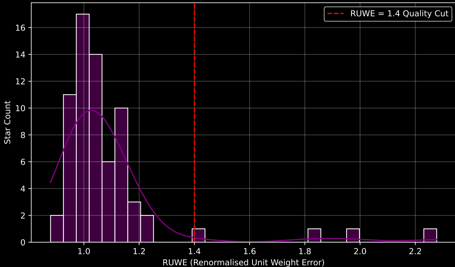
Gaia Cluster: [FSR_0968] RUWE Distribution (n= 69)
