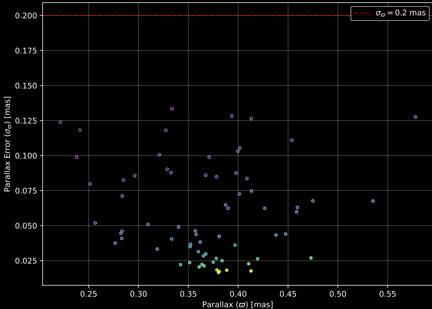
Gaia Cluster: [FSR_0968] Parallax Quality (n= 69)
