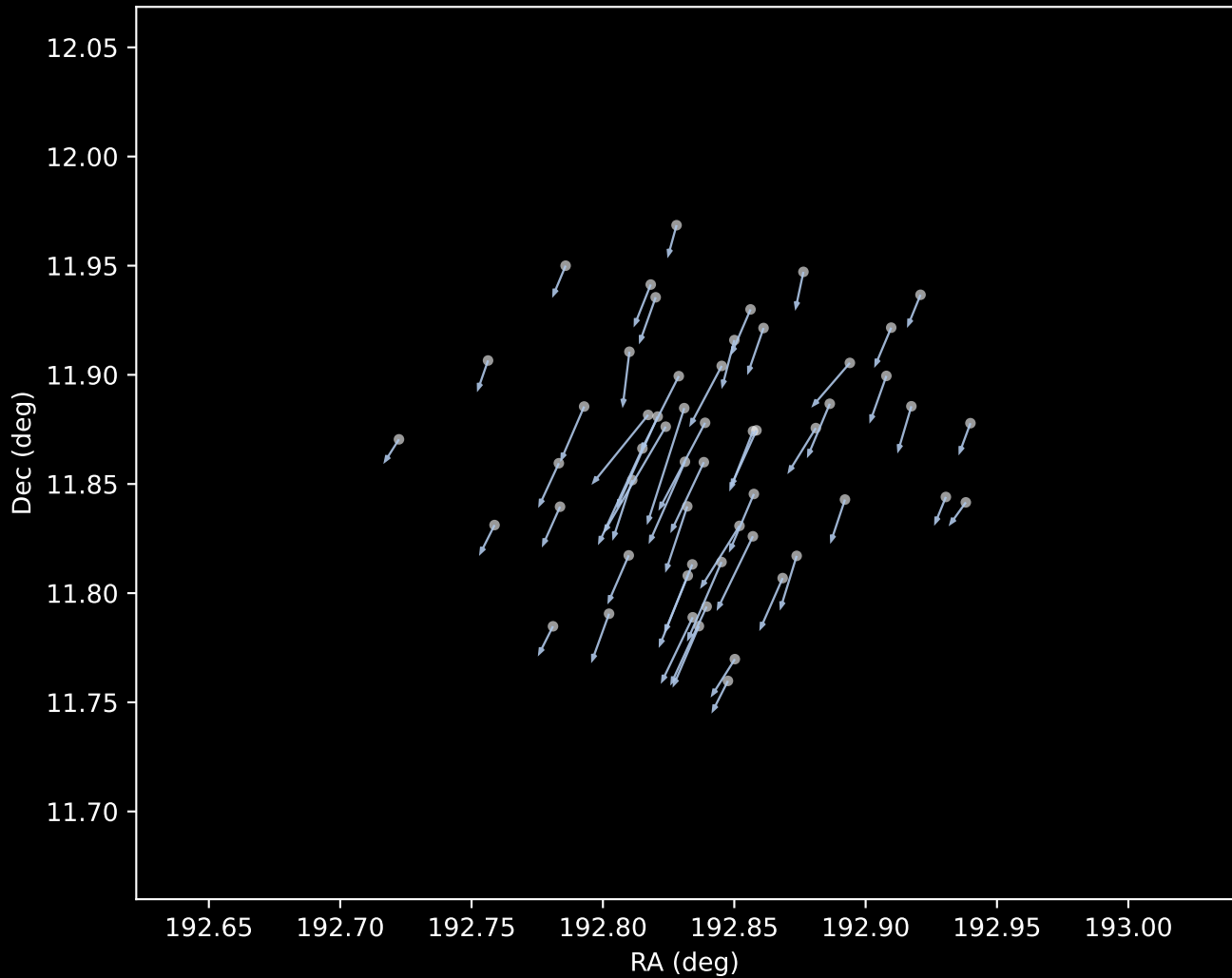
Gaia DR3 Cluster 1 Proper Motion Vectors (n=56)
