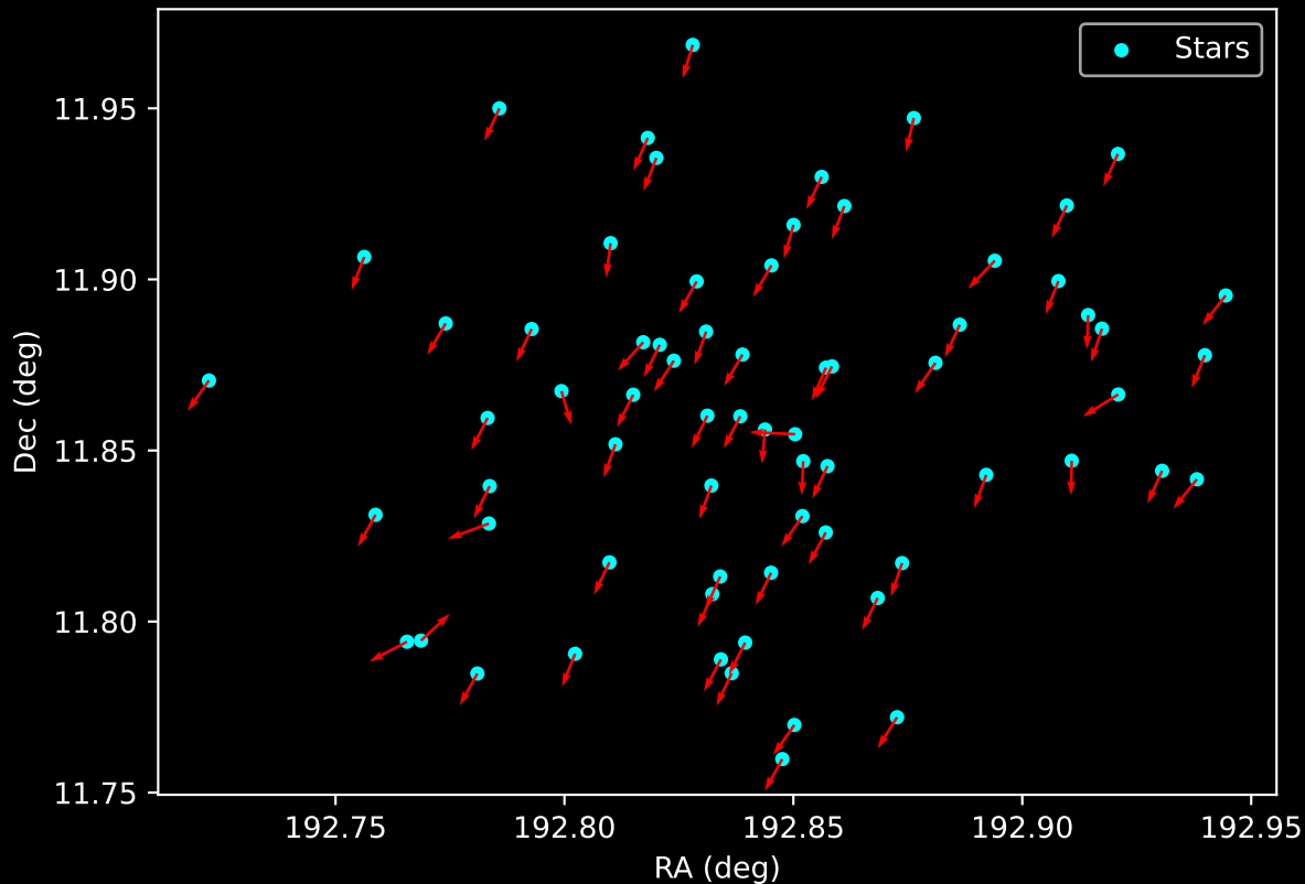
Gaia Cluster: [FSR_0968] Proper Motion Vectors for Gaia Star Field (n= 69)
