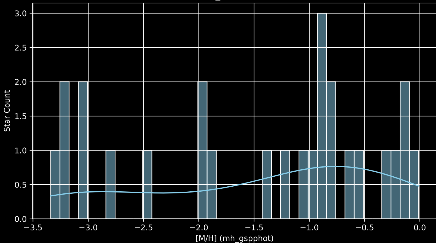
Gaia Cluster: [FSR_1025 [M/H] (mh_gspphot) (n= 26)
