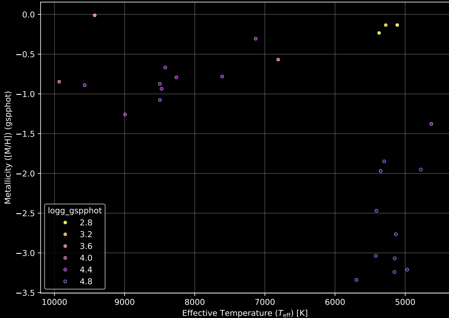
Gaia Cluster: [FSR_1025] Stellar Population Parameters (n= 26)
