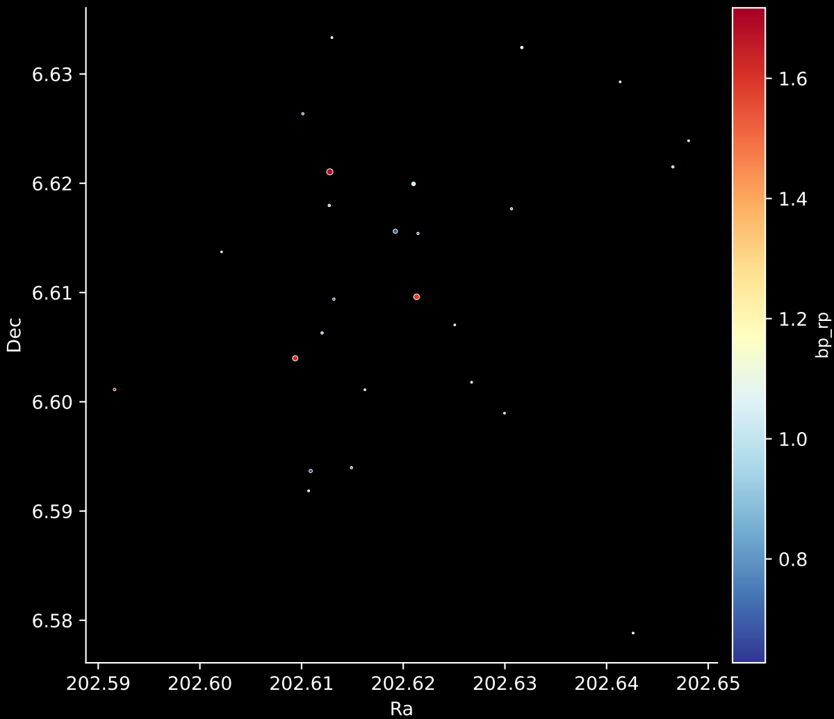
Gaia Cluster: [FSR_1025] Stars: 26
