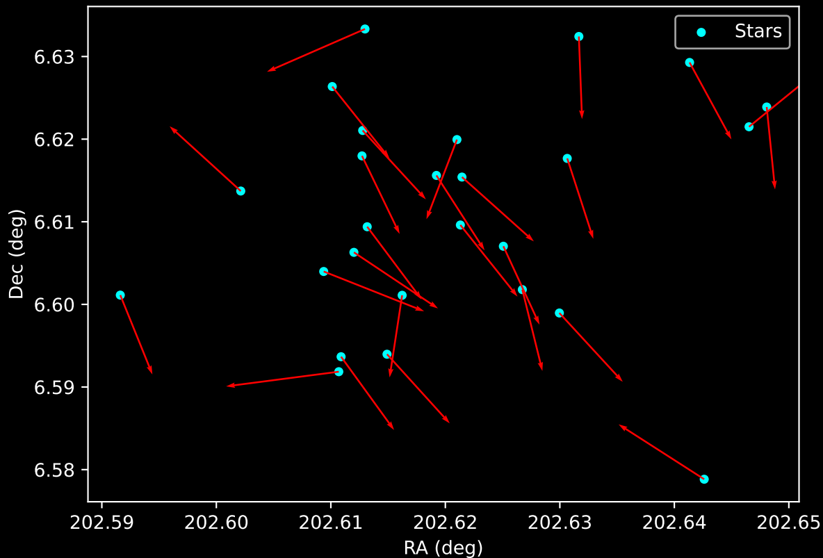
Gaia Cluster: [FSR_1025] Proper Motion Vectors for Gaia Star Field (n= 26)
