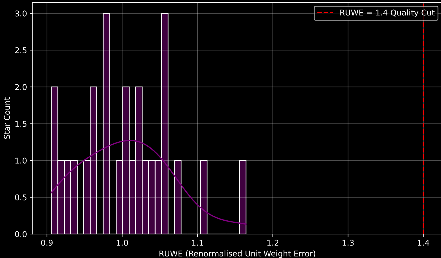
Gaia Cluster: [FSR_1025] RUWE Distribution (n= 26)
