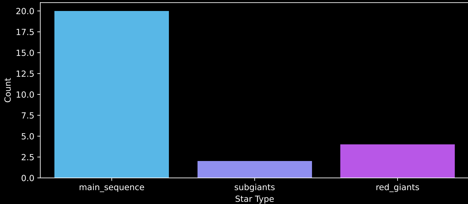
Gaia Cluster: [FSR_1025] Count plot of Star Type
