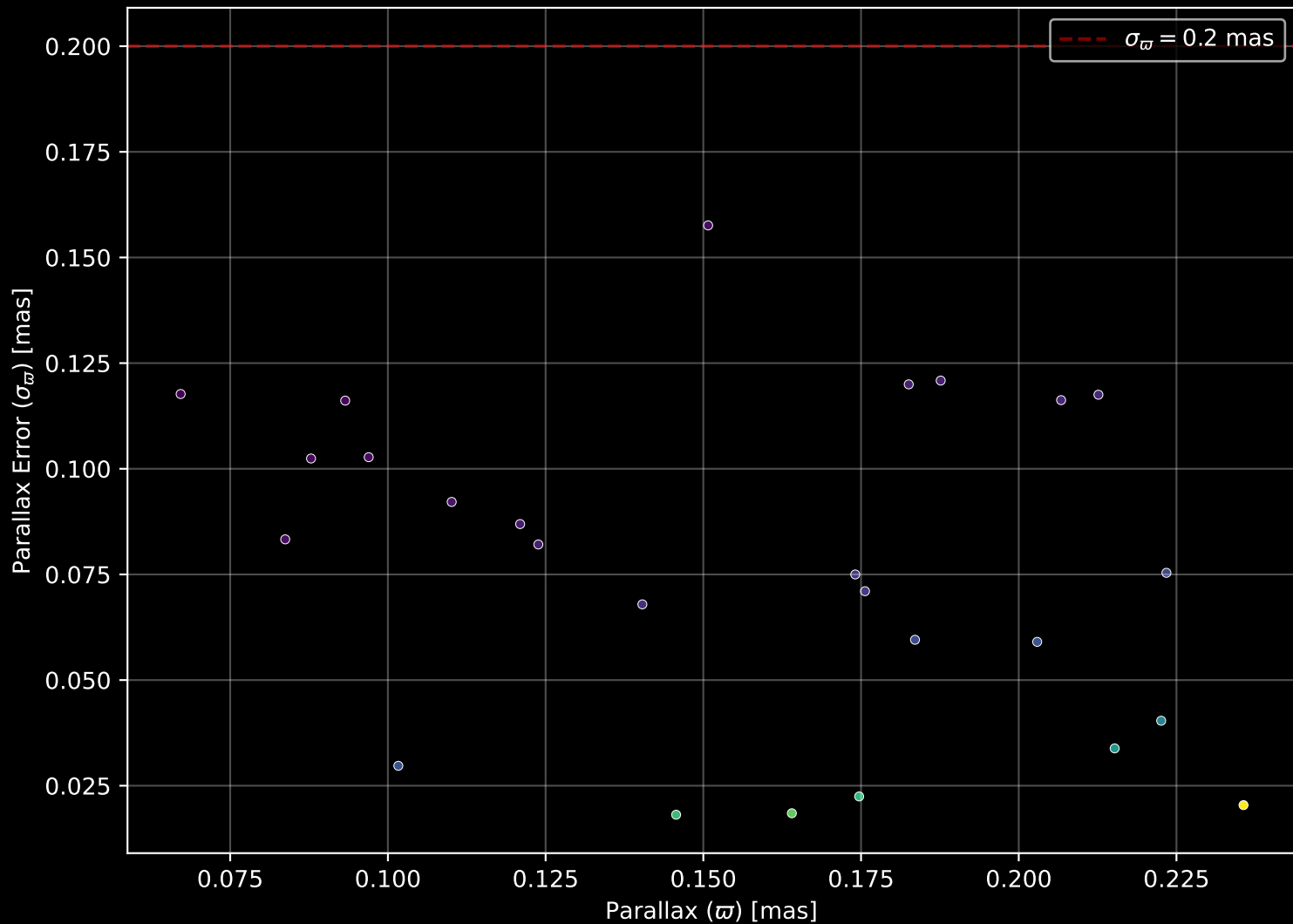
Gaia Cluster: [FSR_1025] Parallax Quality (n= 26)
