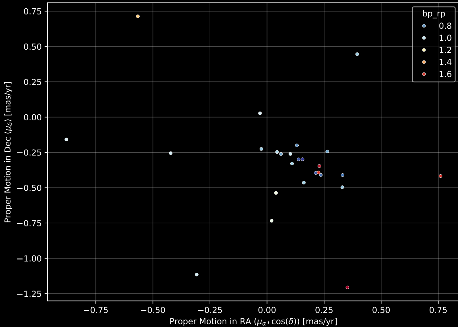
Gaia Cluster: [FSR_1025] Proper Motion Diagram (n= 26)
