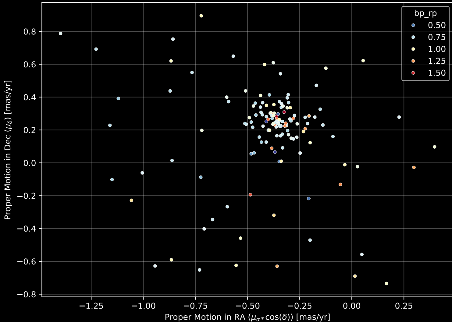
Gaia Cluster: [FSR_1083] Proper Motion Diagram (n= 141)
