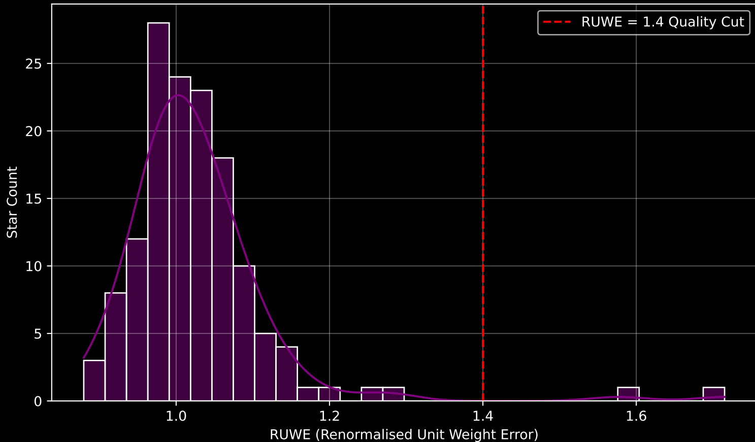
Gaia Cluster: [FSR_1083] RUWE Distribution (n= 141)
