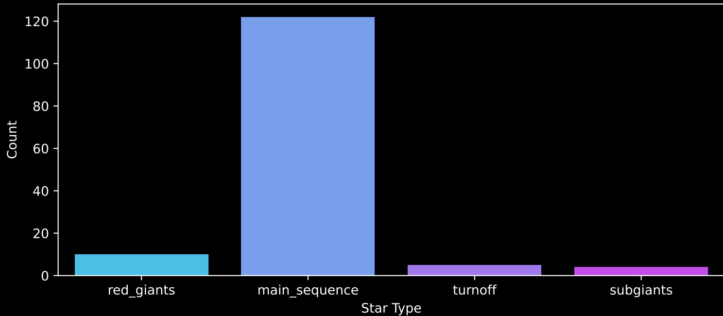
Gaia Cluster: [FSR_1083] Count plot of Star Type
