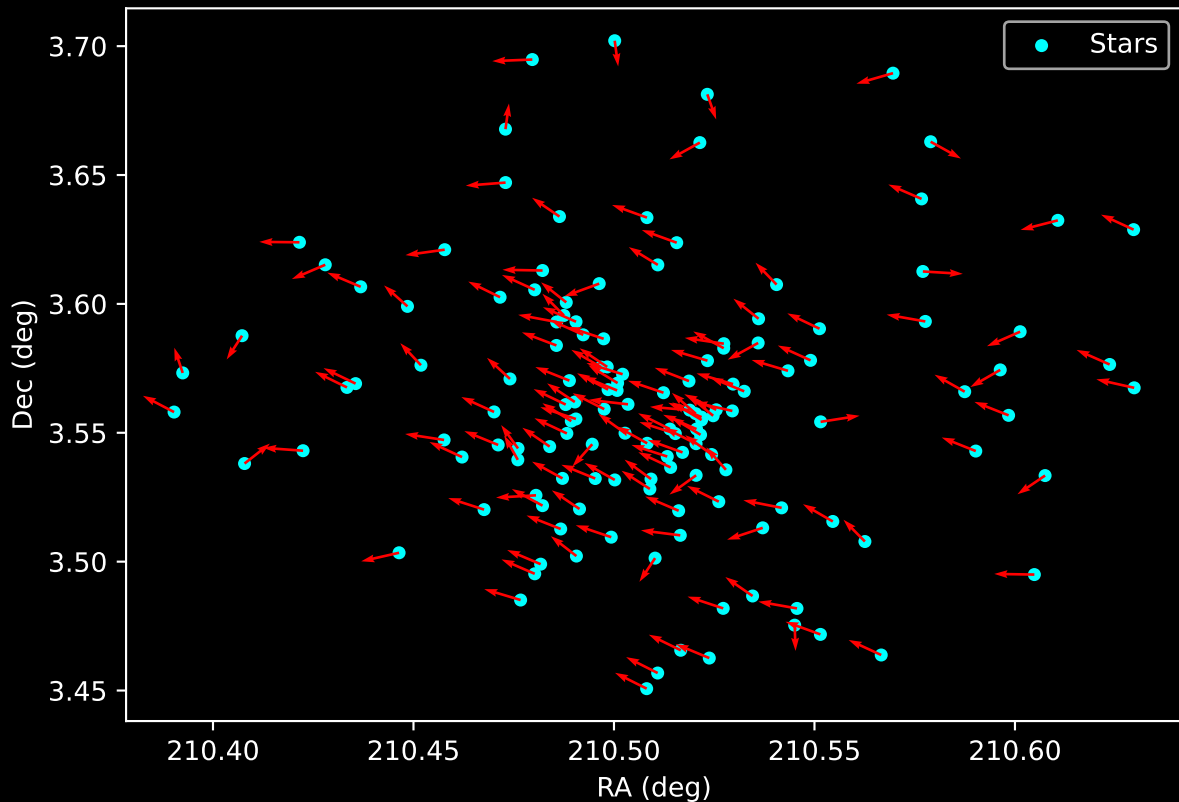
Gaia Cluster: [FSR_1083] Proper Motion Vectors for Gaia Star Field (n= 141)
