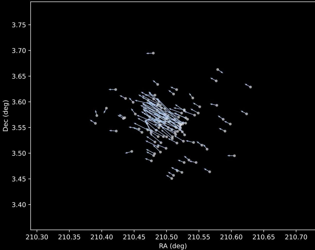
Gaia DR3 Cluster 1 Proper Motion Vectors (n=112)
