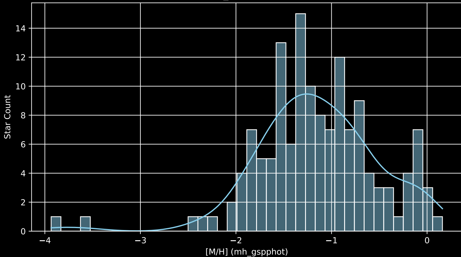
Gaia Cluster: [FSR_1083 [M/H] (mh_gspphot) (n= 141)
