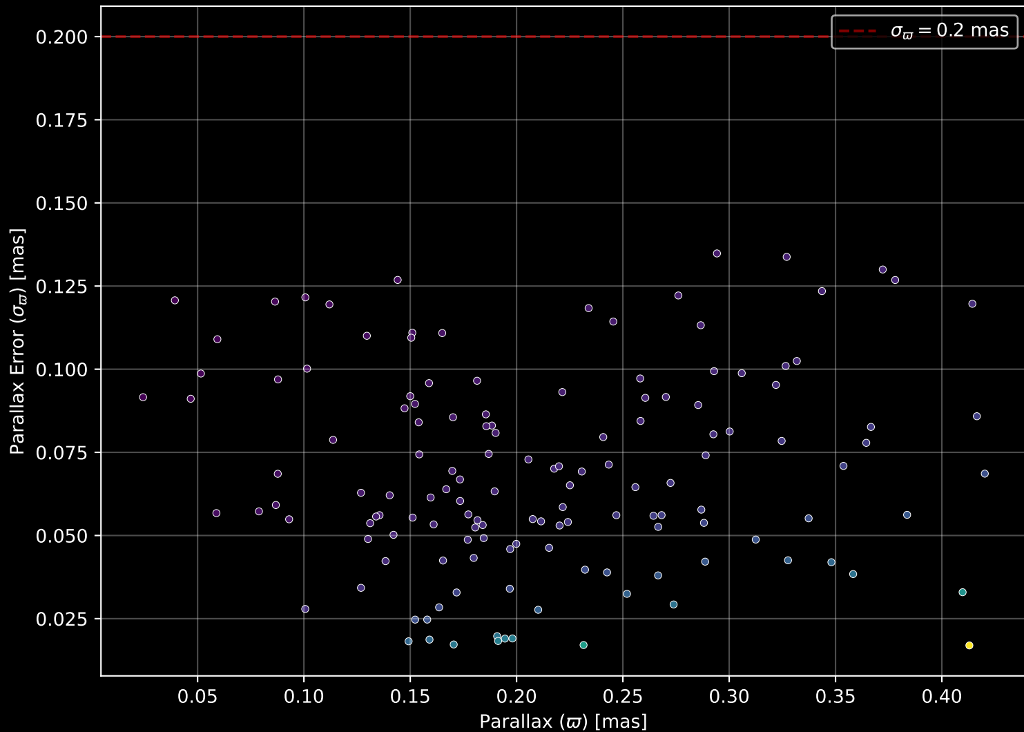
Gaia Cluster: [FSR_1083] Parallax Quality (n= 141)
