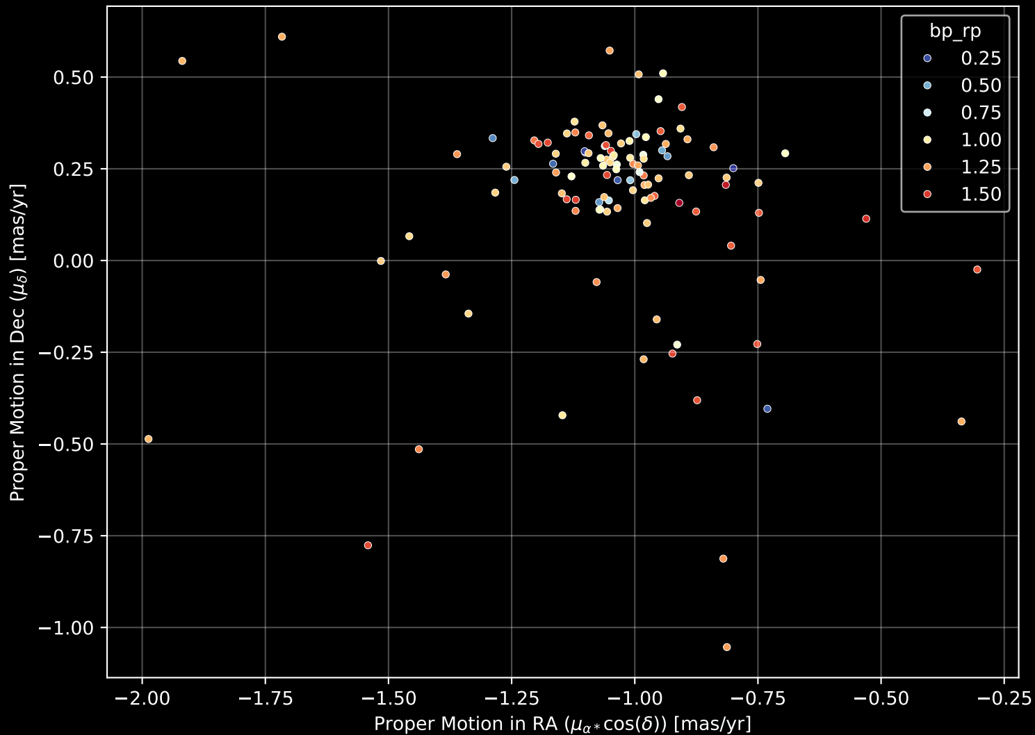
Gaia Cluster: [FSR_1085] Proper Motion Diagram (n= 112)
