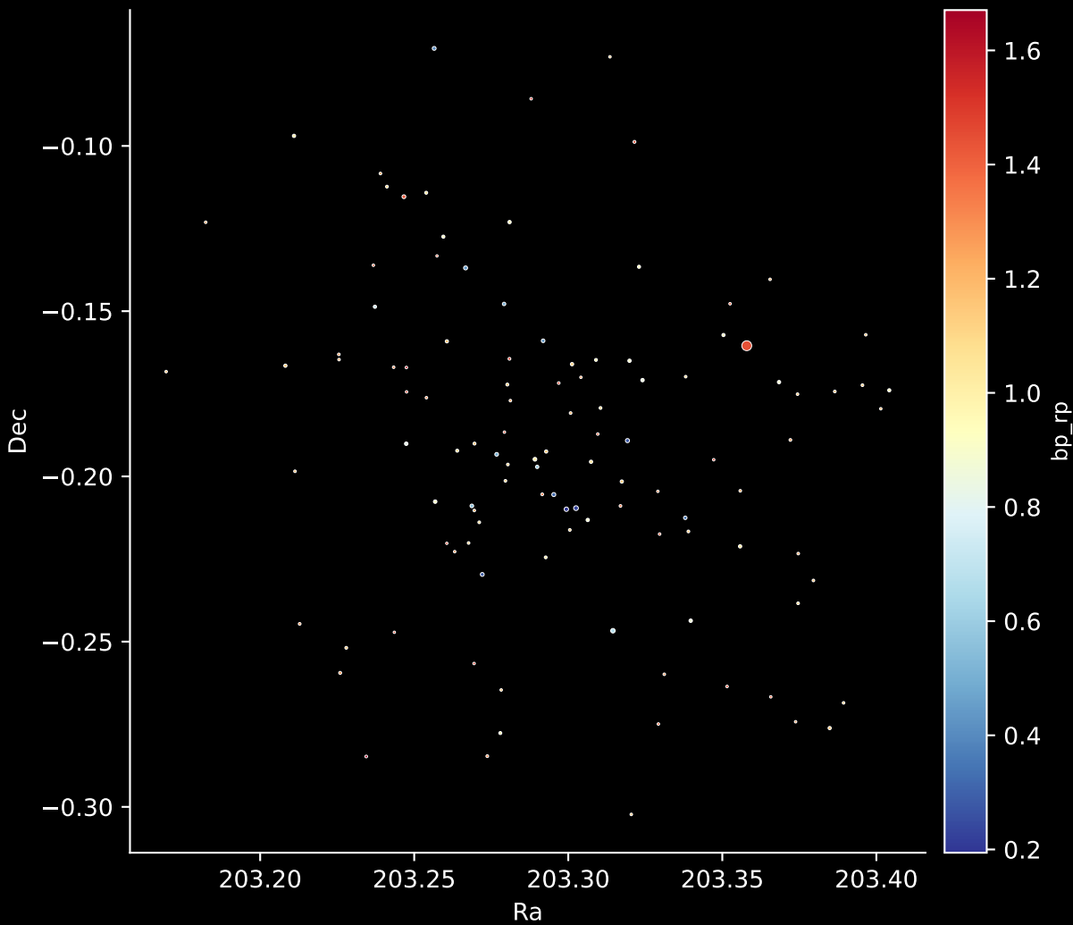
Gaia Cluster: [FSR_1085] Stars: 112
