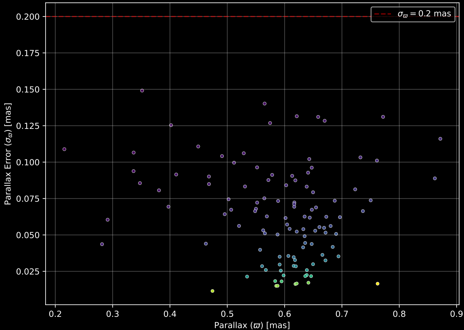
Gaia Cluster: [FSR_1085] Parallax Quality (n= 112)
