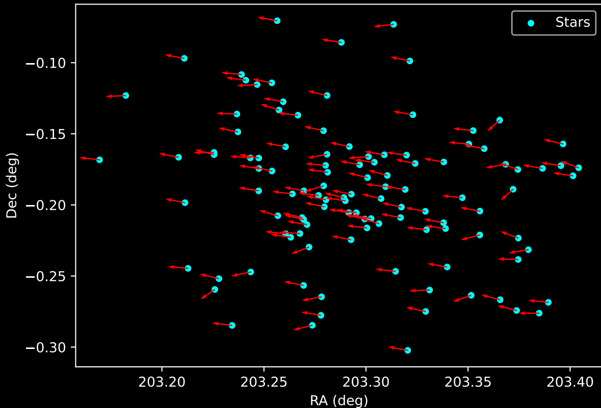
Gaia Cluster: [FSR_1085] Proper Motion Vectors for Gaia Star Field (n= 112)
