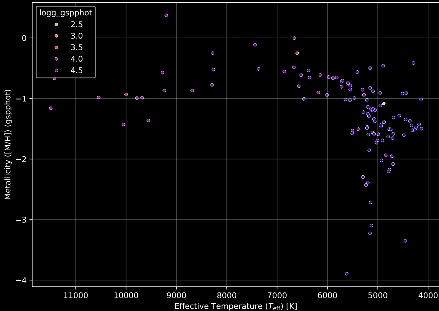
Gaia Cluster: [FSR_1085] Stellar Population Parameters (n= 112)
