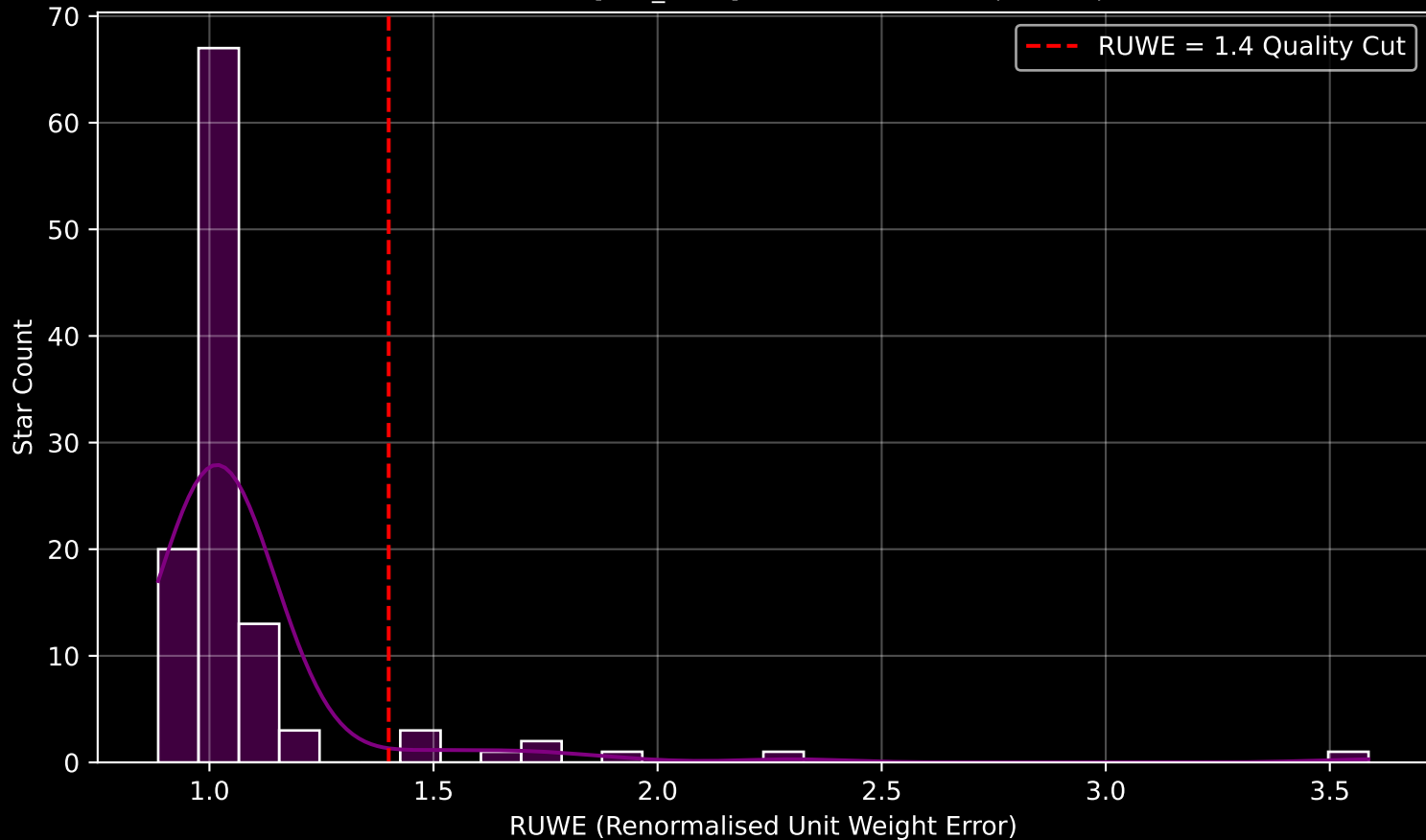
Gaia Cluster: [FSR_1085] RUWE Distribution (n= 112)
