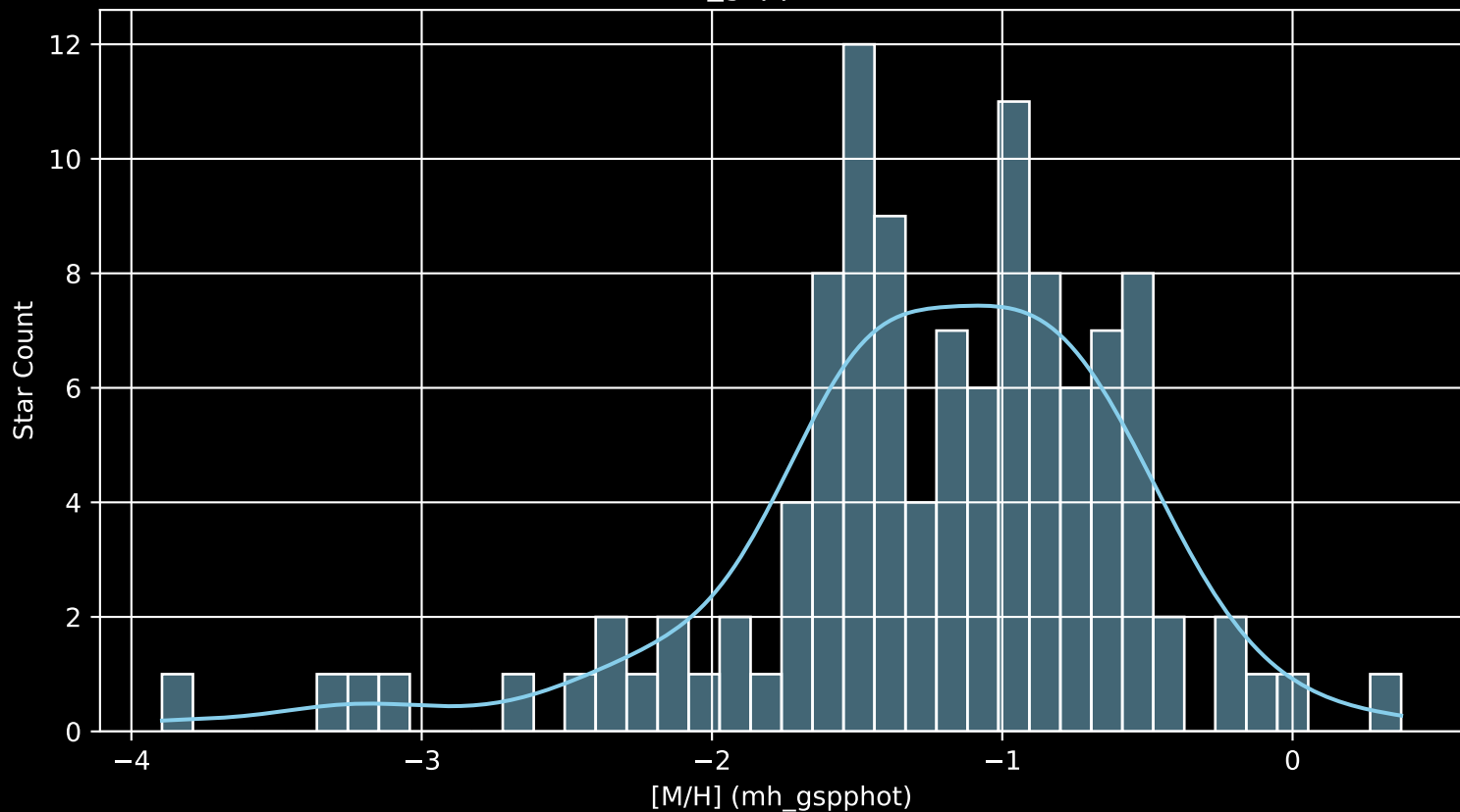
Gaia Cluster: [FSR_1085 [M/H] (mh_gspphot) (n= 112)
