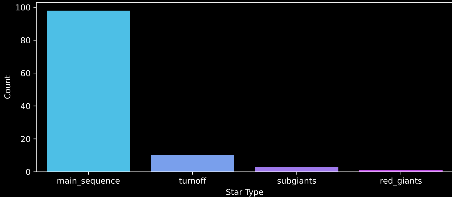
Gaia Cluster: [FSR_1085] Count plot of Star Type
