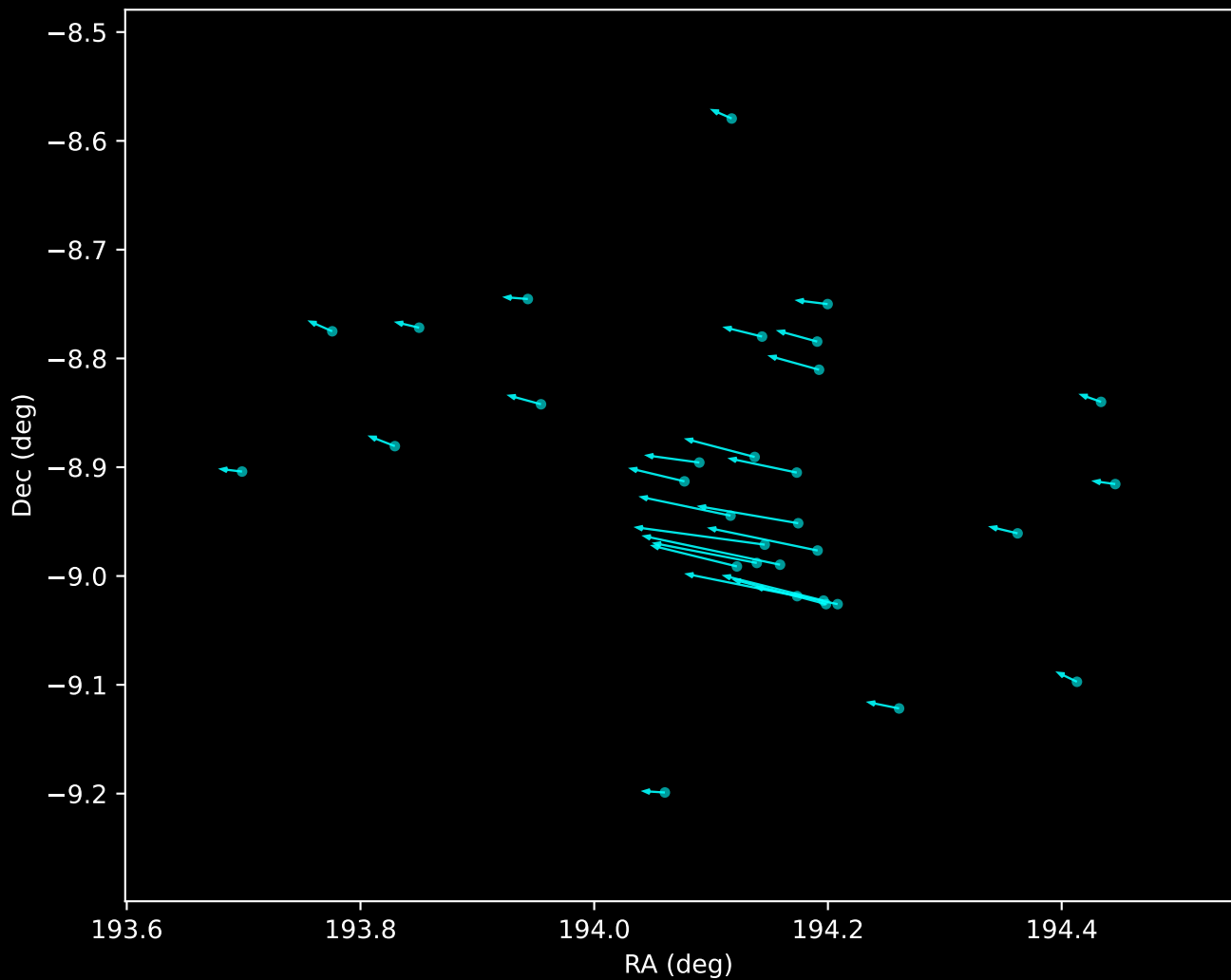
Gaia DR3 Noise Stream Proper Motion Vectors (n=32)
