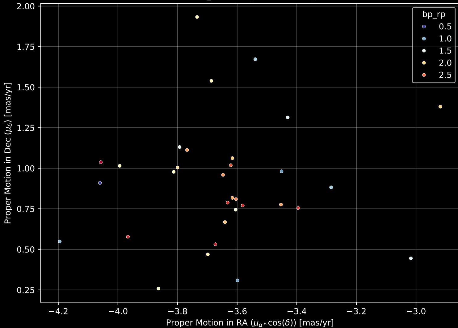
Gaia Cluster: [FSR 1117] Proper Motion Diagram (n= 32)
