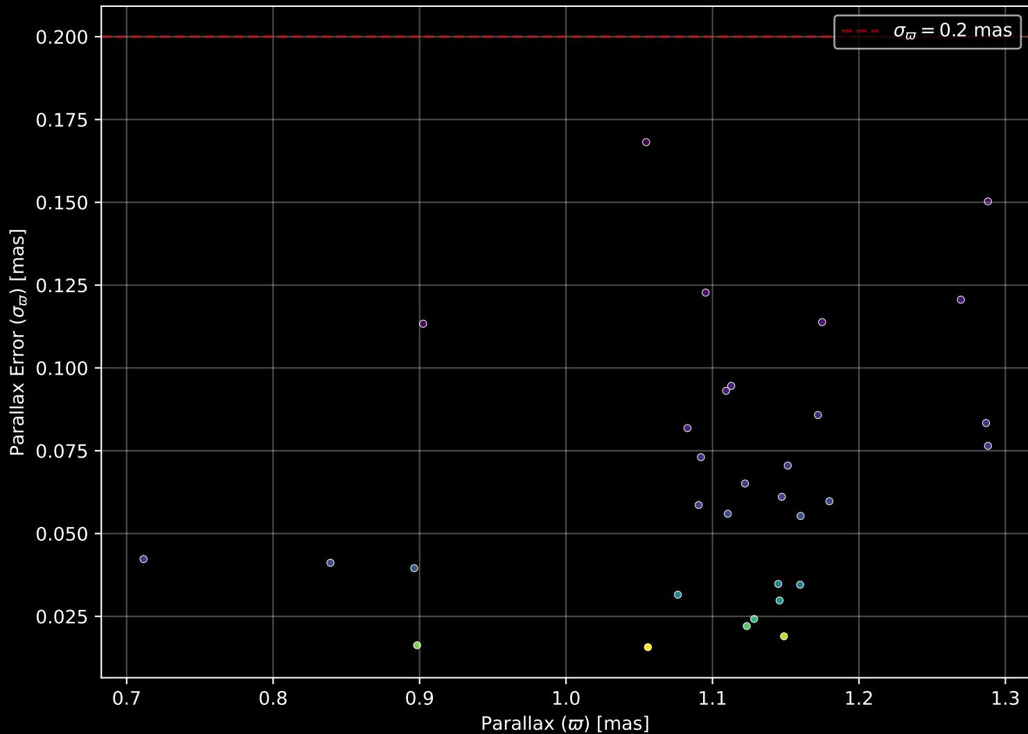
Gaia Cluster: [FSR_1117] Parallax Quality (n= 32)
