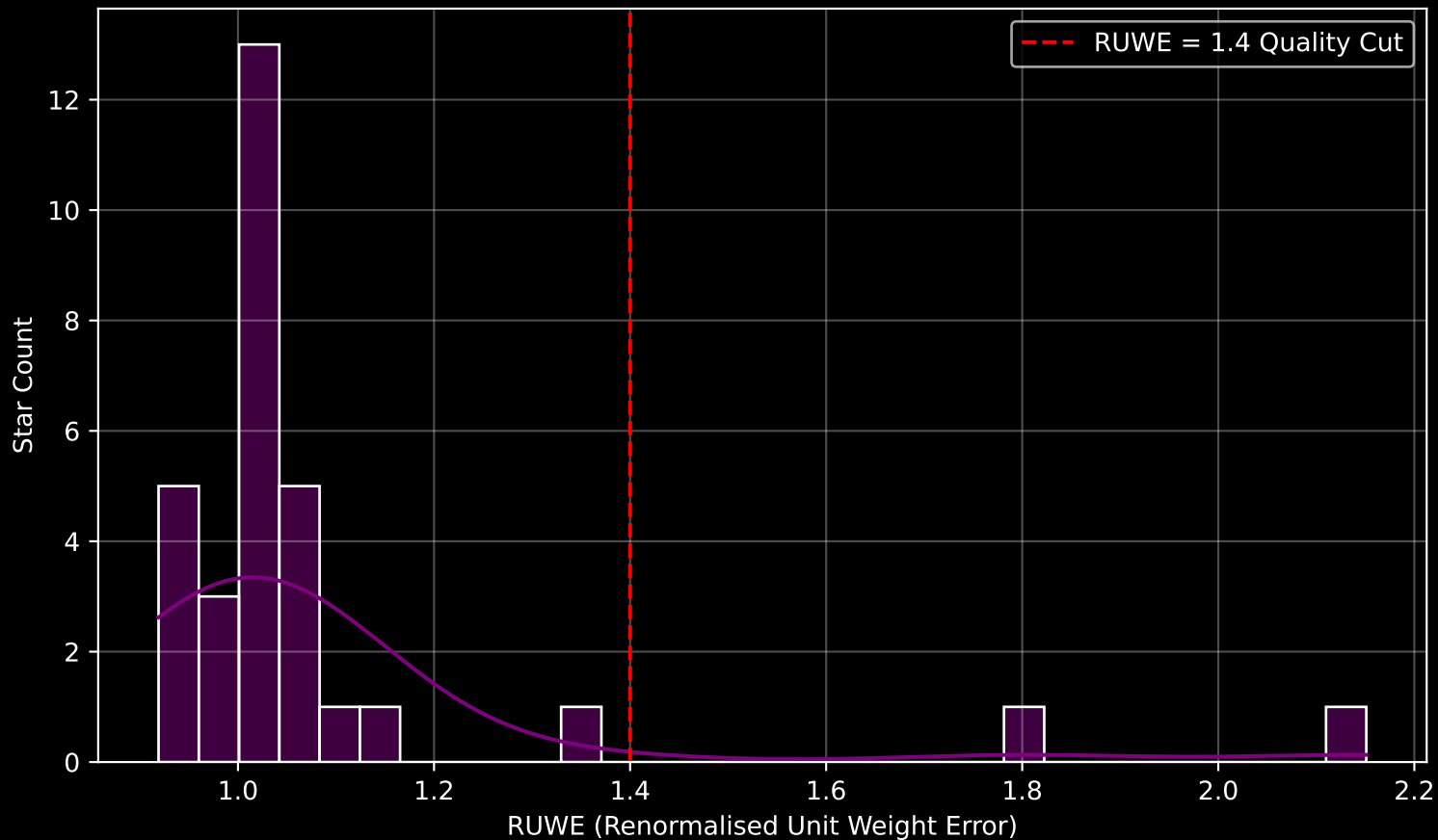
Gaia Cluster: [FSR_1117] RUWE Distribution (n= 31)
