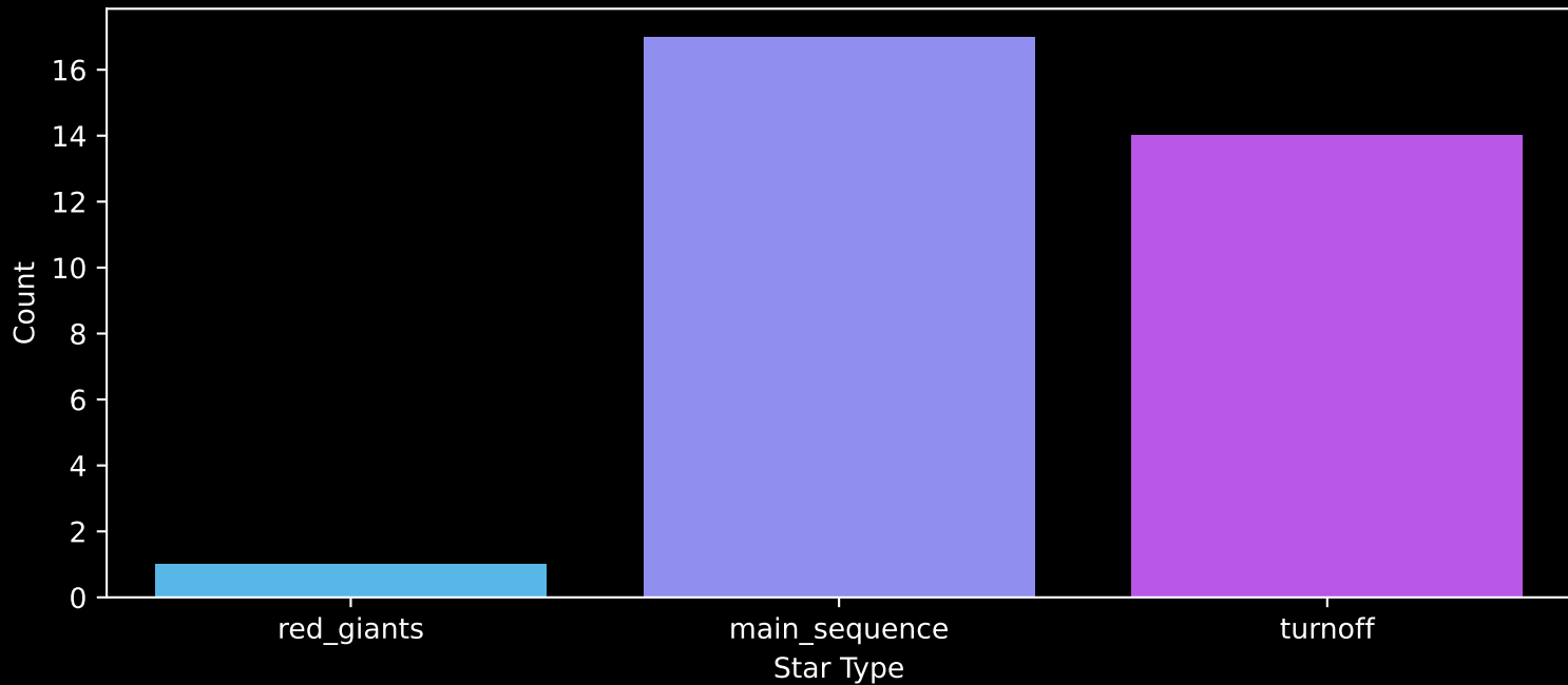
Gaia Cluster: [FSR_1117] Count plot of Star Type
