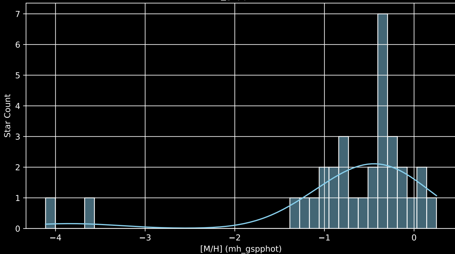
Gaia Cluster: [FSR_1117 [M/H] (mh_gspphot) (n= 32)
