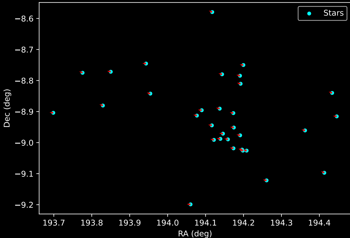
Gaia Cluster: [FSR_1117] Proper Motion Vectors for Gaia Star Field (n= 32)
