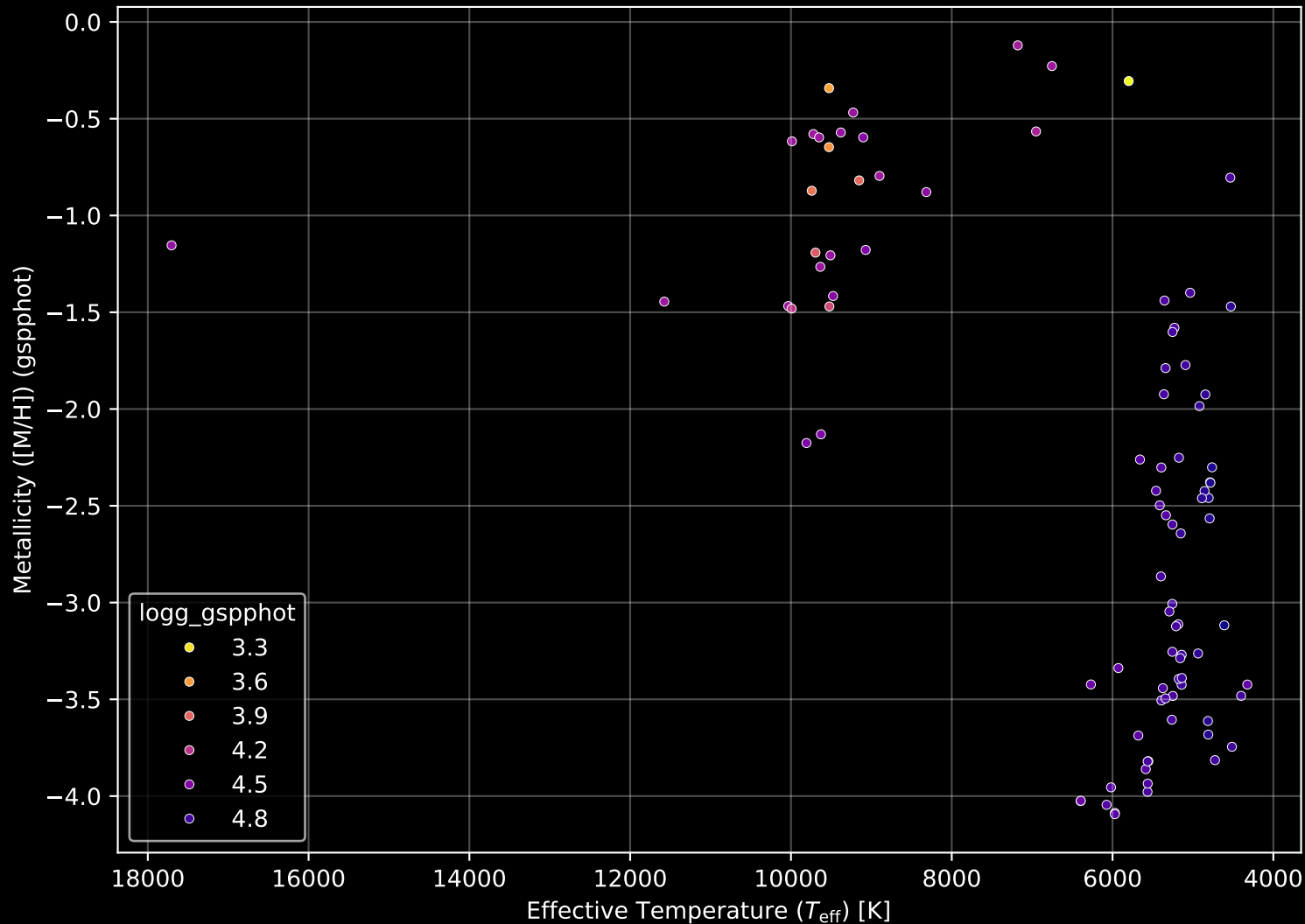
Gaia Cluster: [FSR_1125] Stellar Population Parameters (n= 92)
