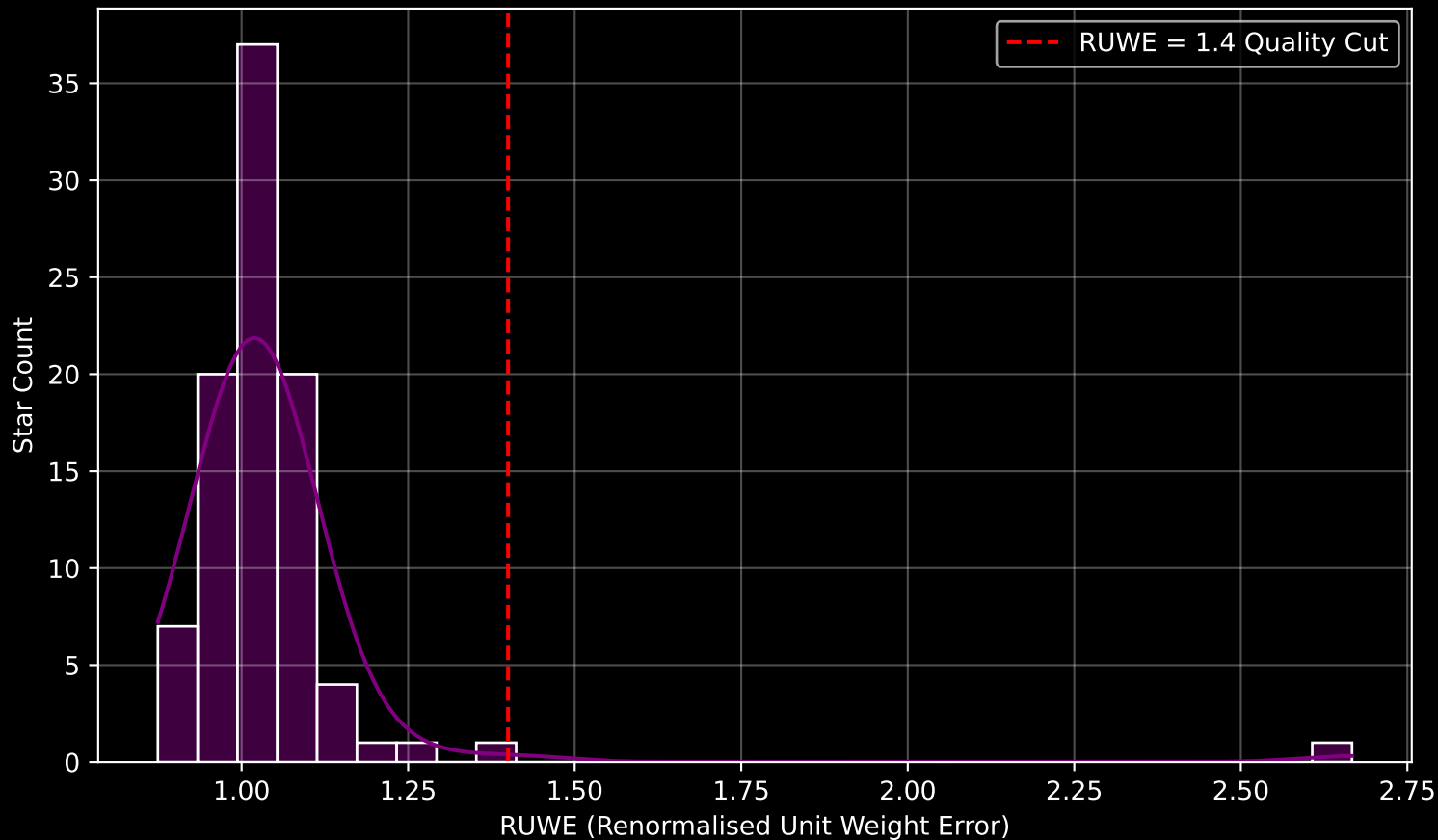
Gaia Cluster: [FSR_1125] RUWE Distribution (n= 92)
