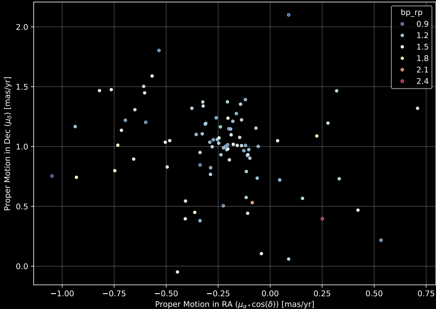
Gaia Cluster: [FSR_1125] Proper Motion Diagram (n= 92)
