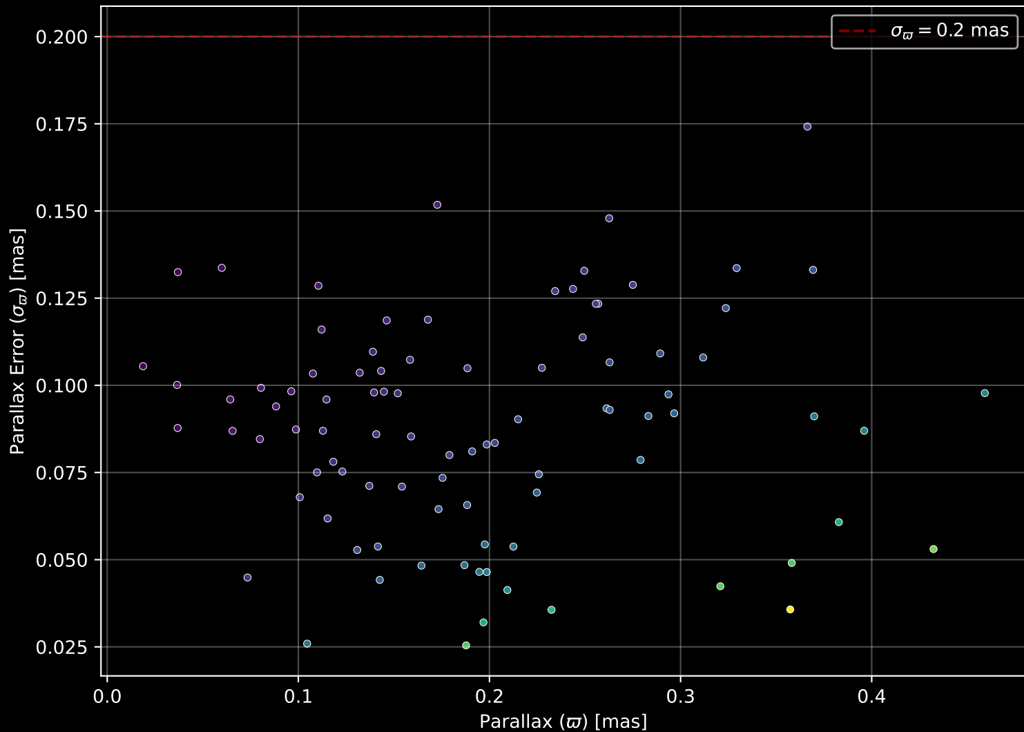
Gaia Cluster: [FSR_1125] Parallax Quality (n= 92)
