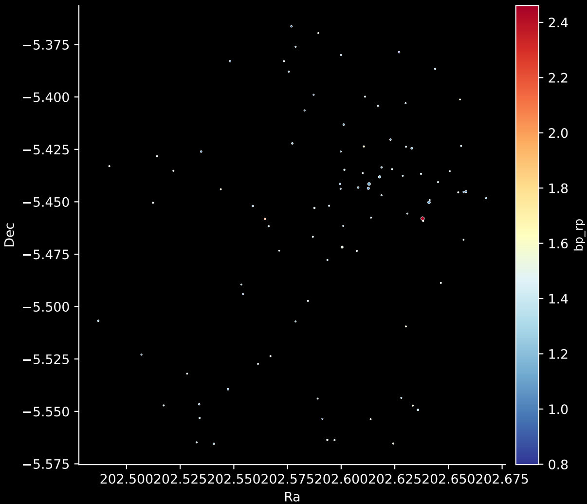
Gaia Cluster: [FSR_1125] Stars: 92
