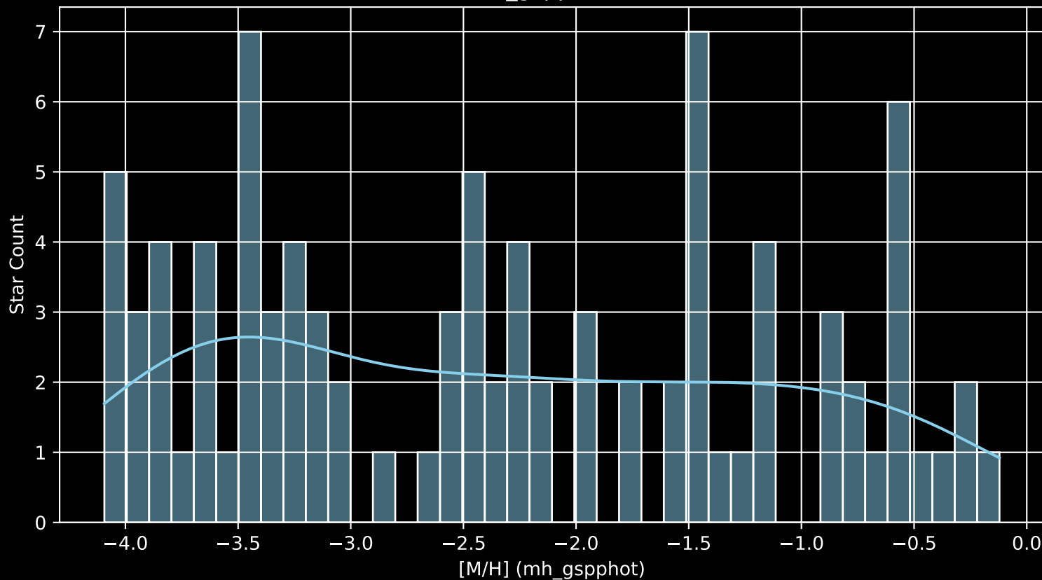
Gaia Cluster: [FSR_1125 [M/H] (mh_gspphot) (n= 92)
