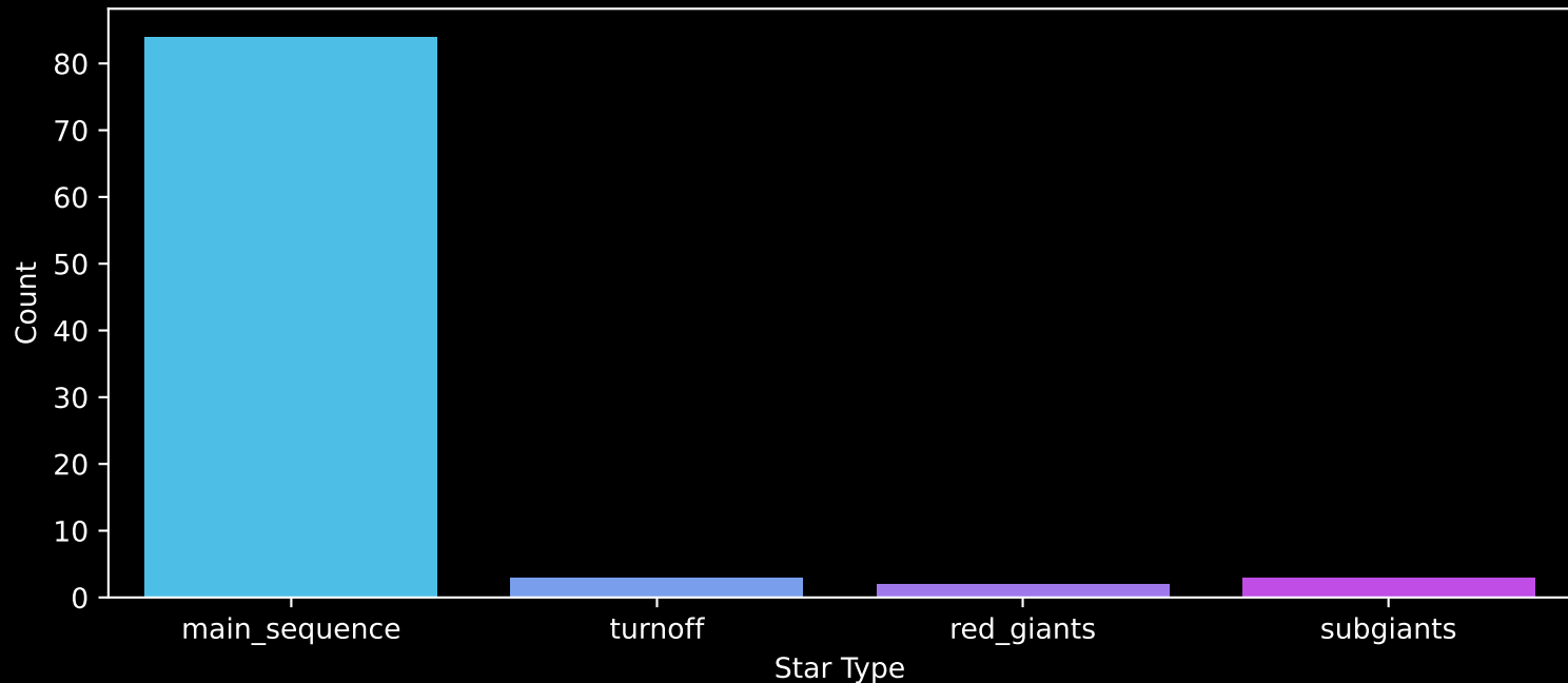
Gaia Cluster: [FSR_1125] Count plot of Star Type
