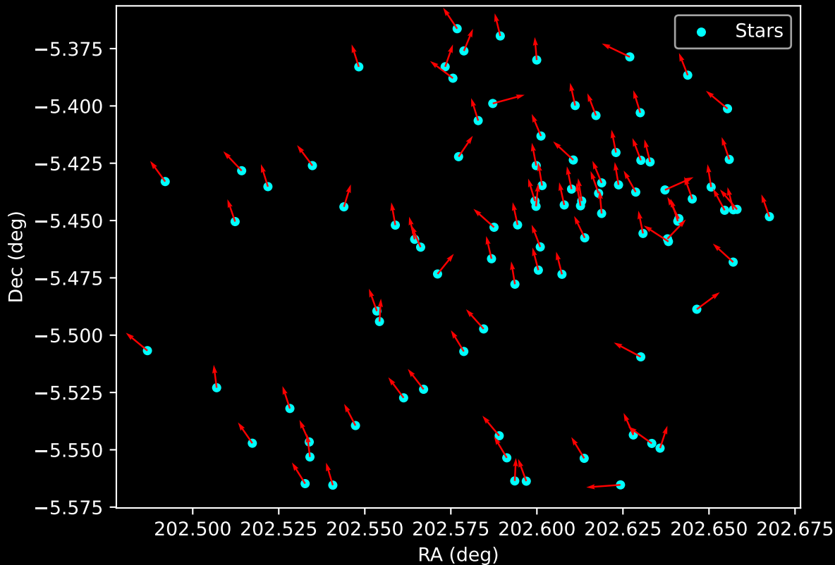
Gaia Cluster: [FSR_1125] Proper Motion Vectors for Gaia Star Field (n= 92)
