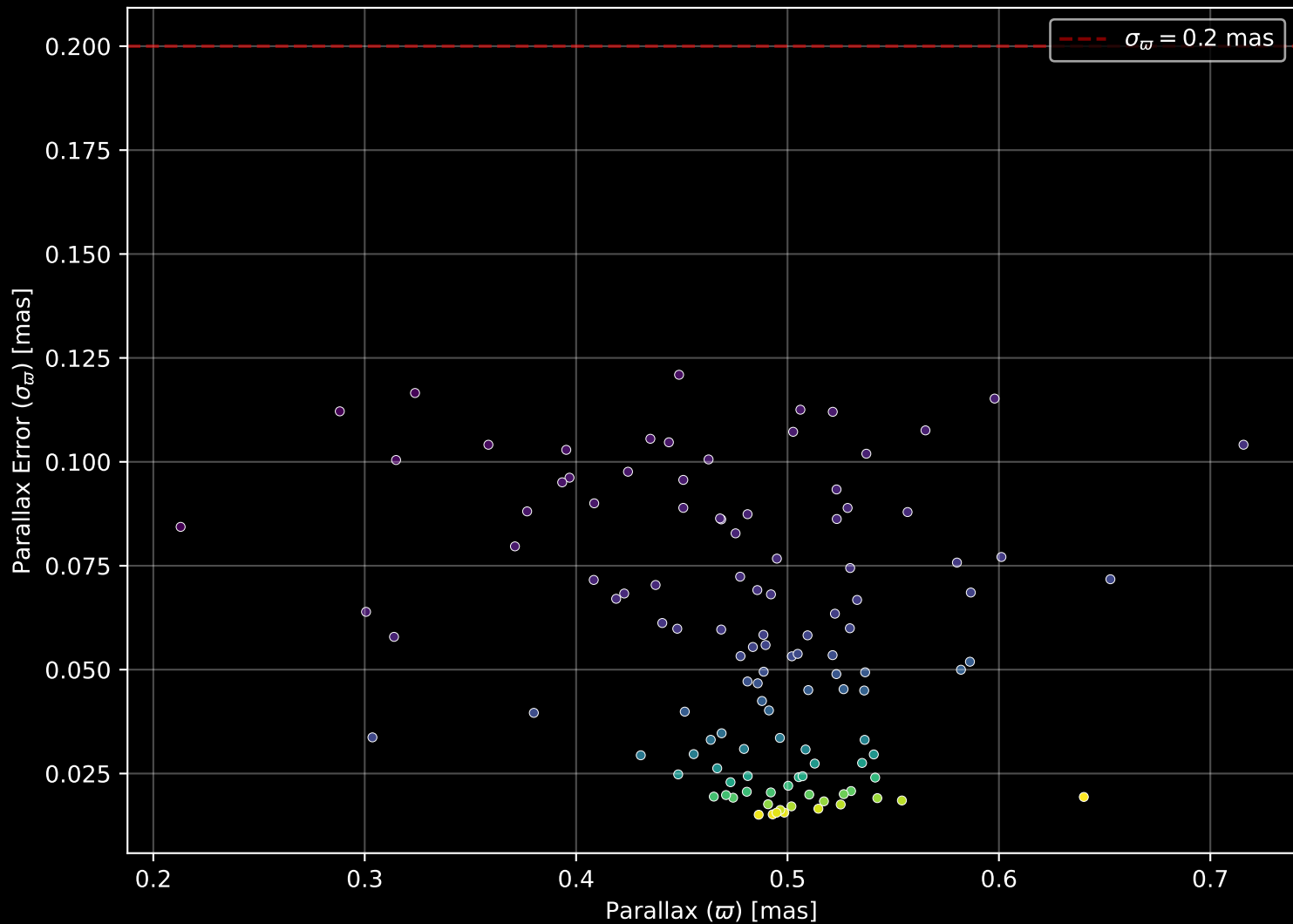
Gaia Cluster: [FSR_1144] Parallax Quality (n= 117)
