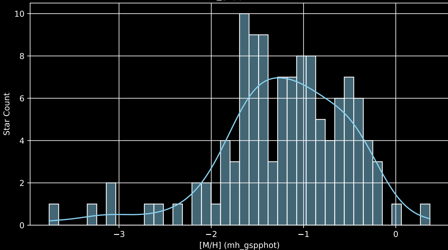
Gaia Cluster: [FSR_1144 [M/H] (mh_gspphot) (n= 117)
