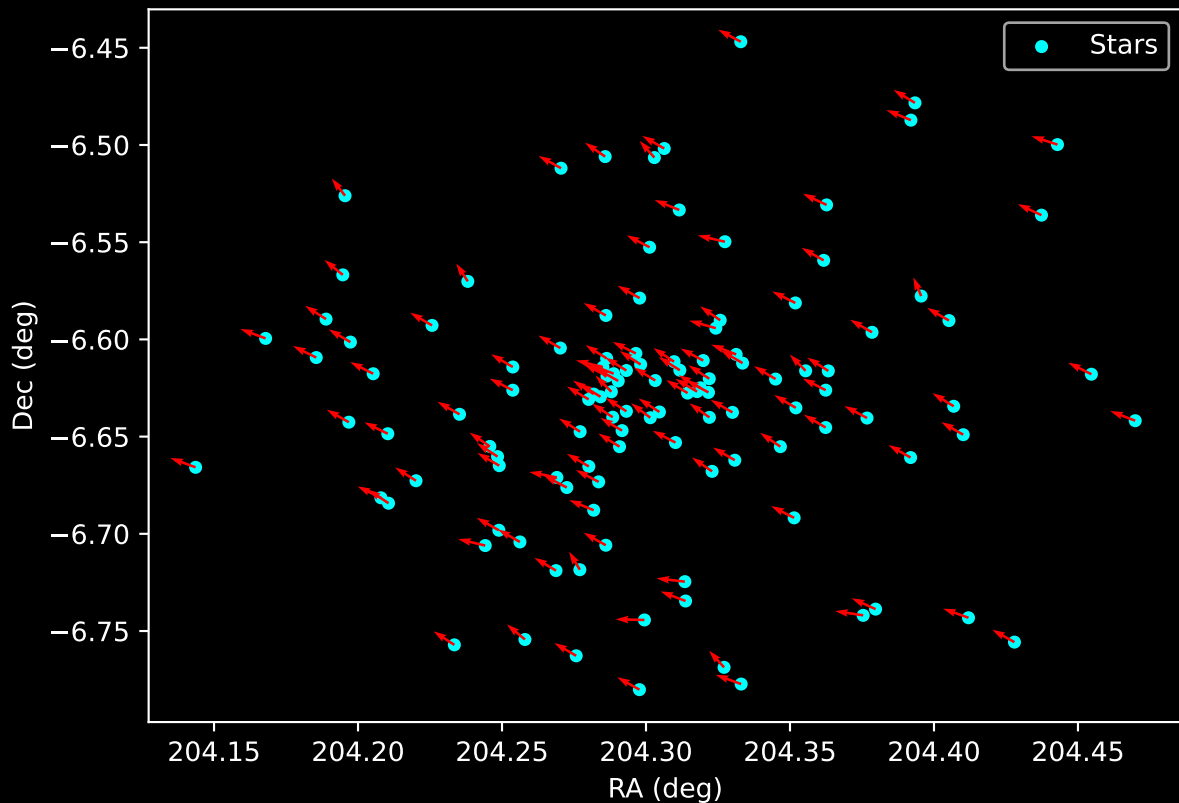
Gaia Cluster: [FSR_1144] Proper Motion Vectors for Gaia Star Field (n= 117)
