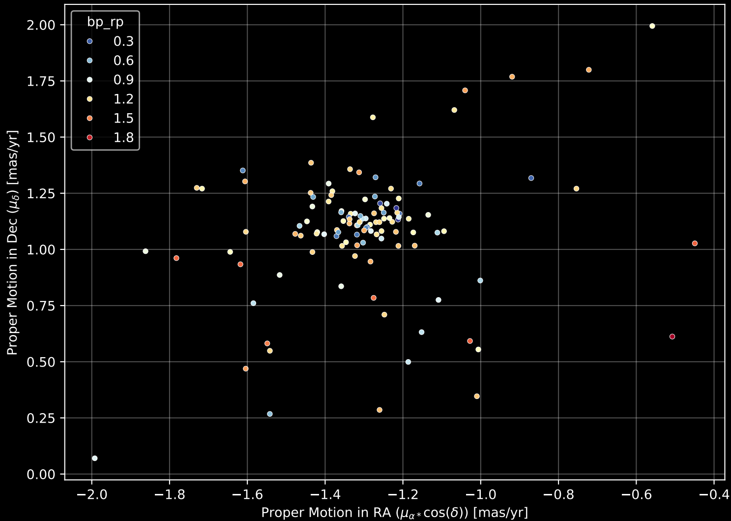
Gaia Cluster: [FSR_1144] Proper Motion Diagram (n= 117)
