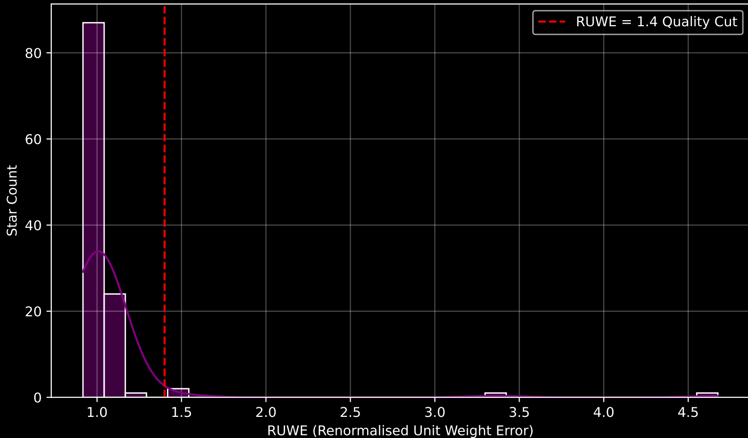
Gaia Cluster: [FSR_1144] RUWE Distribution (n= 116)
