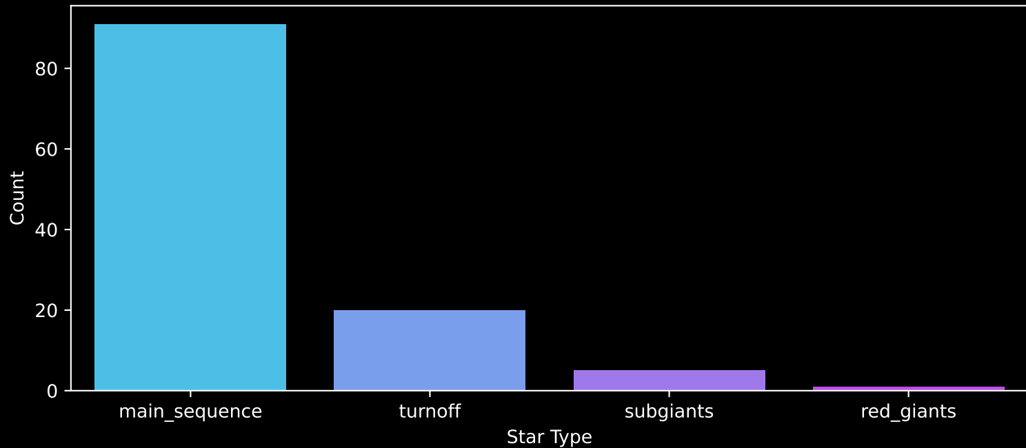
Gaia Cluster: [FSR_1144] Count plot of Star Type
