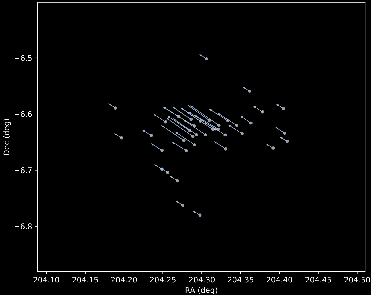
Gaia DR3 Cluster 1 Proper Motion Vectors (n=39)
