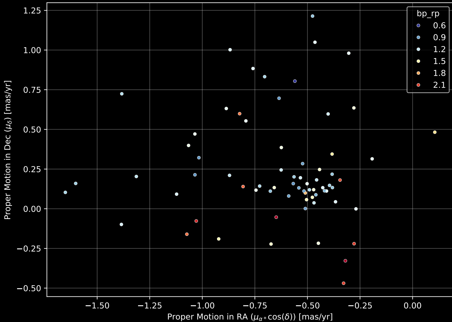
Gaia Cluster: [FSR_1150] Proper Motion Diagram (n= 70)
