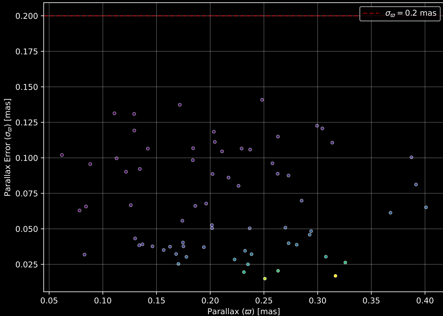
Gaia Cluster: [FSR_1150] Parallax Quality (n= 70)
