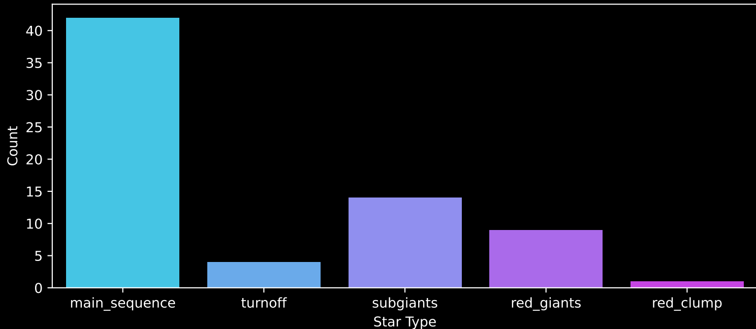
Gaia Cluster: [FSR_1150] Count plot of Star Type
