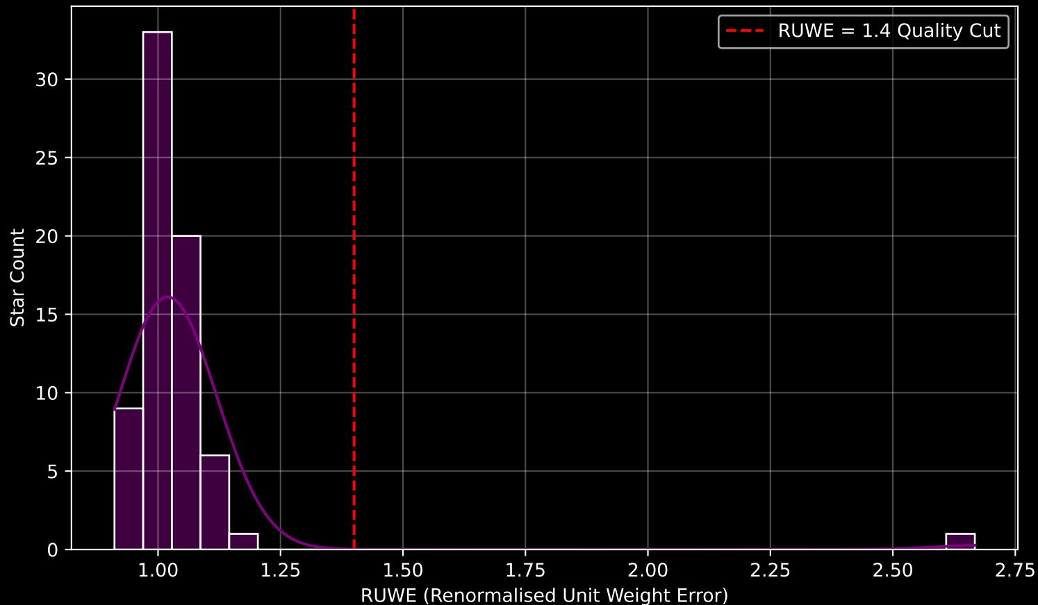
Gaia Cluster: [FSR_1150] RUWE Distribution (n= 70)
