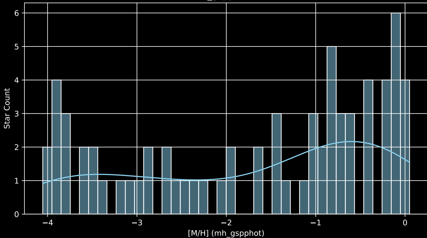
Gaia Cluster: [FSR_1150 [M/H] (mh_gspphot) (n= 69)
