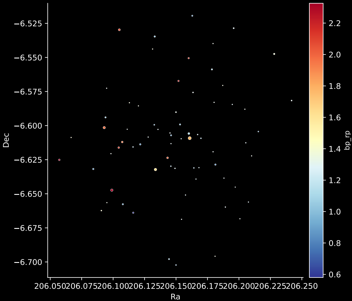
Gaia Cluster: [FSR_1150] Stars: 70
