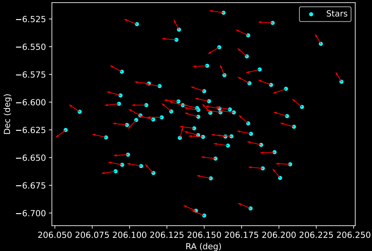
Gaia Cluster: [FSR_1150] Proper Motion Vectors for Gaia Star Field (n= 70)
