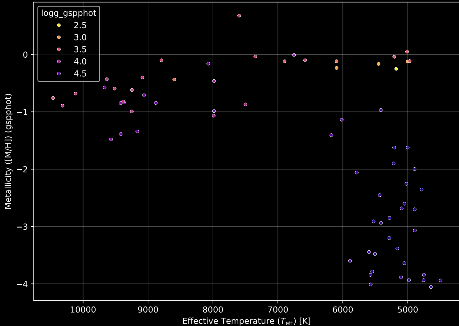
Gaia Cluster: [FSR_1150] Stellar Population Parameters (n= 70)
