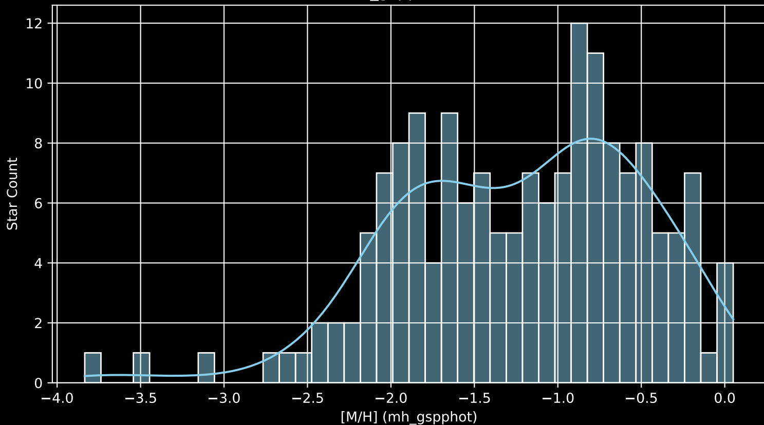
Gaia Cluster: [FSR_1153 [M/H] (mh_gspphot) (n= 165)
