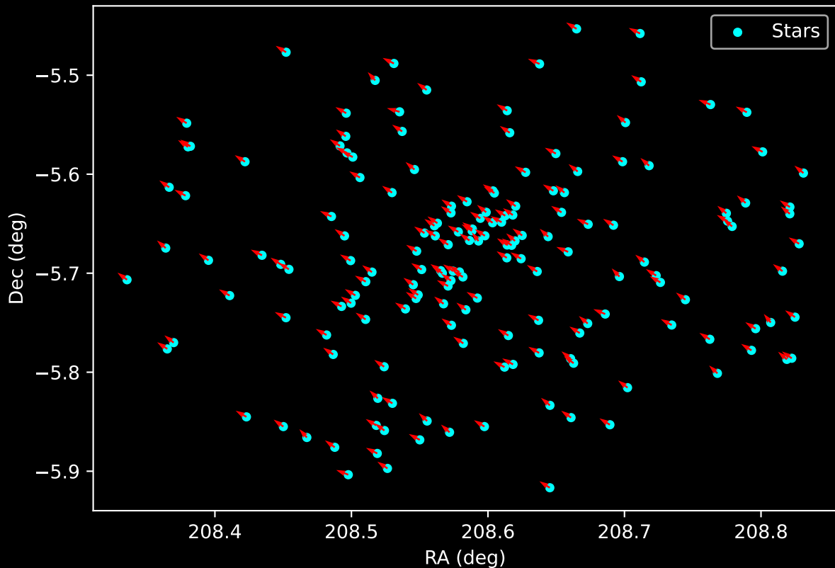
Gaia Cluster: [FSR_1153] Proper Motion Vectors for Gaia Star Field (n= 165)
