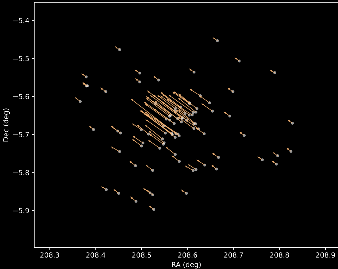
Gaia DR3 Cluster 3 Proper Motion Vectors (n=87)
