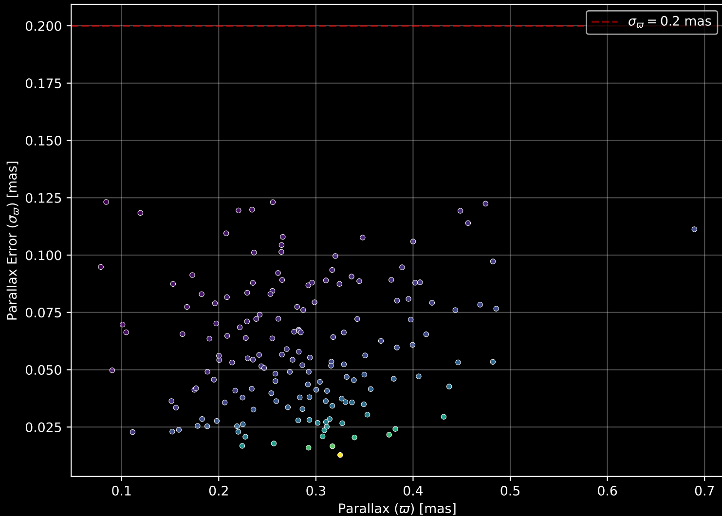
Gaia Cluster: [FSR_1153] Parallax Quality (n= 165)
