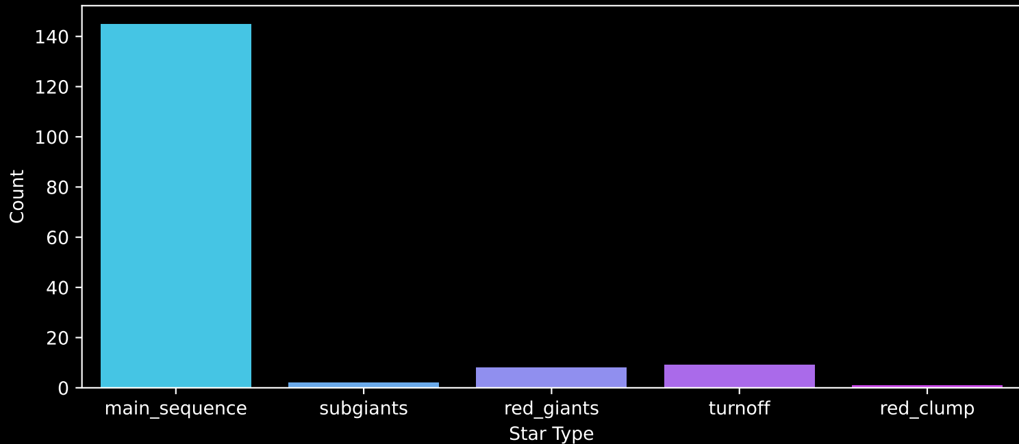
Gaia Cluster: [FSR_1153] Count plot of Star Type
