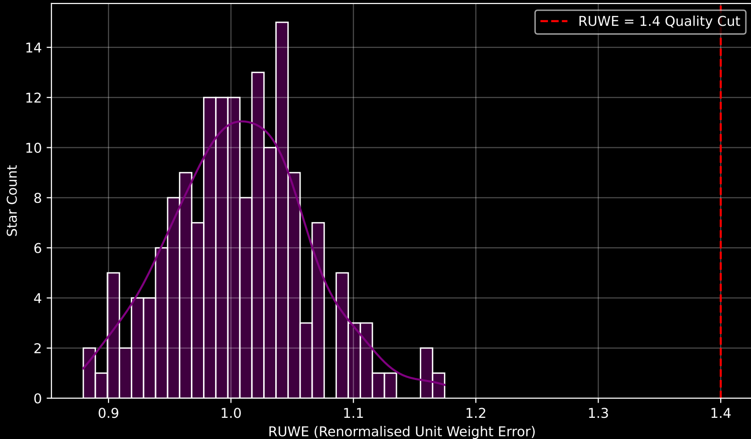
Gaia Cluster: [FSR_1153] RUWE Distribution (n= 165)
