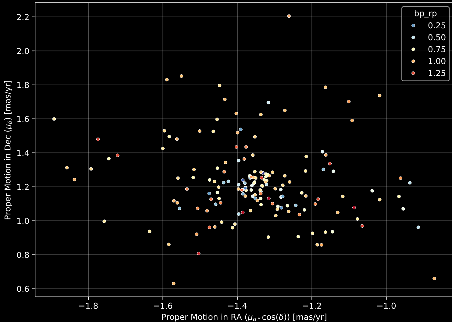
Gaia Cluster: [FSR_1153] Proper Motion Diagram (n= 165)
