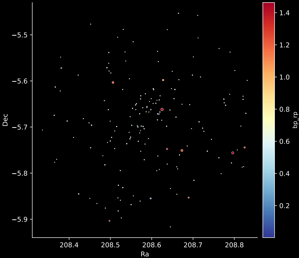
Gaia Cluster: [FSR_1153] Stars: 165
