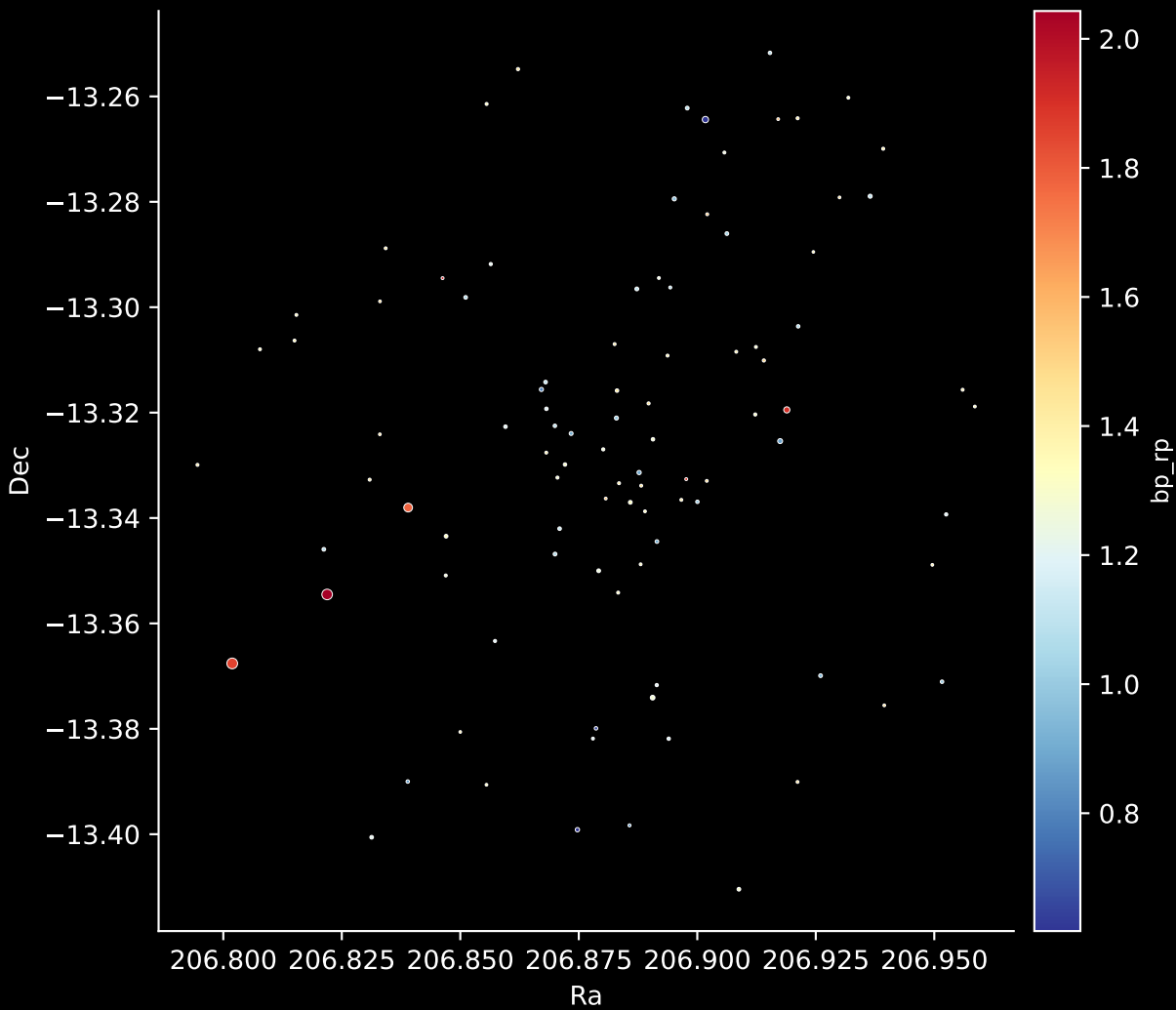
Gaia Cluster: [FSR_1207] Stars: 96
