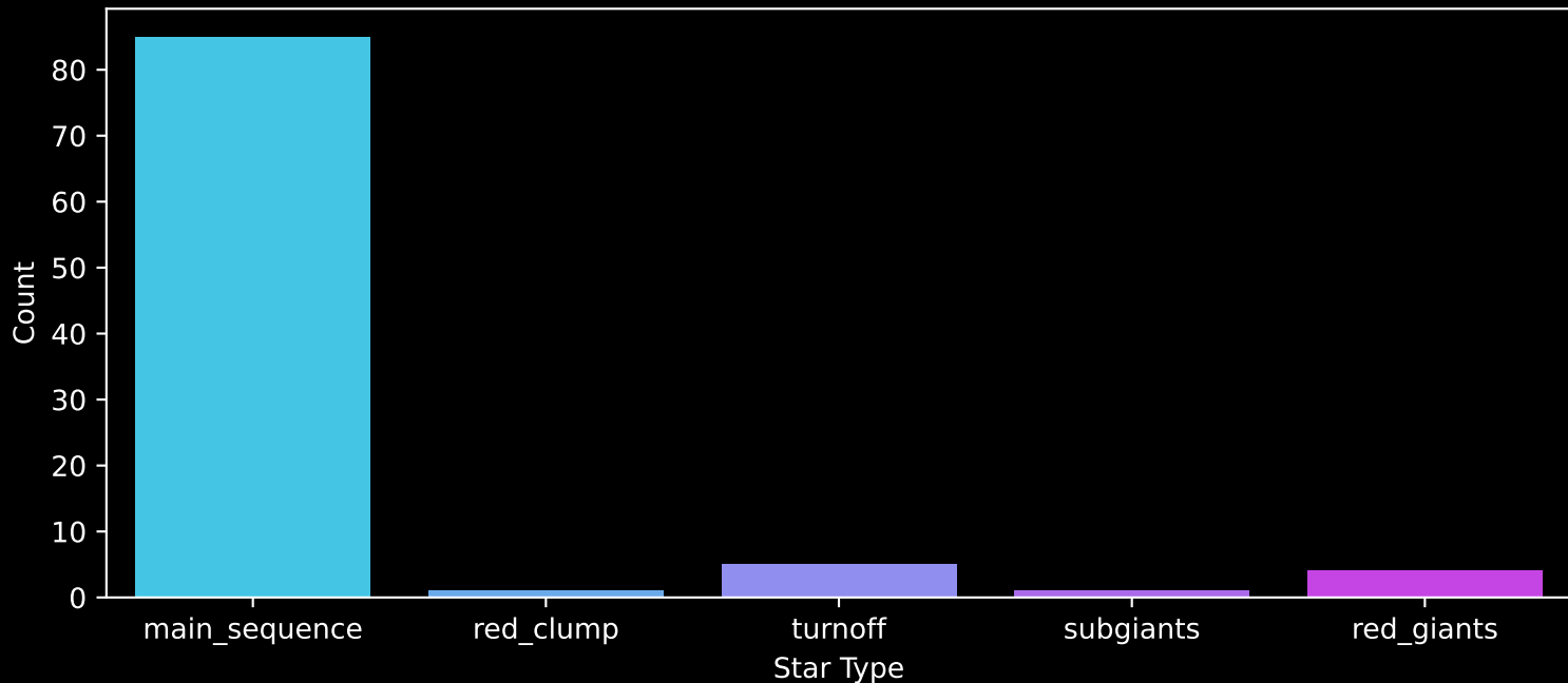
Gaia Cluster: [FSR_1207] Count plot of Star Type
