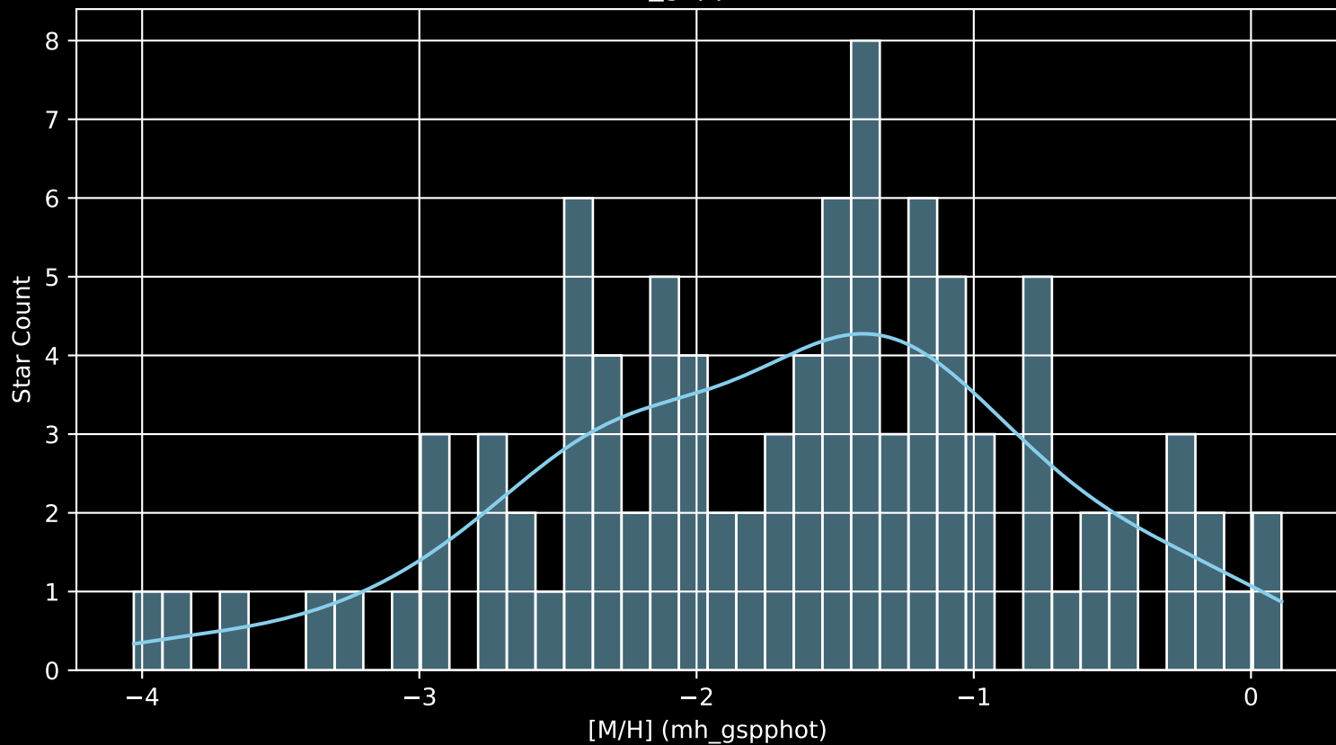
Gaia Cluster: [FSR_1207 [M/H] (mh_gspphot) (n= 96)
