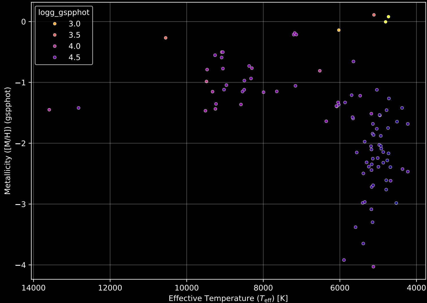
Gaia Cluster: [FSR_1207] Stellar Population Parameters (n= 96)
