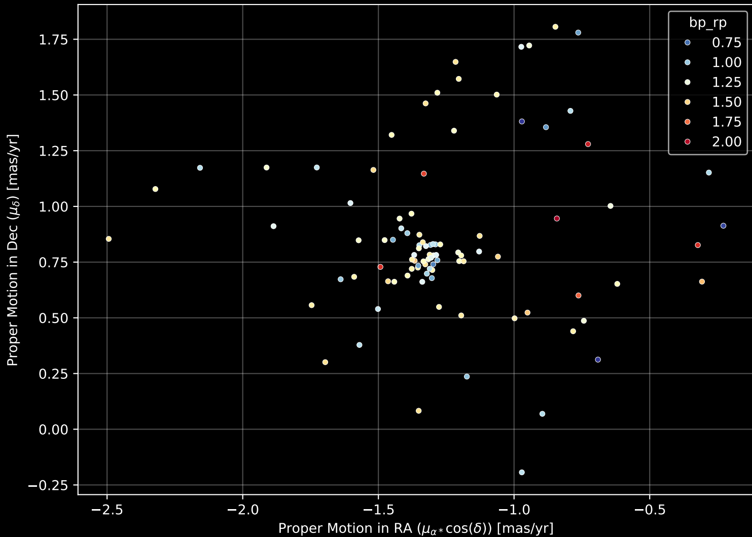
Gaia Cluster: [FSR_1207] Proper Motion Diagram (n= 96)
