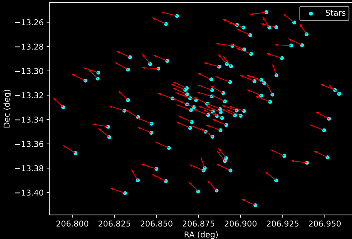
Gaia Cluster: [FSR_1207] Proper Motion Vectors for Gaia Star Field (n= 96)
