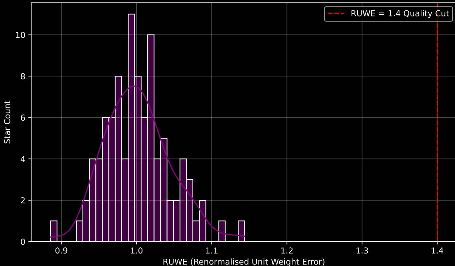
Gaia Cluster: [FSR_1207] RUWE Distribution (n= 96)
