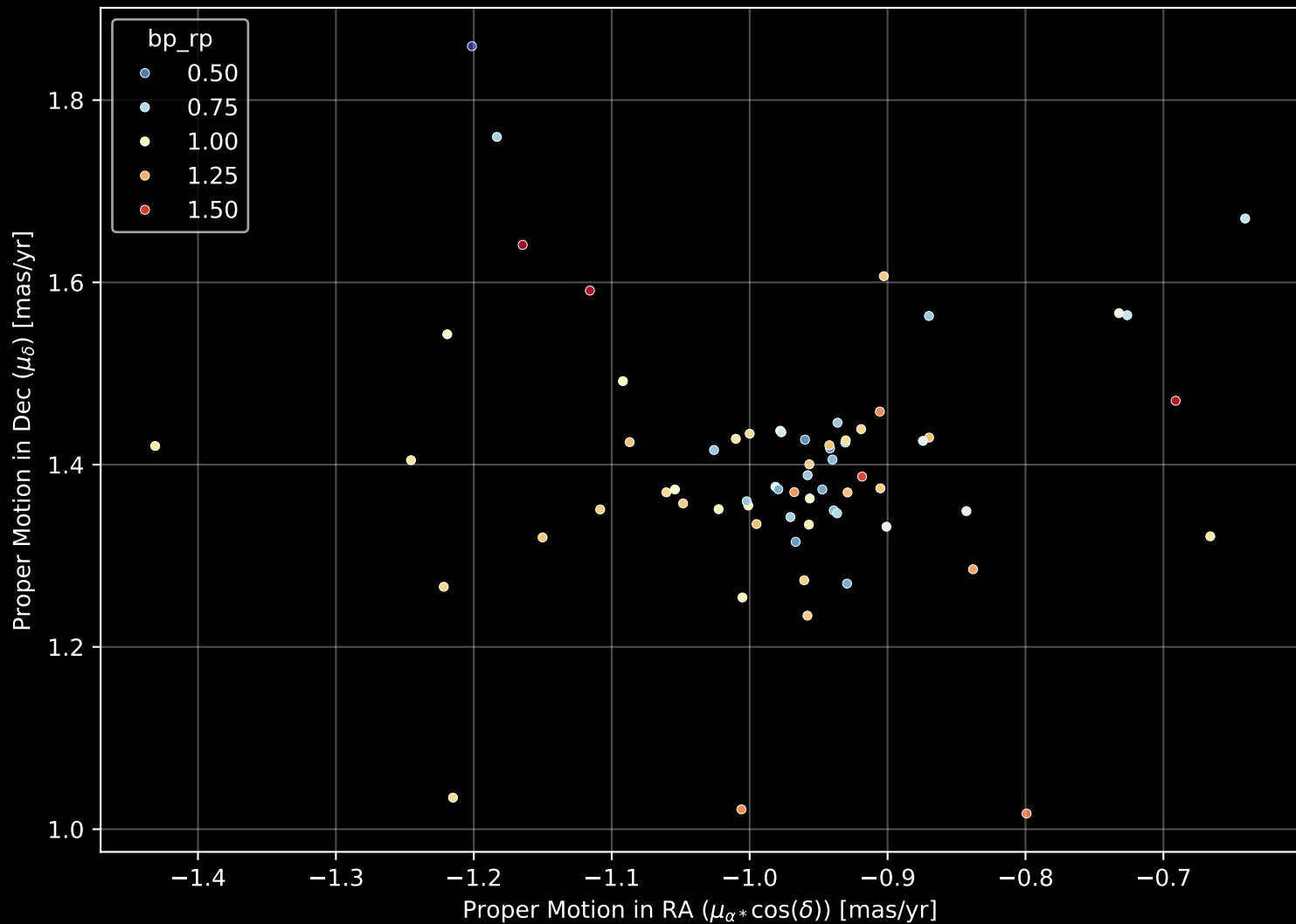
Gaia Cluster: [FSR_1284] Proper Motion Diagram (n= 67)
