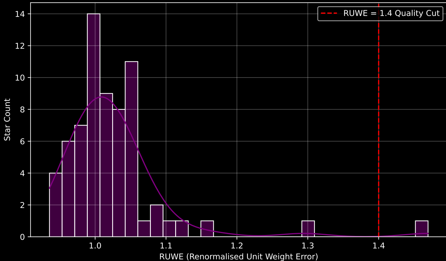
Gaia Cluster: [FSR_1284] RUWE Distribution (n= 67)
