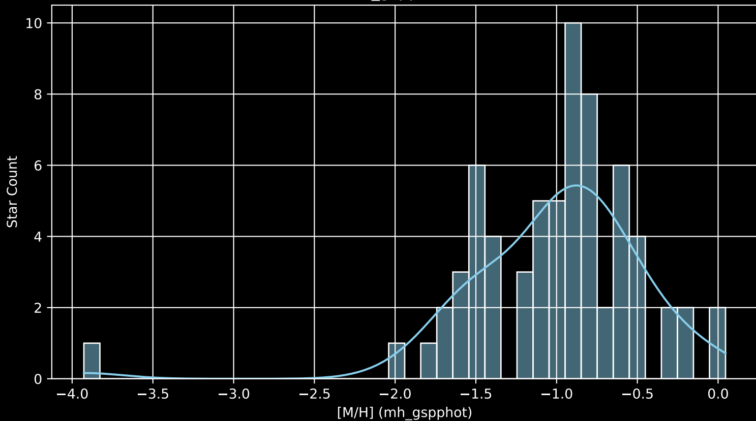
Gaia Cluster: [FSR_1284 [M/H] (mh_gspphot) (n= 67)
