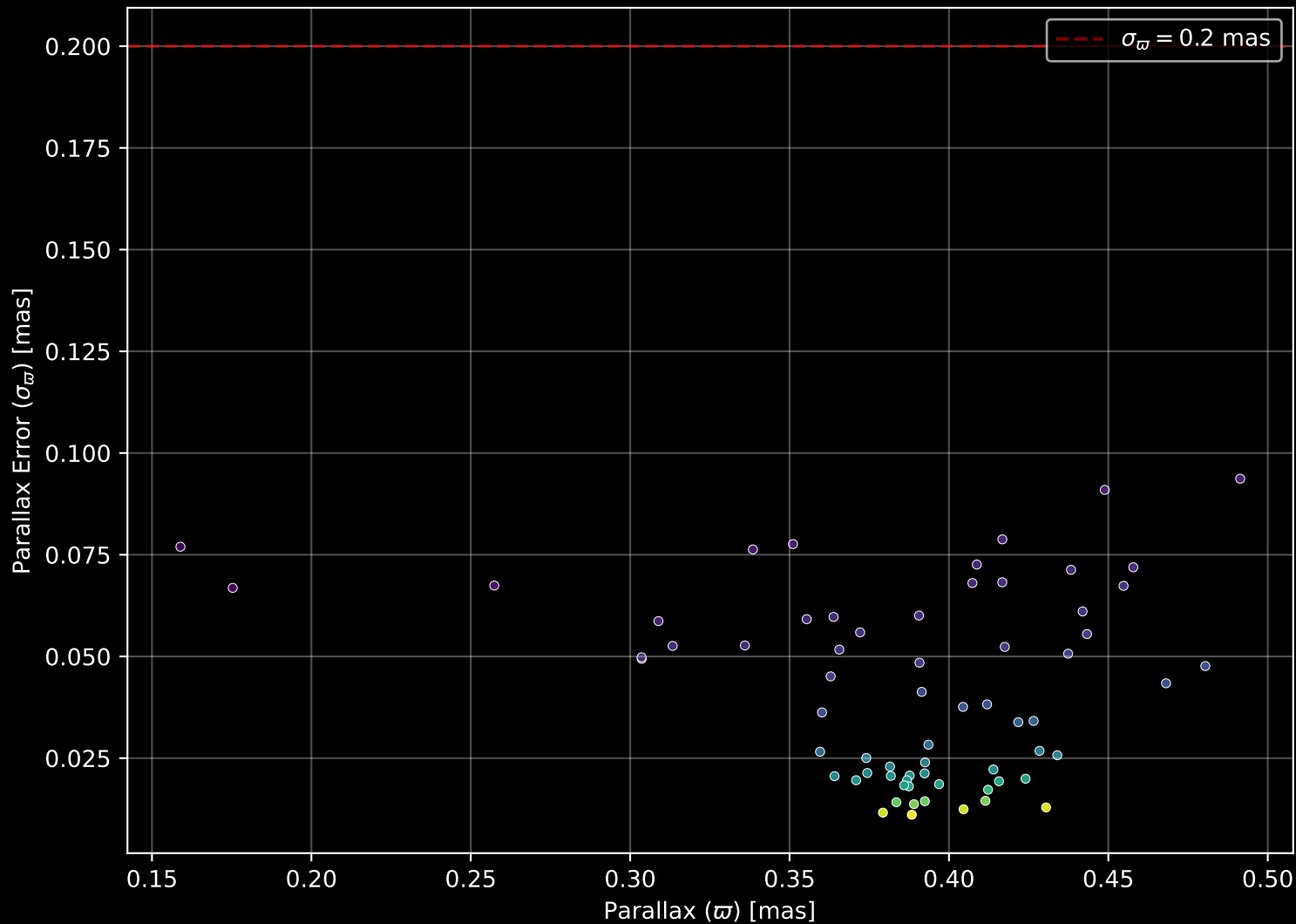
Gaia Cluster: [FSR_1284] Parallax Quality (n= 67)
