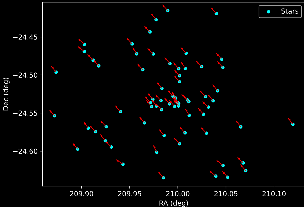
Gaia Cluster: [FSR_1284] Proper Motion Vectors for Gaia Star Field (n= 67)
