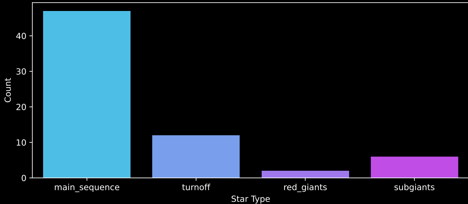
Gaia Cluster: [FSR_1284] Count plot of Star Type
