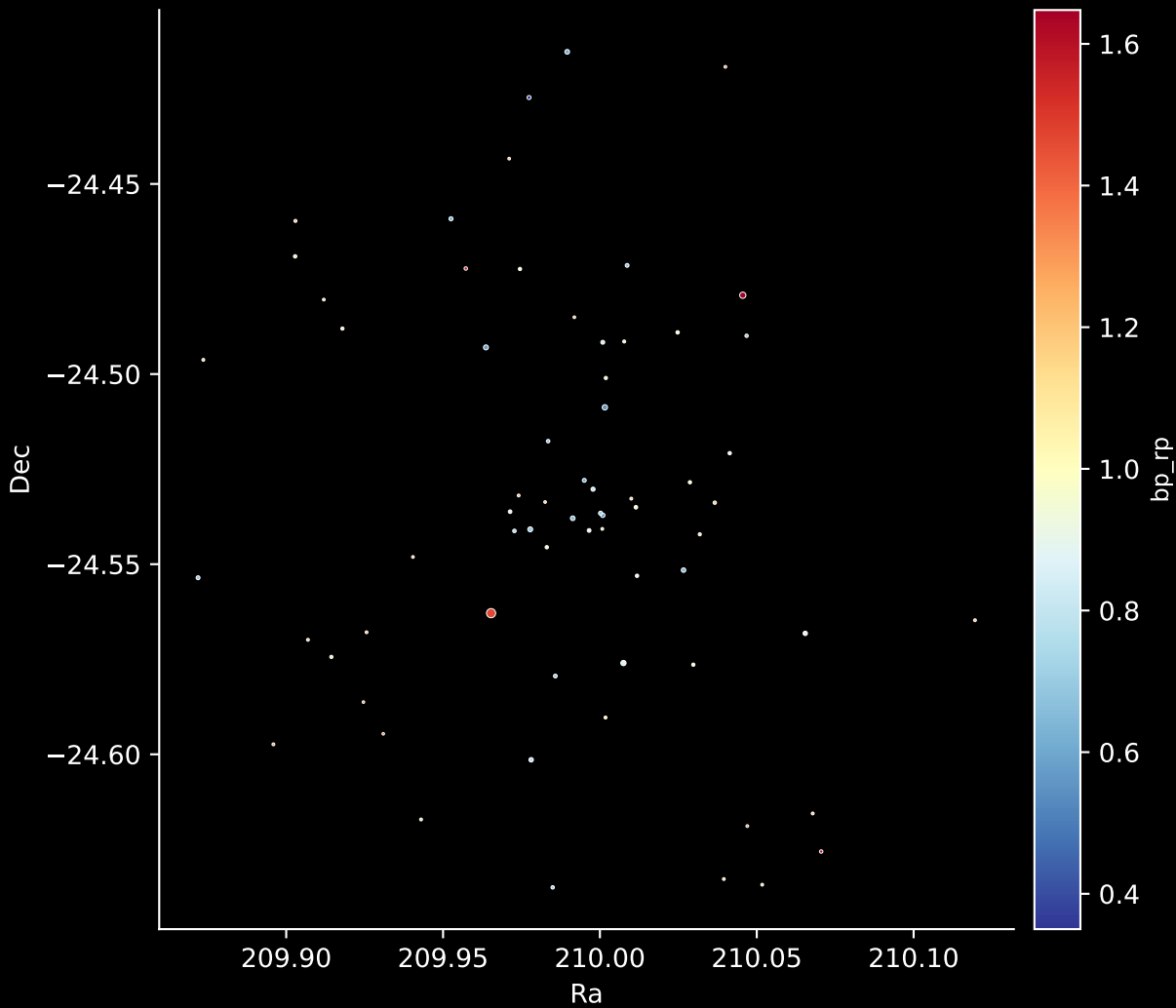
Gaia Cluster: [FSR_1284] Stars: 67
