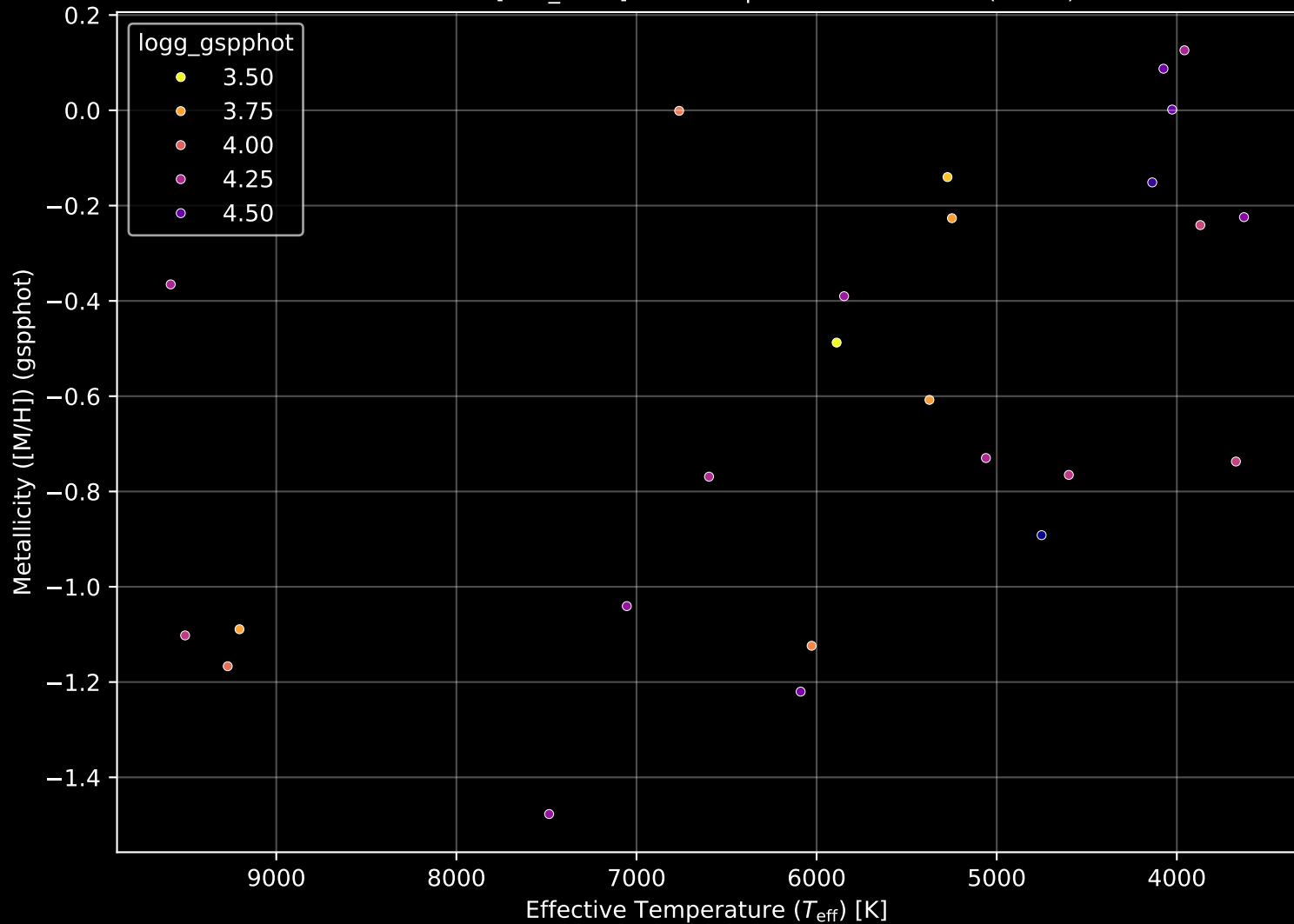
Gaia Cluster: [FSR_1297] Stellar Population Parameters (n= 25)
