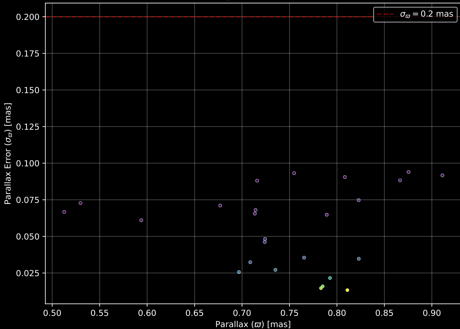
Gaia Cluster: [FSR_1297] Parallax Quality (n= 25)
