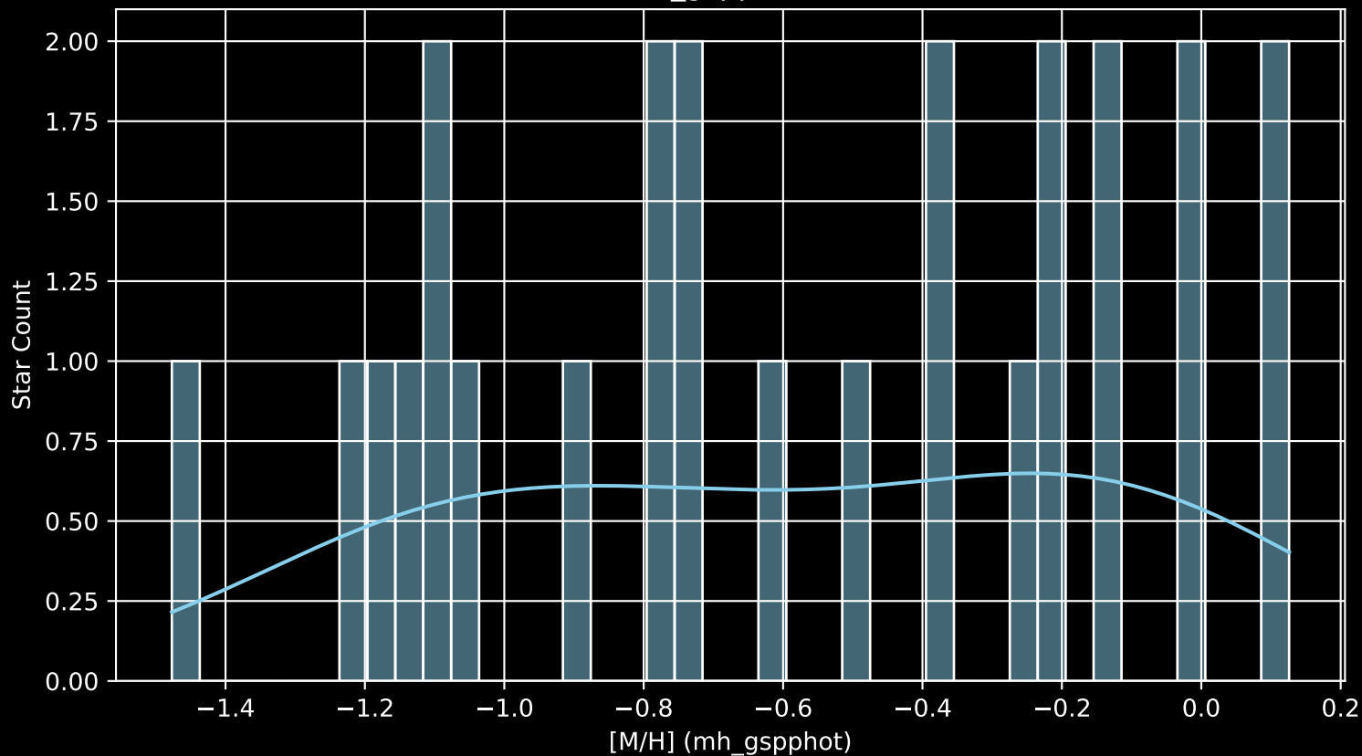
Gaia Cluster: [FSR_1297 [M/H] (mh_gspphot) (n= 25)
