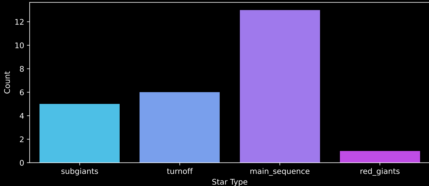
Gaia Cluster: [FSR_1297] Count plot of Star Type
