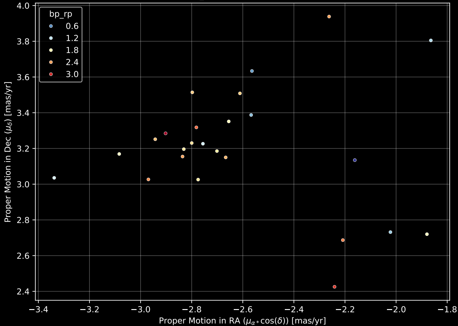
Gaia Cluster: [FSR_1297] Proper Motion Diagram (n= 25)
