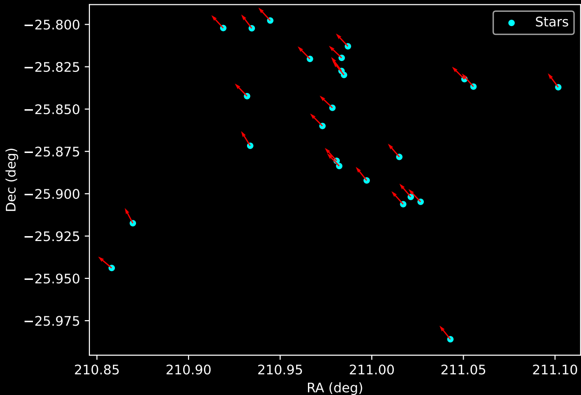
Gaia Cluster: [FSR_1297] Proper Motion Vectors for Gaia Star Field (n= 25)
