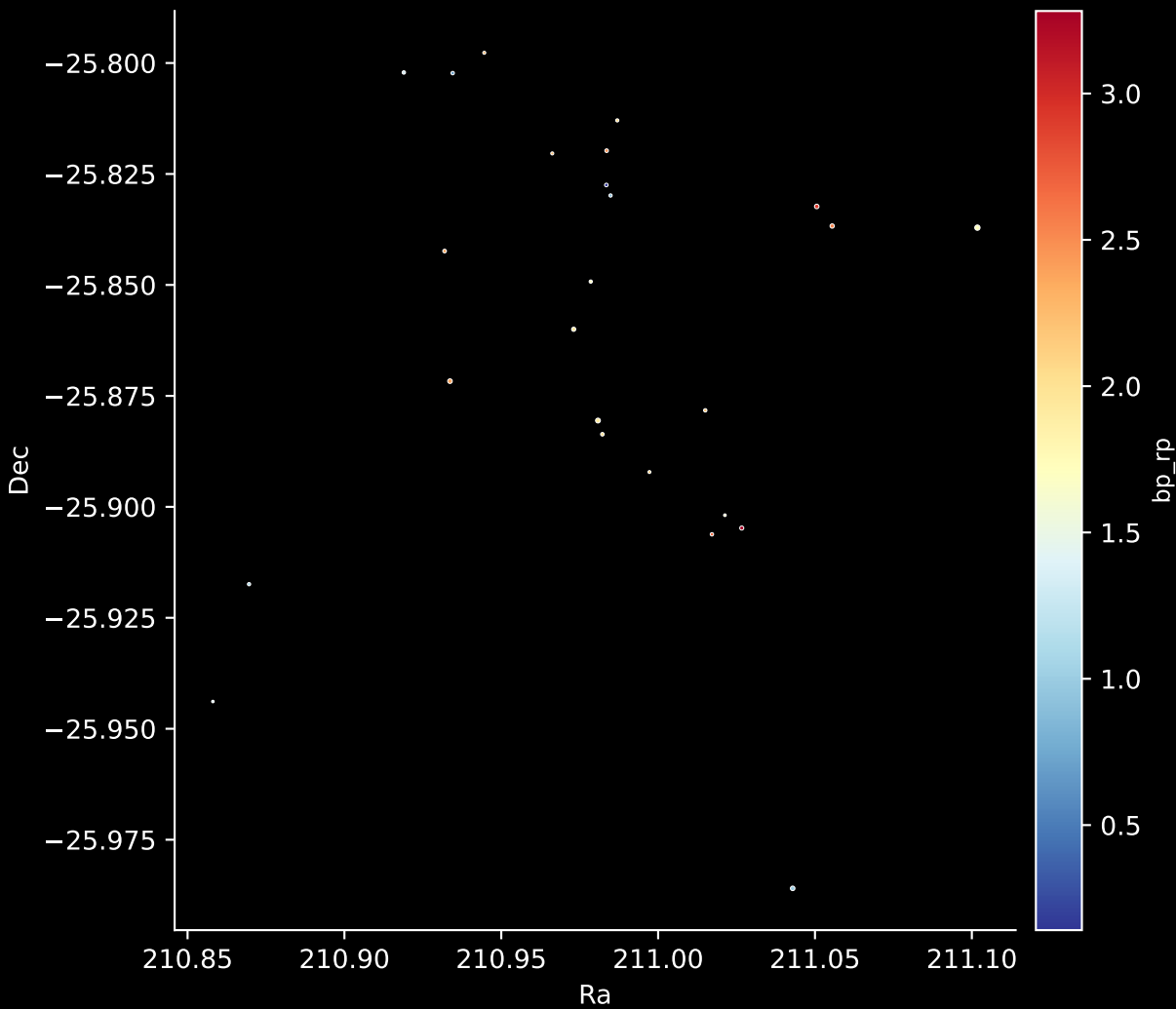
Gaia Cluster: [FSR_1297] Stars: 25
