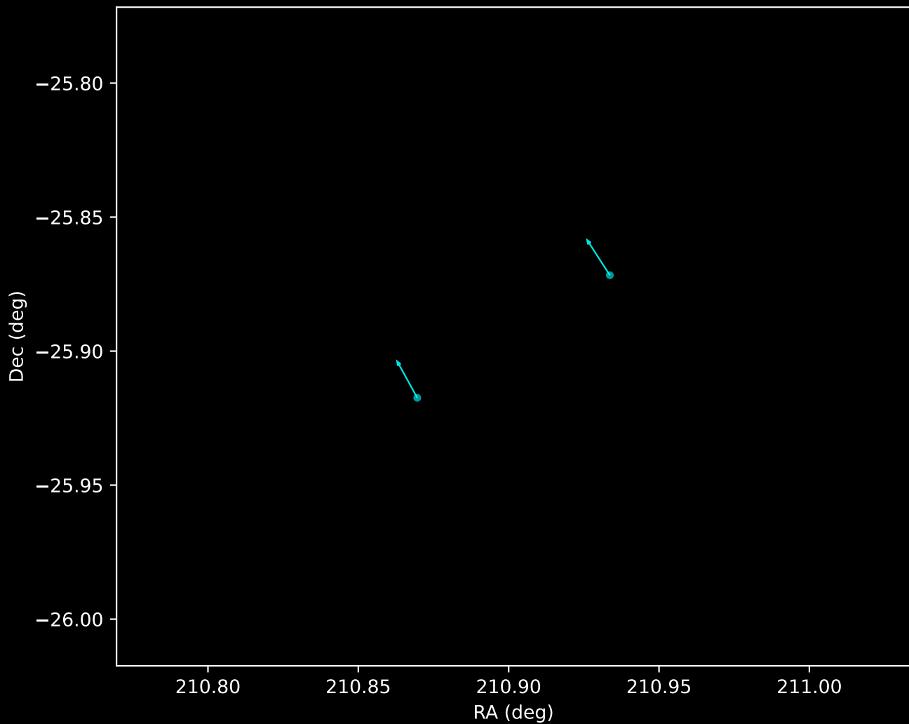
Gaia DR3 Noise Stream Proper Motion Vectors (n=2)
