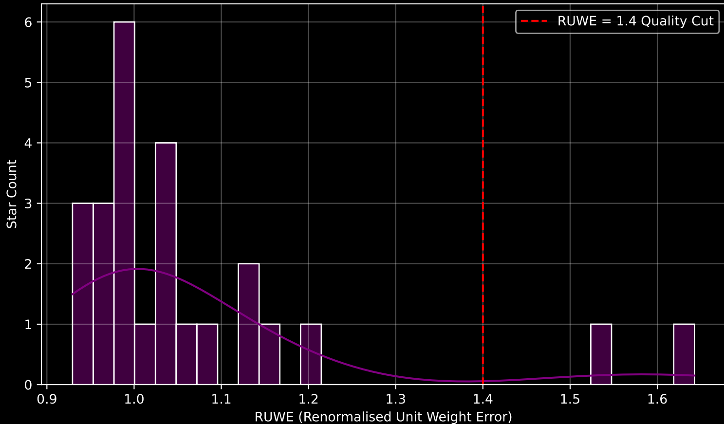
Gaia Cluster: [FSR_1297] RUWE Distribution (n= 25)
