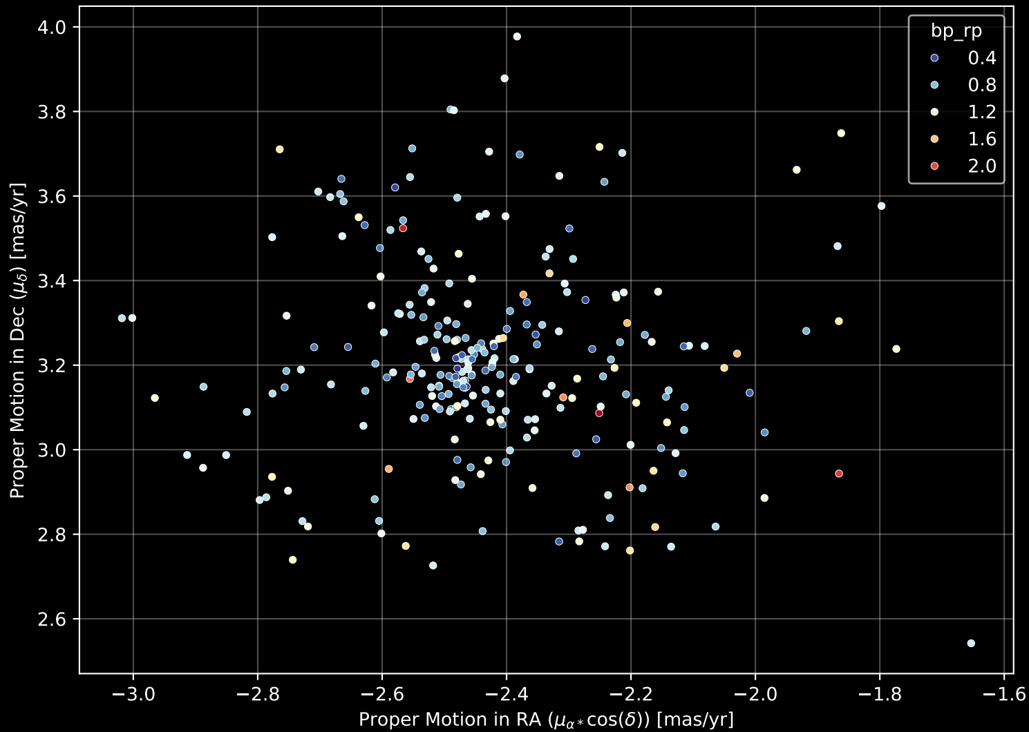
Gaia Cluster: [FSR_1315] Proper Motion Diagram (n= 269)
