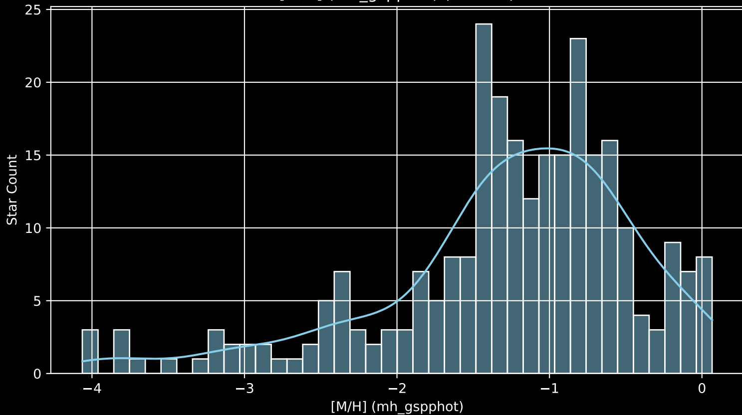
Gaia Cluster: [FSR_1315 [M/H] (mh_gspphot) (n= 269)
