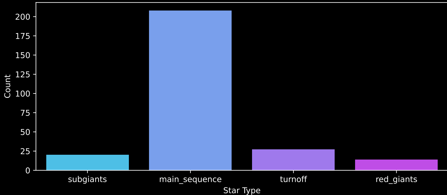
Gaia Cluster: [FSR_1315] Count plot of Star Type
