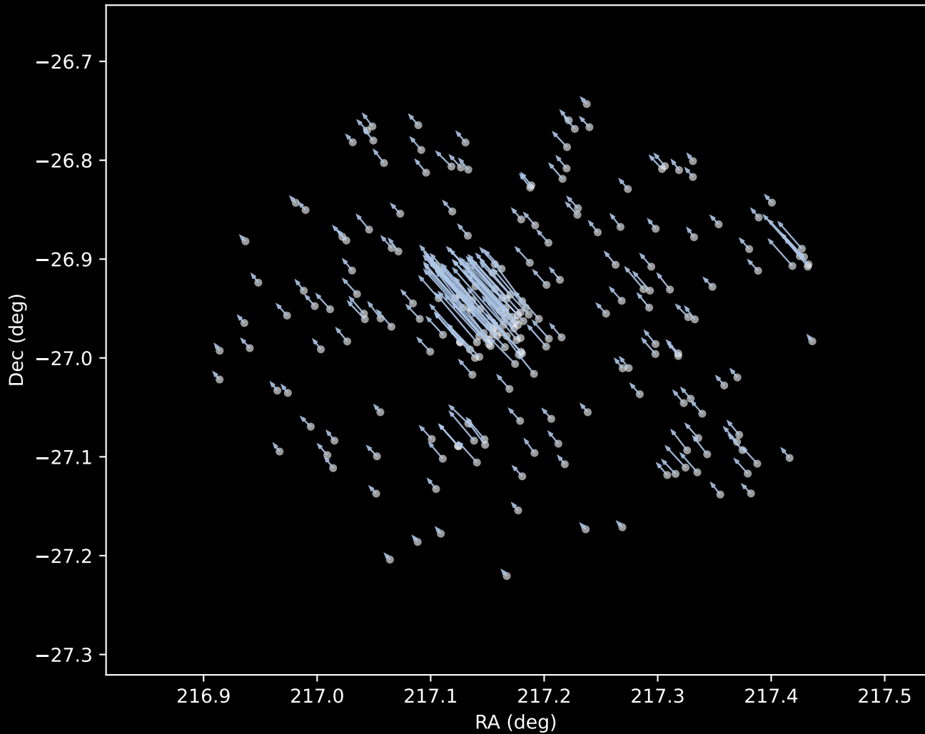
Gaia DR3 Cluster 1 Proper Motion Vectors (n=223)
