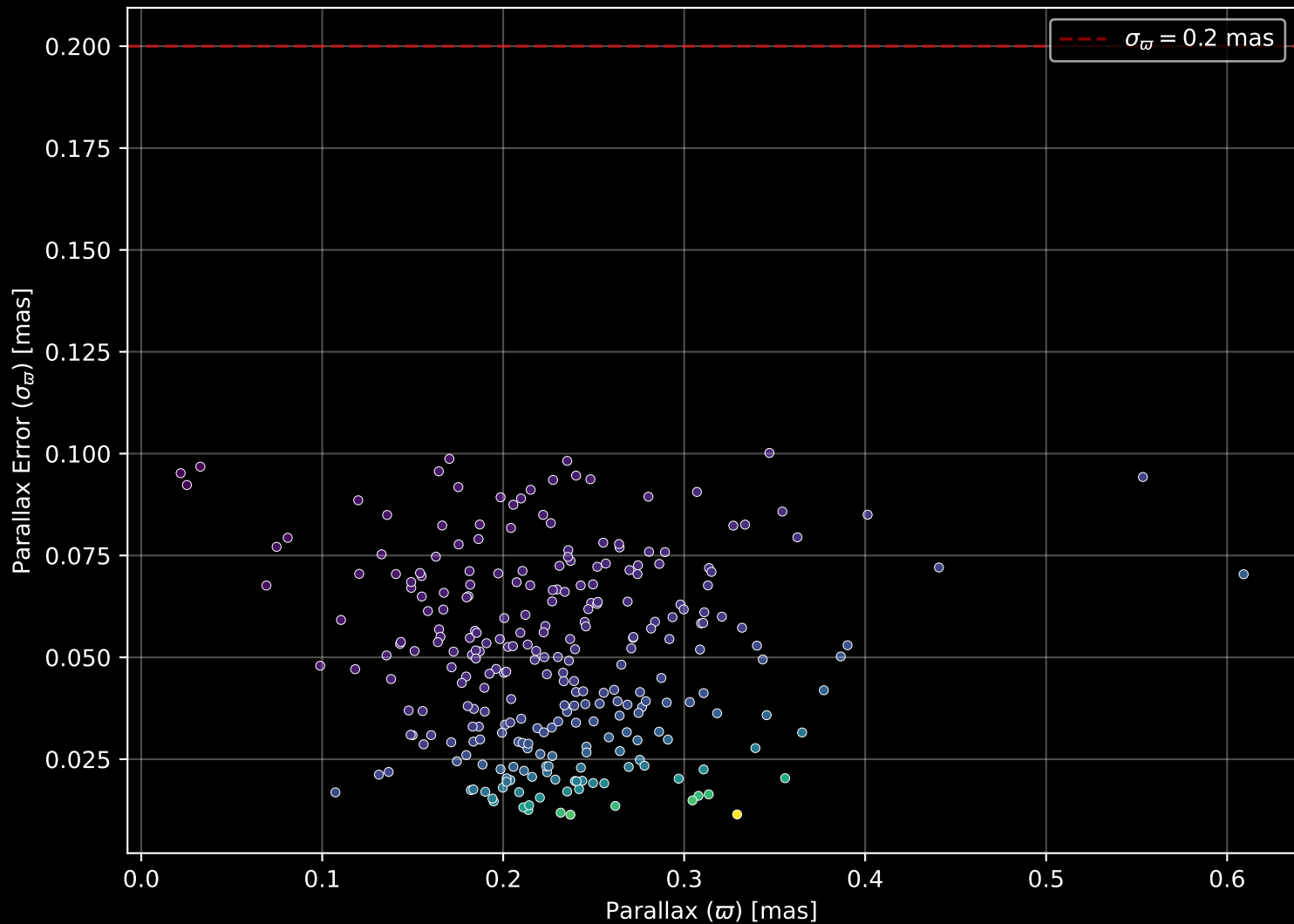
Gaia Cluster: [FSR_1315] Parallax Quality (n= 269)
