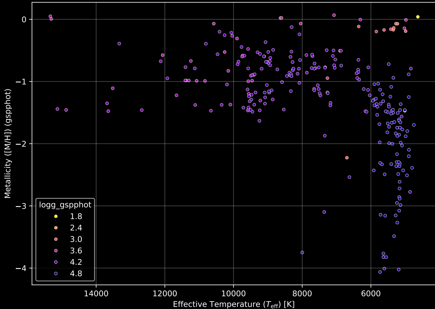
Gaia Cluster: [FSR_1315] Stellar Population Parameters (n= 269)
