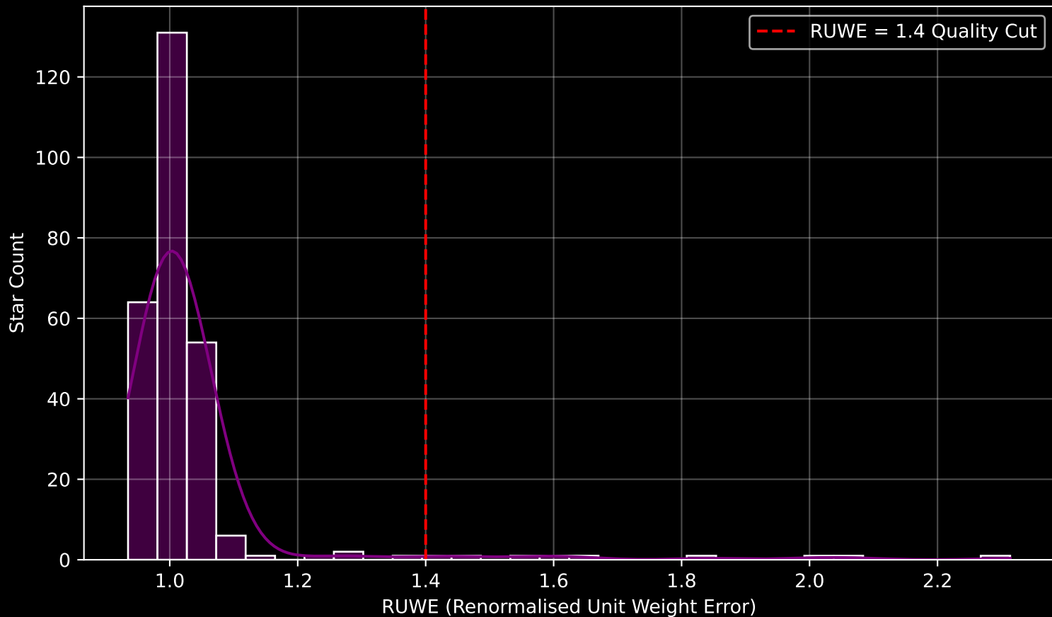
Gaia Cluster: [FSR_1315] RUWE Distribution (n= 269)
