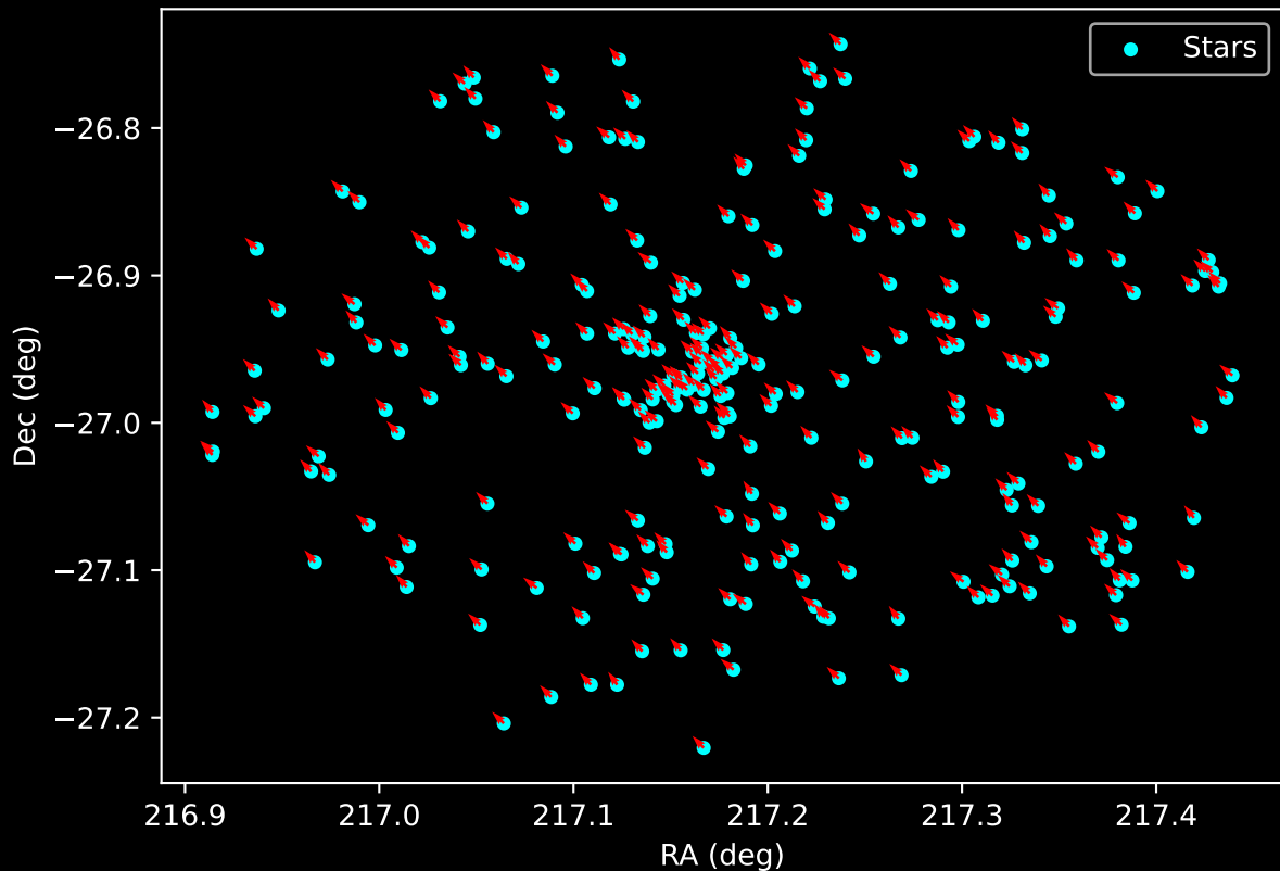
Gaia Cluster: [FSR_1315] Proper Motion Vectors for Gaia Star Field (n= 269)
