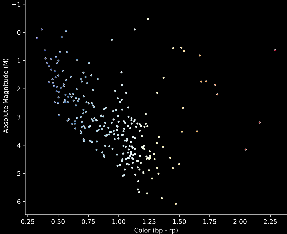
Gaia Cluster: [FSR_1315] Stars (n= 269) Hertzsprung-Russel Diagram
