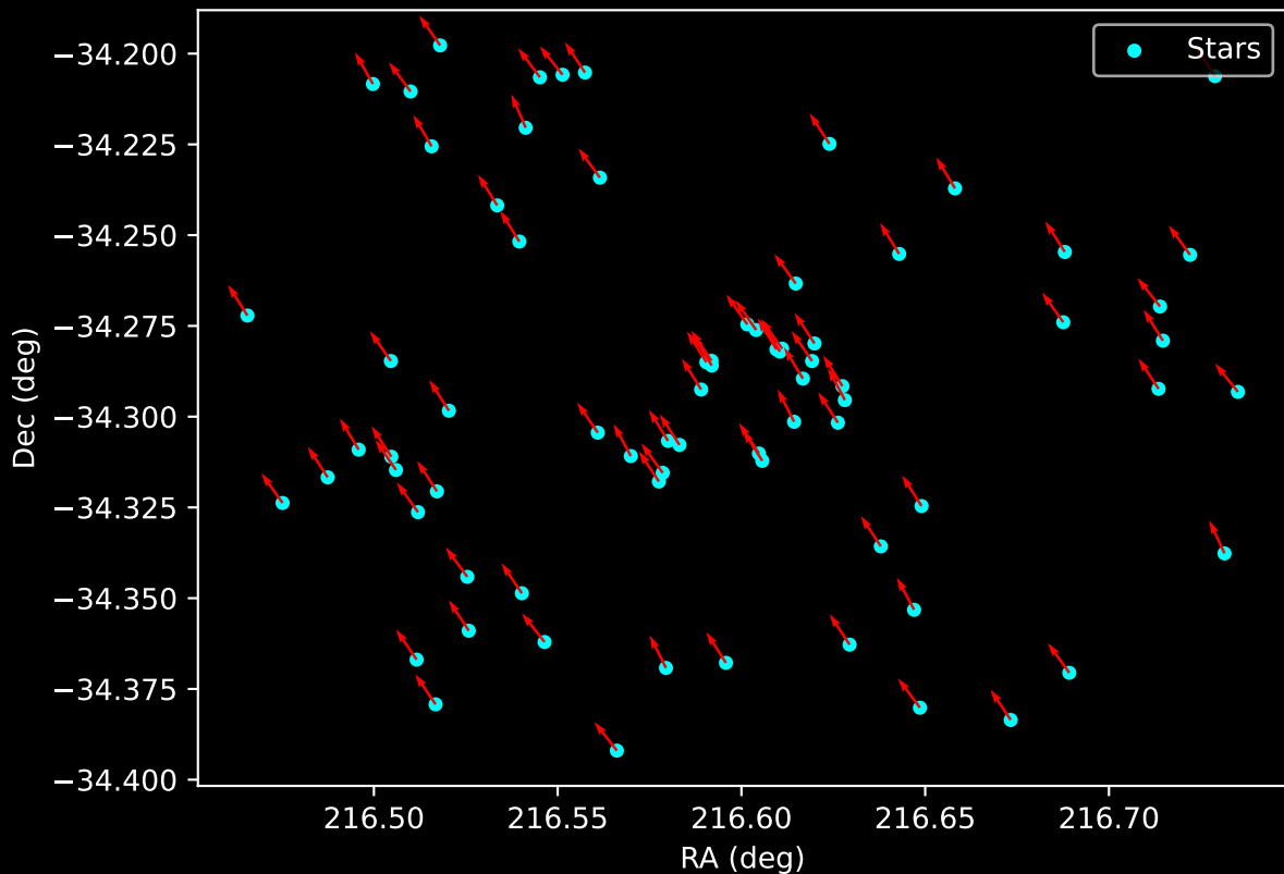
Gaia Cluster: [FSR_1352] Proper Motion Vectors for Gaia Star Field (n= 74)
