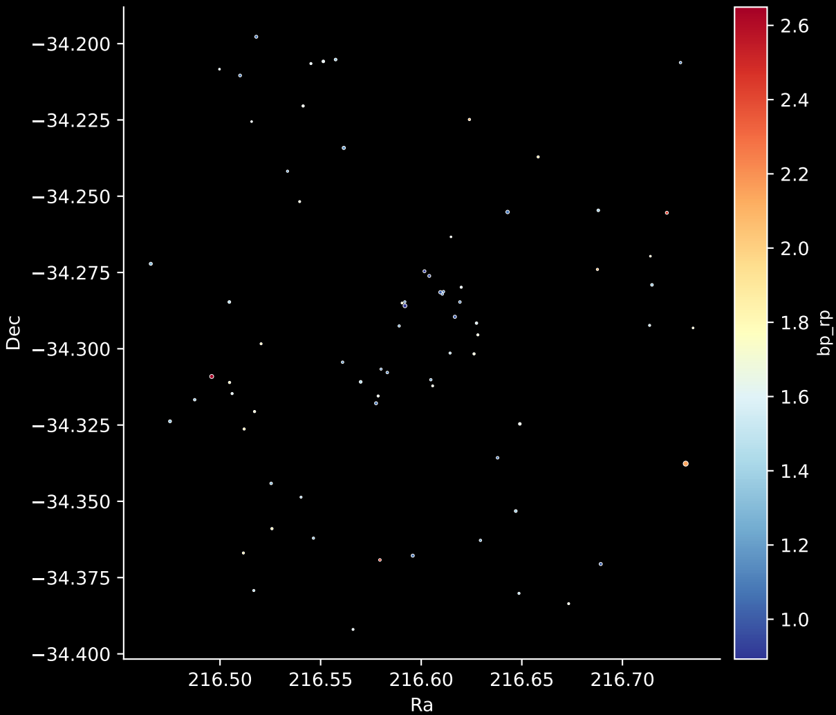
Gaia Cluster: [FSR_1352] Stars: 74
