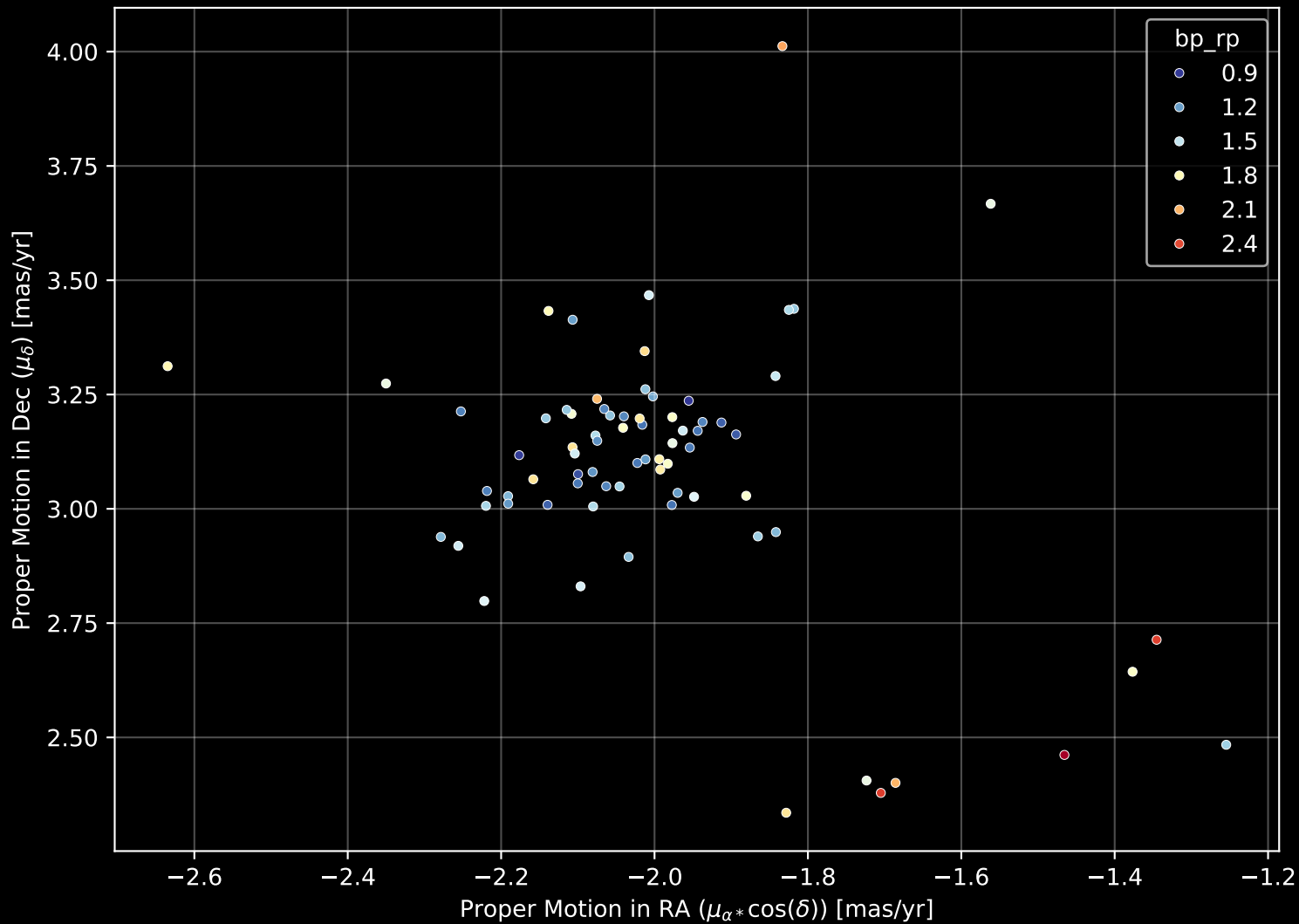
Gaia Cluster: [FSR_1352] Proper Motion Diagram (n= 74)
