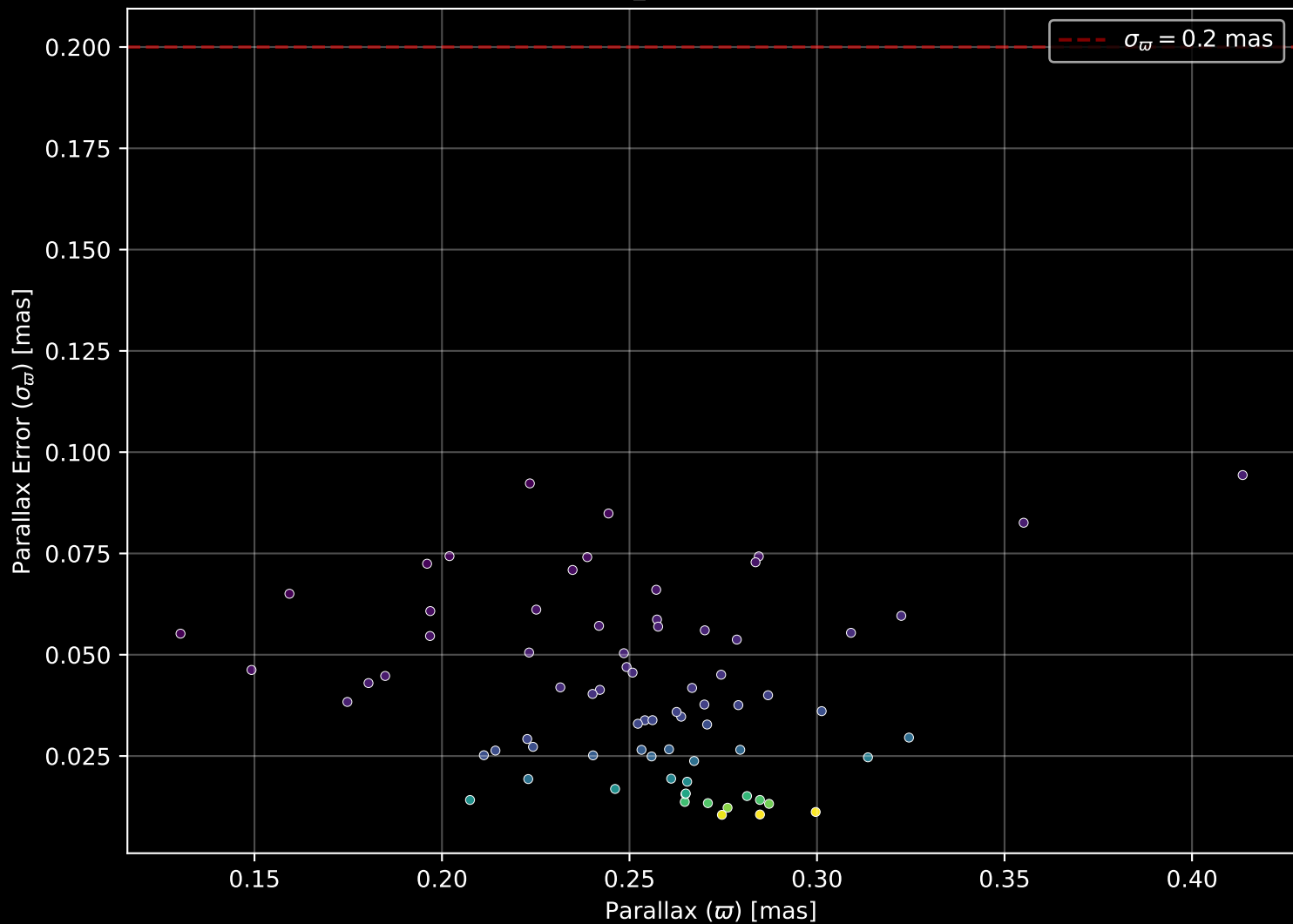
Gaia Cluster: [FSR_1352] Parallax Quality (n= 74)
