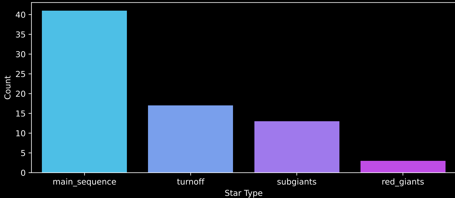
Gaia Cluster: [FSR_1352] Count plot of Star Type
