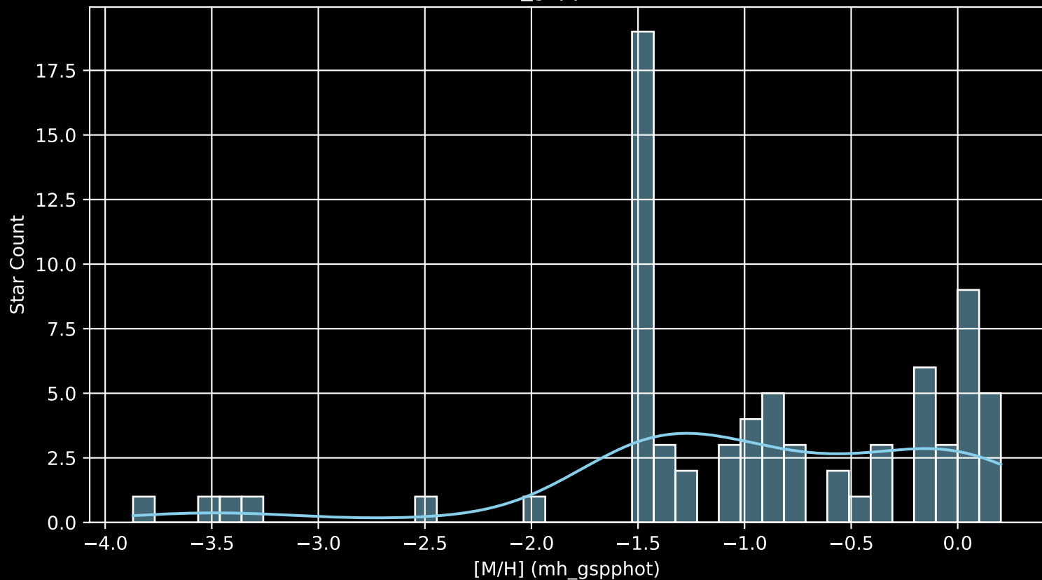
Gaia Cluster: [FSR_1352 [M/H] (mh_gspphot) (n= 74)
