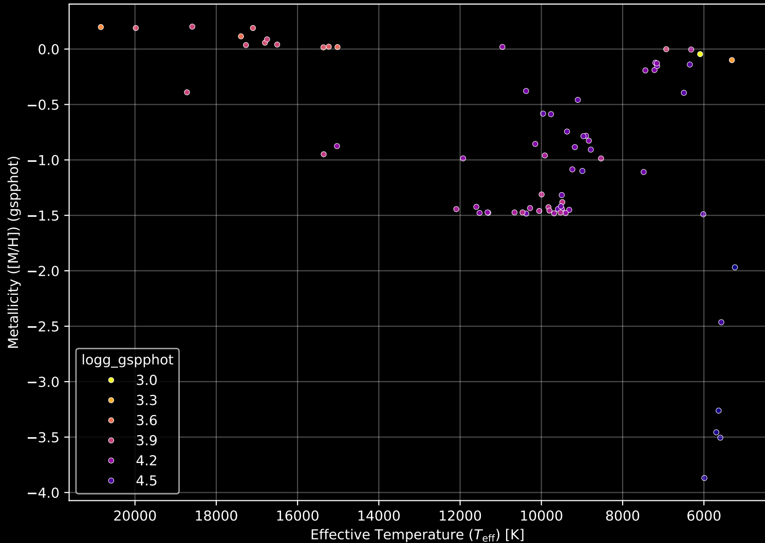
Gaia Cluster: [FSR_1352] Stellar Population Parameters (n= 74)
