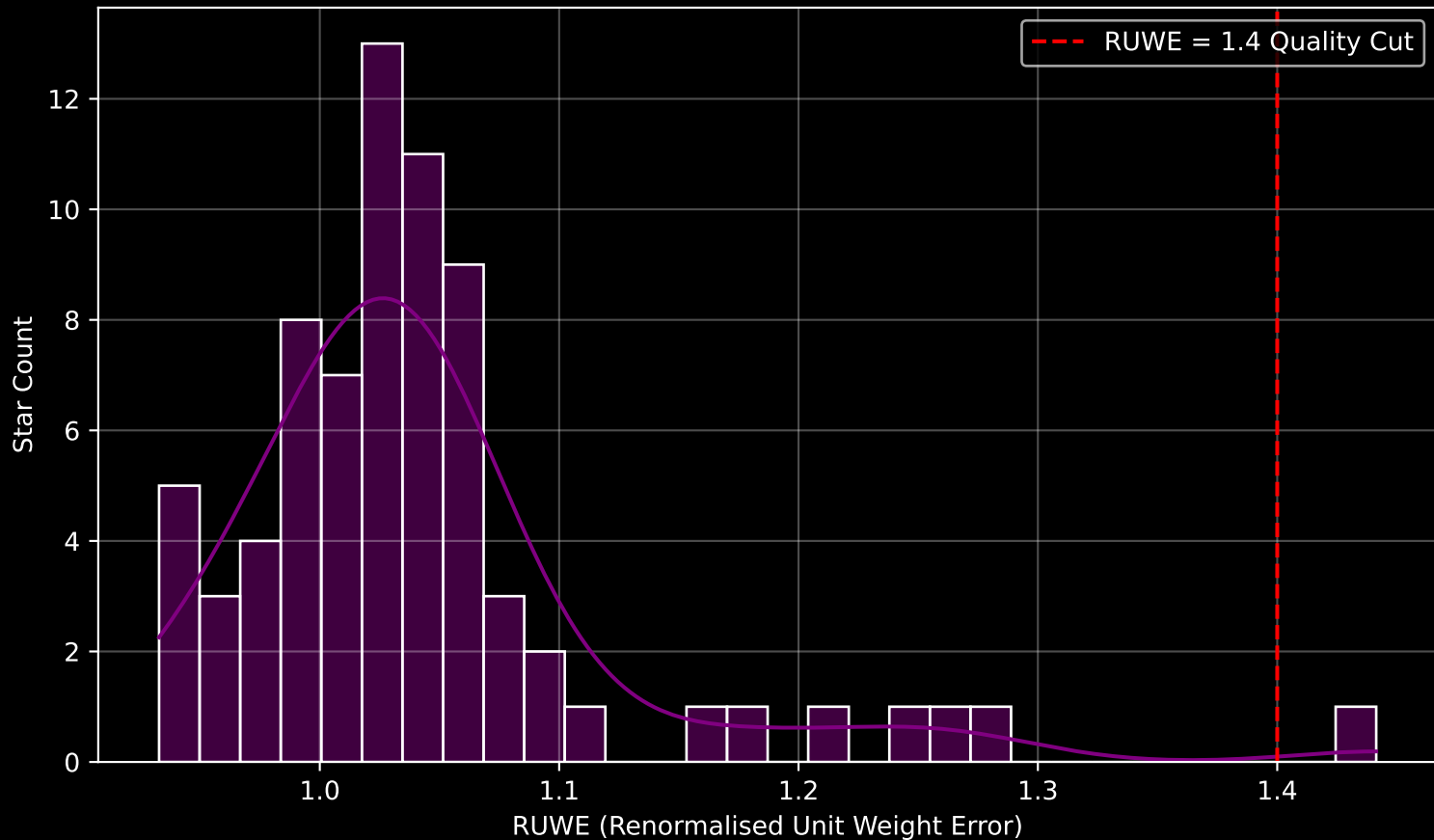
Gaia Cluster: [FSR_1352] RUWE Distribution (n= 73)
