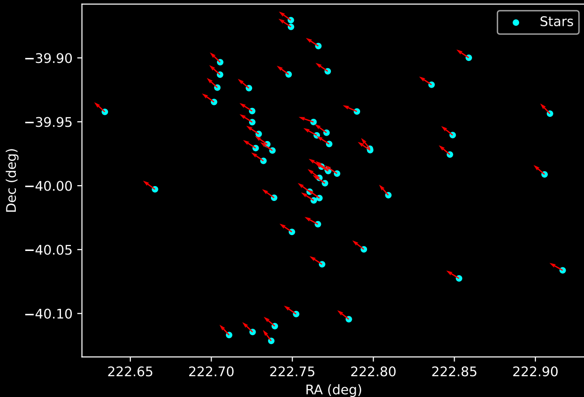
Gaia Cluster: [FSR_1380] Proper Motion Vectors for Gaia Star Field (n= 55)
