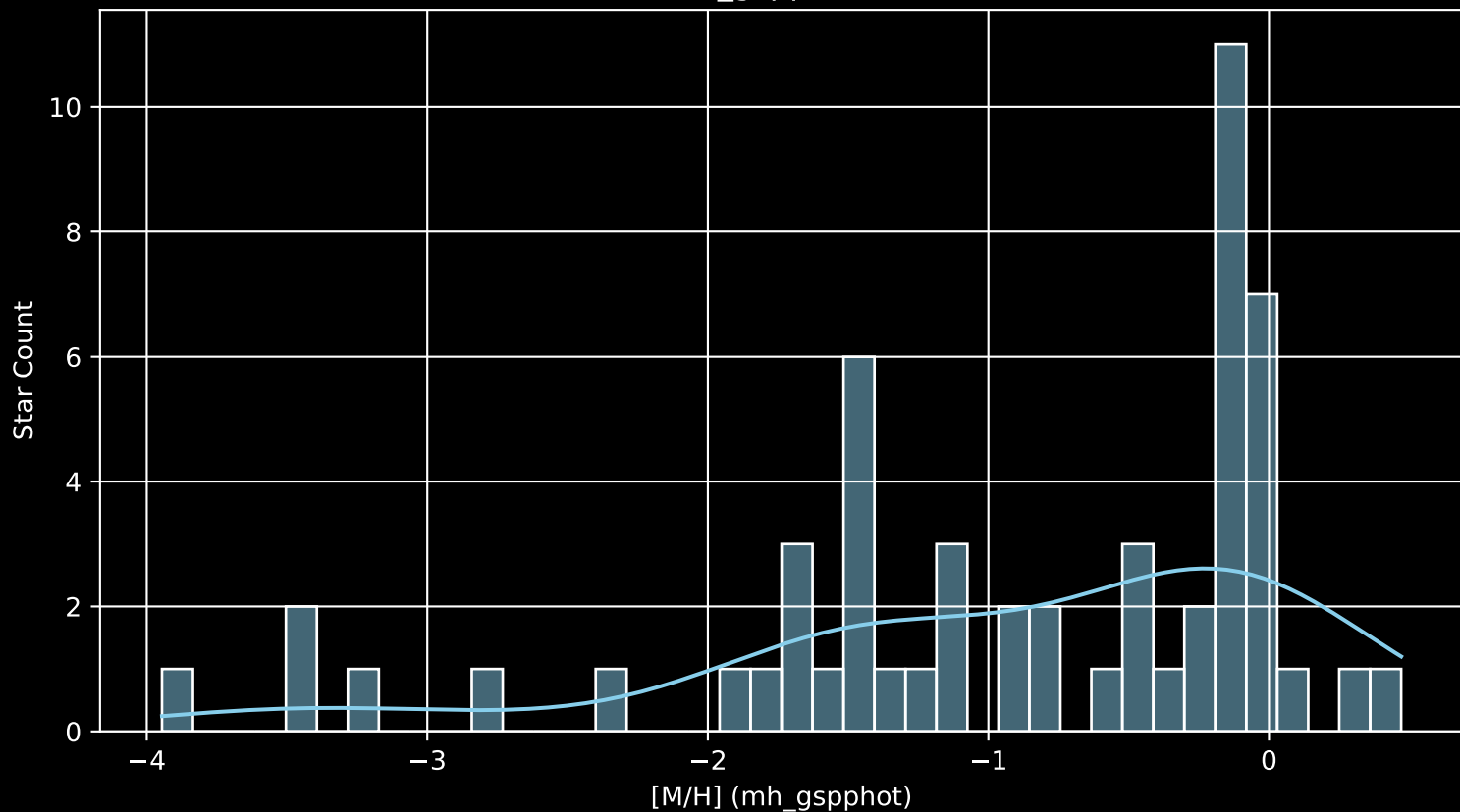
Gaia Cluster: [FSR_1380 [M/H] (mh_gspphot) (n= 55)
