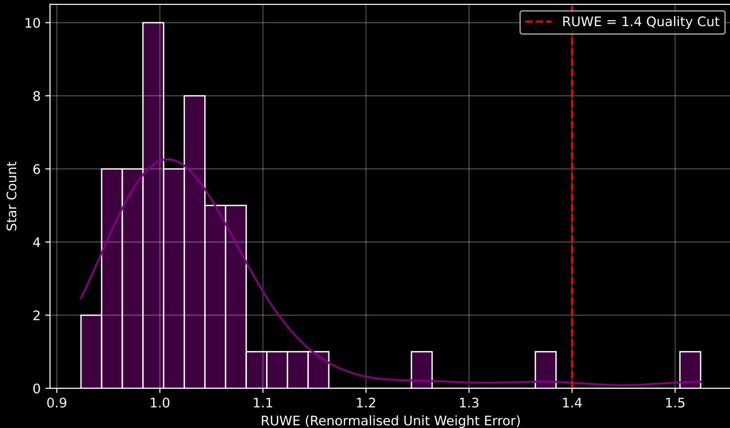
Gaia Cluster: [FSR_1380] RUWE Distribution (n= 55)
