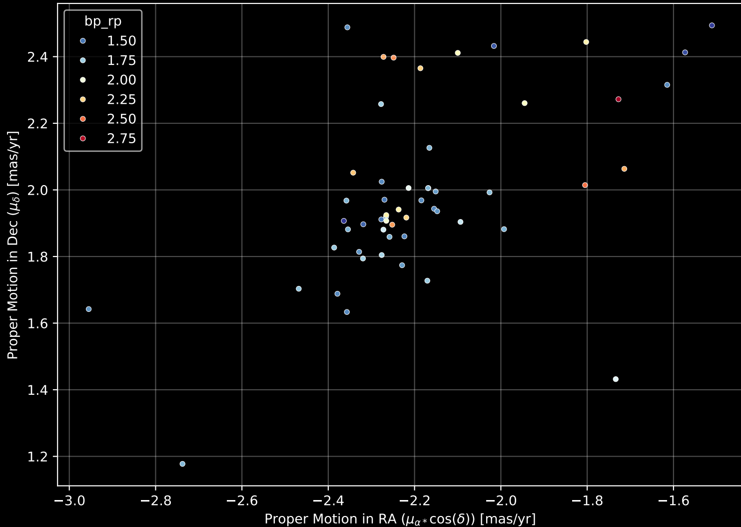
Gaia Cluster: [FSR_1380] Proper Motion Diagram (n= 55)
