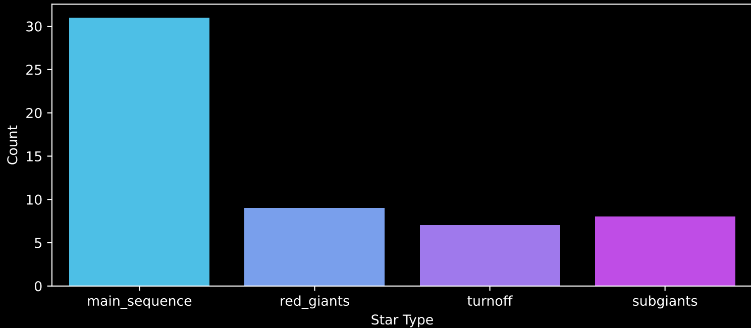
Gaia Cluster: [FSR_1380] Count plot of Star Type
