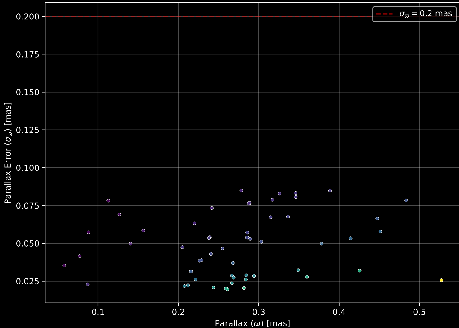
Gaia Cluster: [FSR_1380] Parallax Quality (n= 55)
