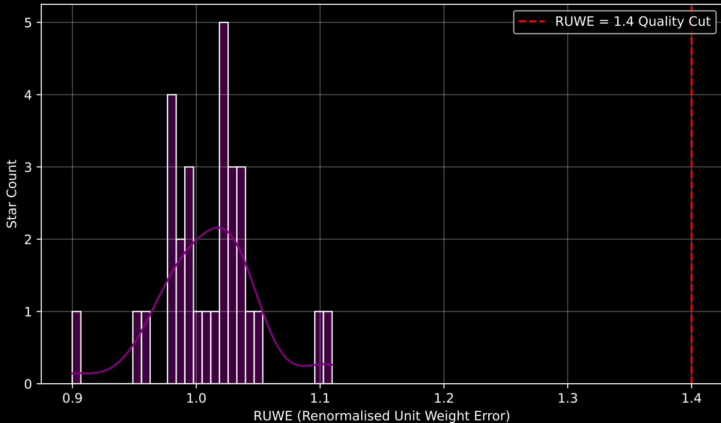
Gaia Cluster: [FSR_1399] RUWE Distribution (n= 30)
