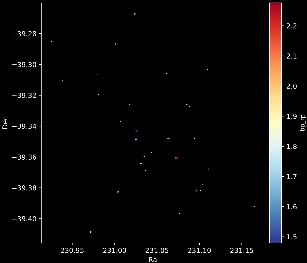
Gaia Cluster: [FSR_1399] Stars: 30
