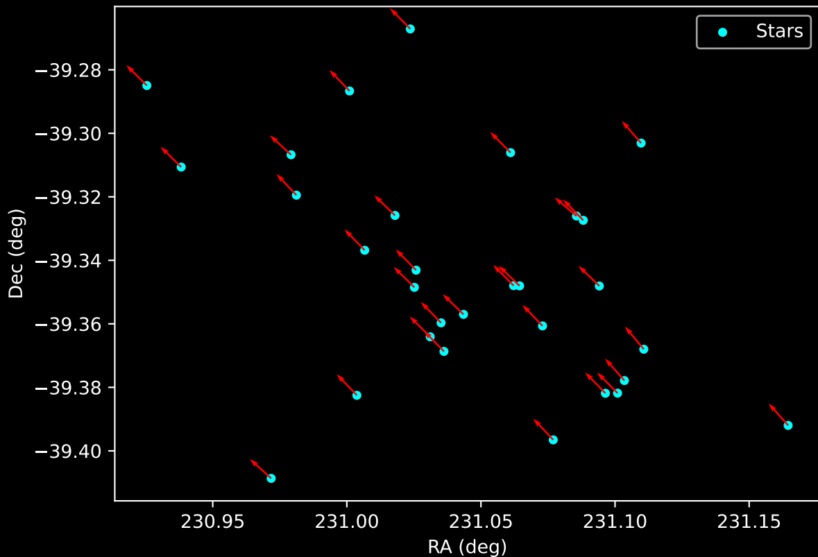
Gaia Cluster: [FSR_1399] Proper Motion Vectors for Gaia Star Field (n= 30)
