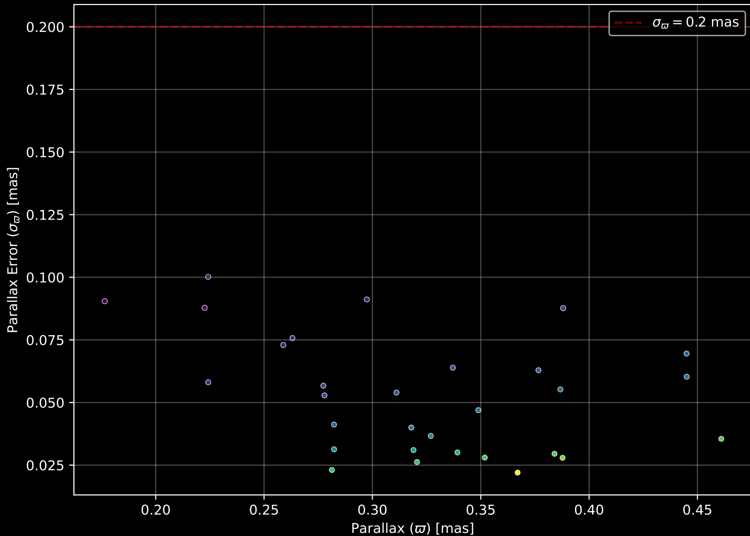
Gaia Cluster: [FSR_1399] Parallax Quality (n= 30)
