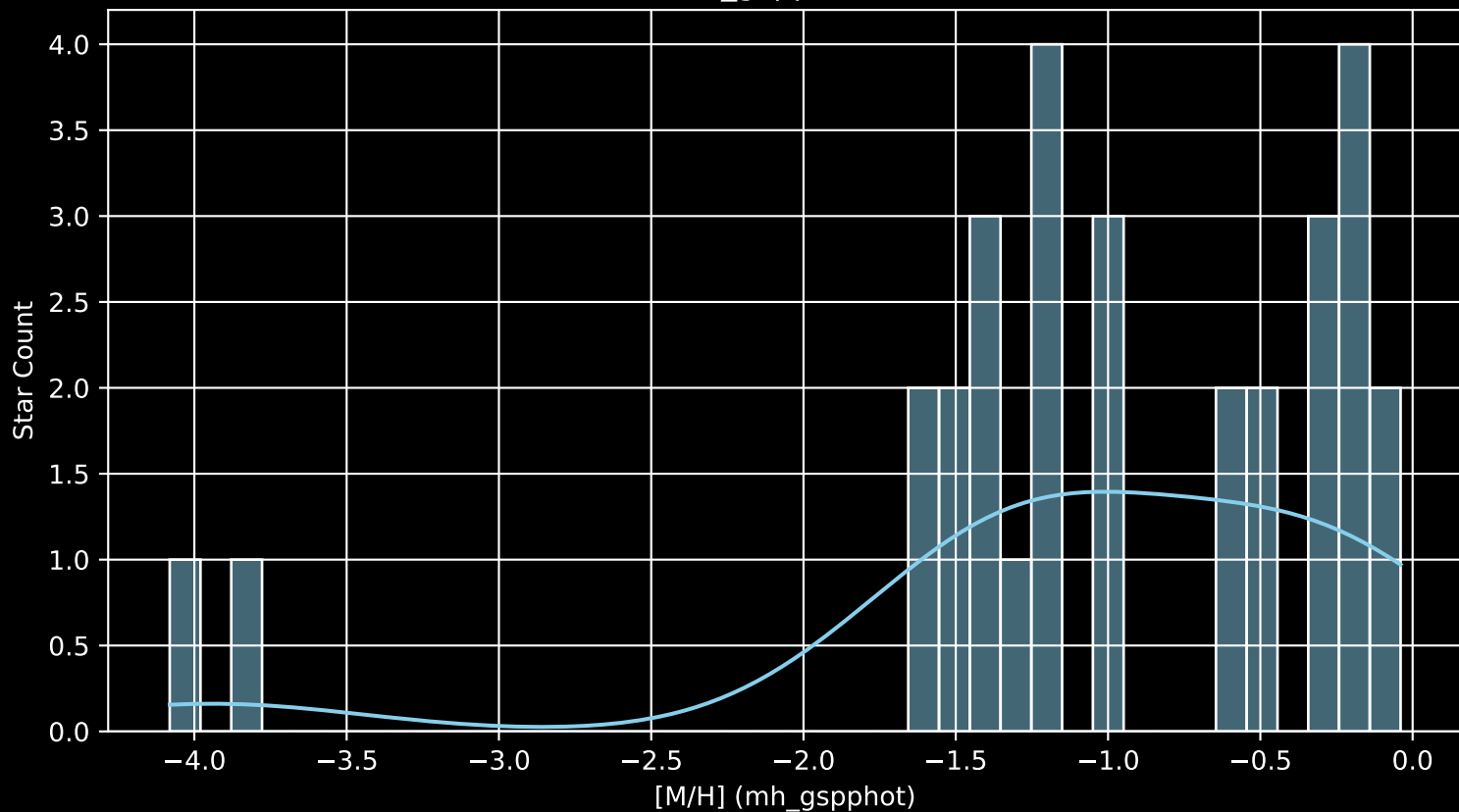
Gaia Cluster: [FSR_1399 [M/H] (mh_gspphot) (n= 30)
