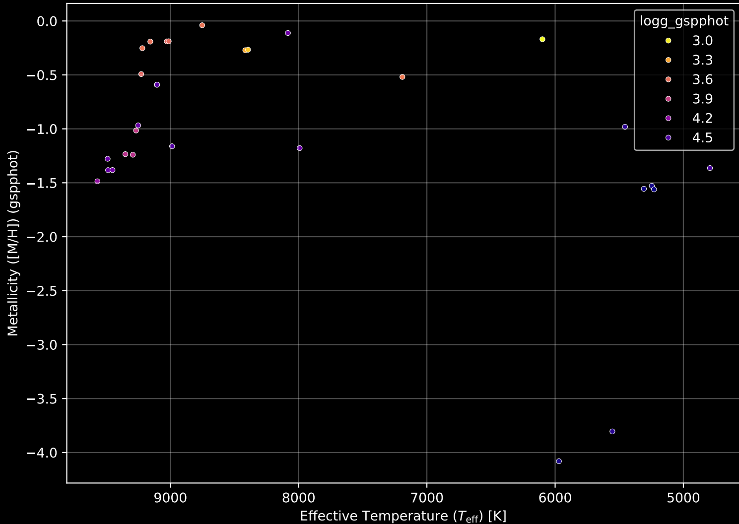
Gaia Cluster: [FSR_1399] Stellar Population Parameters (n= 30)
