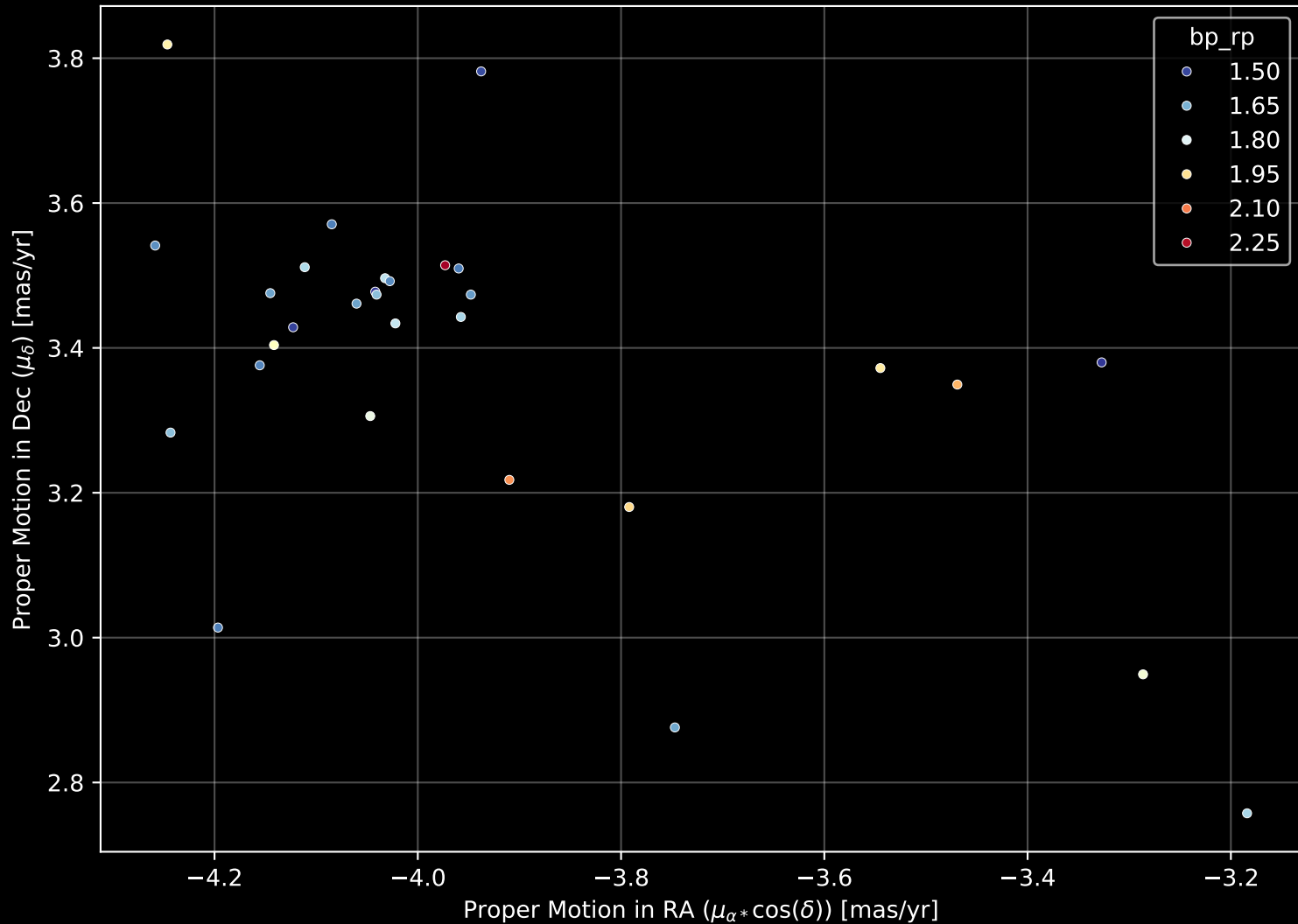
Gaia Cluster: [FSR_1399] Proper Motion Diagram (n= 30)
