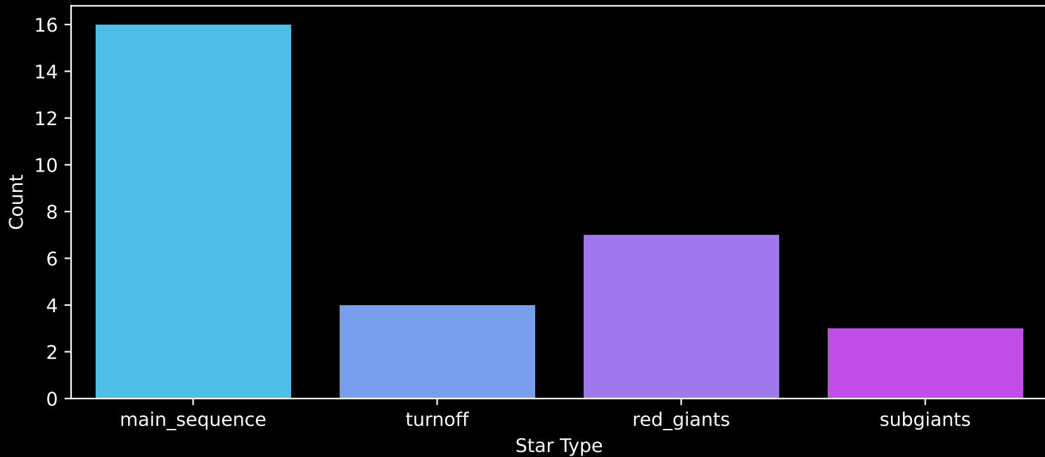
Gaia Cluster: [FSR_1399] Count plot of Star Type
