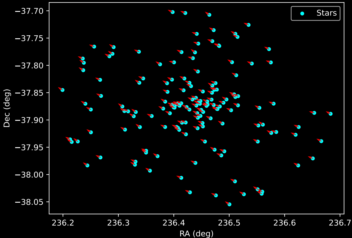
Gaia Cluster: [FSR_1402] Proper Motion Vectors for Gaia Star Field (n= 149)
