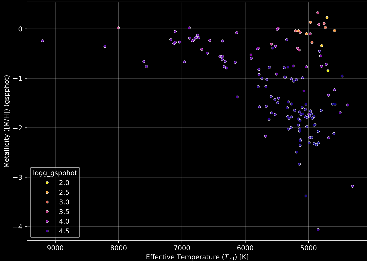
Gaia Cluster: [FSR_1402] Stellar Population Parameters (n= 149)
