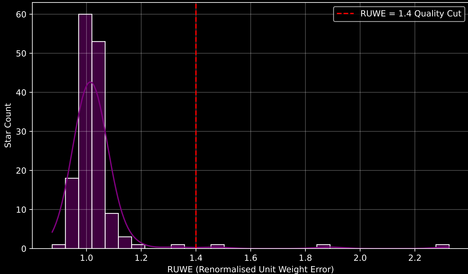
Gaia Cluster: [FSR_1402] RUWE Distribution (n= 149)
