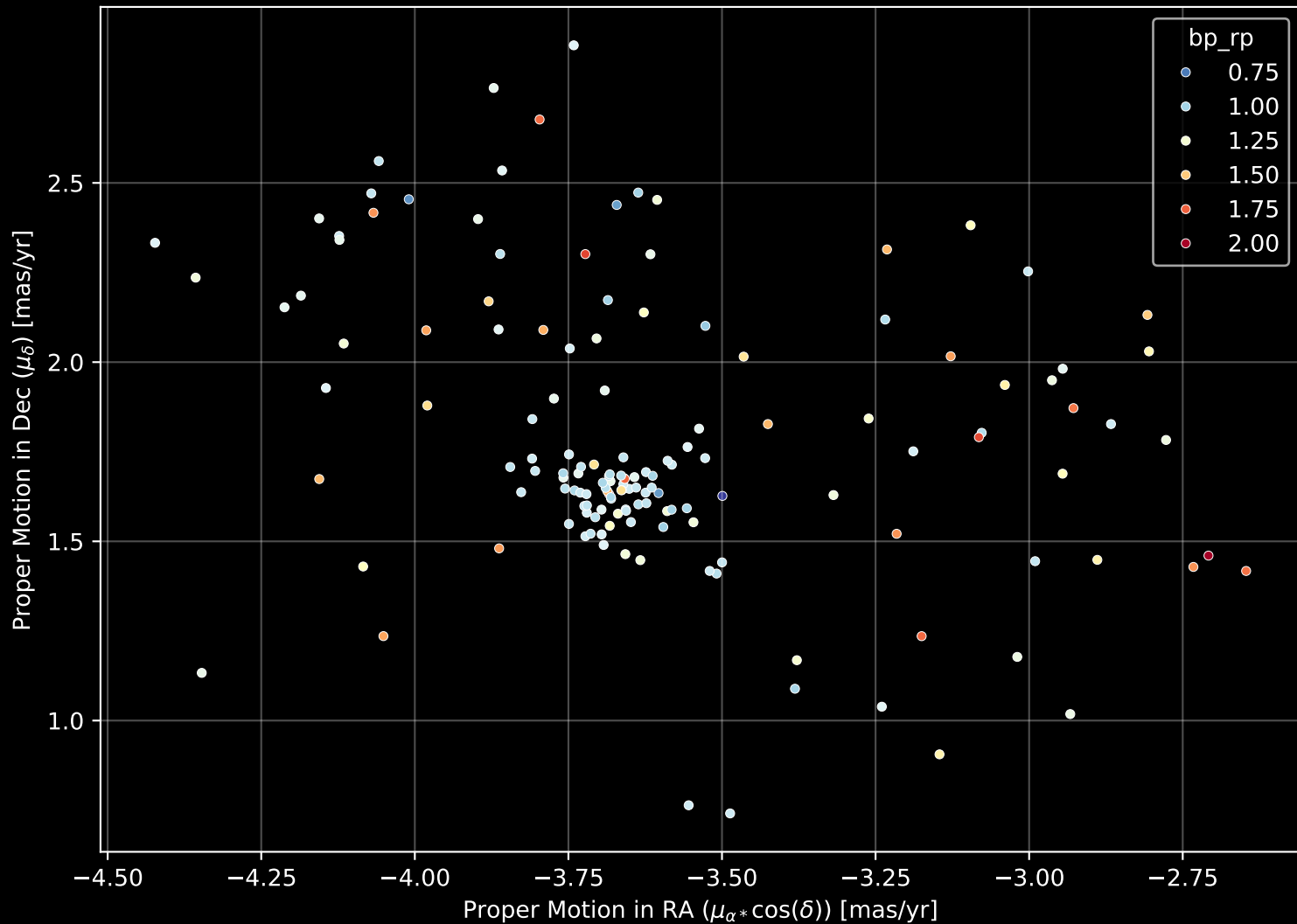
Gaia Cluster: [FSR_1402] Proper Motion Diagram (n= 149)
