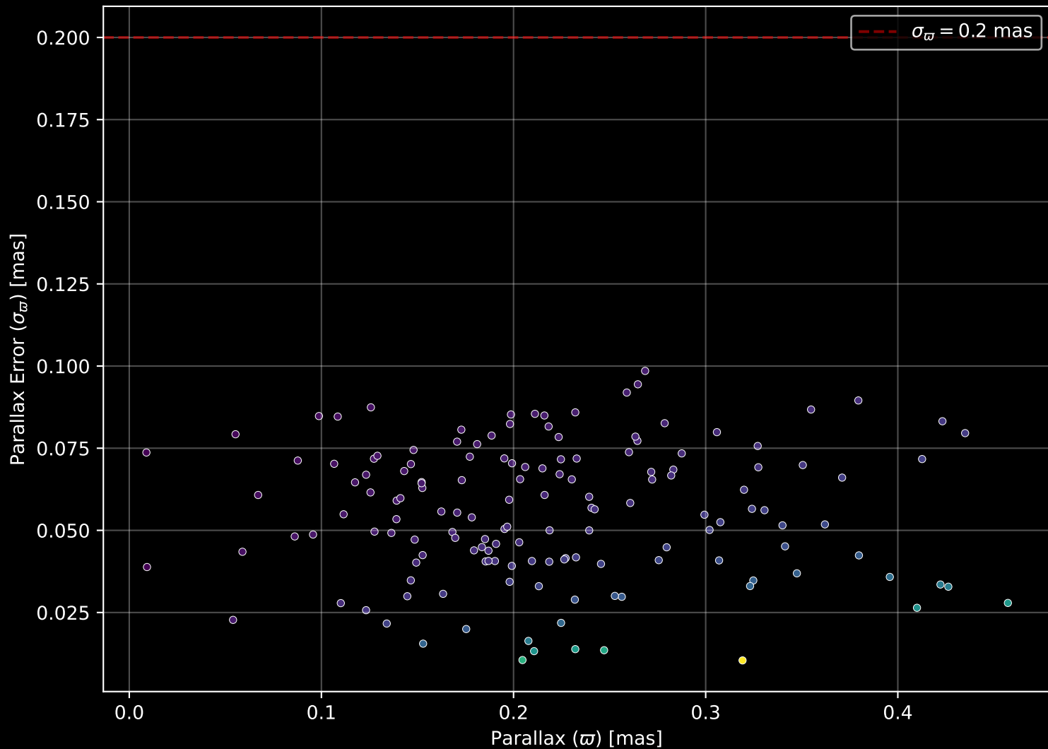
Gaia Cluster: [FSR_1402] Parallax Quality (n= 149)
