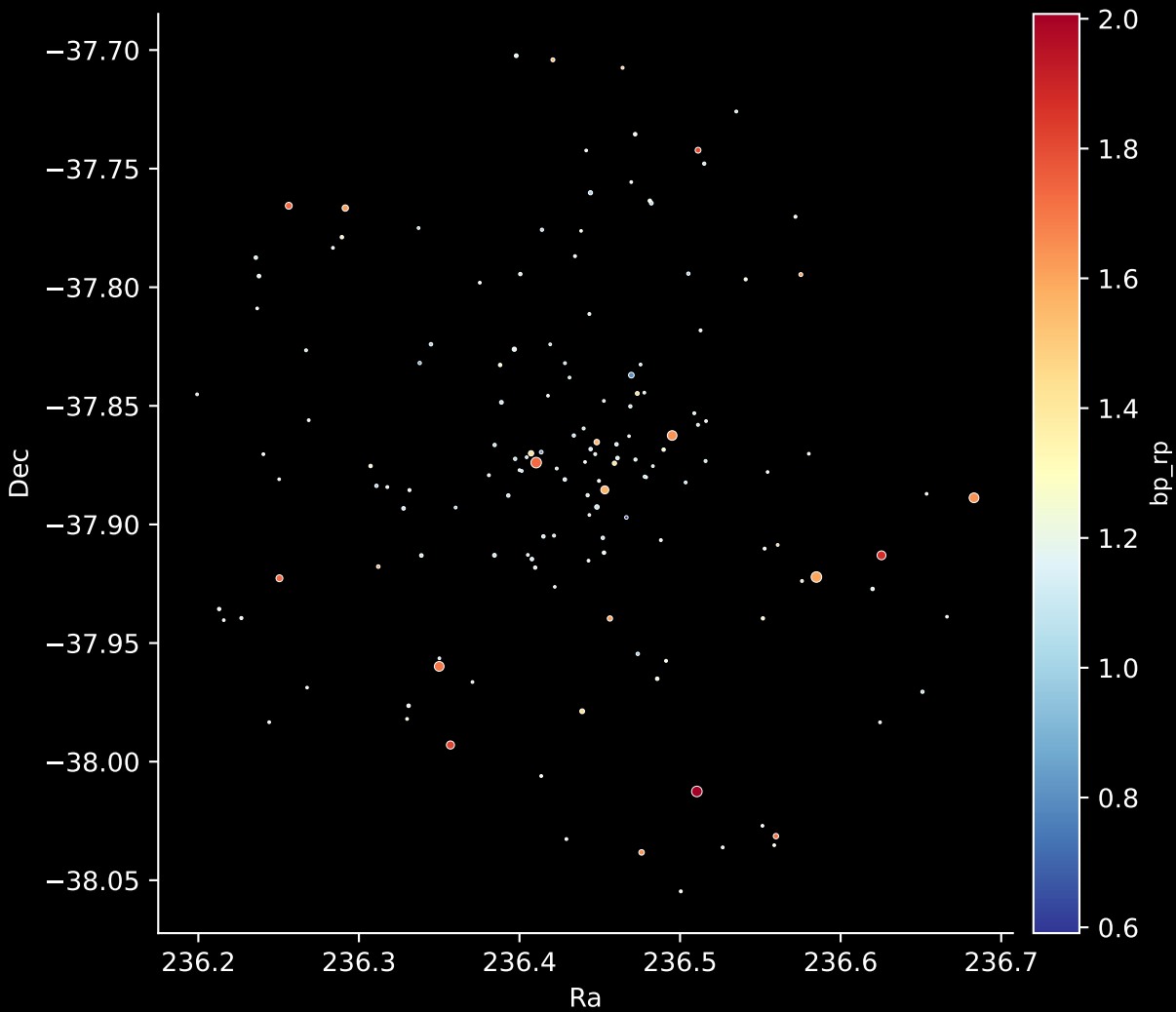
Gaia Cluster: [FSR_1402] Stars: 149
