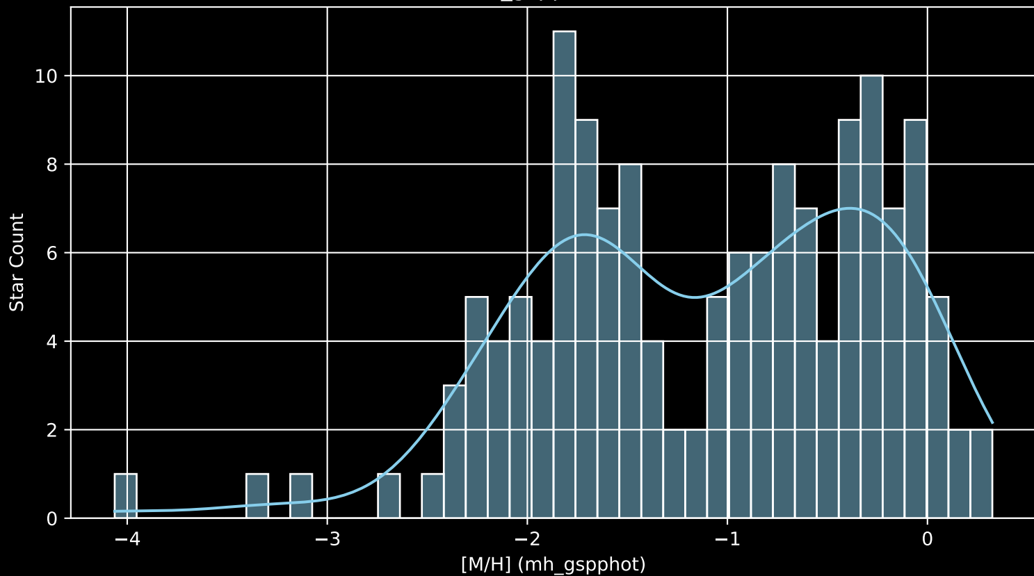
Gaia Cluster: [FSR_1402 [M/H] (mh_gspphot) (n= 149)
