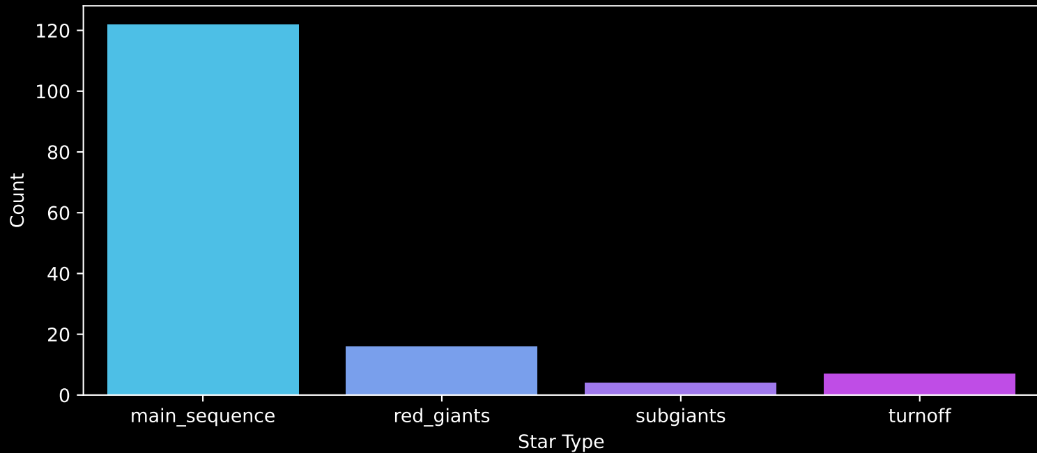
Gaia Cluster: [FSR_1402] Count plot of Star Type
