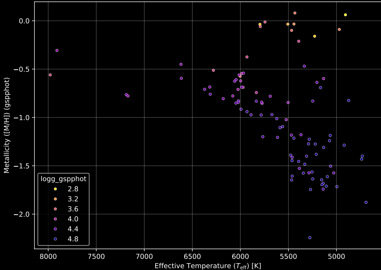
Gaia Cluster: [FSR_1407] Stellar Population Parameters (n= 98)
