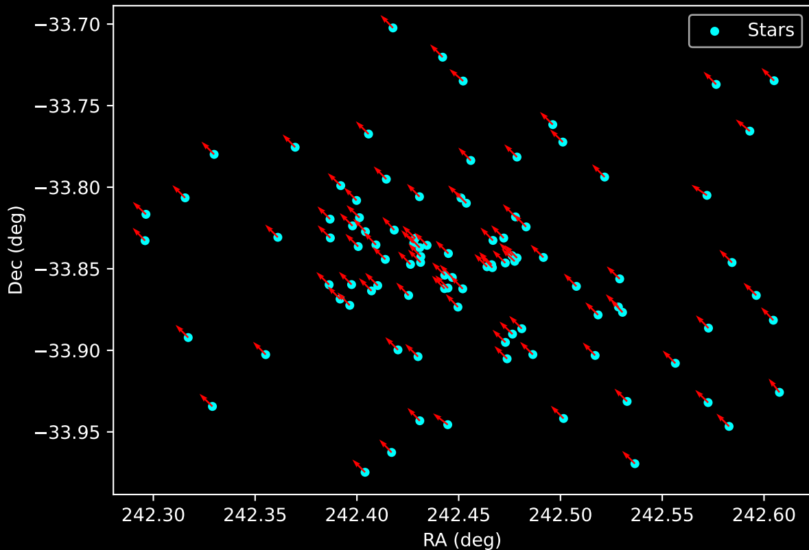
Gaia Cluster: [FSR_1407] Proper Motion Vectors for Gaia Star Field (n= 98)
