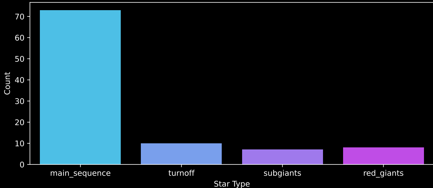
Gaia Cluster: [FSR_1407] Count plot of Star Type
