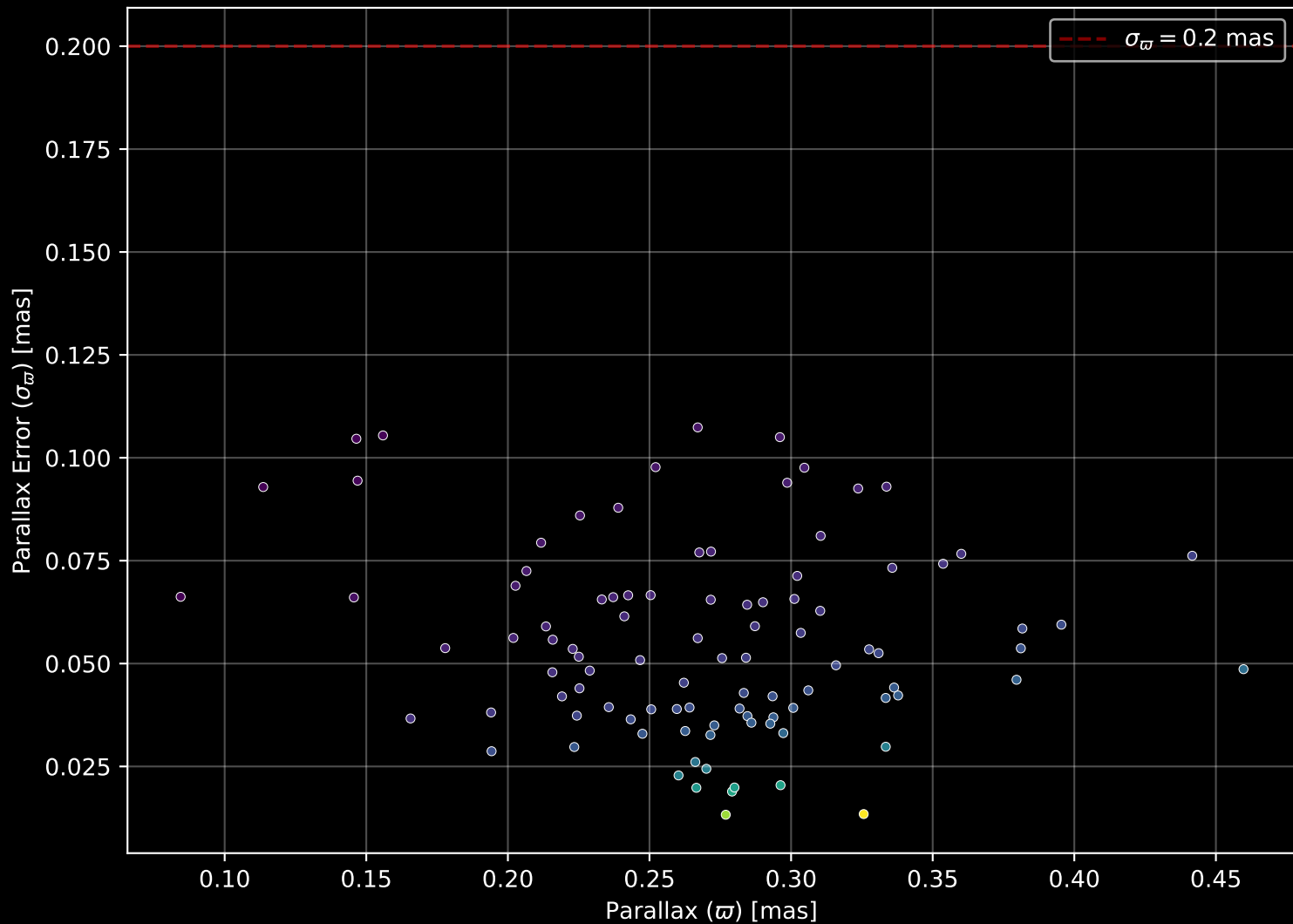
Gaia Cluster: [FSR_1407] Parallax Quality (n= 98)
