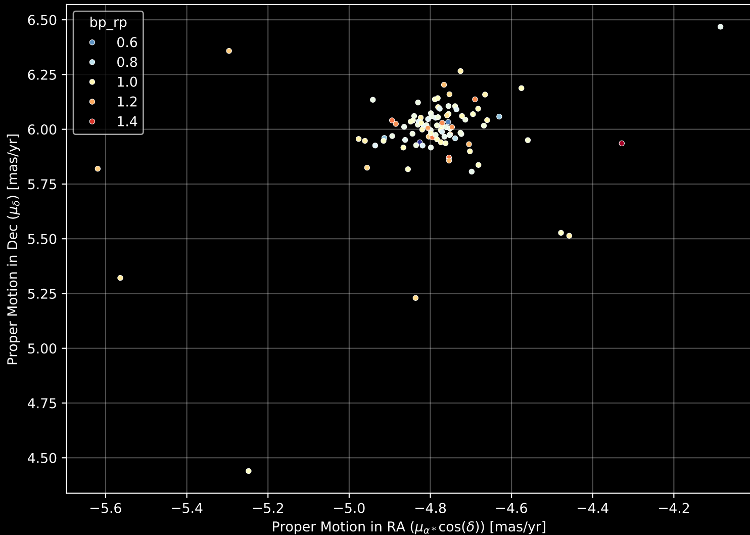
Gaia Cluster: [FSR_1407] Proper Motion Diagram (n= 98)
