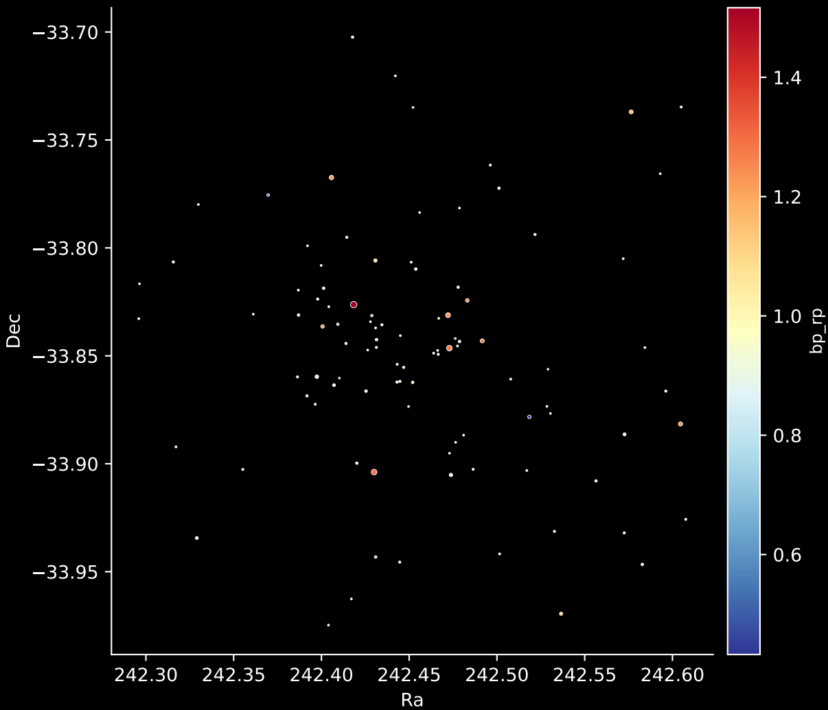
Gaia Cluster: [FSR_1407] Stars: 98
