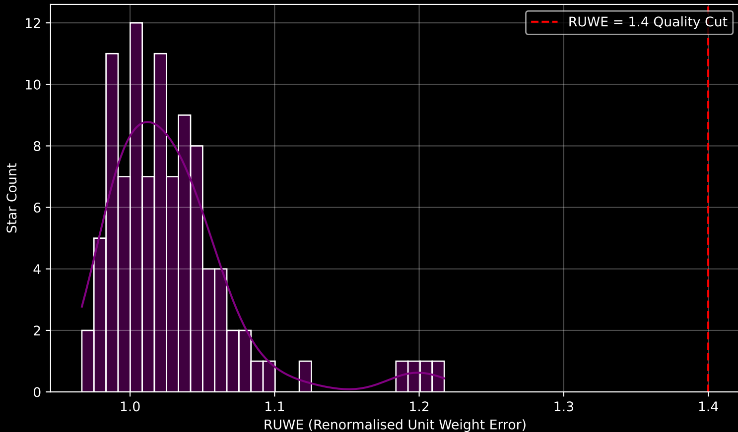
Gaia Cluster: [FSR_1407] RUWE Distribution (n= 98)
