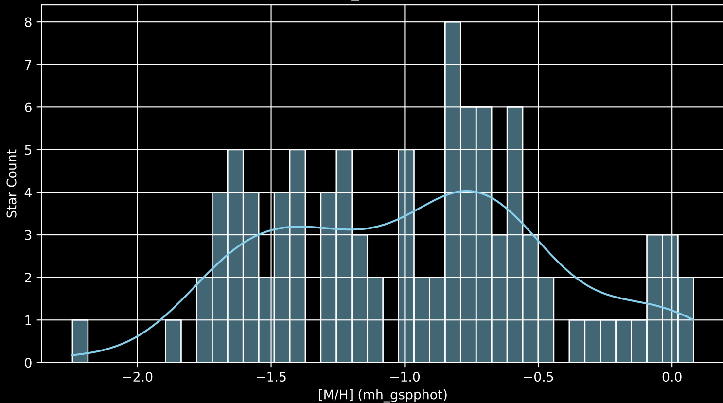
Gaia Cluster: [FSR_1407 [M/H] (mh_gspphot) (n= 98)
