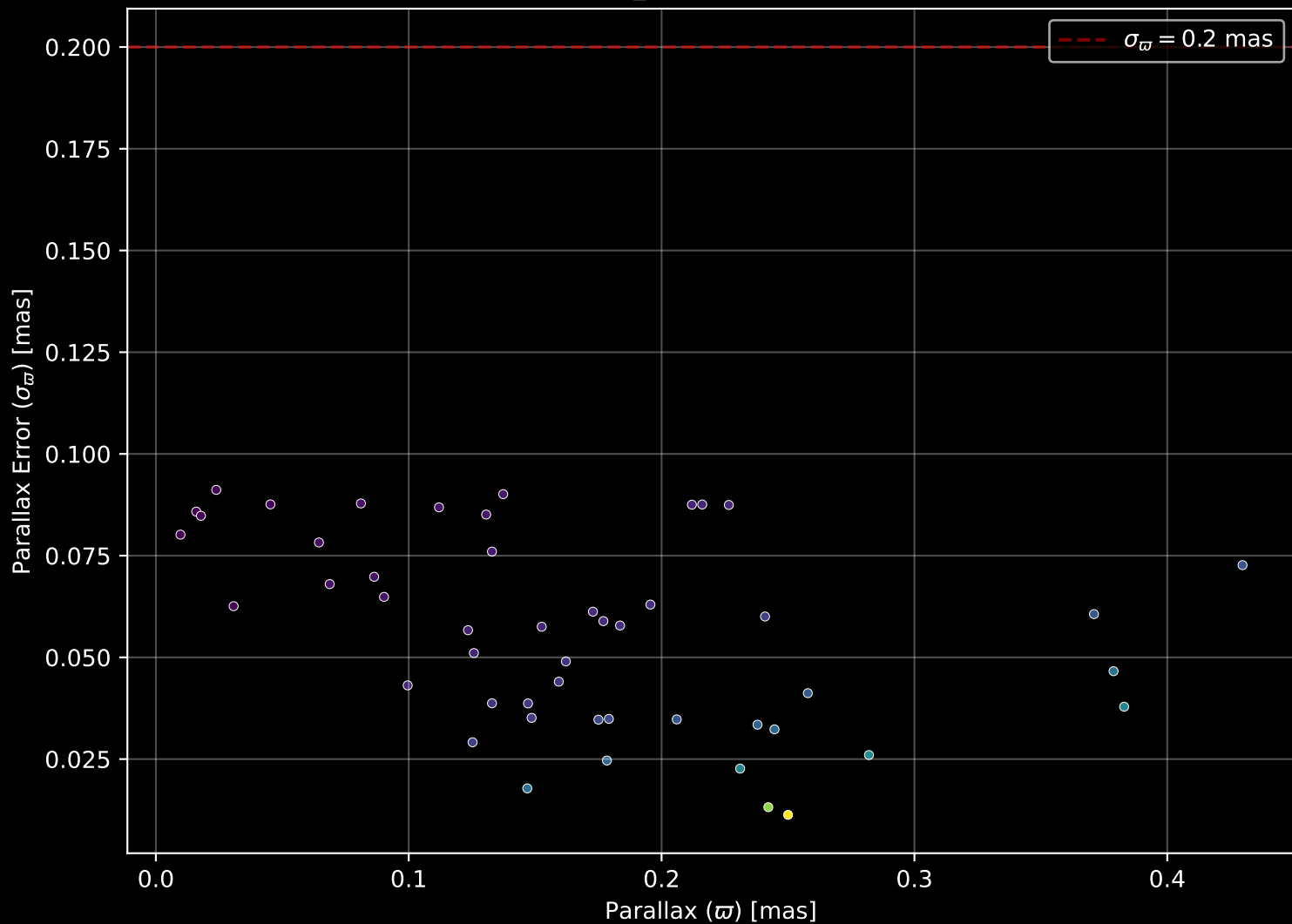
Gaia Cluster: [FSR_1509] Parallax Quality (n= 49)
