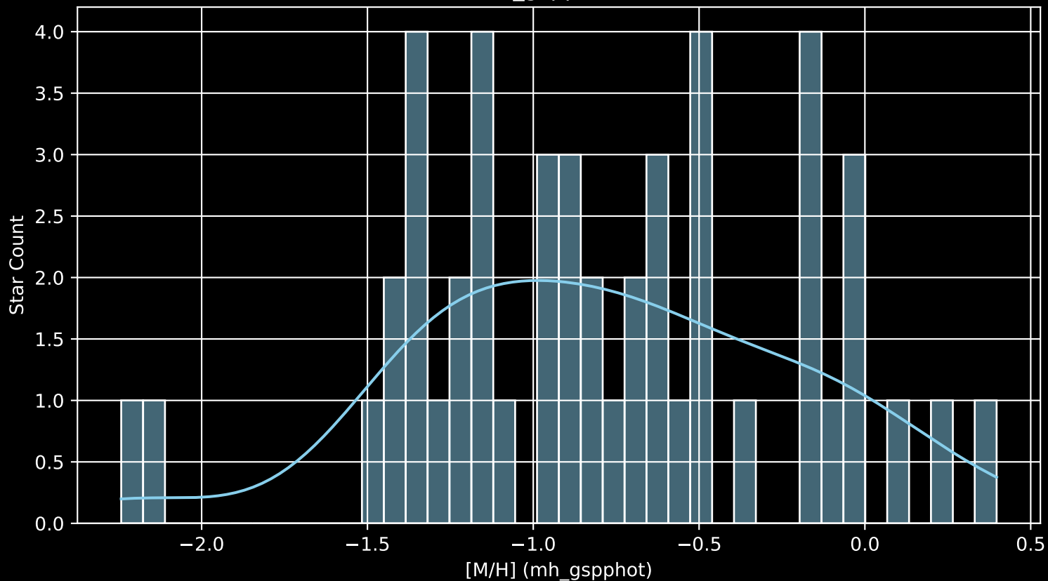
Gaia Cluster: [FSR_1509 [M/H] (mh_gspphot) (n= 48)
