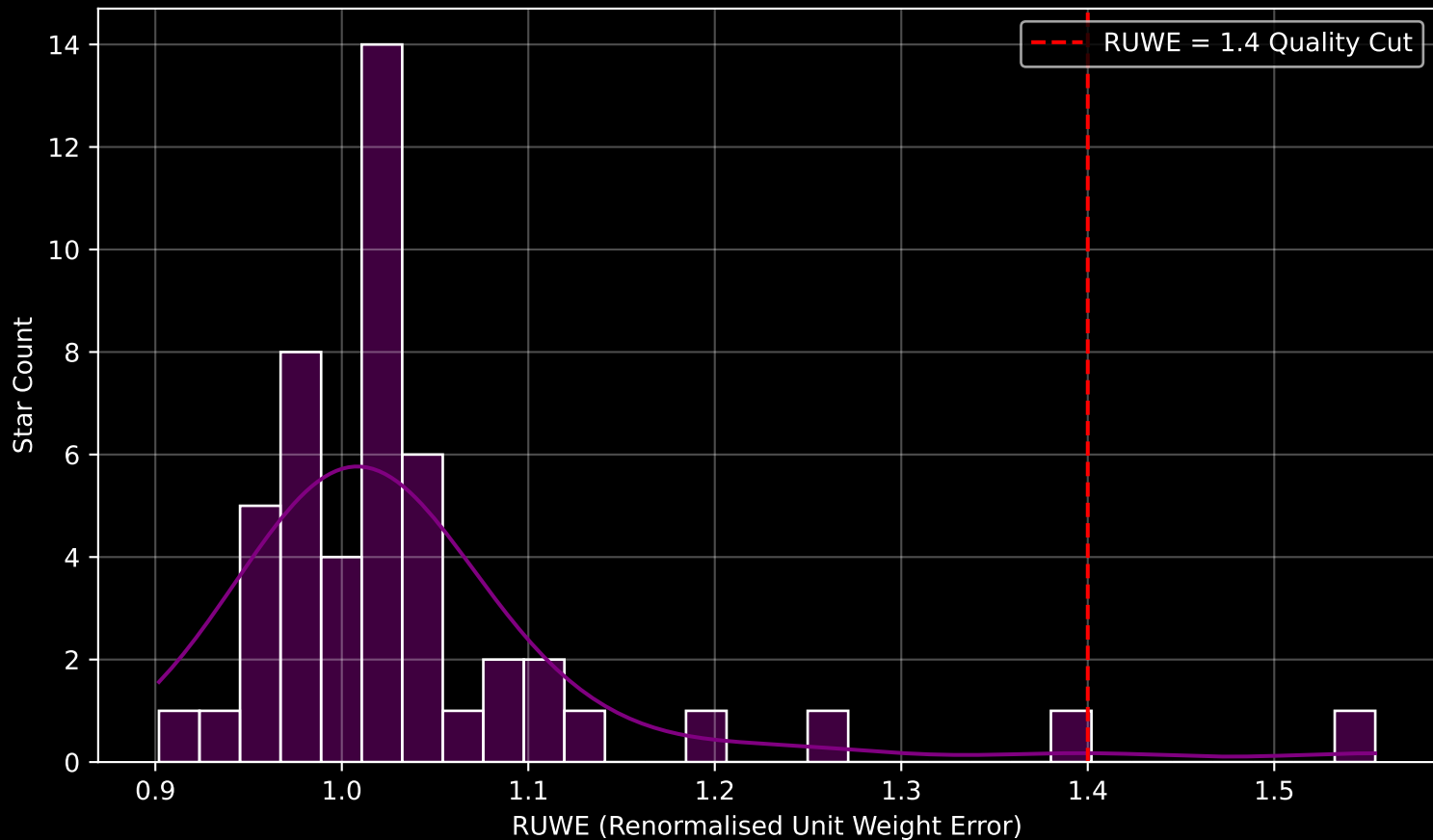
Gaia Cluster: [FSR_1509] RUWE Distribution (n = 49)
