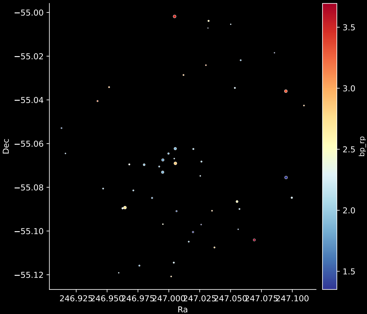
Gaia Cluster: [FSR_1509] Stars: 49
