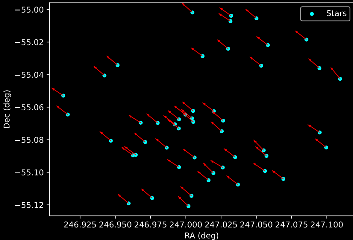
Gaia Cluster: [FSR_1509] Proper Motion Vectors for Gaia Star Field (n= 49)
