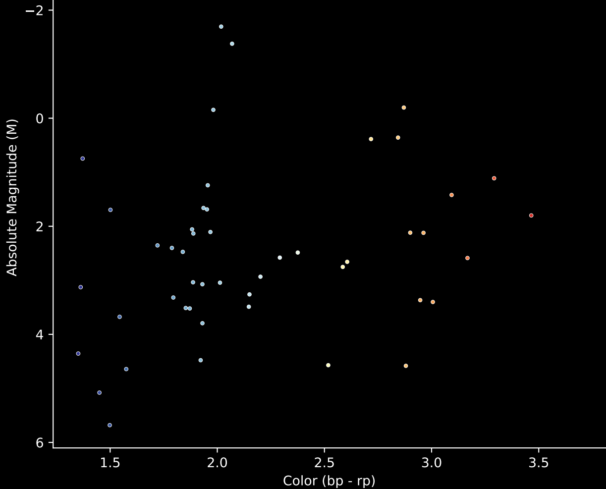
Gaia Cluster: [FSR_1509] Stars (n= 49) Hertzsprung-Russel Diagram
