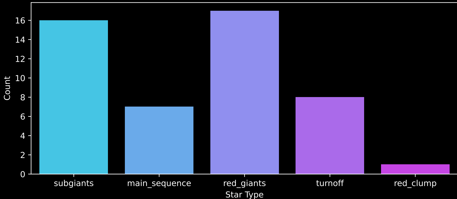
Gaia Cluster: [FSR_1509] Count plot of Star Type
