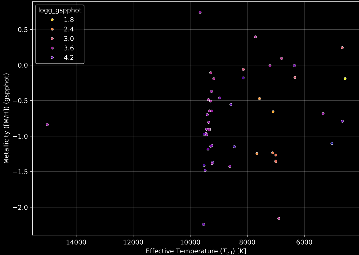
Gaia Cluster: [FSR_1509] Stellar Population Parameters (n= 49)
