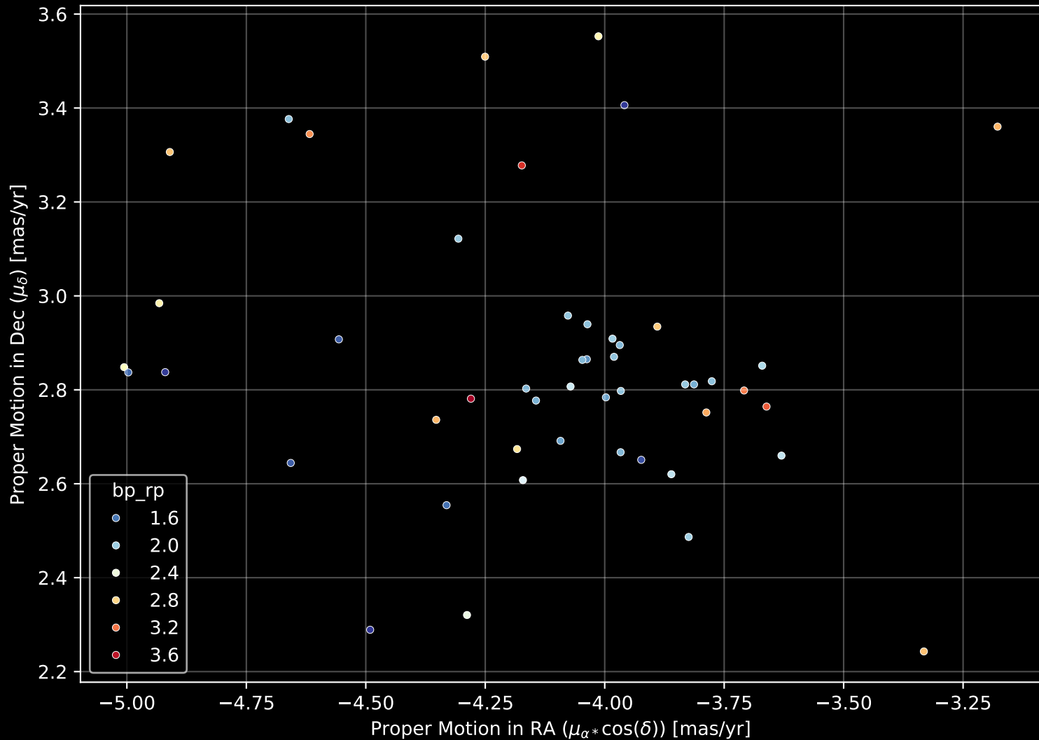
Gaia Cluster: [FSR_1509] Proper Motion Diagram (n= 49)
