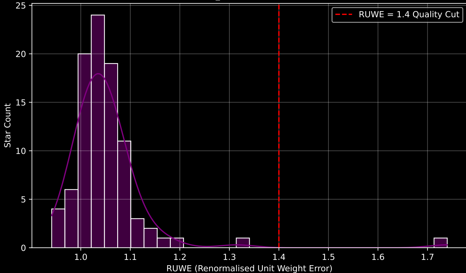
Gaia Cluster: [FSR_1521] RUWE Distribution (n= 93)
