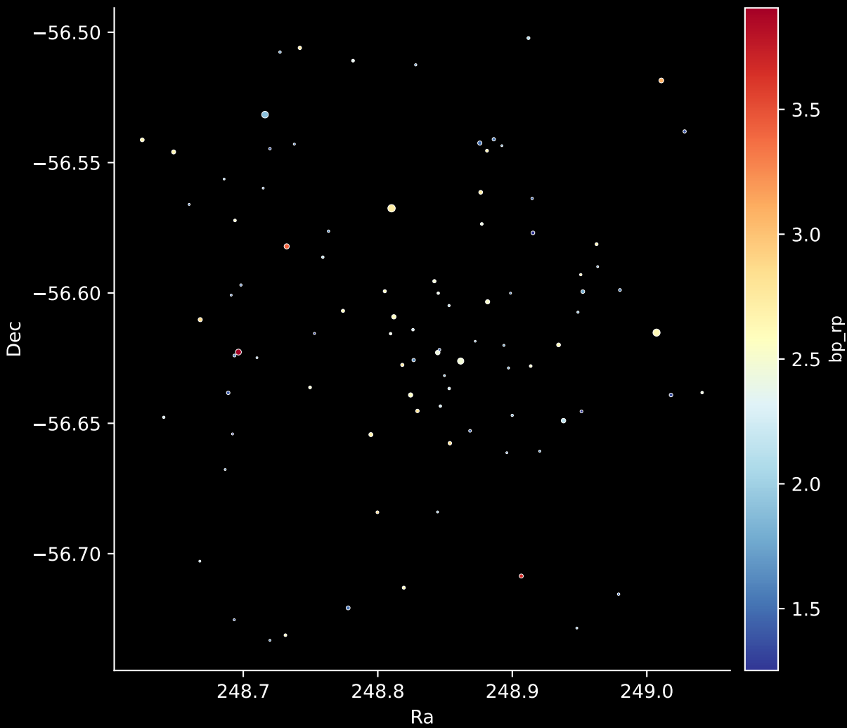
Gaia Cluster: [FSR_1521] Stars: 93
