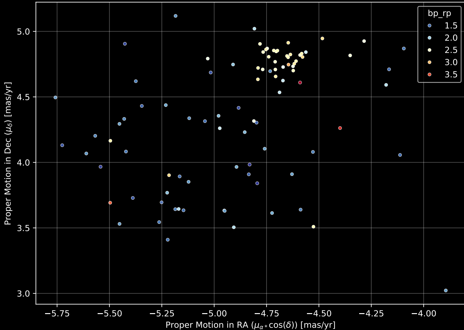
Gaia Cluster: [FSR_1521] Proper Motion Diagram (n= 93)
