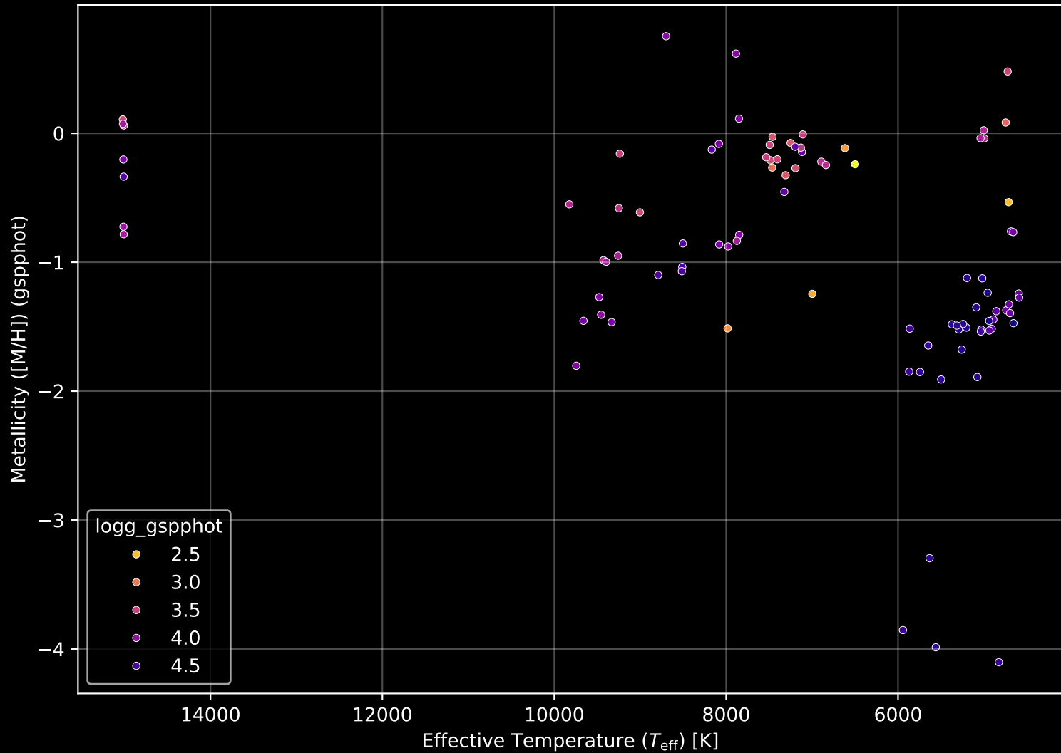
Gaia Cluster: [FSR_1521] Stellar Population Parameters (n= 93)
