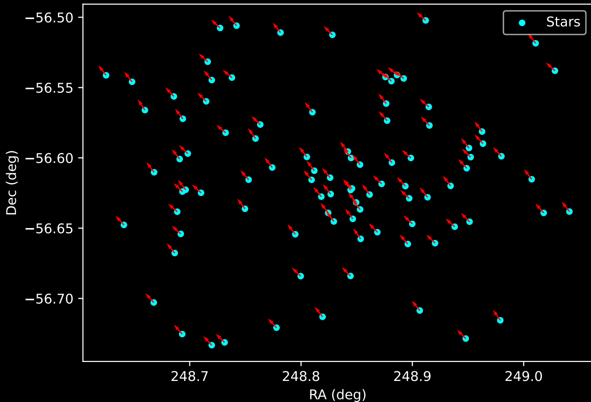
Gaia Cluster: [FSR_1521] Proper Motion Vectors for Gaia Star Field (n= 93)
