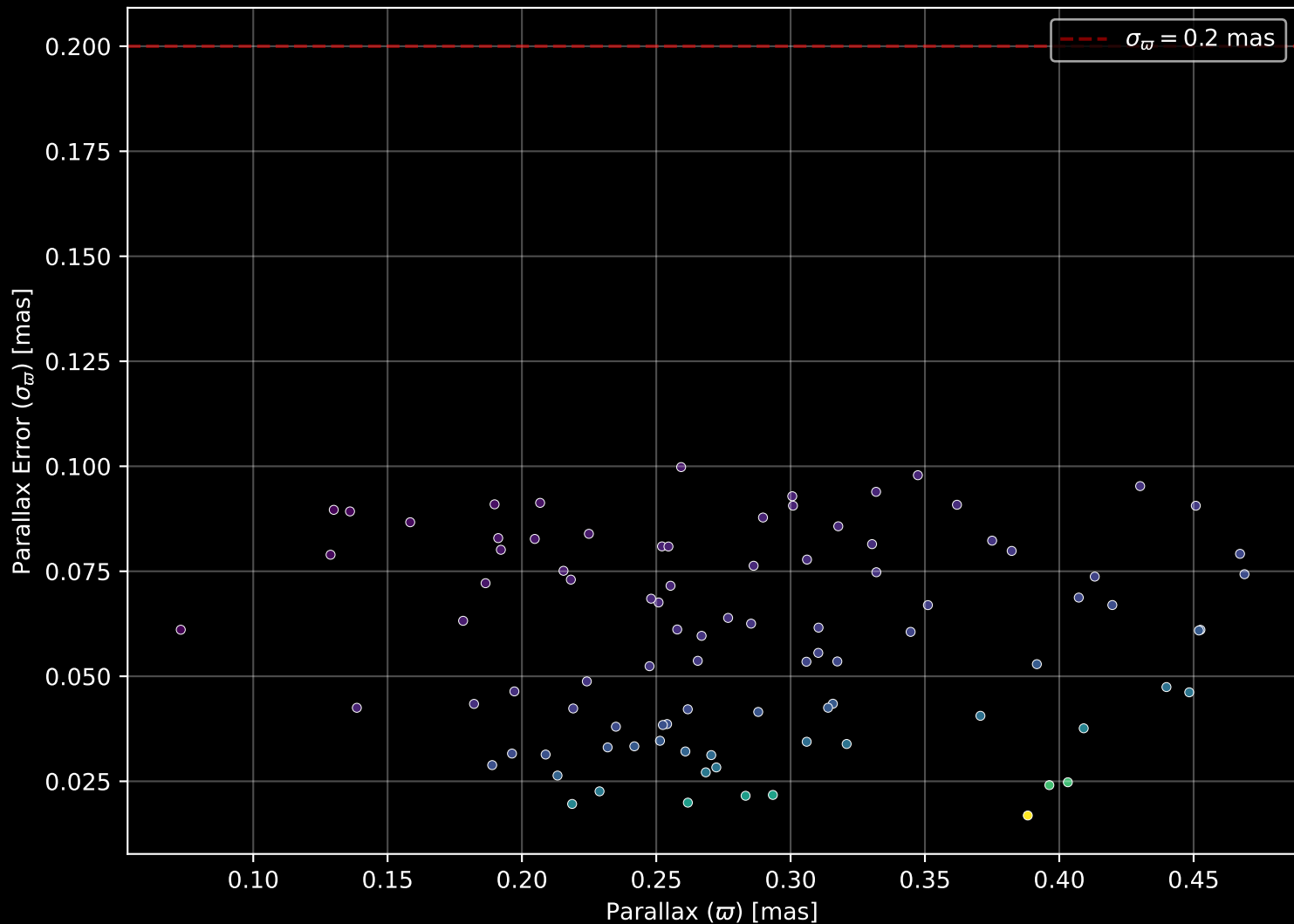
Gaia Cluster: [FSR_1521] Parallax Quality (n= 93)
