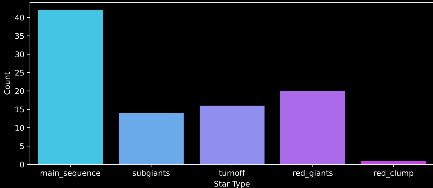
Gaia Cluster: [FSR_1521] Count plot of Star Type
