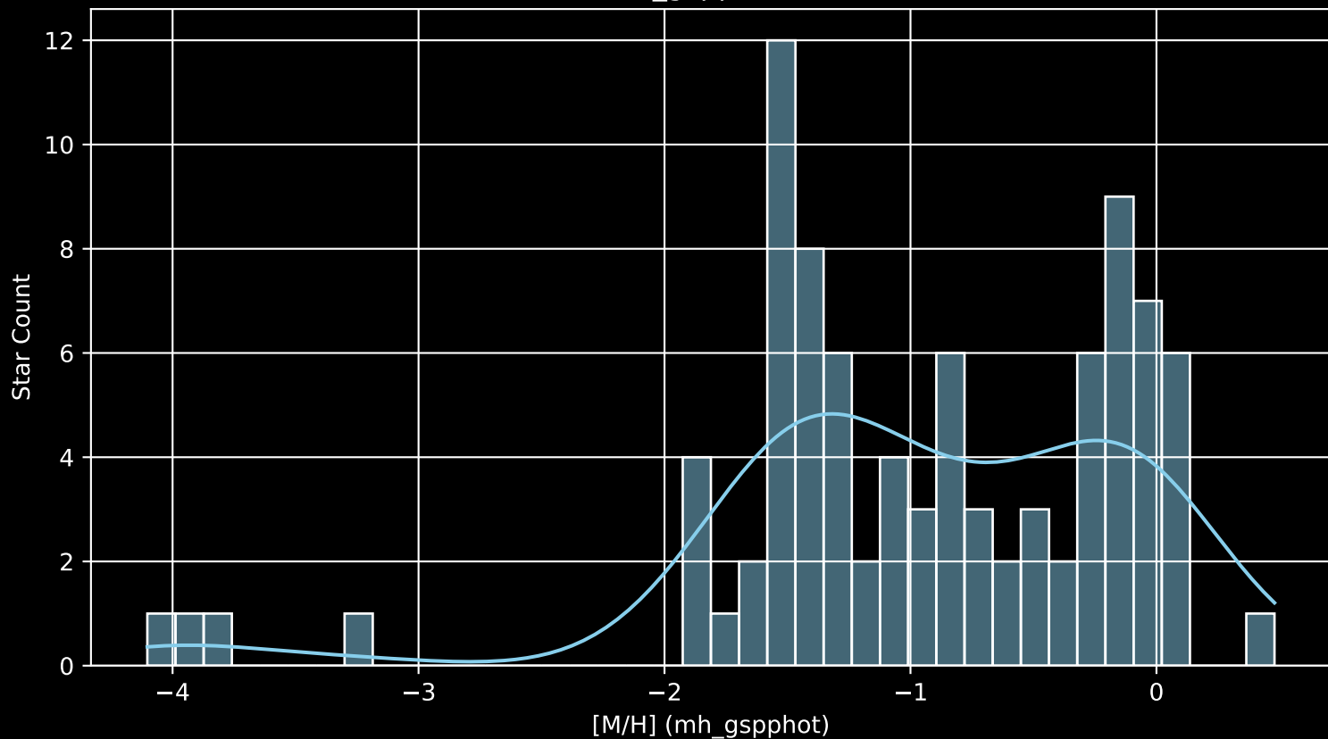
Gaia Cluster: [FSR_1521 [M/H] (mh_gspphot) (n= 91)
