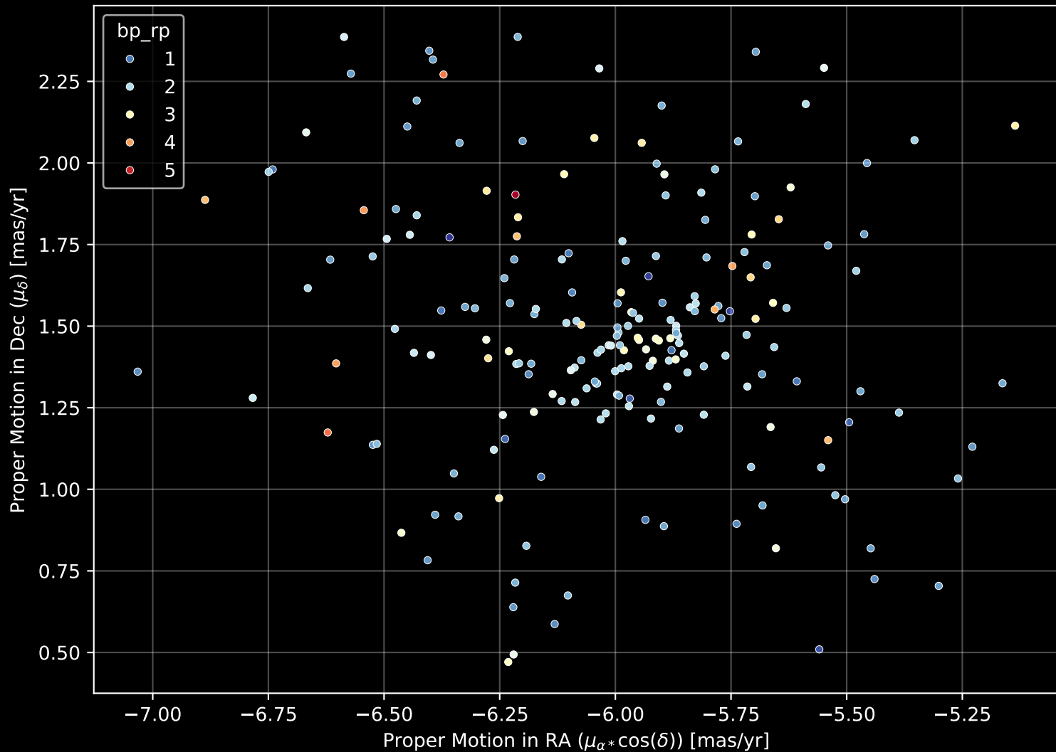
Gaia Cluster: [FSR_1586] Proper Motion Diagram (n= 207)
