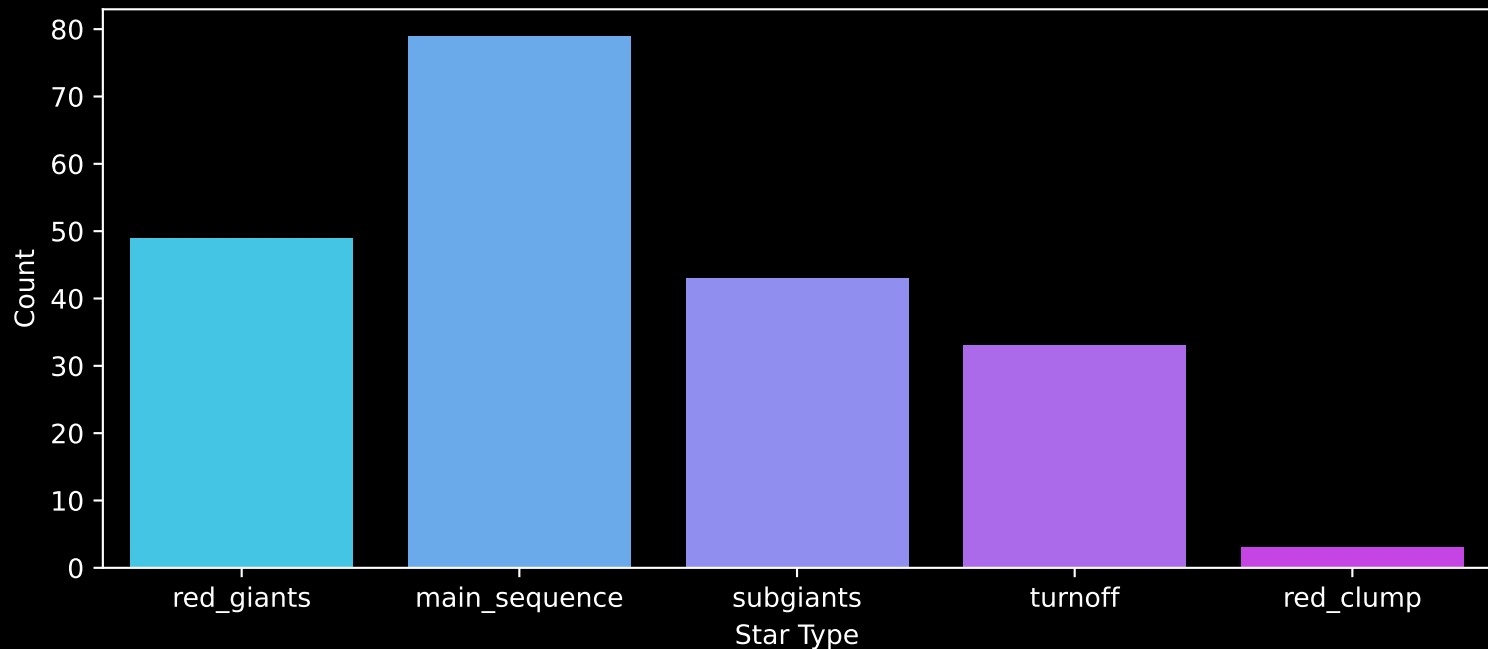
Gaia Cluster: [FSR_1586] Count plot of Star Type
