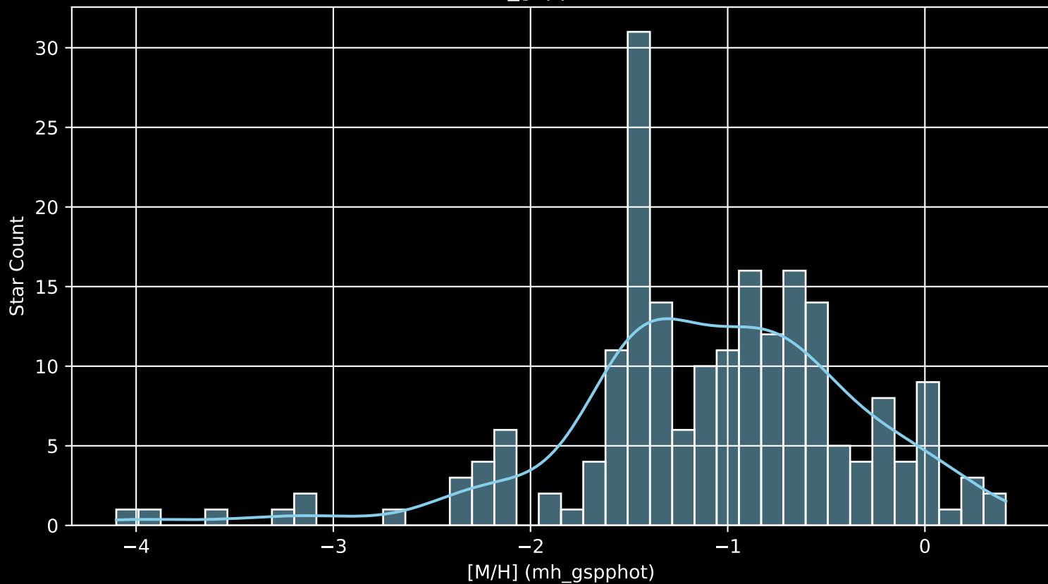
Gaia Cluster: [FSR_1586 [M/H] (mh_gspphot) (n= 204)
