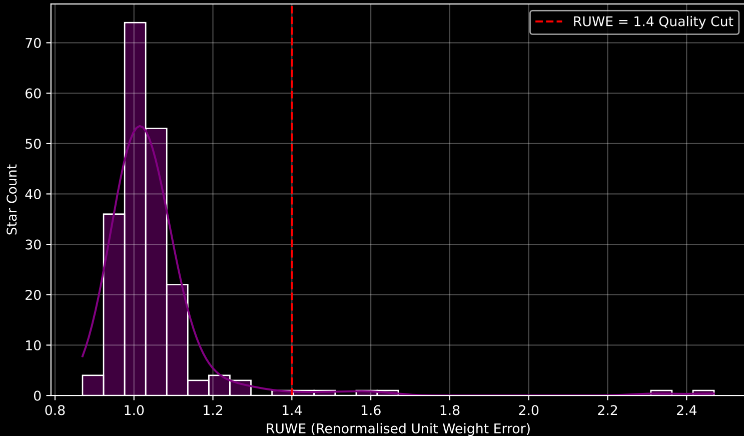
Gaia Cluster: [FSR_1586] RUWE Distribution (n= 206)
