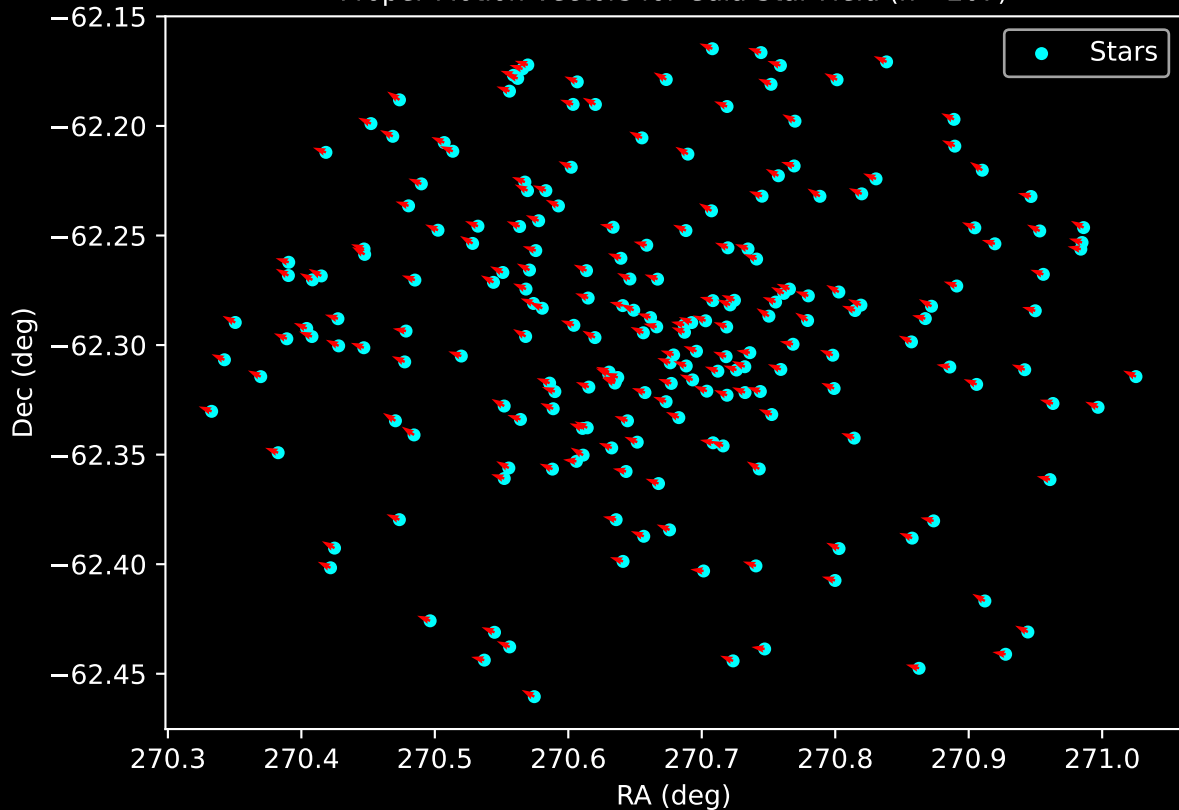
Gaia Cluster: [FSR_1586] Proper Motion Vectors for Gaia Star Field (n= 207)
