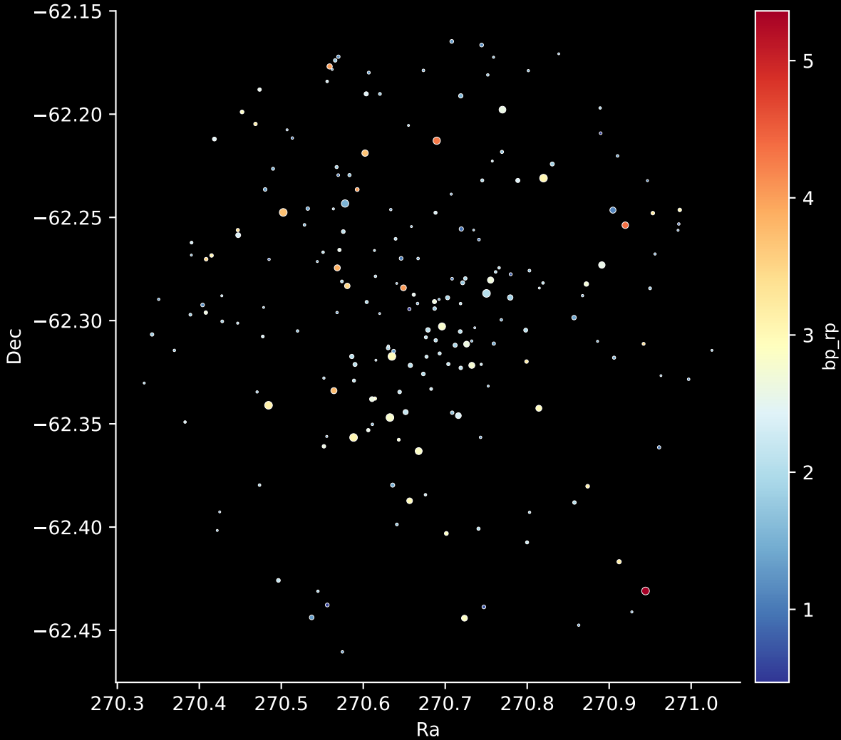
Gaia Cluster: [FSR_1586] Stars: 207
