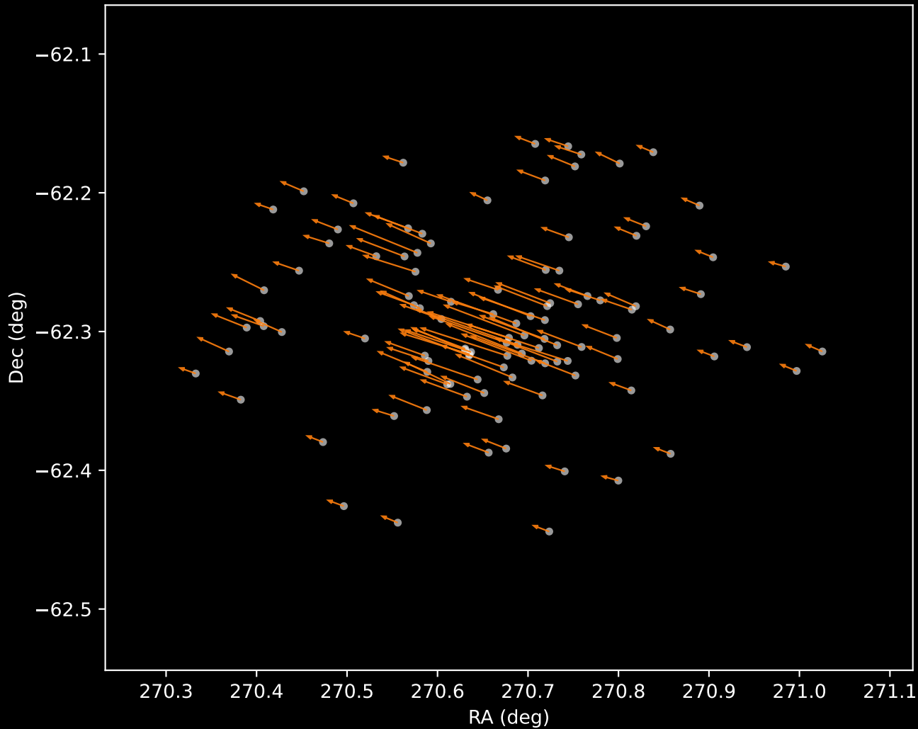
Gaia DR3 Cluster 2 Proper Motion Vectors (n=108)
