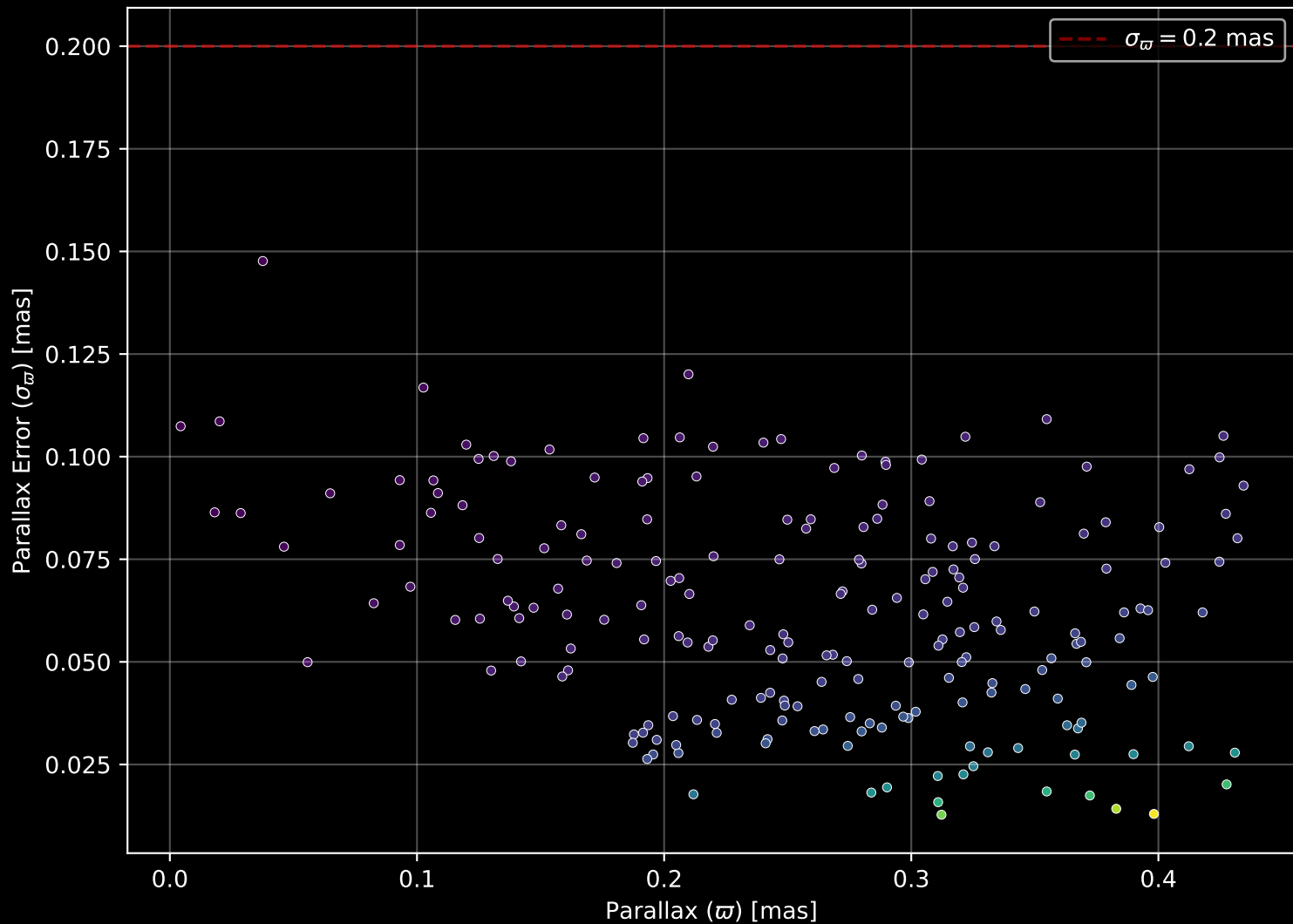
Gaia Cluster: [FSR_1586] Parallax Quality (n= 207)
