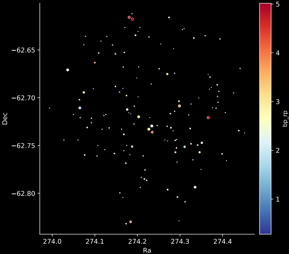
Gaia Cluster: [FSR_1591] Stars: 136
