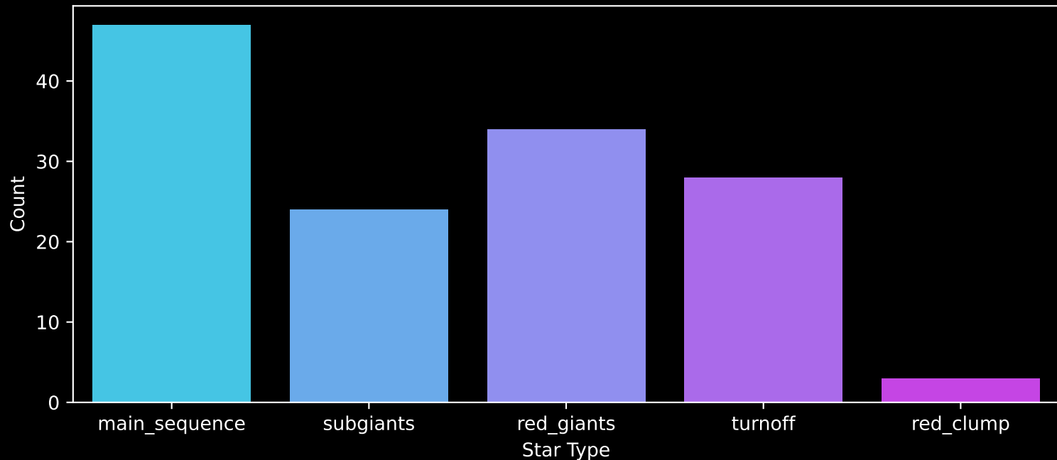
Gaia Cluster: [FSR_1591] Count plot of Star Type
