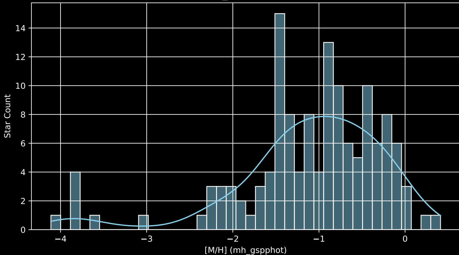
Gaia Cluster: [FSR_1591 [M/H] (mh_gspphot) (n= 135)
