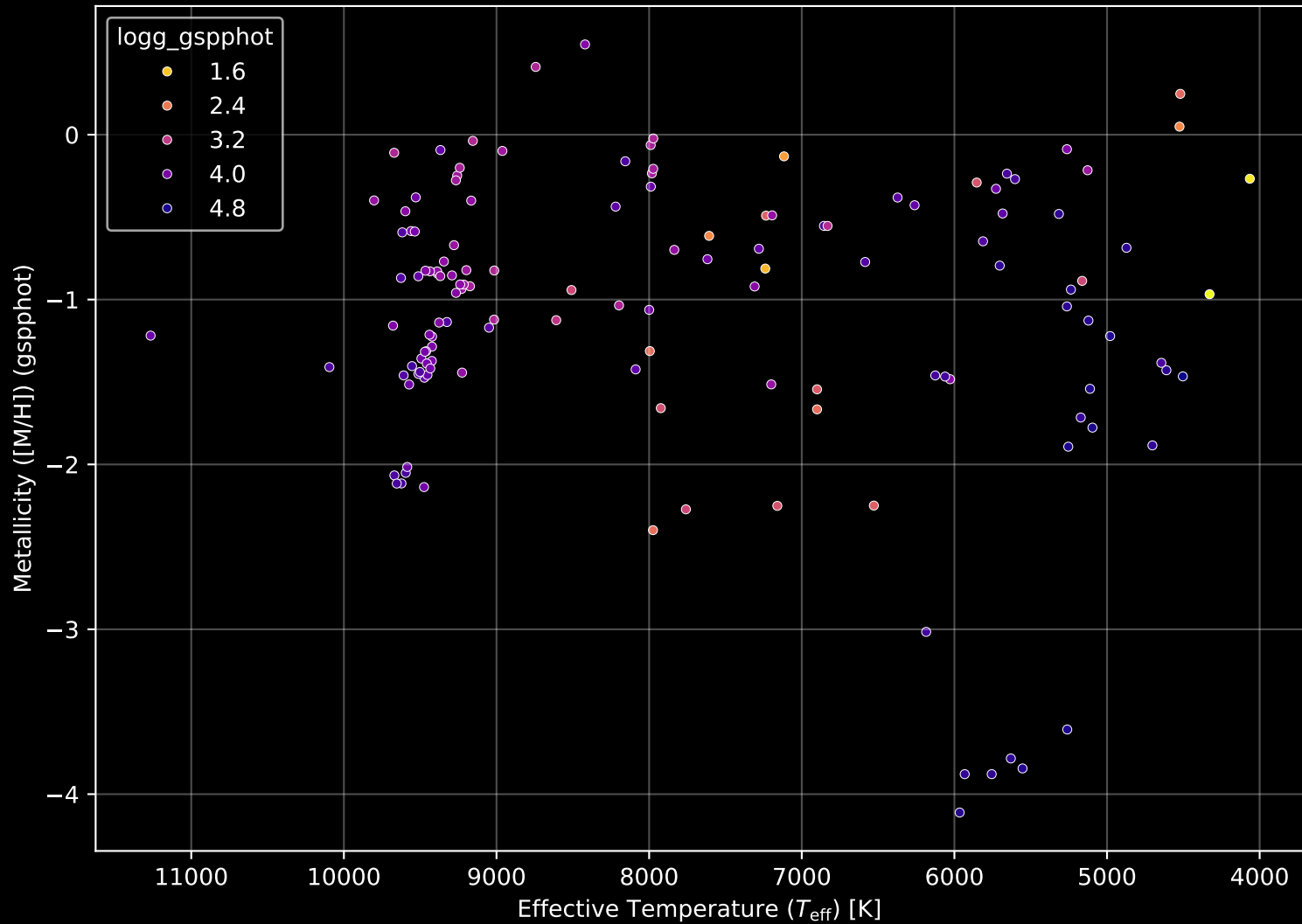
Gaia Cluster: [FSR_1591] Stellar Population Parameters (n= 136)
