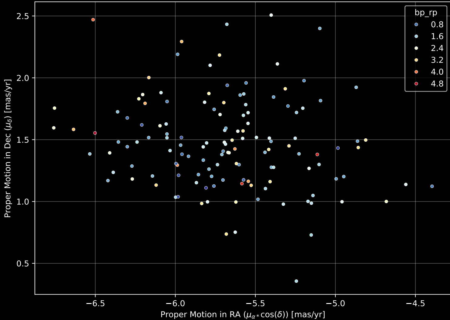
Gaia Cluster: [FSR_1591] Proper Motion Diagram (n= 136)
