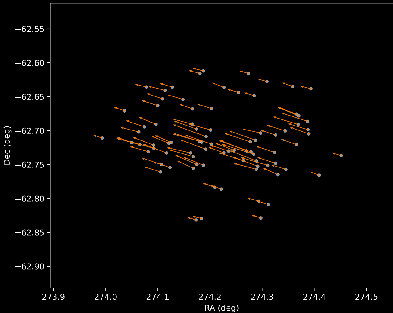
Gaia DR3 Cluster 2 Proper Motion Vectors (n=82)
