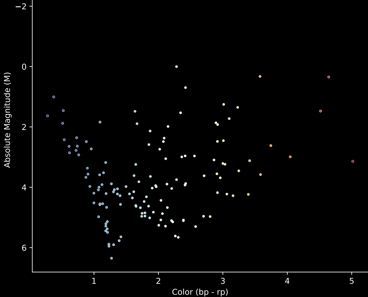
Gaia Cluster: [FSR_1591] Stars (n= 136) Hertzsprung-Russel Diagram
