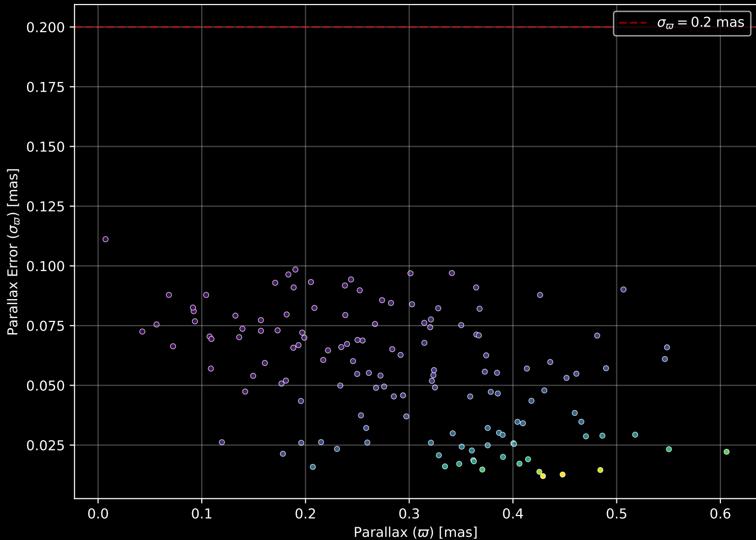
Gaia Cluster: [FSR_1591] Parallax Quality (n= 136)
