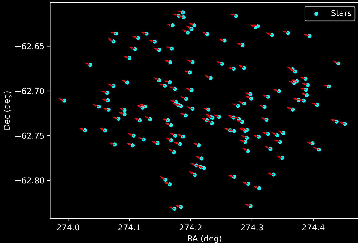
Gaia Cluster: [FSR_1591] Proper Motion Vectors for Gaia Star Field (n= 136)
