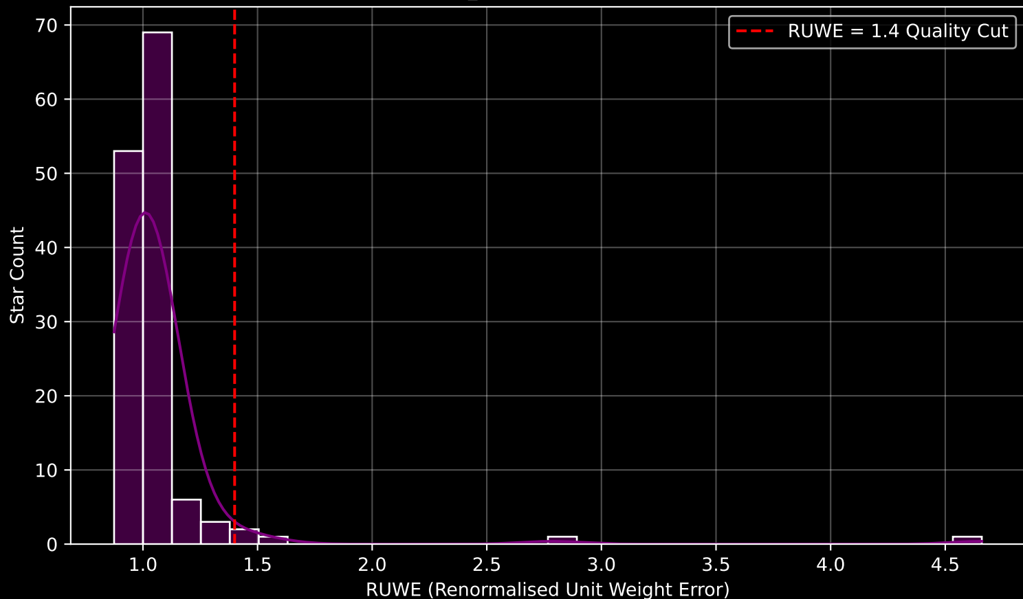
Gaia Cluster: [FSR_1591] RUWE Distribution (n= 136)
