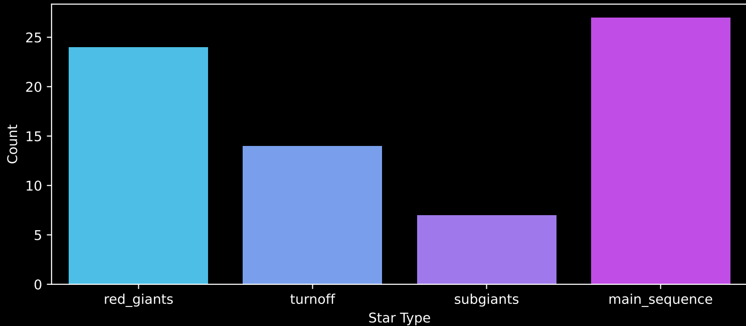
Gaia Cluster: [FSR_1663] Count plot of Star Type
