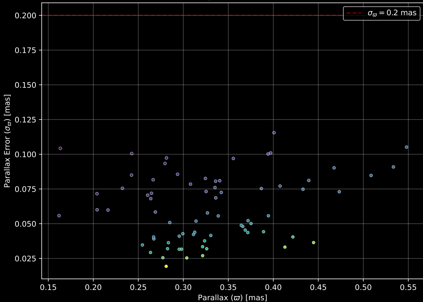
Gaia Cluster: [FSR_1663] Parallax Quality (n= 72)
