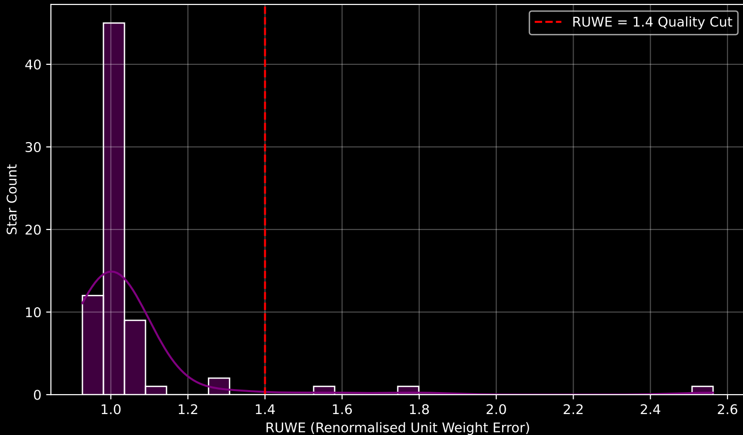
Gaia Cluster: [FSR_1663] RUWE Distribution (n= 72)
