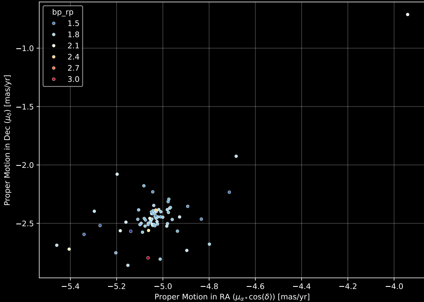
Gaia Cluster: [FSR_1663] Proper Motion Diagram (n= 72)
