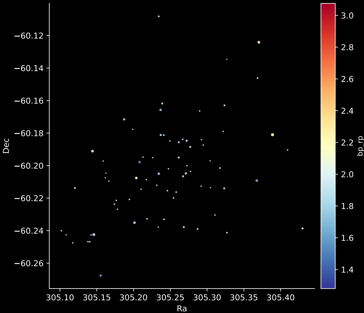
Gaia Cluster: [FSR_1663] Stars: 72
