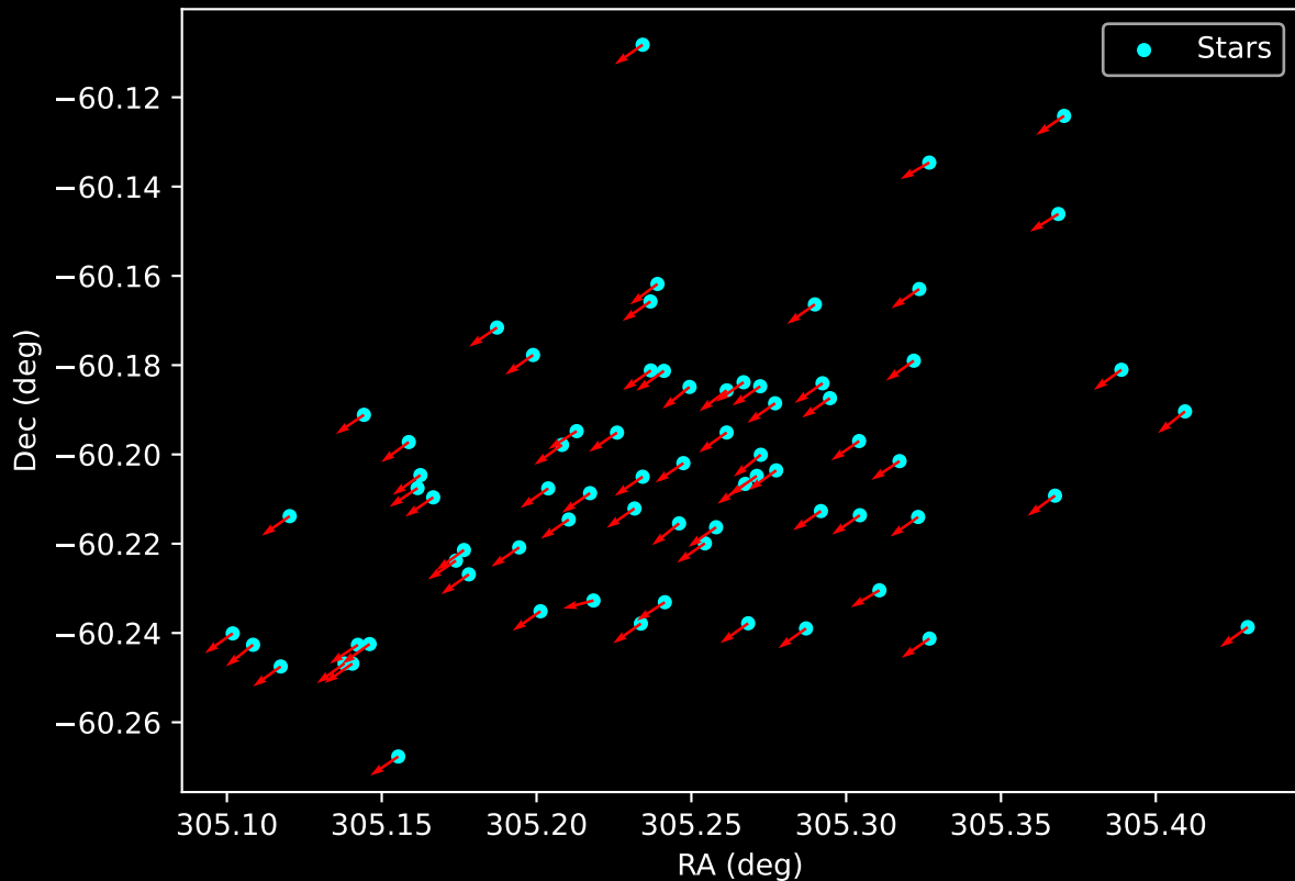
Gaia Cluster: [FSR_1663] Proper Motion Vectors for Gaia Star Field (n= 72)
