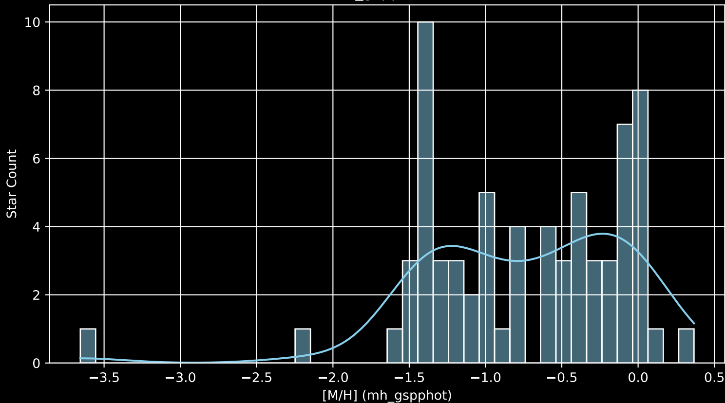
Gaia Cluster: [FSR_1663 [M/H] (mh_gspphot) (n= 69)
