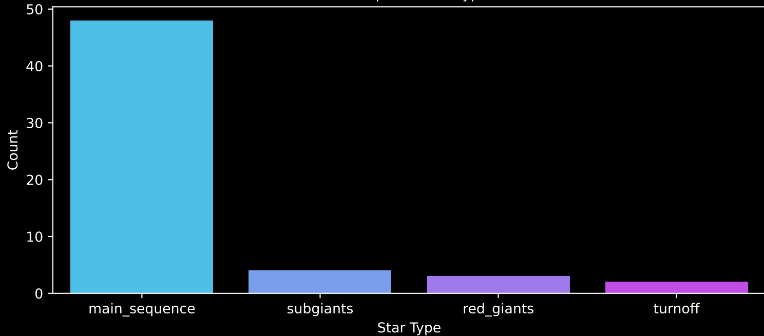
Gaia Cluster: [Gaia_2] Count plot of Star Type
