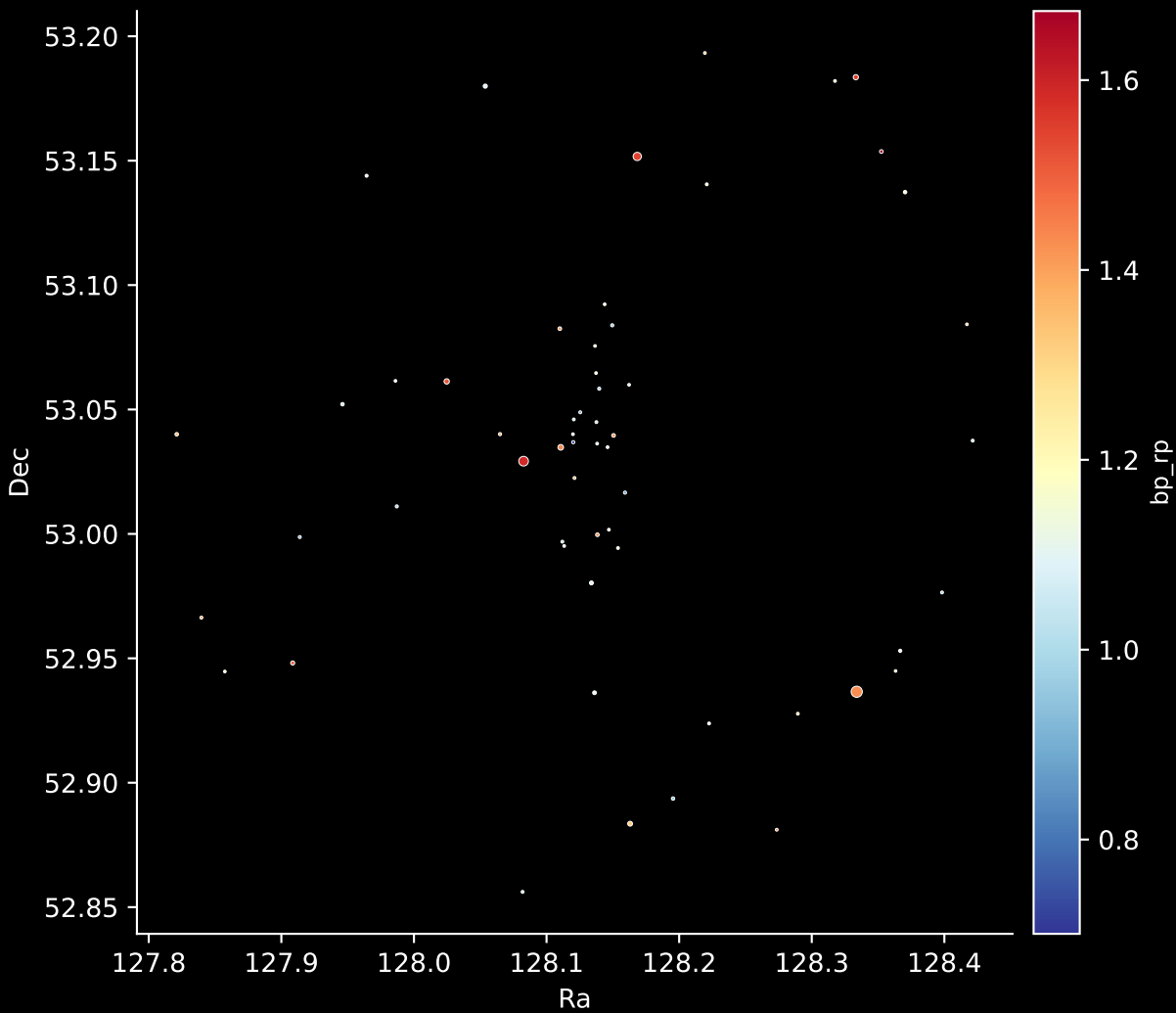
Gaia Cluster: [Gaia_2] Stars: 57
