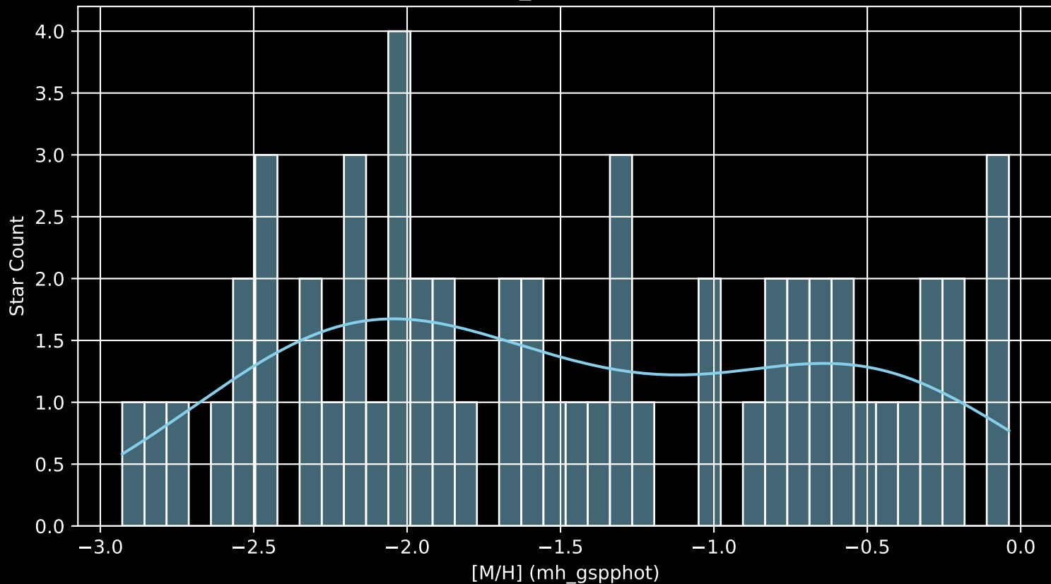
Gaia Cluster: [Gaia_2 [M/H] (mh_gspphot) (n= 57)
