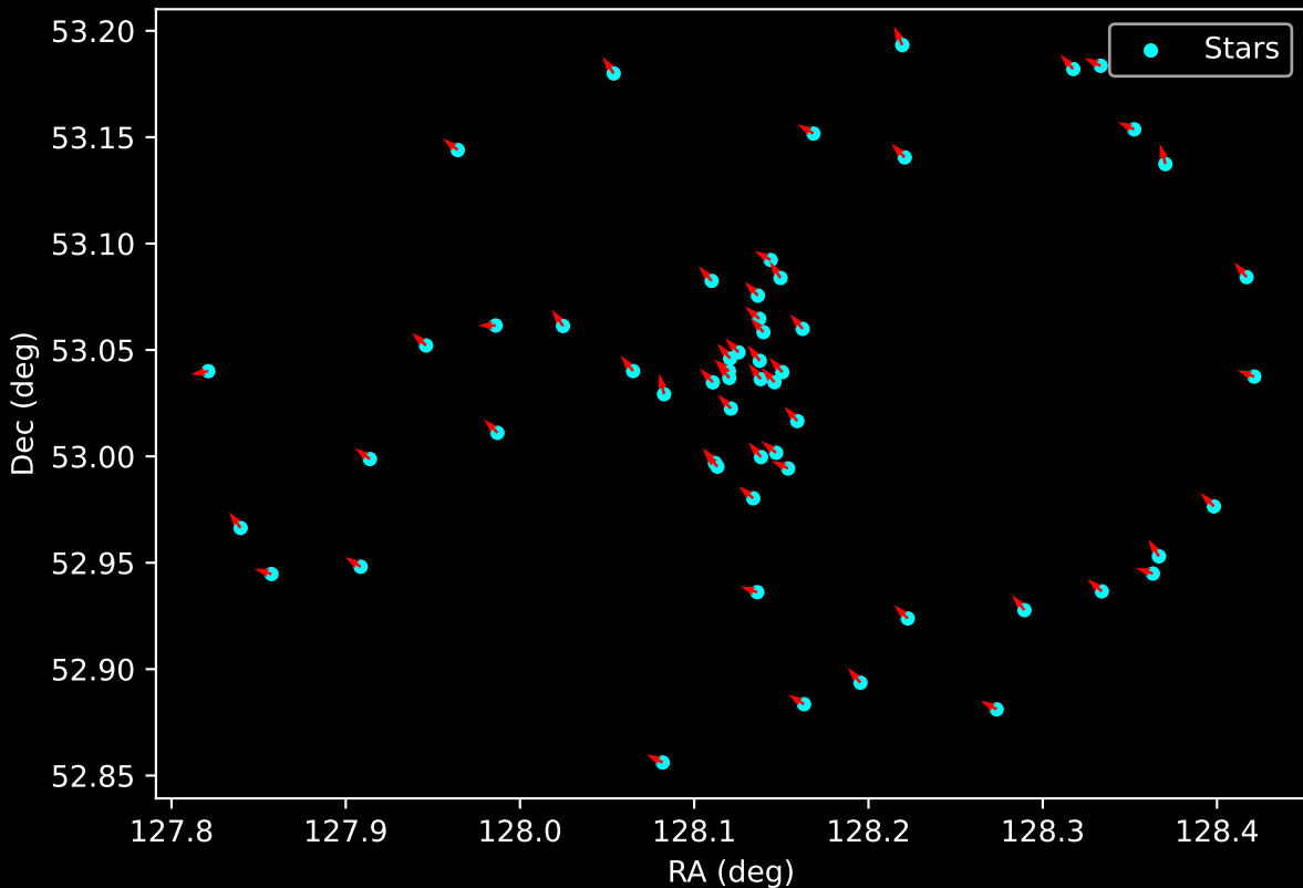
Gaia Cluster: [Gaia_2] Proper Motion Vectors for Gaia Star Field (n= 57)
