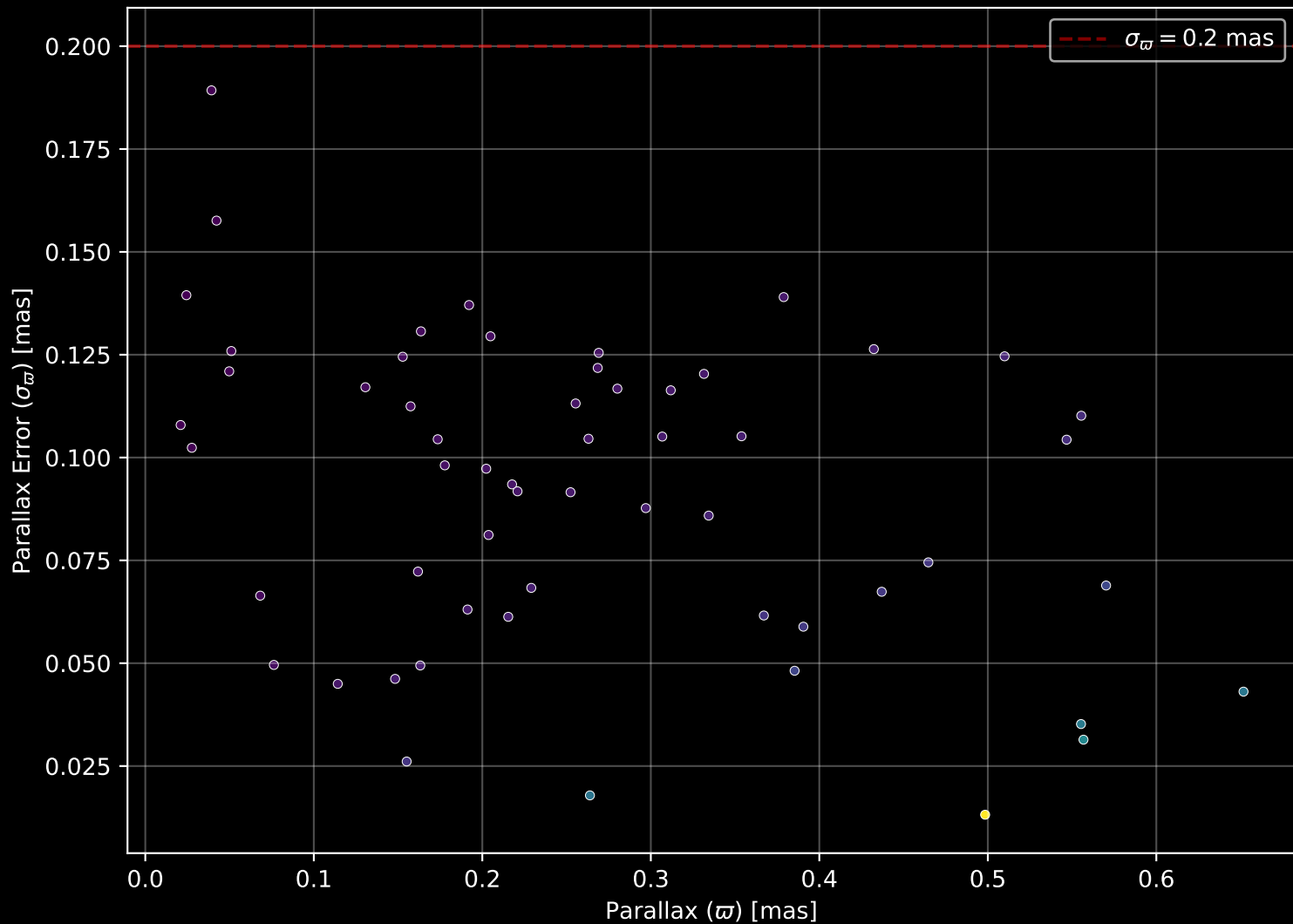
Gaia Cluster: [Gaia_2] Parallax Quality (n= 57)
