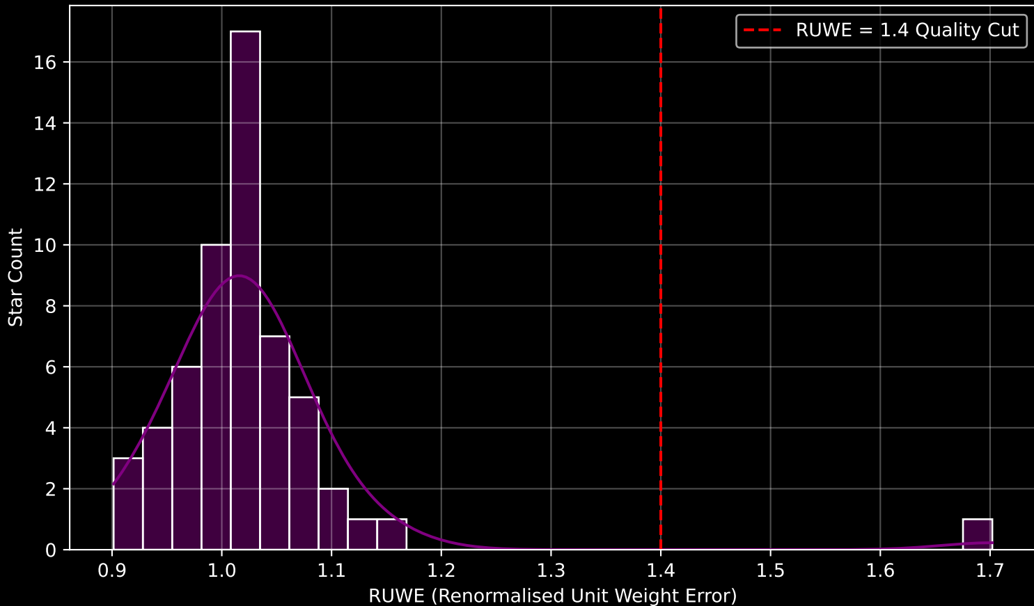
Gaia Cluster: [Gaia_2] RUWE Distribution (n= 57)
