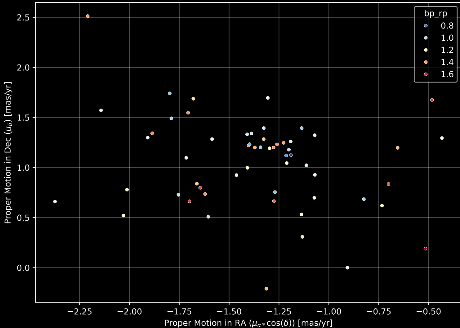
Gaia Cluster: [Gaia_2] Proper Motion Diagram (n= 57)
