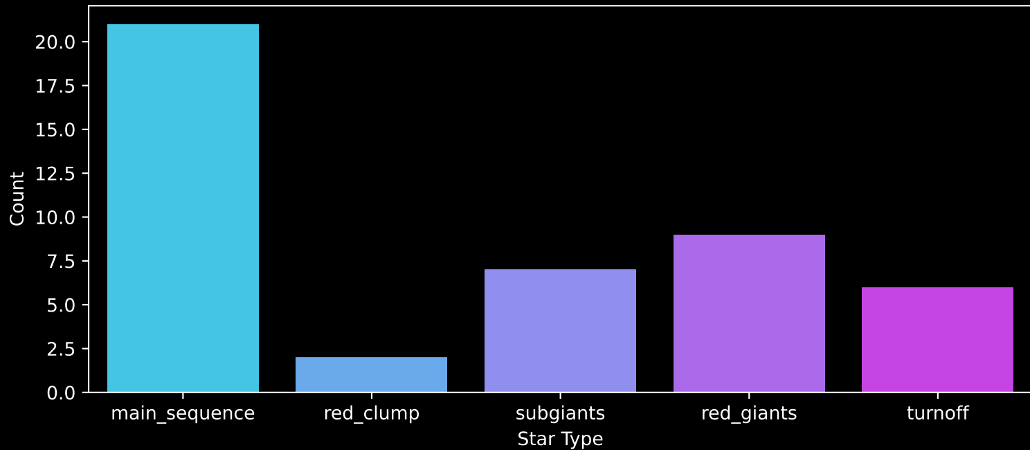
Gaia Cluster: [Graham_1] Count plot of Star Type
