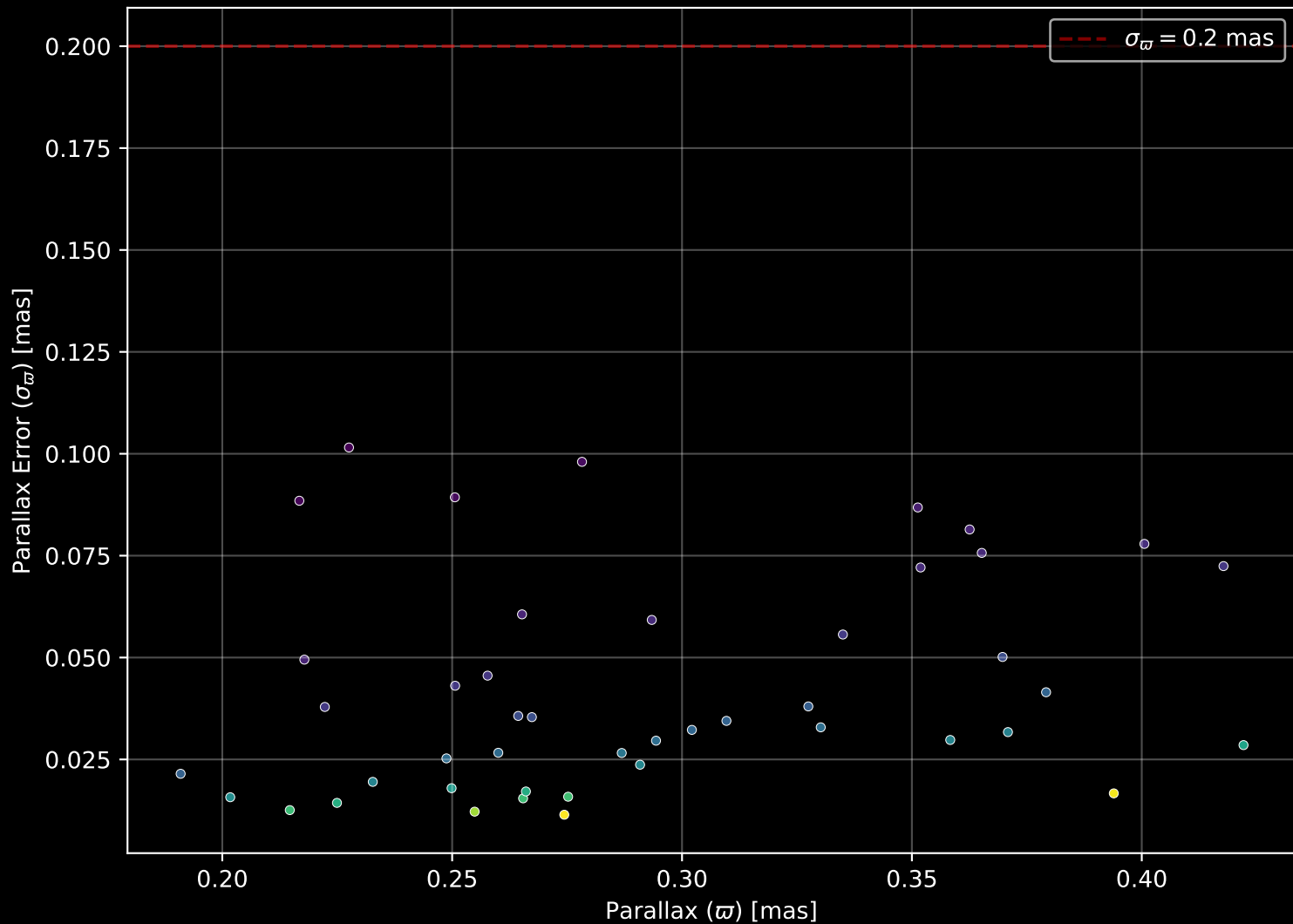
Gaia Cluster: [Graham_1] Parallax Quality (n= 45)
