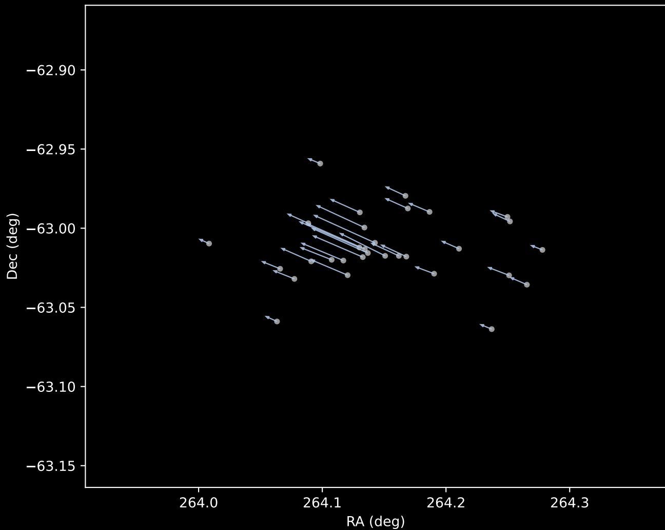
Gaia DR3 Cluster 1 Proper Motion Vectors (n=31)
