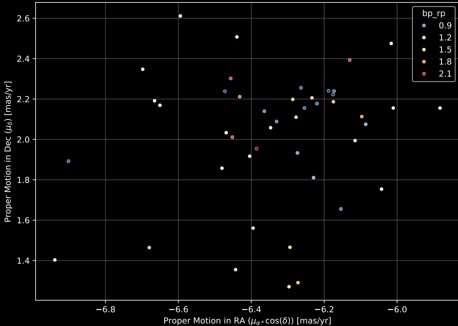
Gaia Cluster: [Graham_1] Proper Motion Diagram (n= 45)
