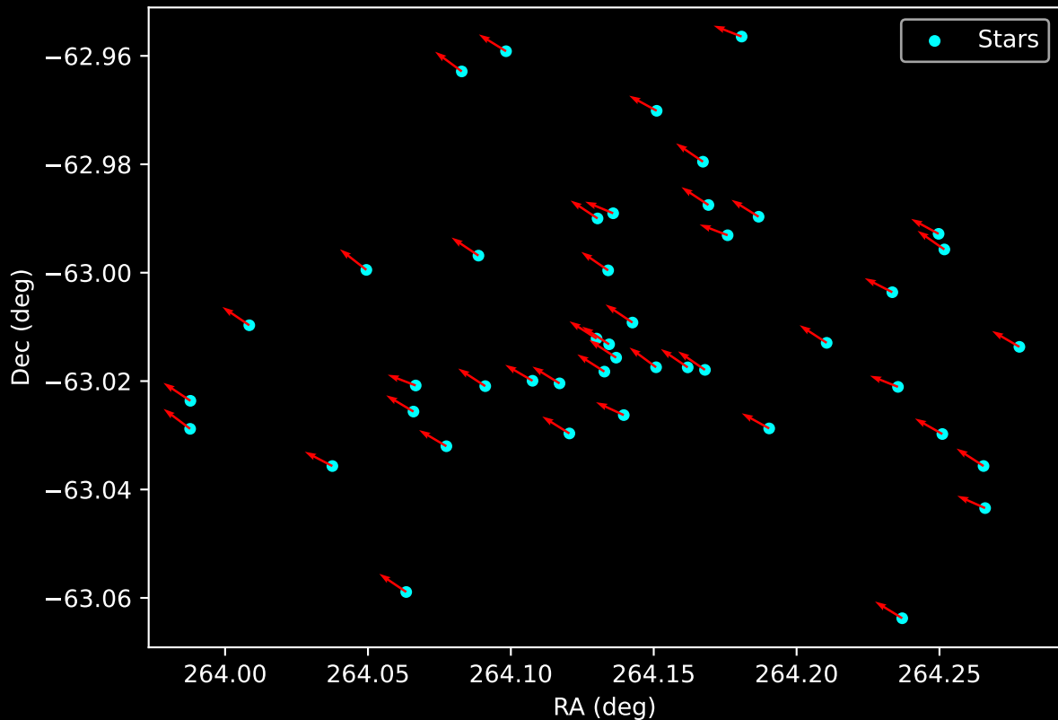
Gaia Cluster: [Graham_1] Proper Motion Vectors for Gaia Star Field (n= 45)
