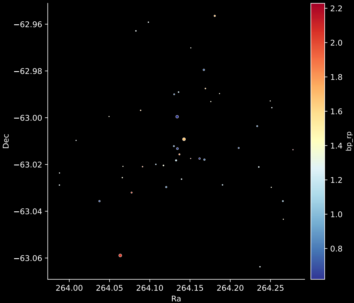
Gaia Cluster: [Graham_1] Stars: 45
