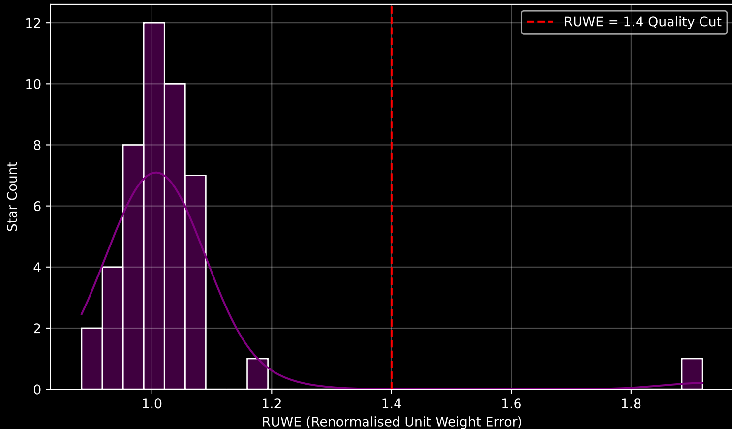
Gaia Cluster: [Graham_1] RUWE Distribution (n= 45)
