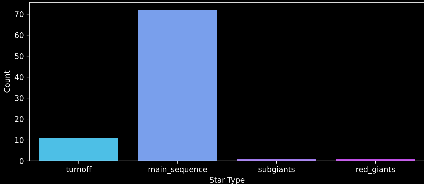
Gaia Cluster: [Gulliver_11] Count plot of Star Type
