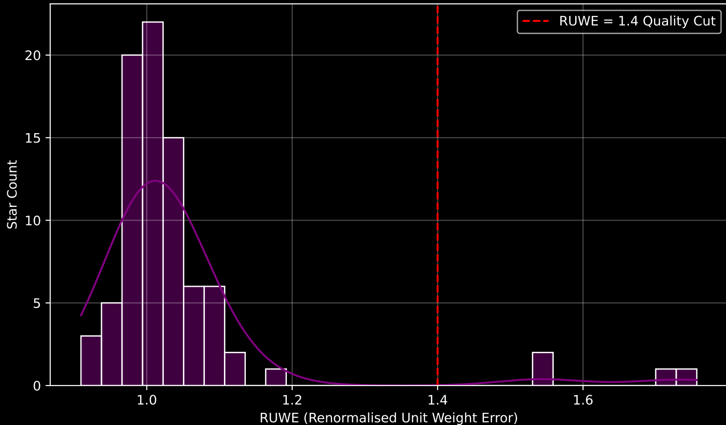
Gaia Cluster: [Gulliver_11] RUWE Distribution (n= 84)
