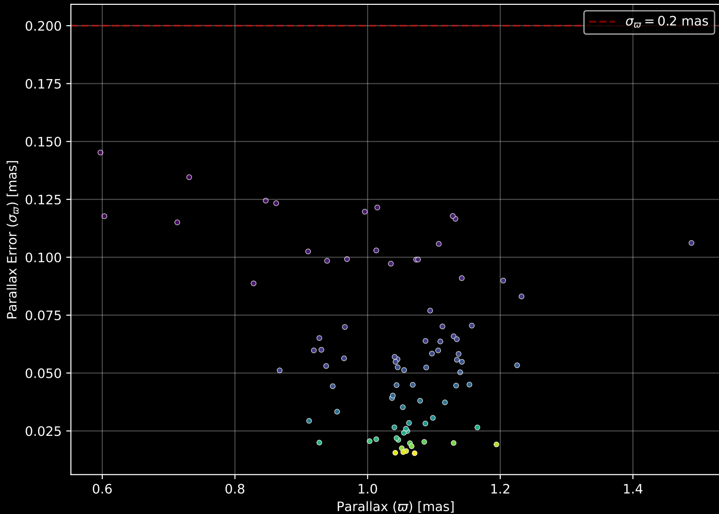
Gaia Cluster: [Gulliver_11] Parallax Quality (n= 85)
