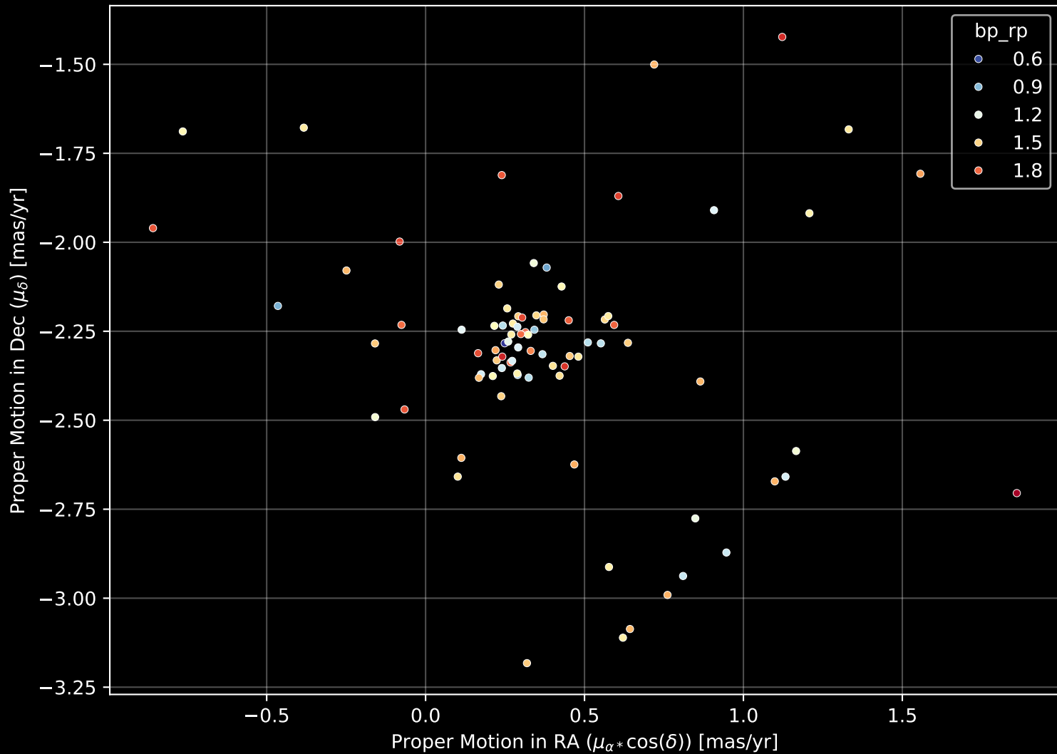
Gaia Cluster: [Gulliver_11] Proper Motion Diagram (n= 85)
