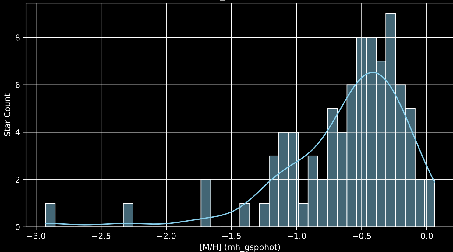
Gaia Cluster: [Gulliver_11 [M/H] (mh_gspphot) (n= 85)
