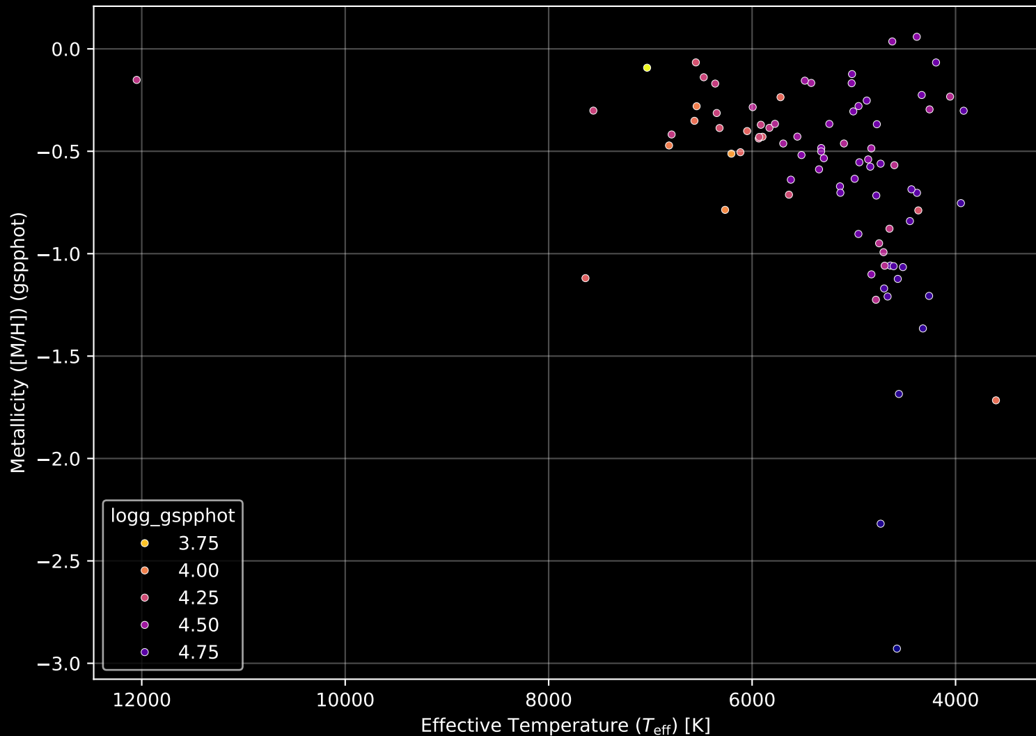
Gaia Cluster: [Gulliver_11] Stellar Population Parameters (n= 85)
