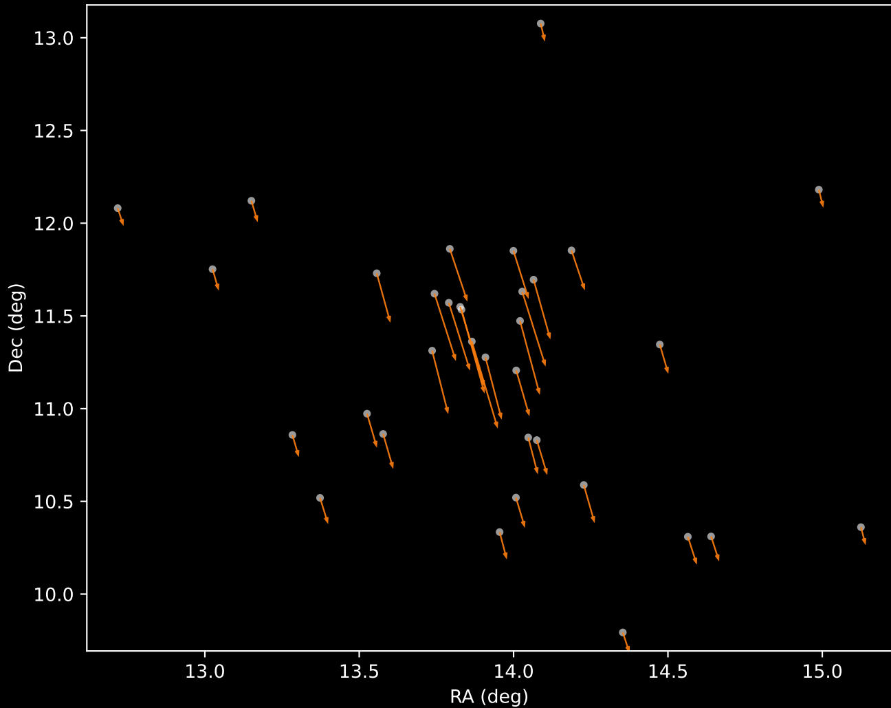
Gaia DR3 Cluster 2 Proper Motion Vectors (n=34)
