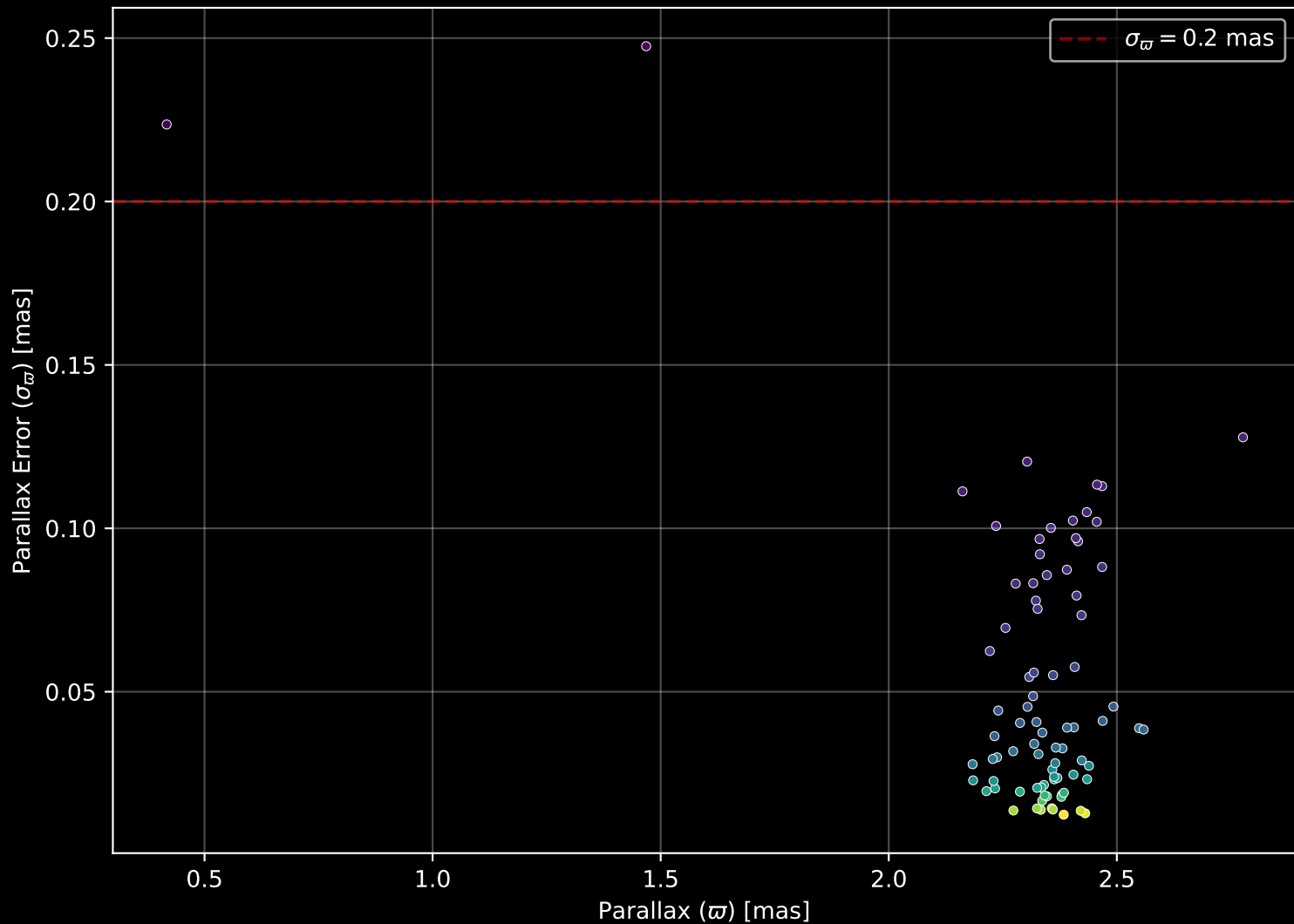
Gaia Cluster: [Gulliver 20] Parallax Quality (n= 83)
