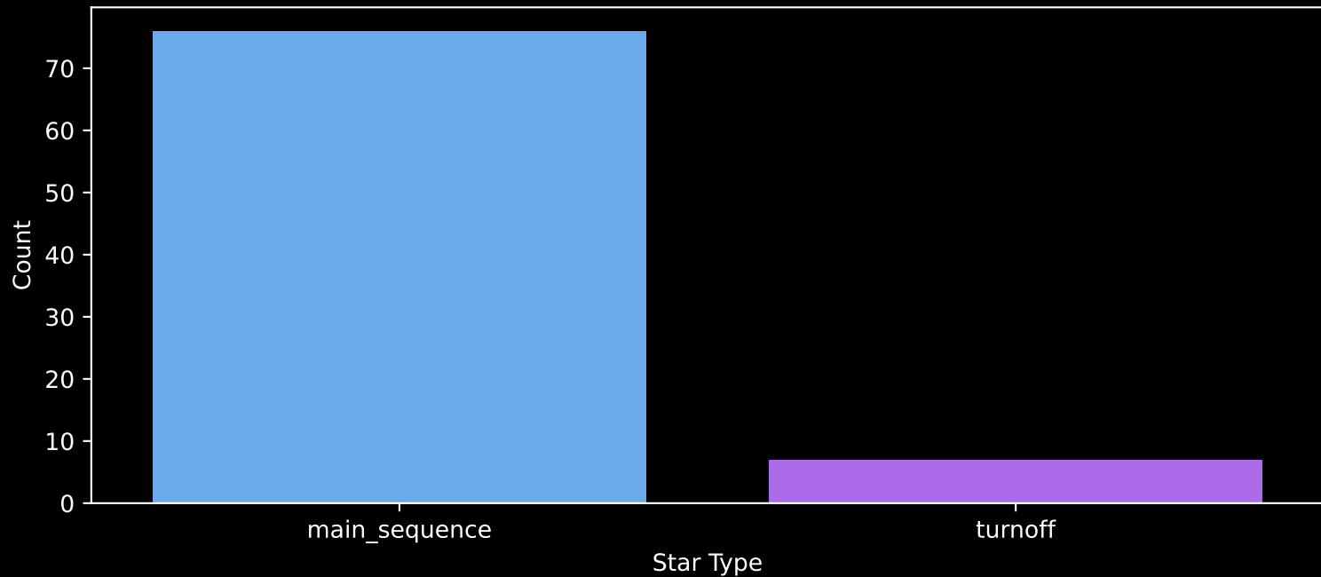
Gaia Cluster: [Gulliver_20] Count plot of Star Type
