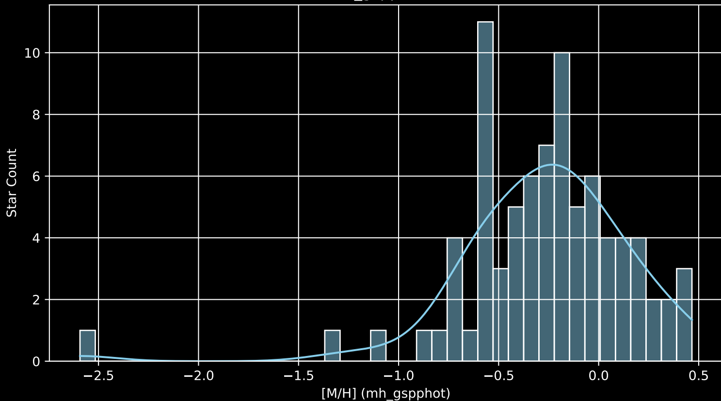
Gaia Cluster: [Gulliver_20 [M/H] (mh_gspphot) (n= 82)
