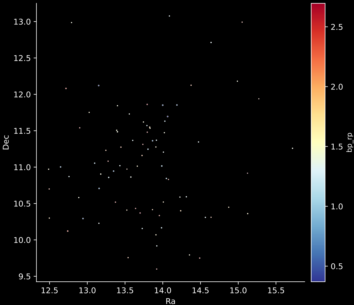
Gaia Cluster: [Gulliver_20] Stars: 83
