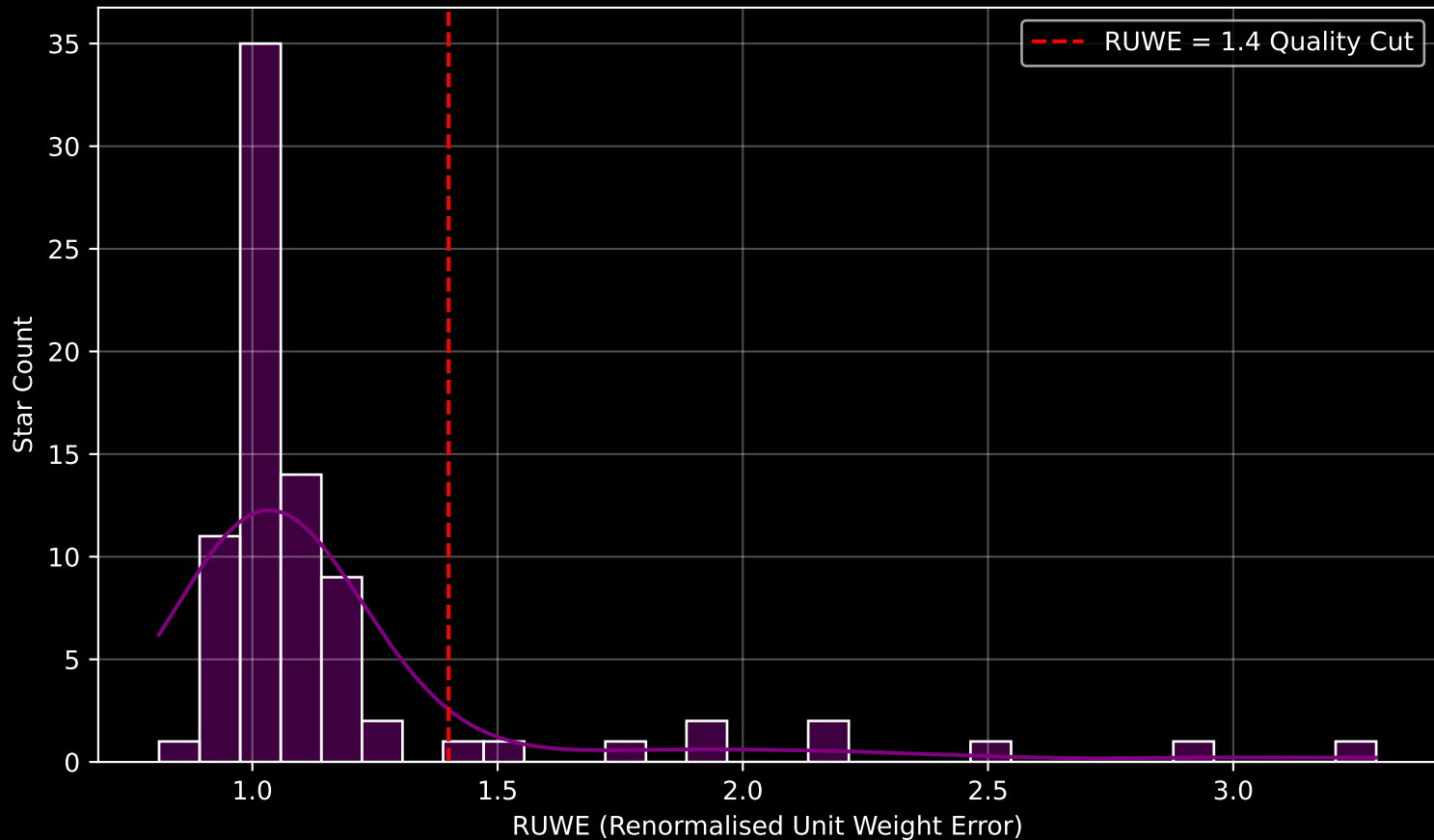
Gaia Cluster: [Gulliver_20] RUWE Distribution (n= 82)
