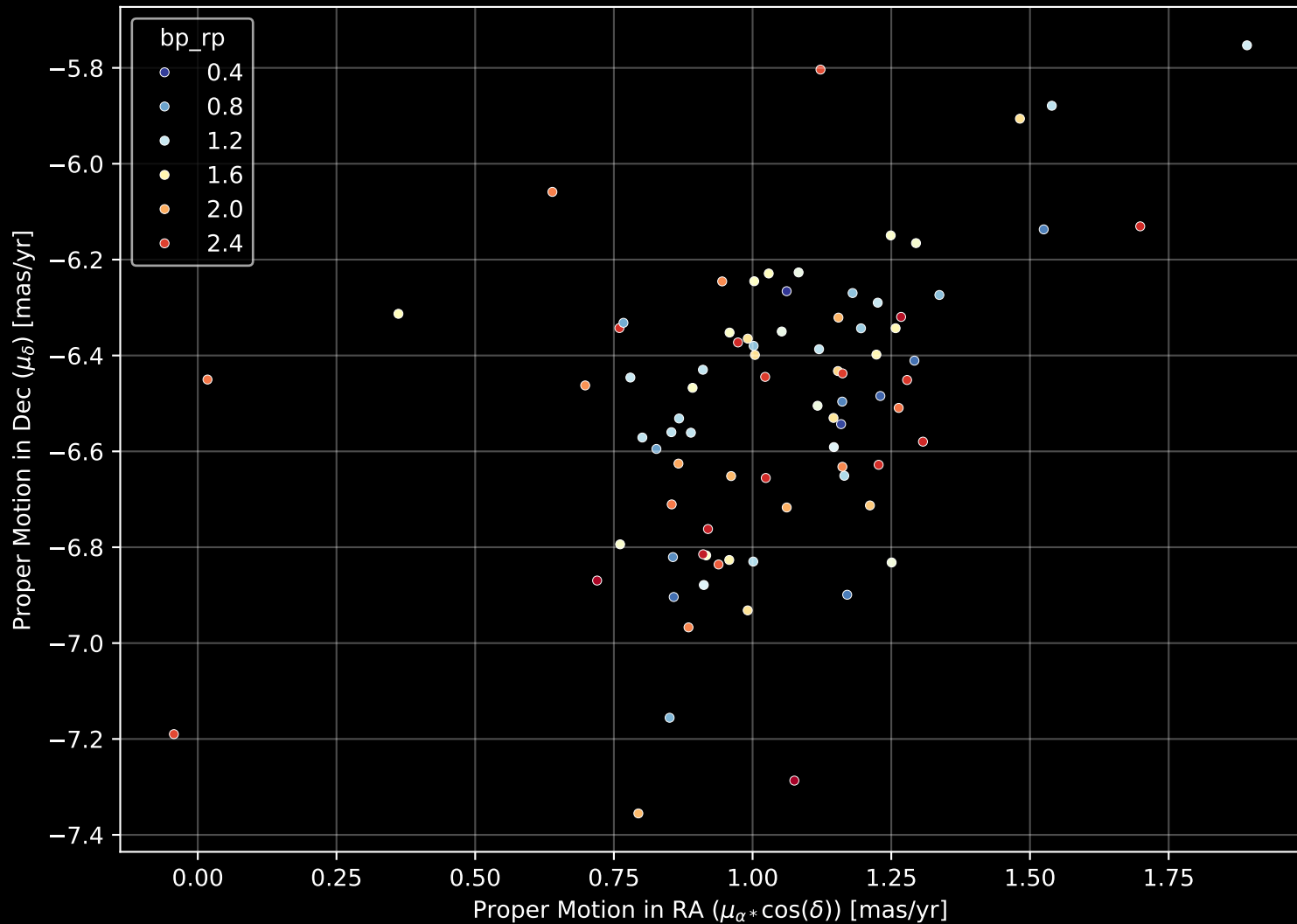
Gaia Cluster: [Gulliver_20] Proper Motion Diagram (n= 83)
