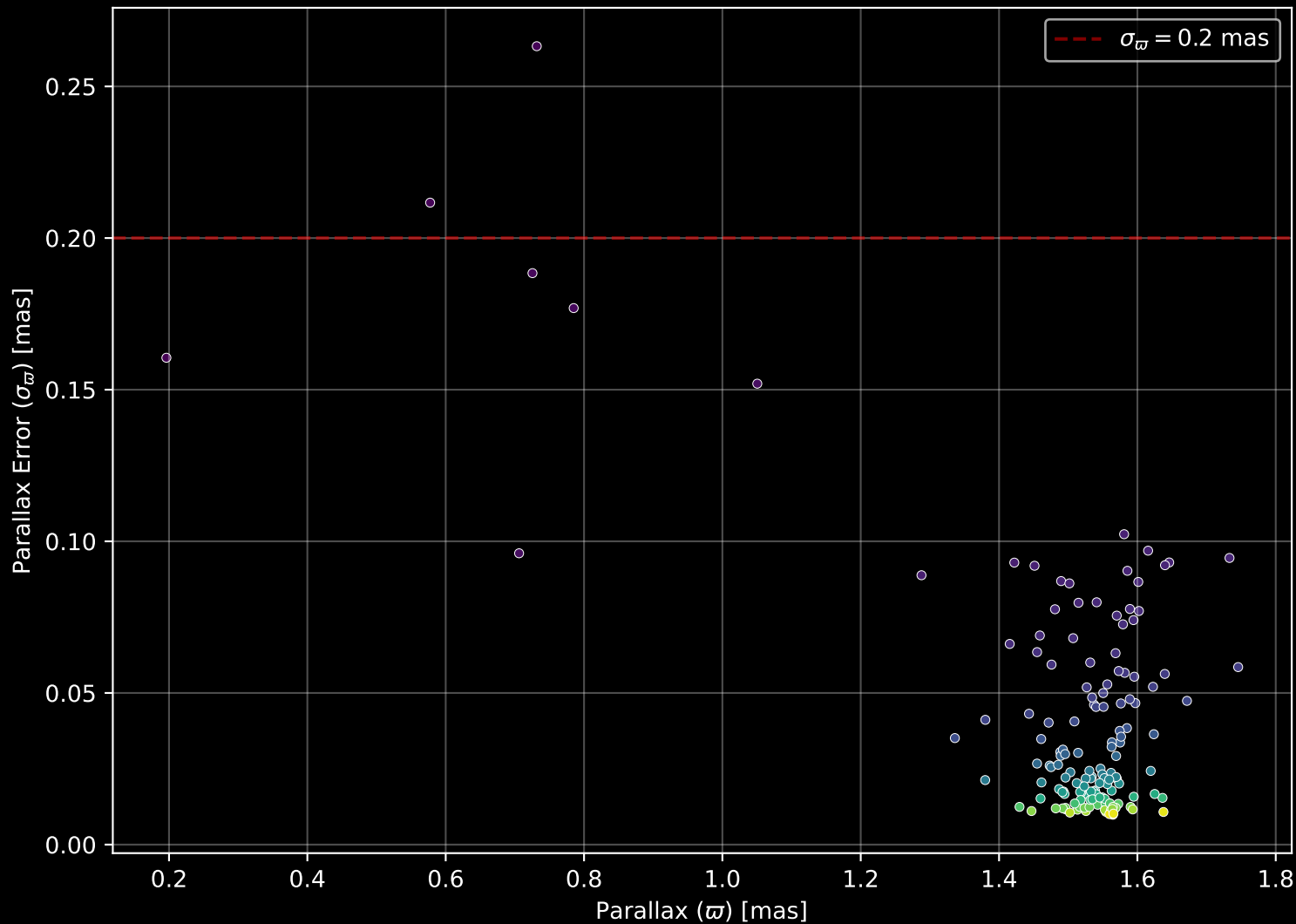
Gaia Cluster: [Gulliver_21] Parallax Quality (n= 151)
