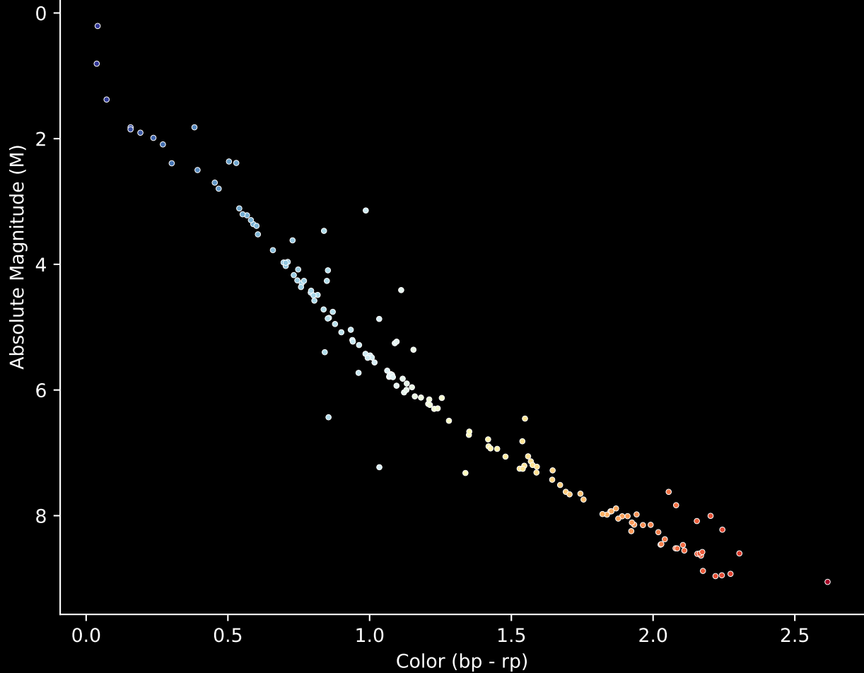
Gaia Cluster: [Gulliver_21] Stars (n= 151) Hertzsprung-Russel Diagram
