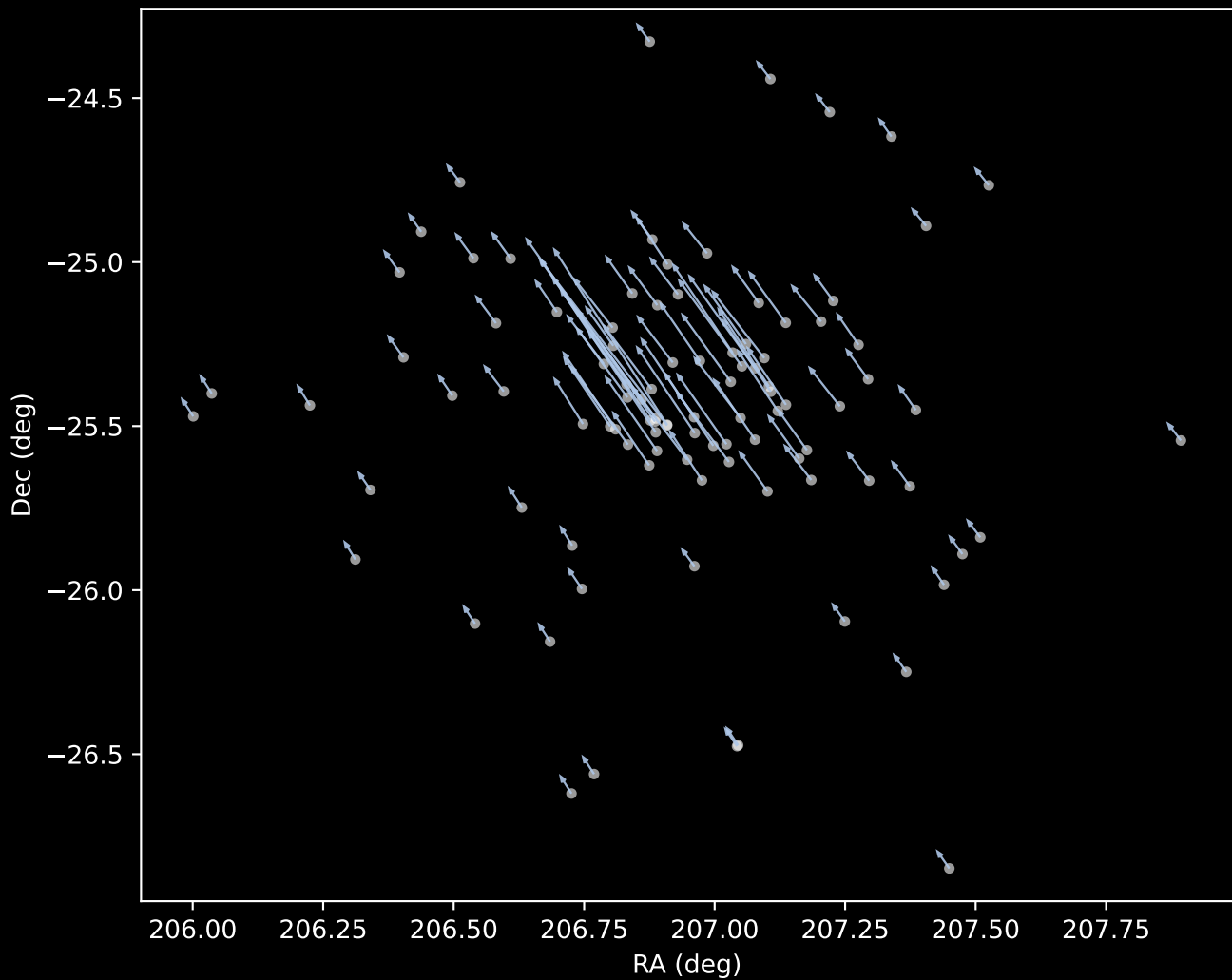
Gaia DR3 Cluster 1 Proper Motion Vectors (n=98)
