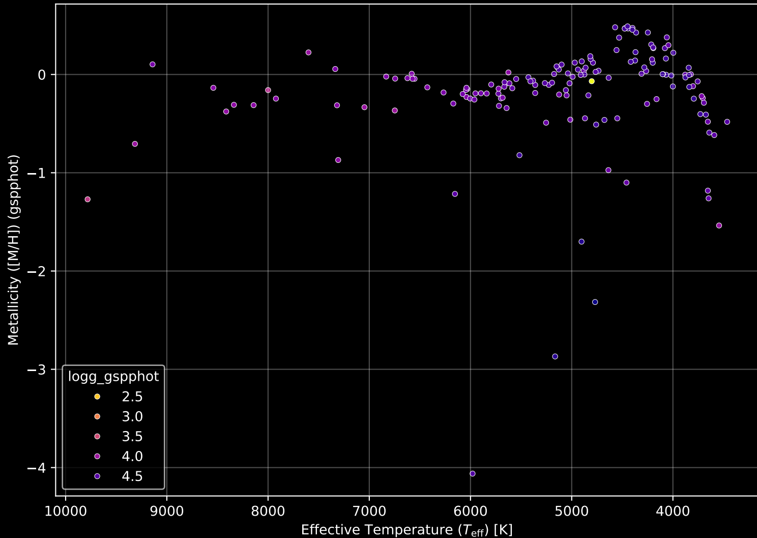
Gaia Cluster: [Gulliver_21] Stellar Population Parameters (n= 151)
