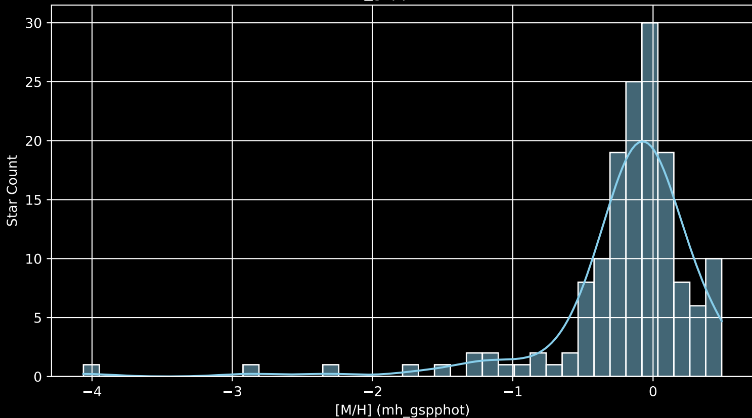
Gaia Cluster: [Gulliver_21 [M/H] (mh_gspphot) (n= 151)
