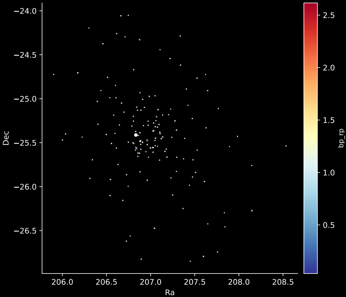
Gaia Cluster: [Gulliver_21] Stars: 151
