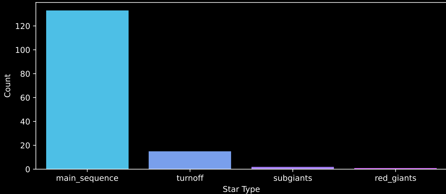
Gaia Cluster: [Gulliver_21] Count plot of Star Type
