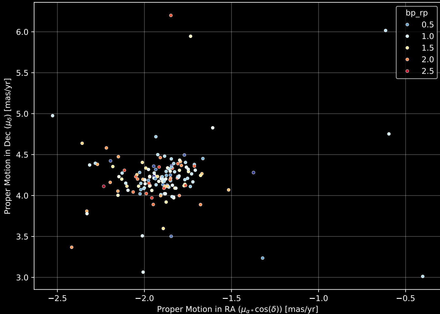
Gaia Cluster: [Gulliver_21] Proper Motion Diagram (n= 151)
