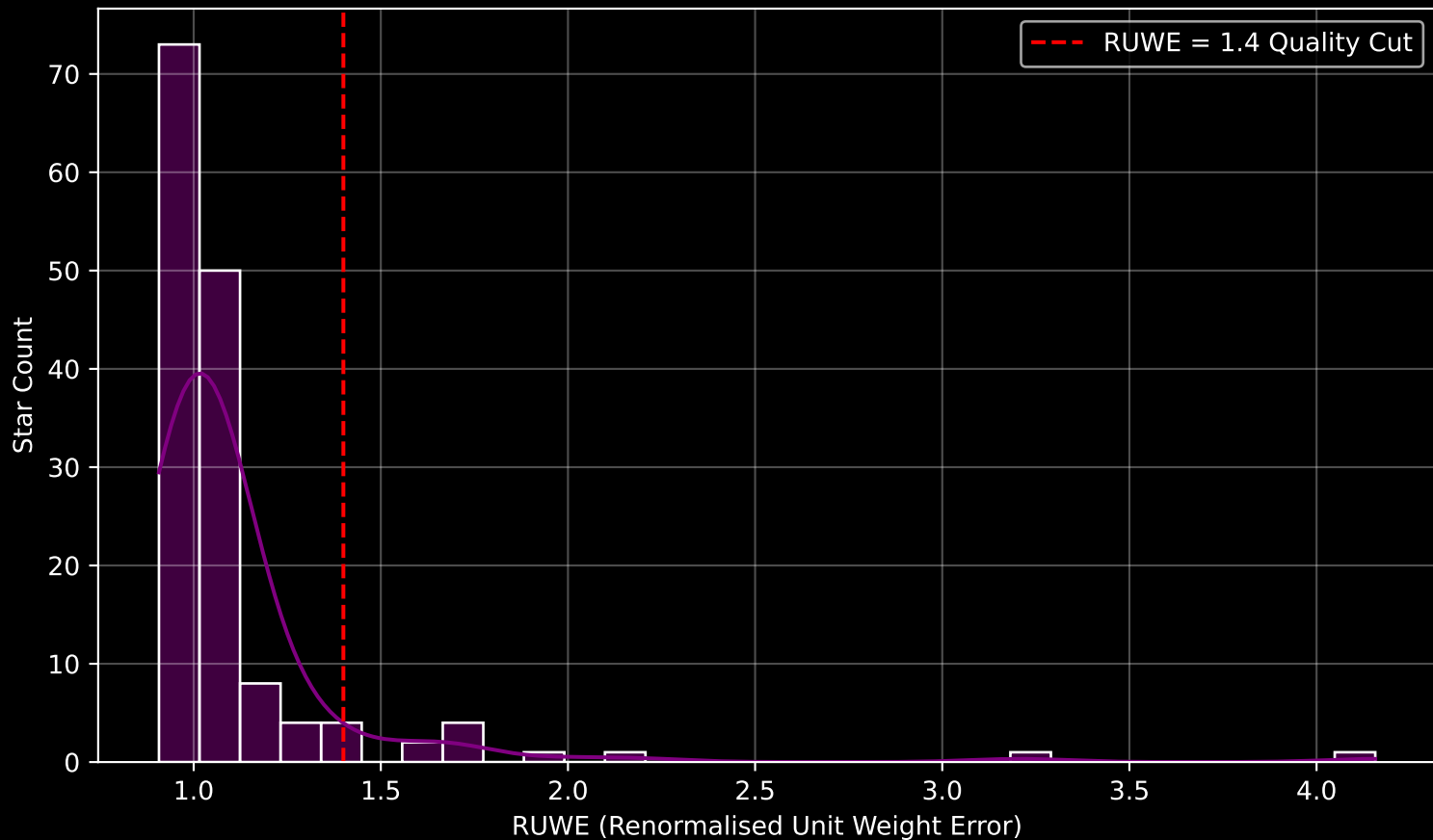
Gaia Cluster: [Gulliver_21] RUWE Distribution (n= 149)
