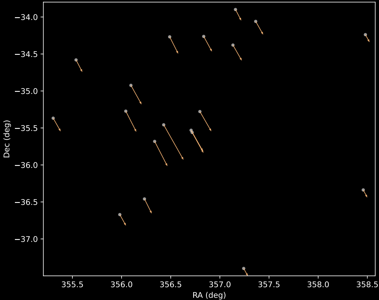
Gaia DR3 Cluster 43 Proper Motion Vectors (n=19)
