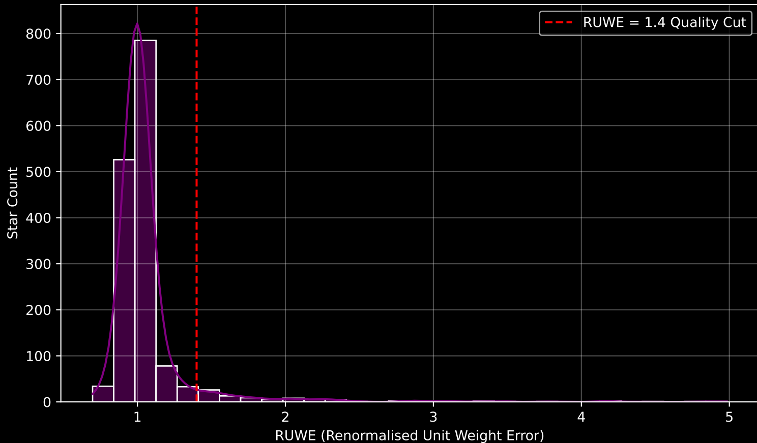
Gaia Cluster: [Gulliver_29] RUWE Distribution (n= 1543)
