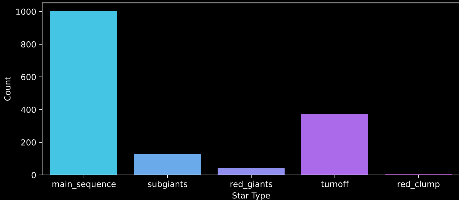
Gaia Cluster: [Gulliver_29] Count plot of Star Type
