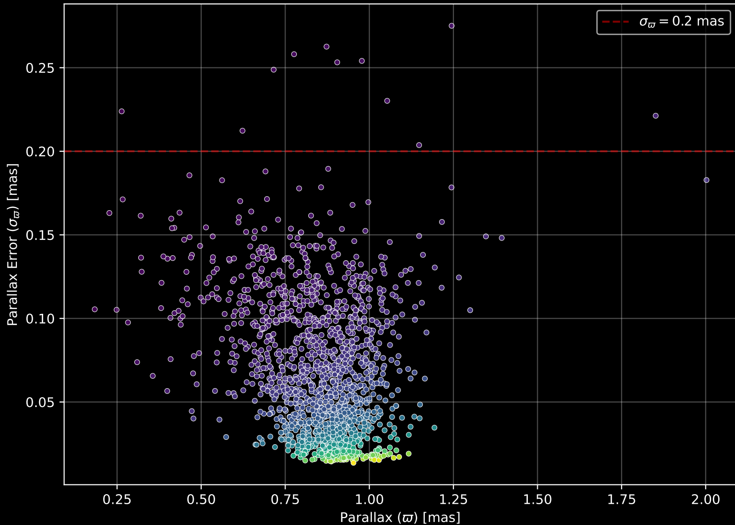
Gaia Cluster: [Gulliver_29] Parallax Quality (n= 1545)
