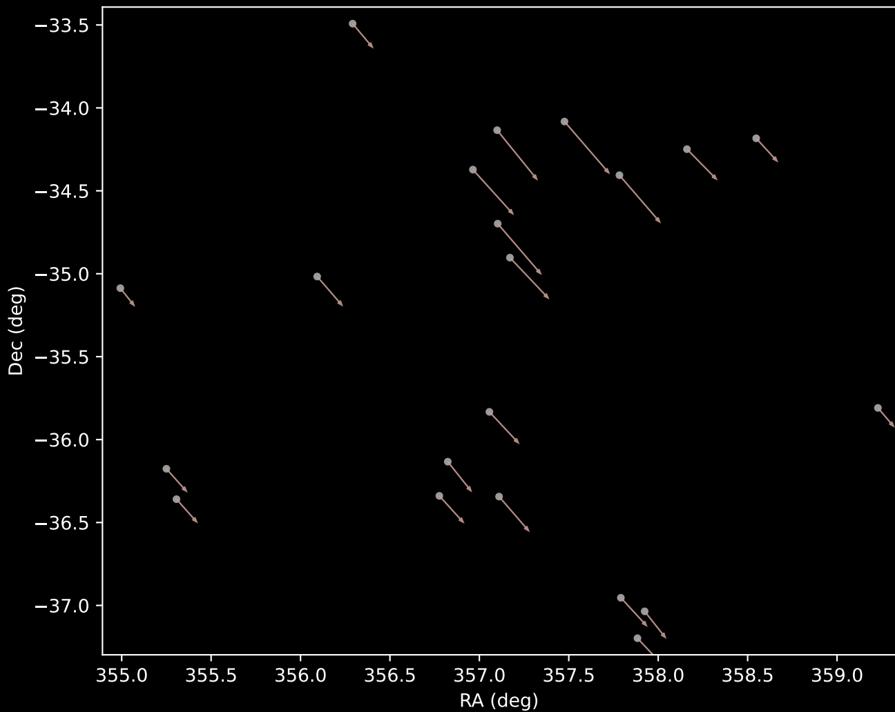
Gaia DR3 Cluster 11 Proper Motion Vectors (n=21)
