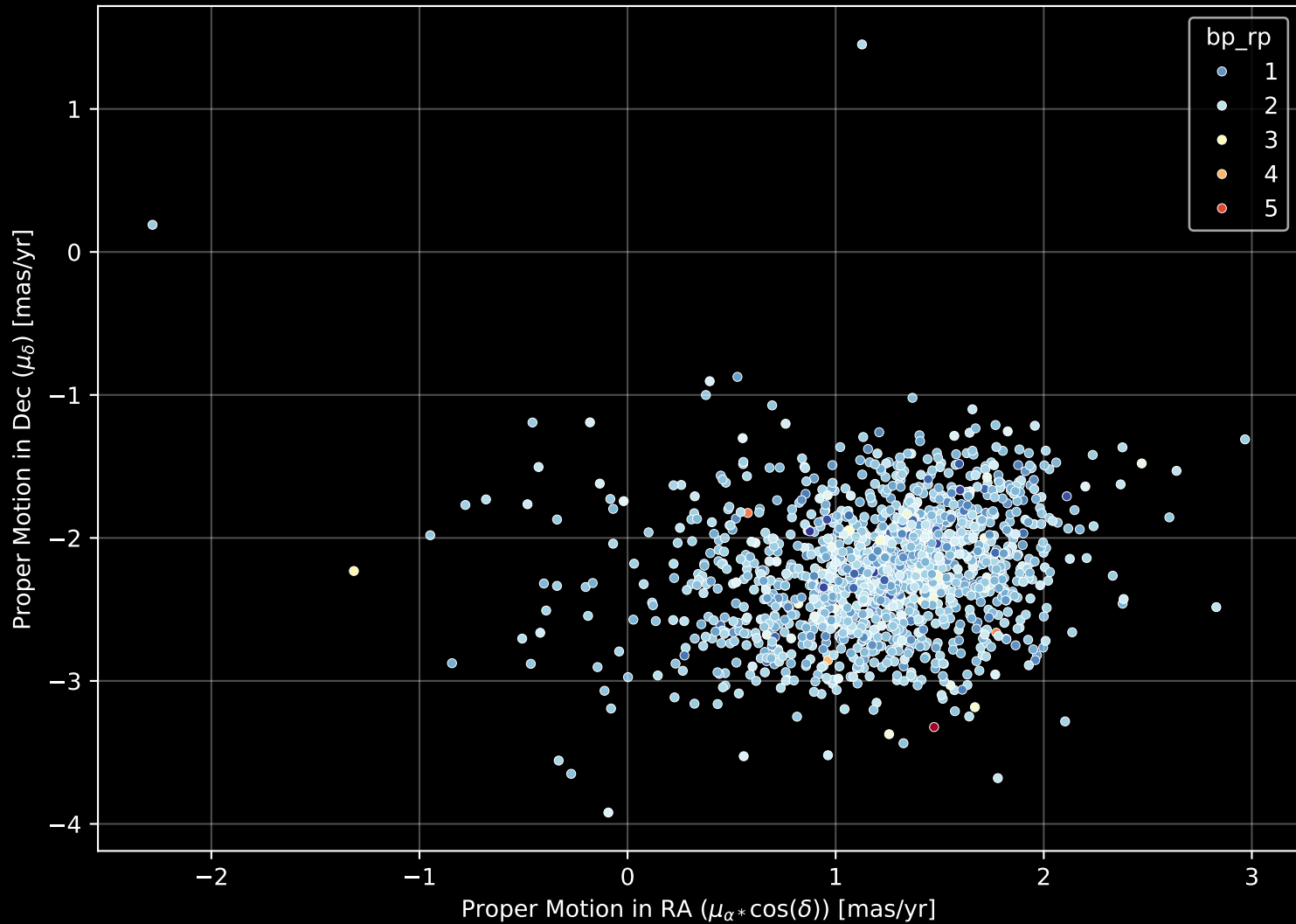
Gaia Cluster: [Gulliver_29] Proper Motion Diagram (n= 1545)
