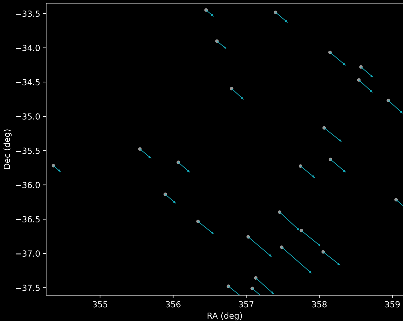
Gaia DR3 Cluster 18 Proper Motion Vectors (n=25)
