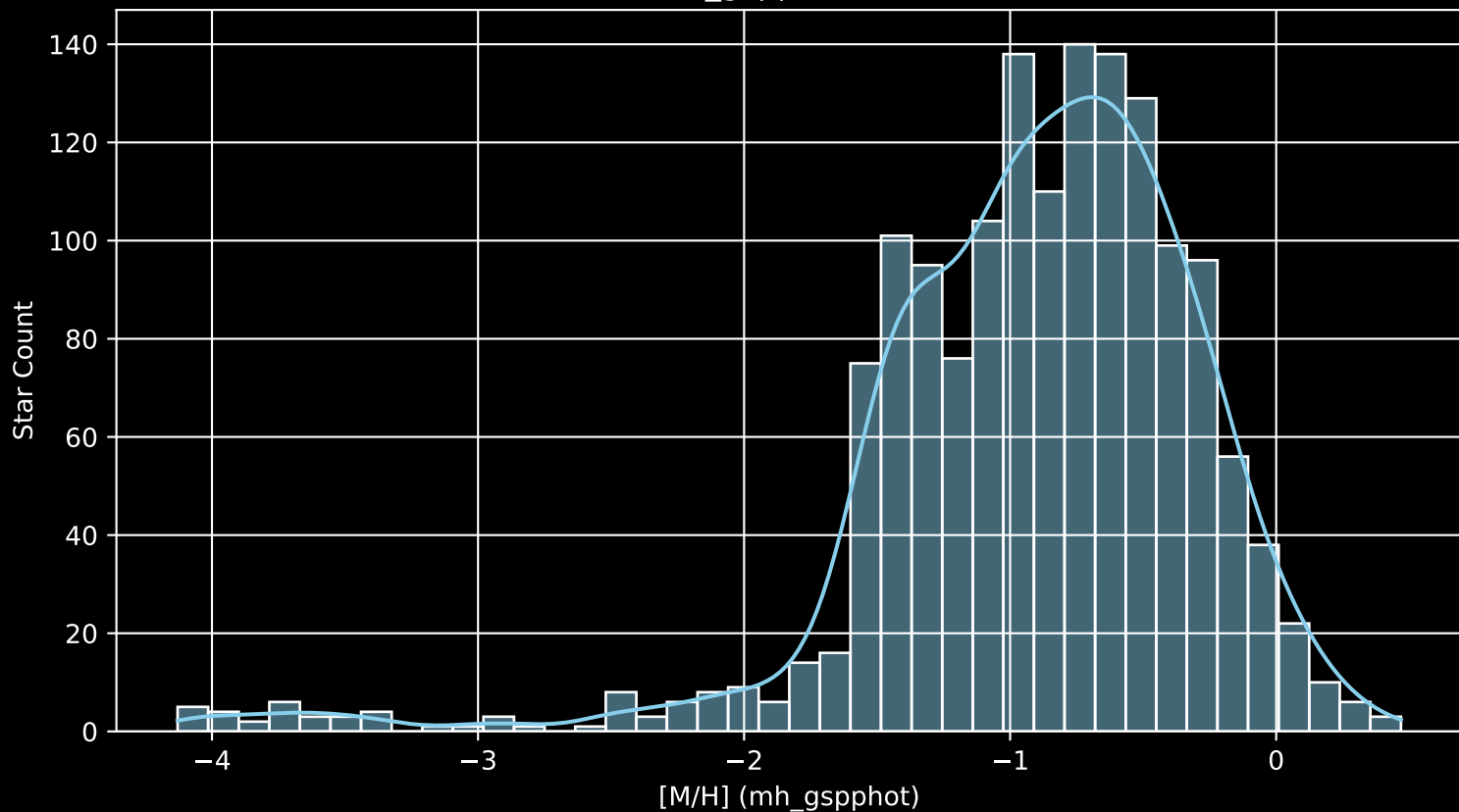
Gaia Cluster: [Gulliver_29 [M/H] (mh_gspphot) (n= 1540)
