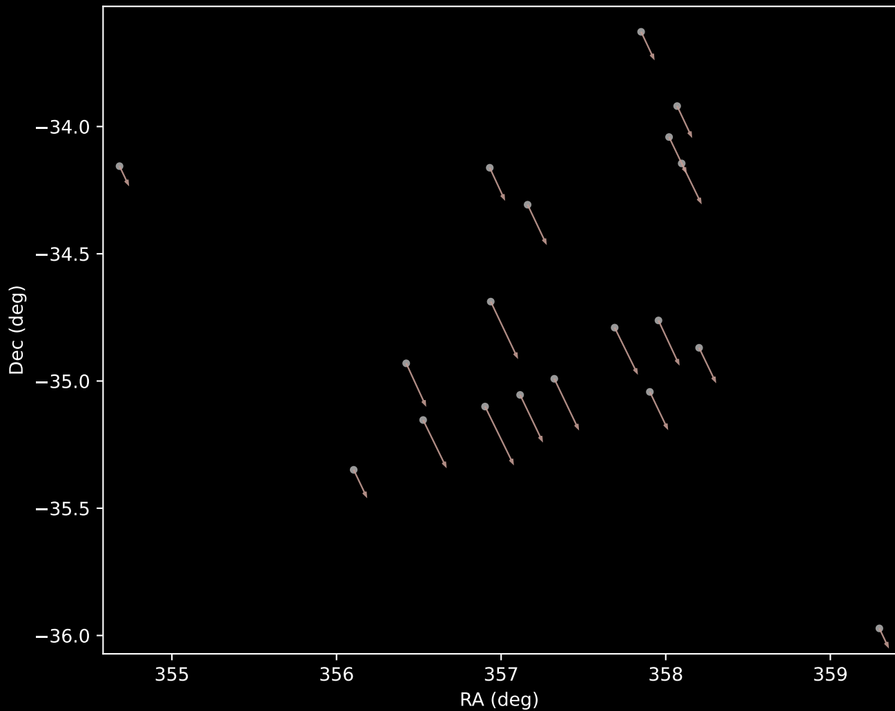
Gaia DR3 Cluster 51 Proper Motion Vectors (n=19)
