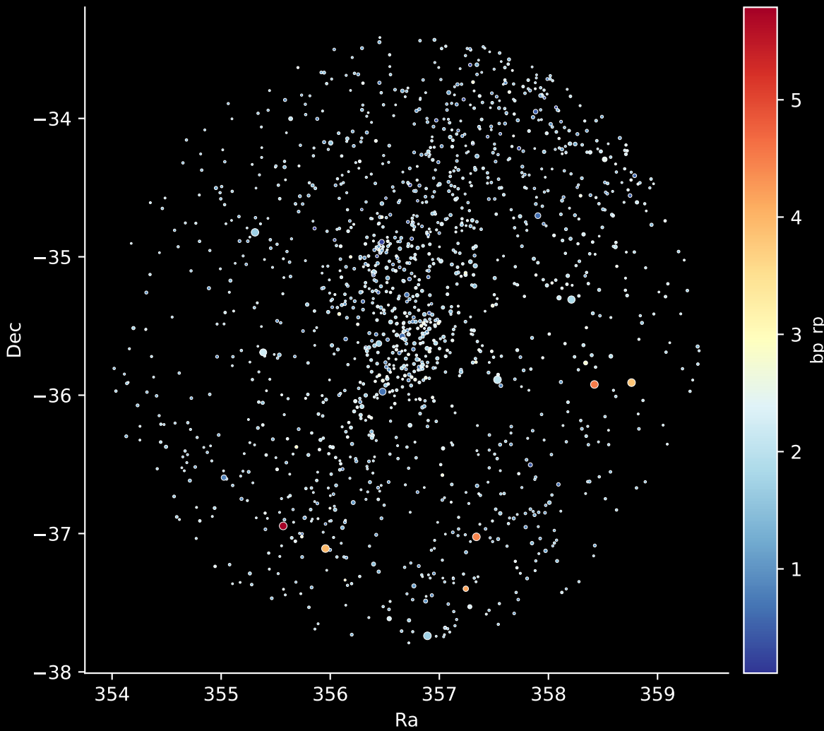
Gaia Cluster: [Gulliver_29] Stars: 1545
