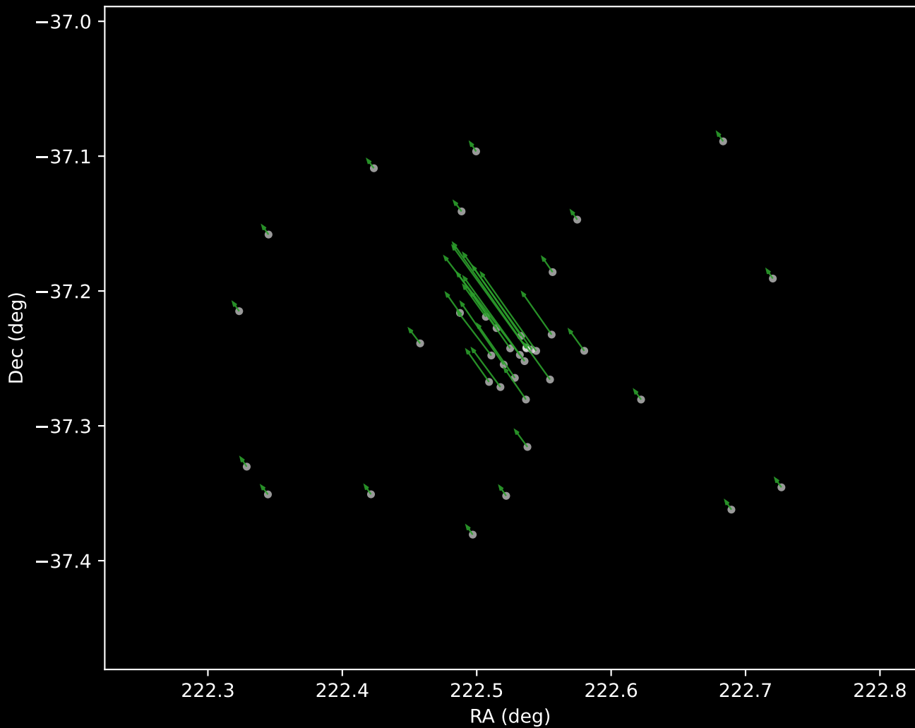
Gaia DR3 Cluster 4 Proper Motion Vectors (n=39)
