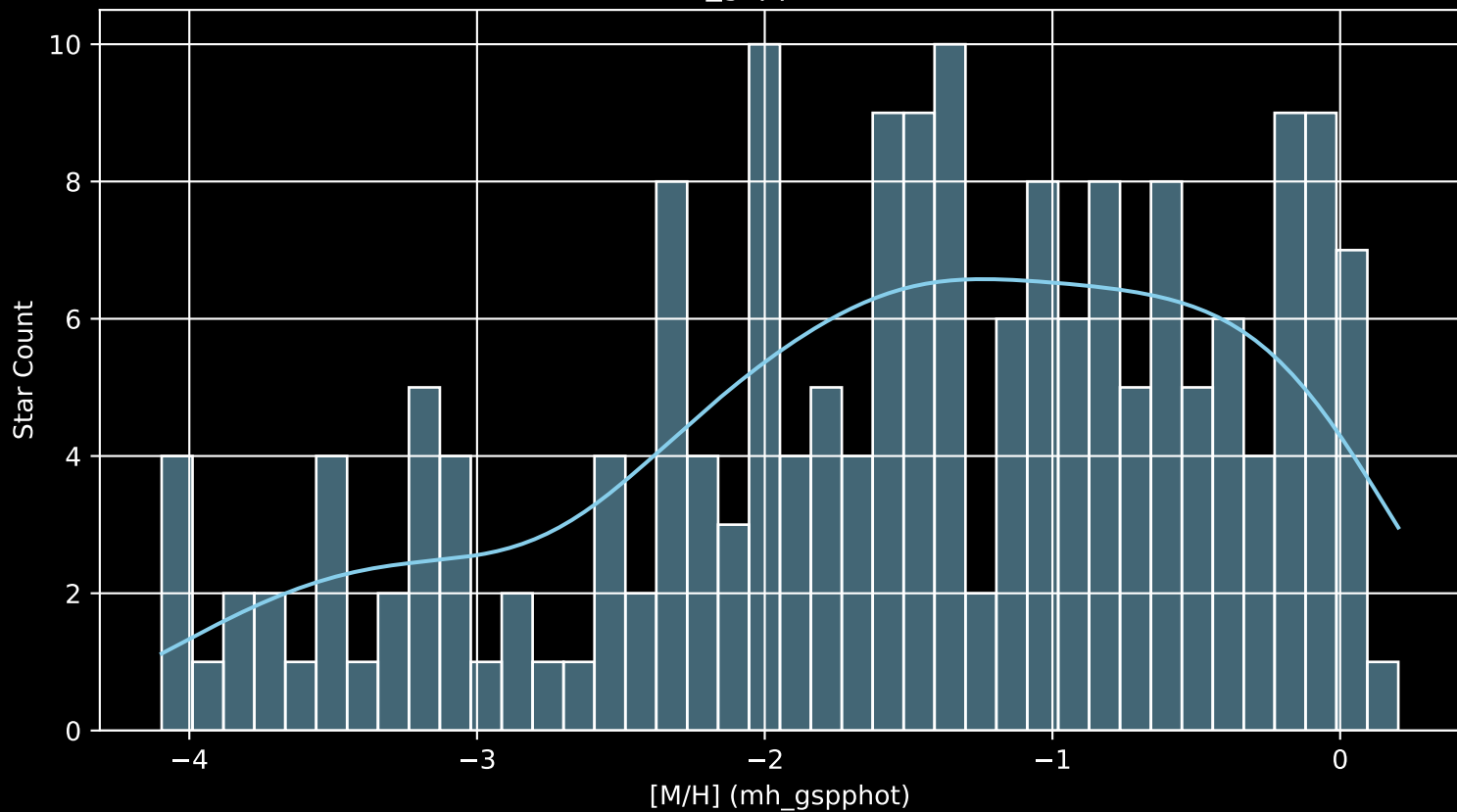
Gaia Cluster: [Gulliver_3 [M/H] (mh_gspphot) (n= 187)
