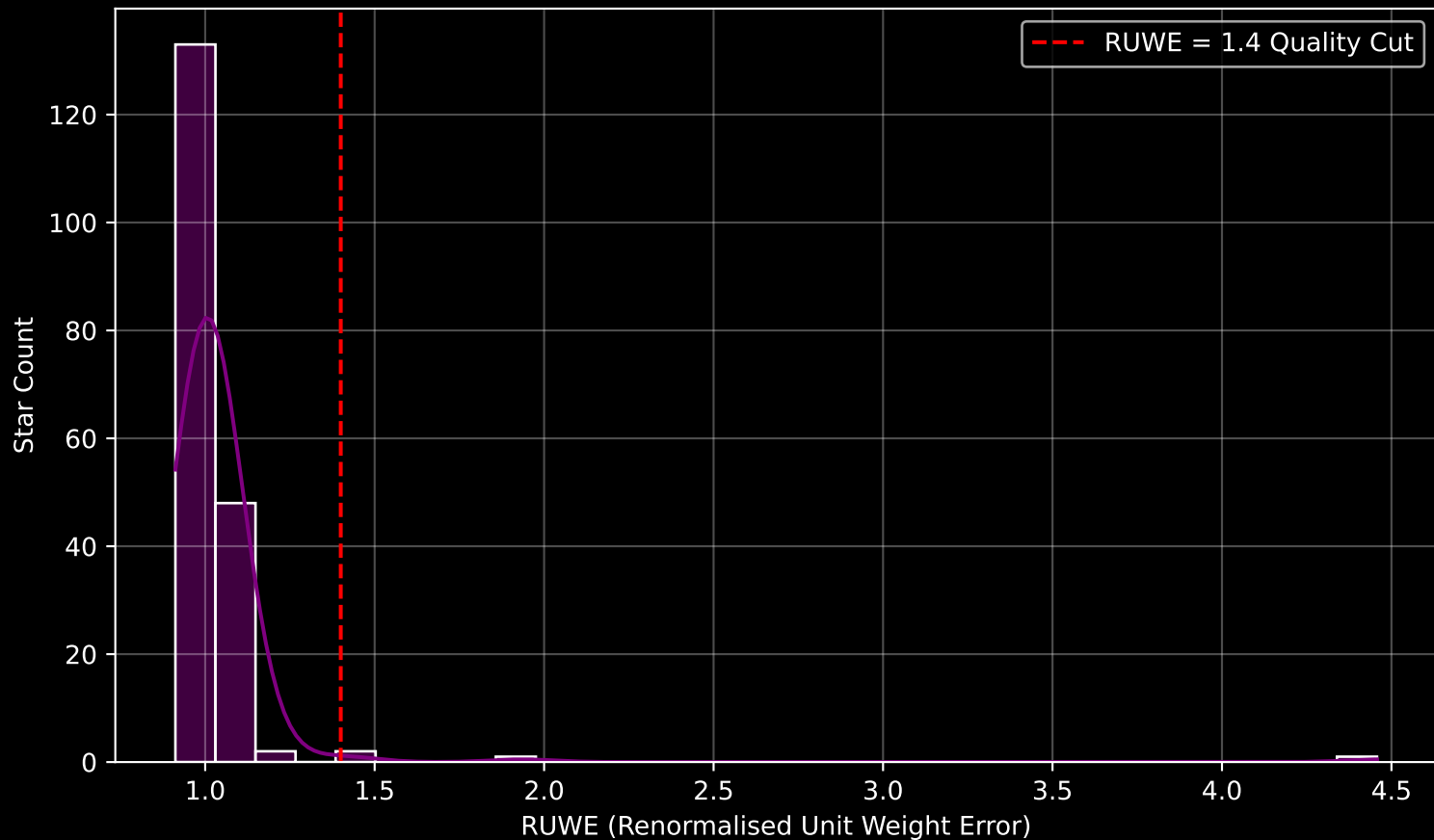
Gaia Cluster: [Gulliver_3] RUWE Distribution (n= 187)
