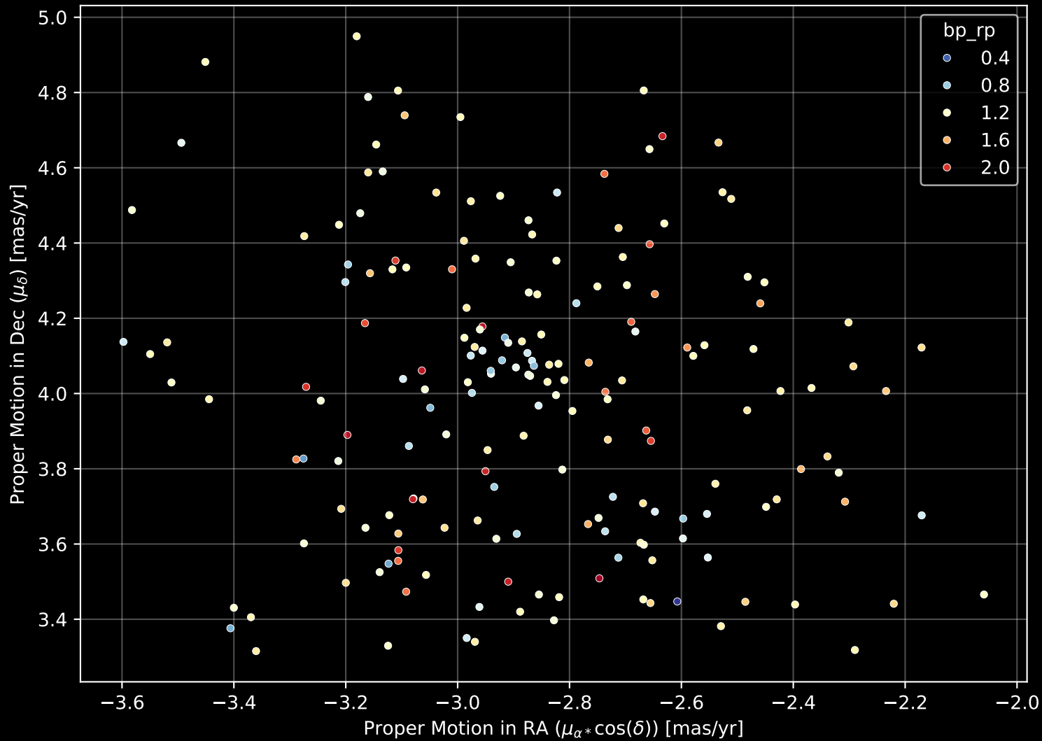
Gaia Cluster: [Gulliver_3] Proper Motion Diagram (n= 187)
