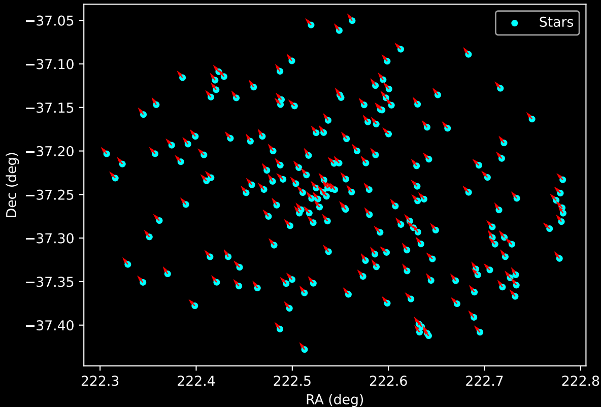
Gaia Cluster: [Gulliver_3] Proper Motion Vectors for Gaia Star Field (n= 187)
