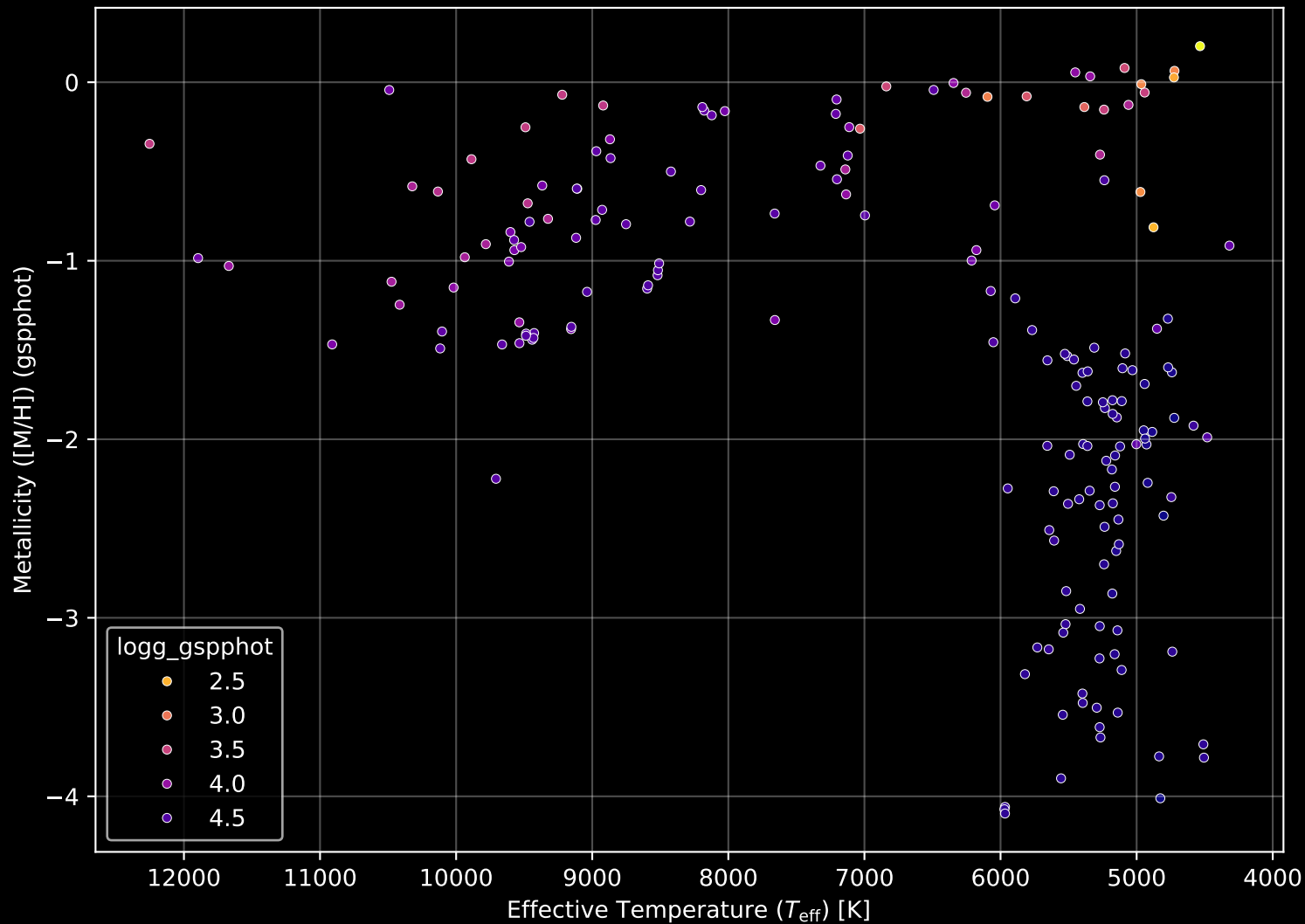
Gaia Cluster: [Gulliver_3] Stellar Population Parameters (n= 187)
