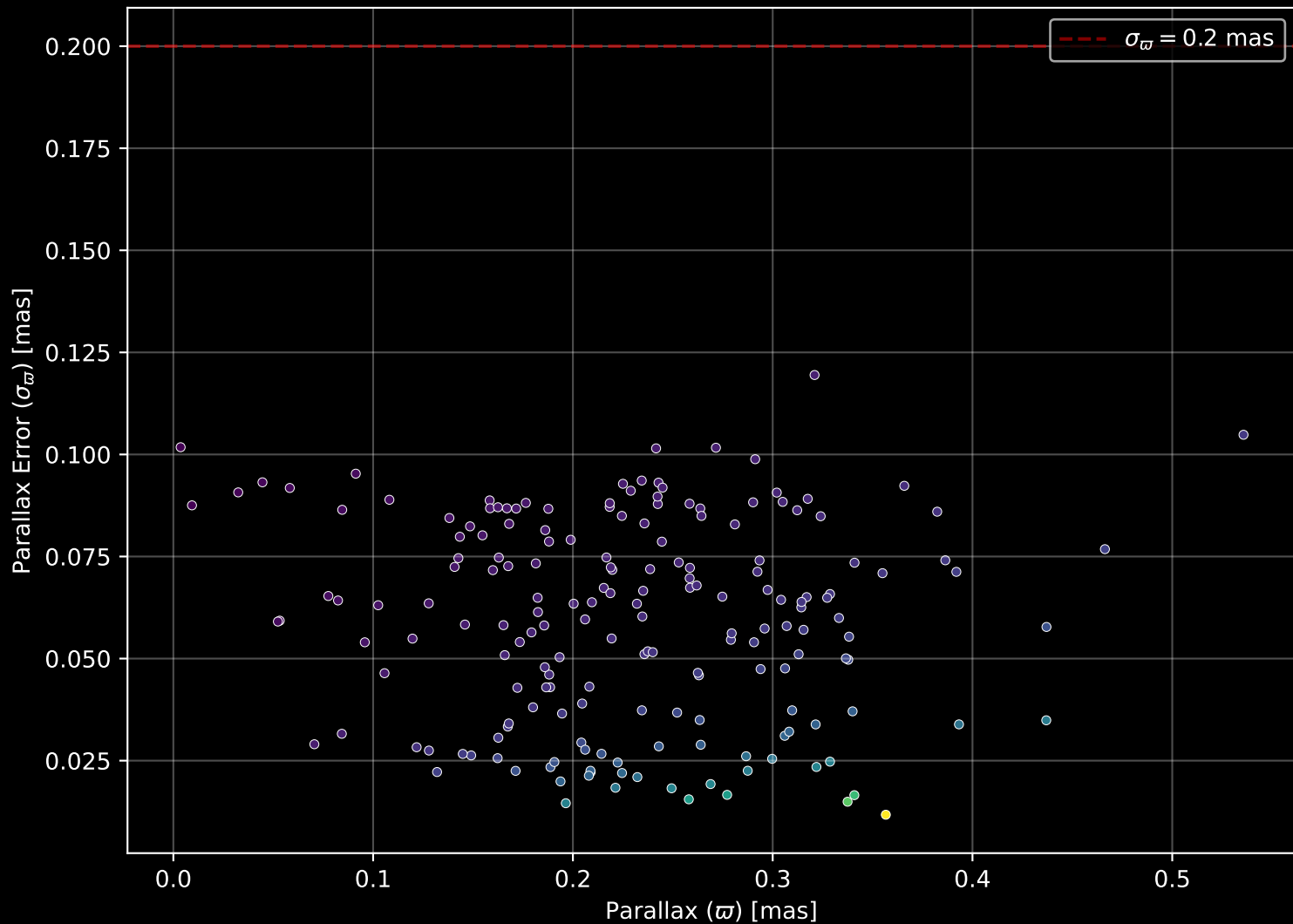
Gaia Cluster: [Gulliver_3] Parallax Quality (n= 187)
