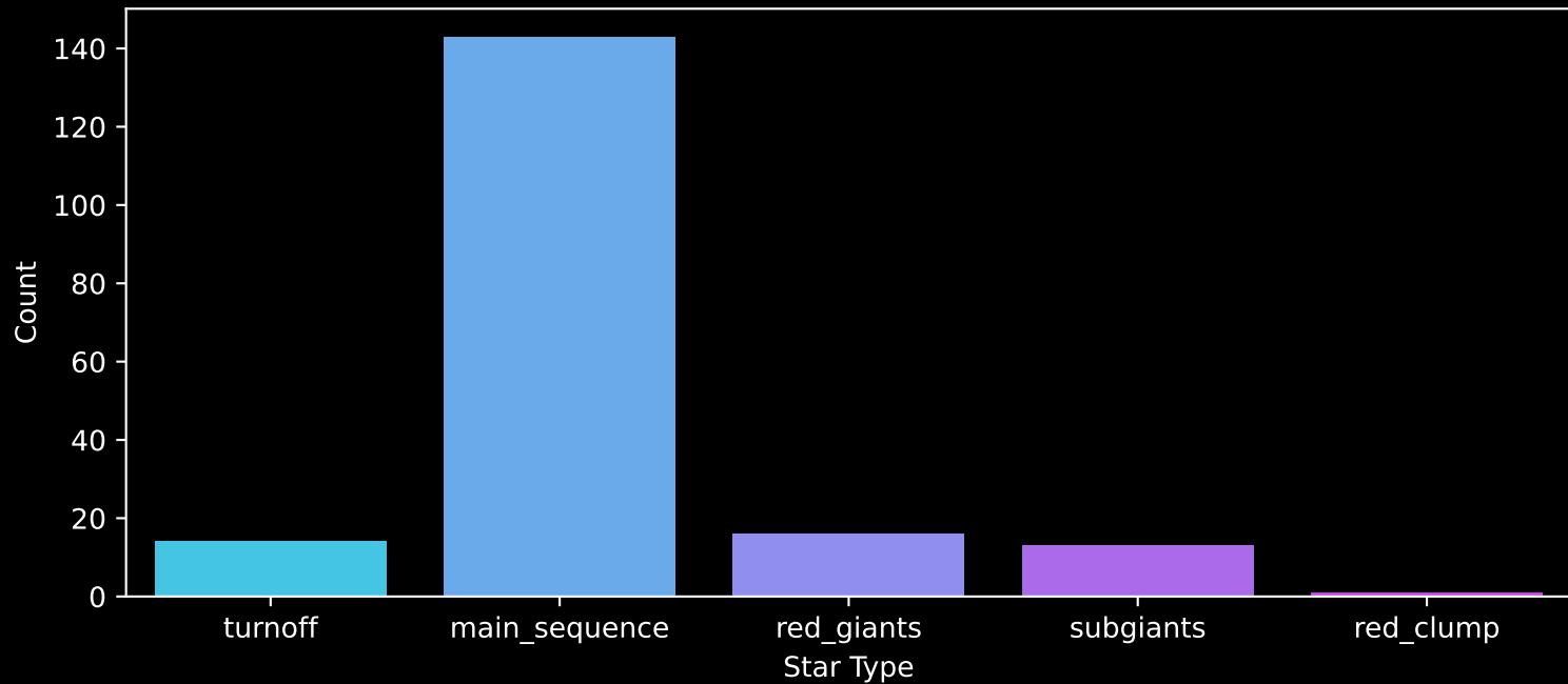
Gaia Cluster: [Gulliver_3] Count plot of Star Type
