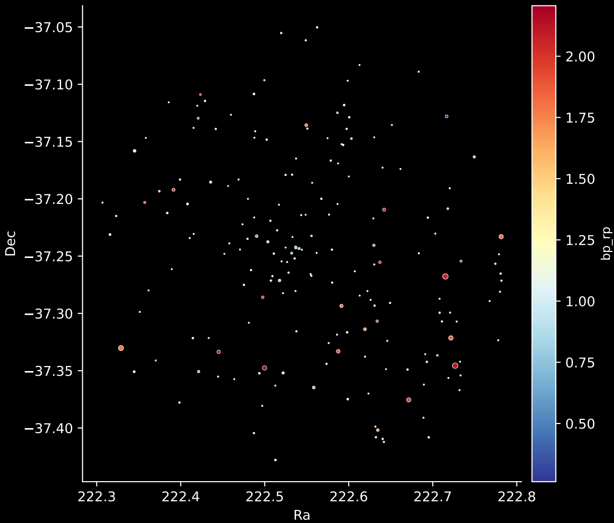
Gaia Cluster: [Gulliver_3] Stars: 187
