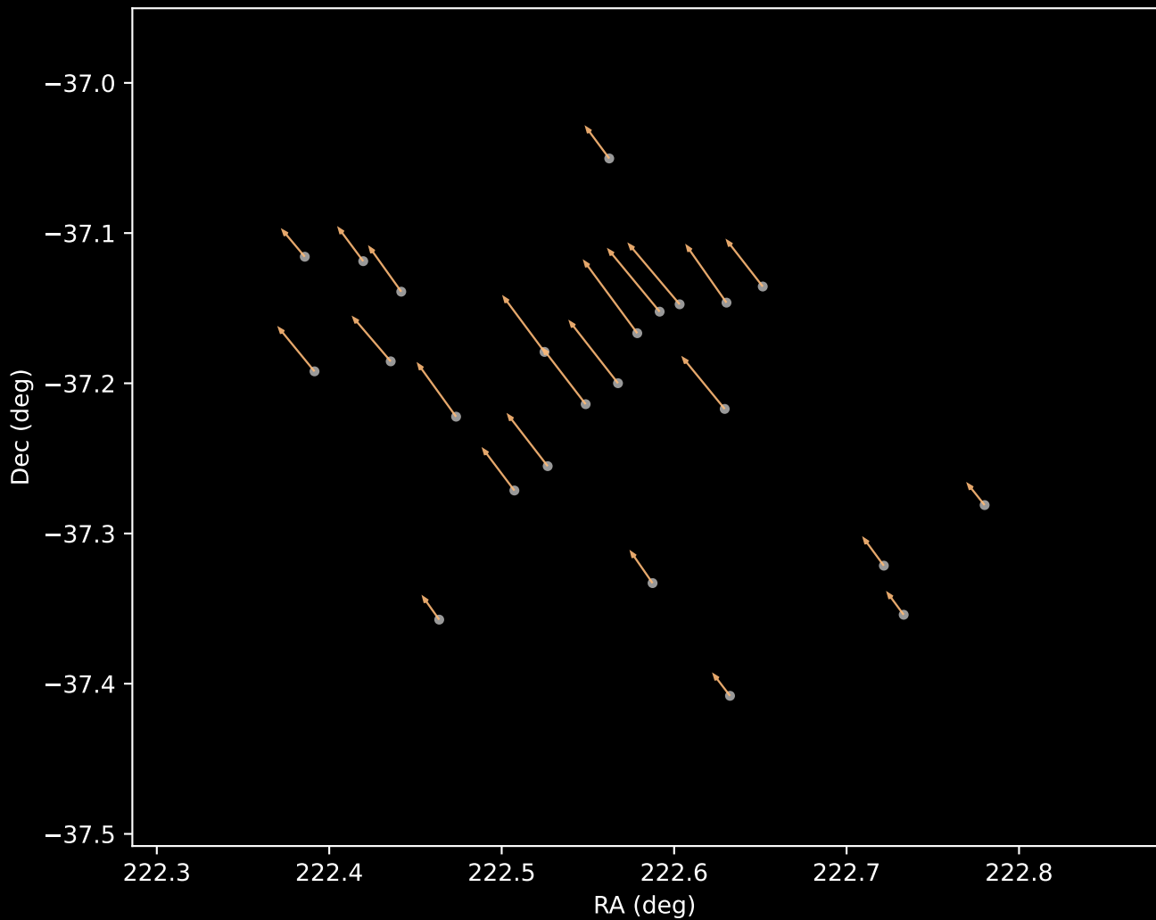
Gaia DR3 Cluster 3 Proper Motion Vectors (n=24)
