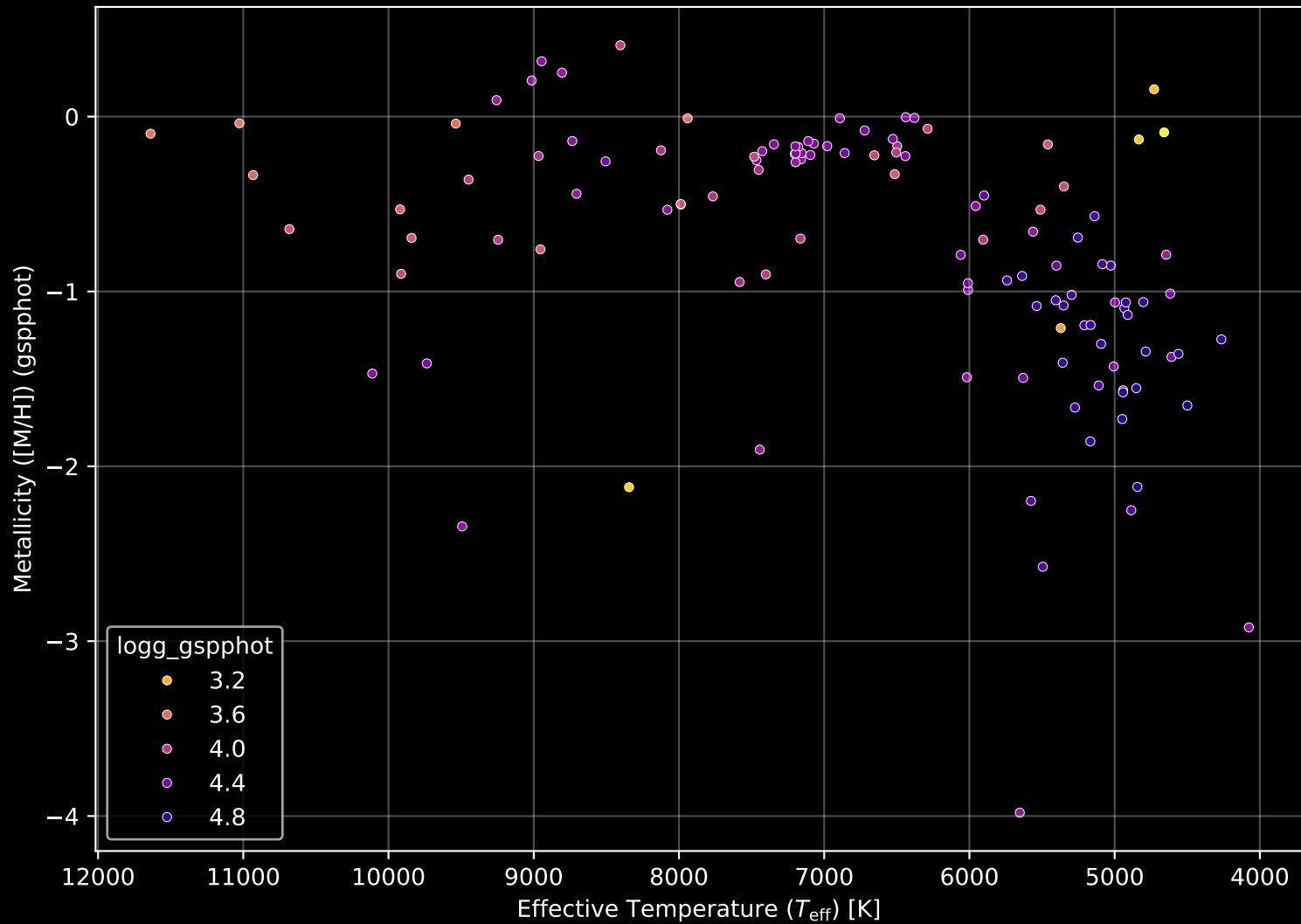
Gaia Cluster: [Gulliver_31] Stellar Population Parameters (n= 119)
