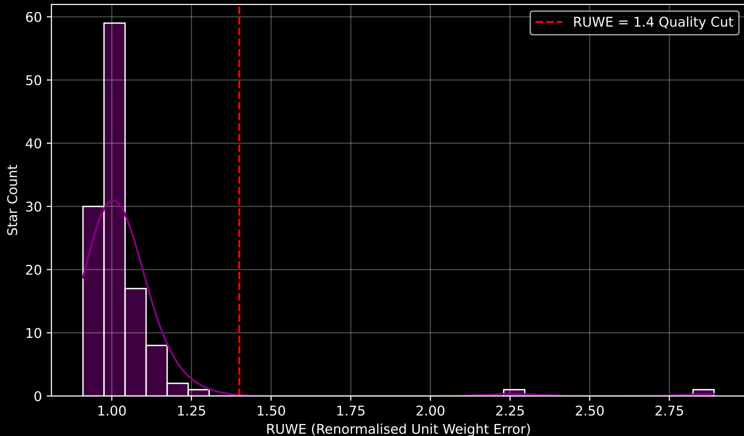
Gaia Cluster: [Gulliver_31] RUWE Distribution (n= 119)
