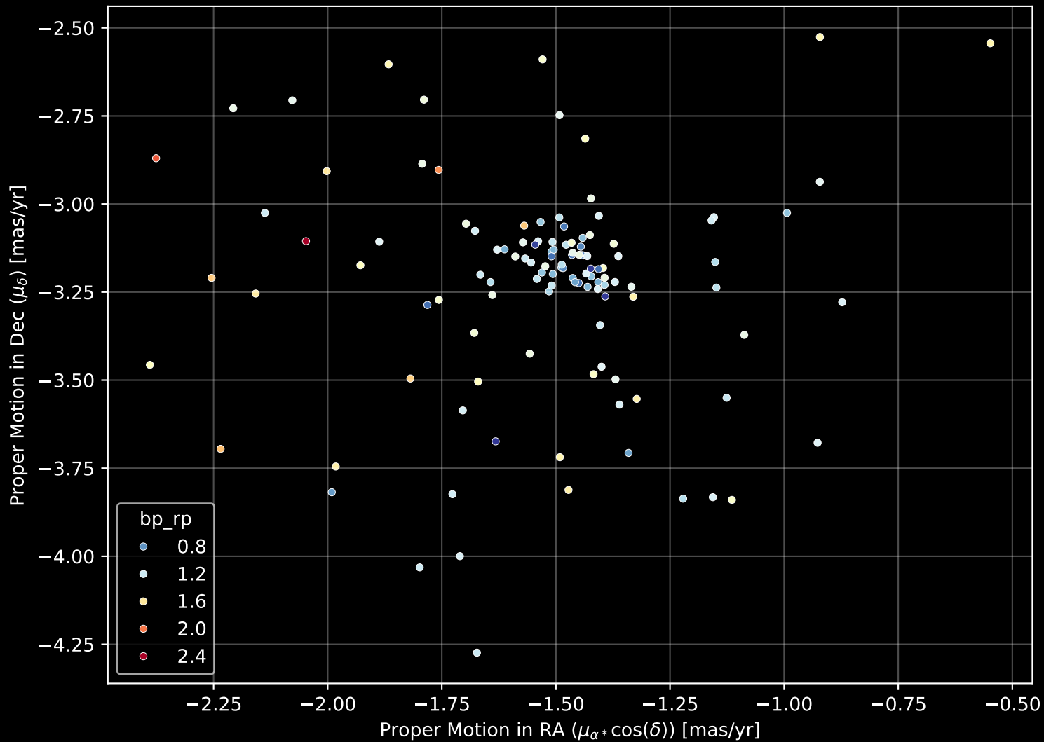
Gaia Cluster: [Gulliver_31] Proper Motion Diagram (n= 119)
