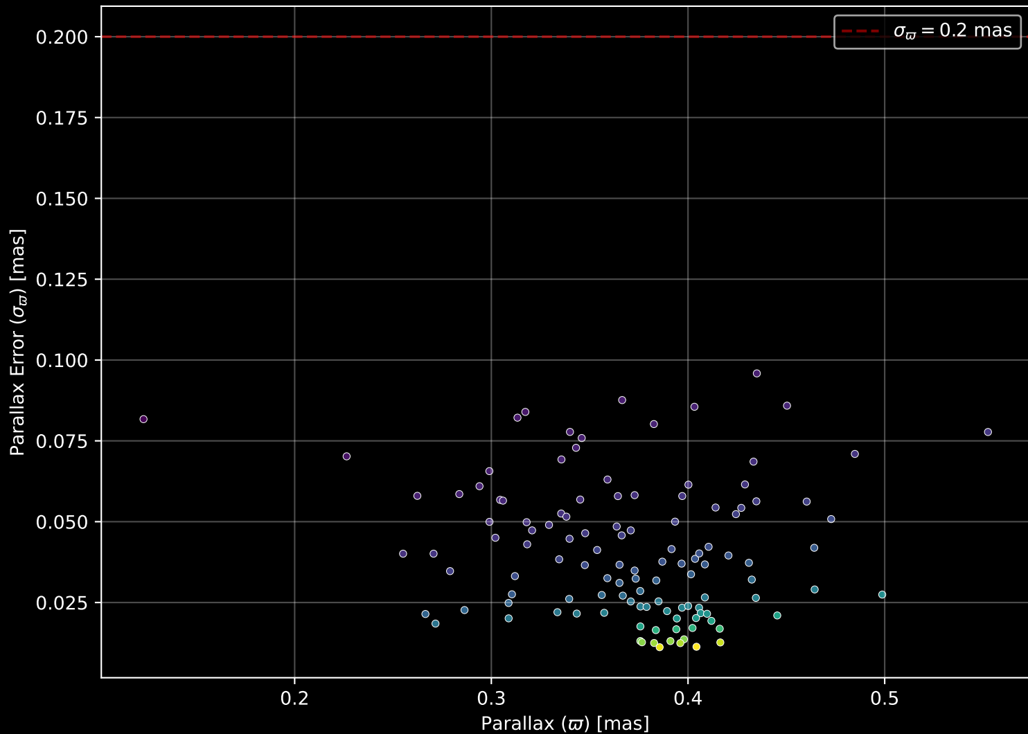
Gaia Cluster: [Gulliver_31] Parallax Quality (n= 119)
