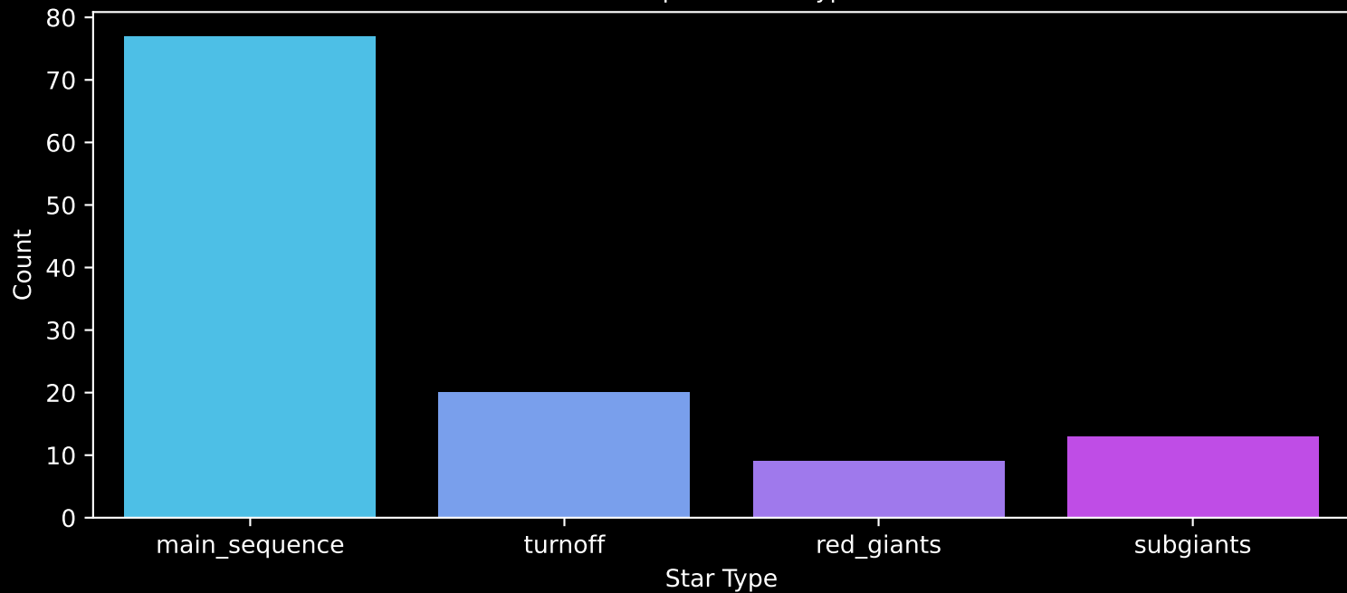
Gaia Cluster: [Gulliver_31] Count plot of Star Type
