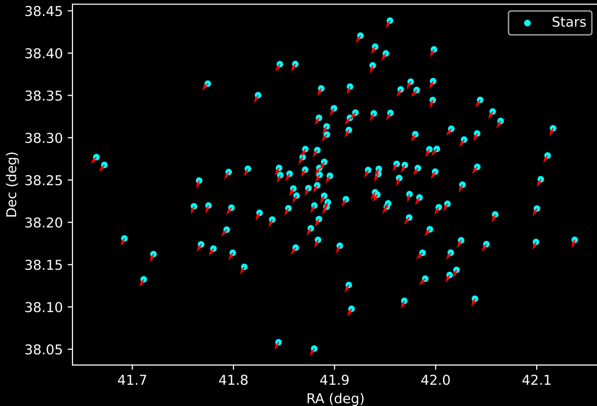
Gaia Cluster: [Gulliver_31] Proper Motion Vectors for Gaia Star Field (n= 119)
