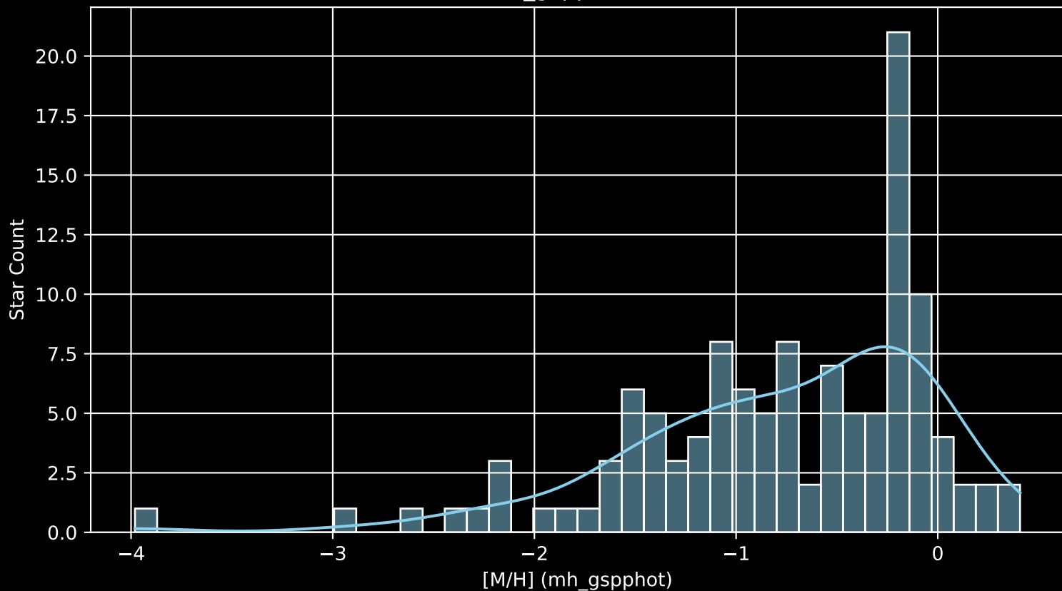
Gaia Cluster: [Gulliver_31 [M/H] (mh_gspphot) (n= 119)
