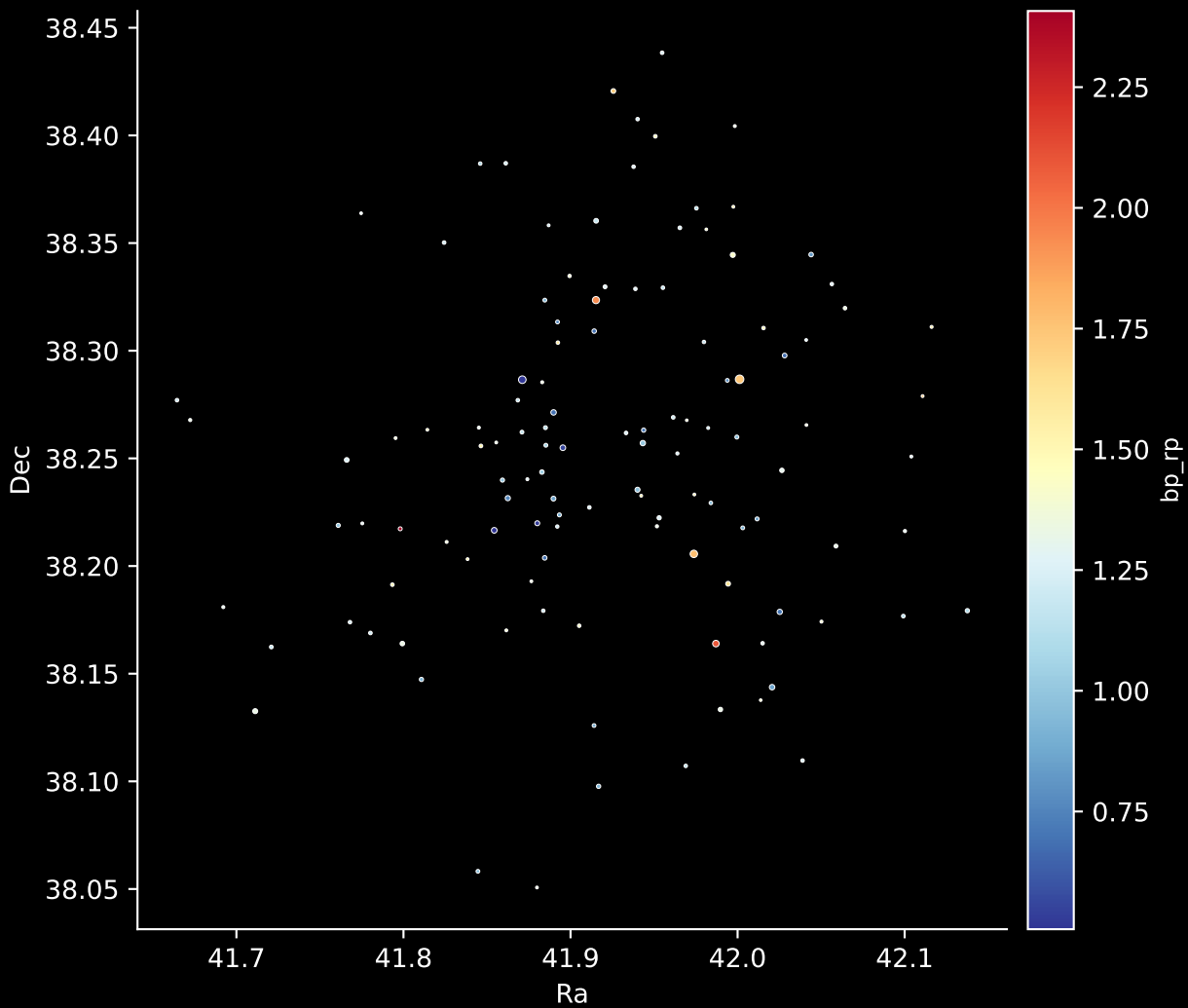
Gaia Cluster: [Gulliver_31] Stars: 119
