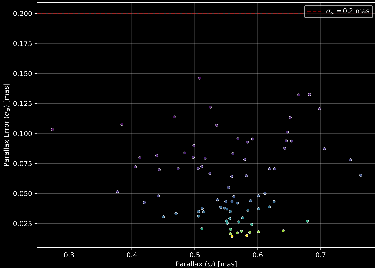
Gaia Cluster: [Gulliver_32] Parallax Quality (n= 81)
