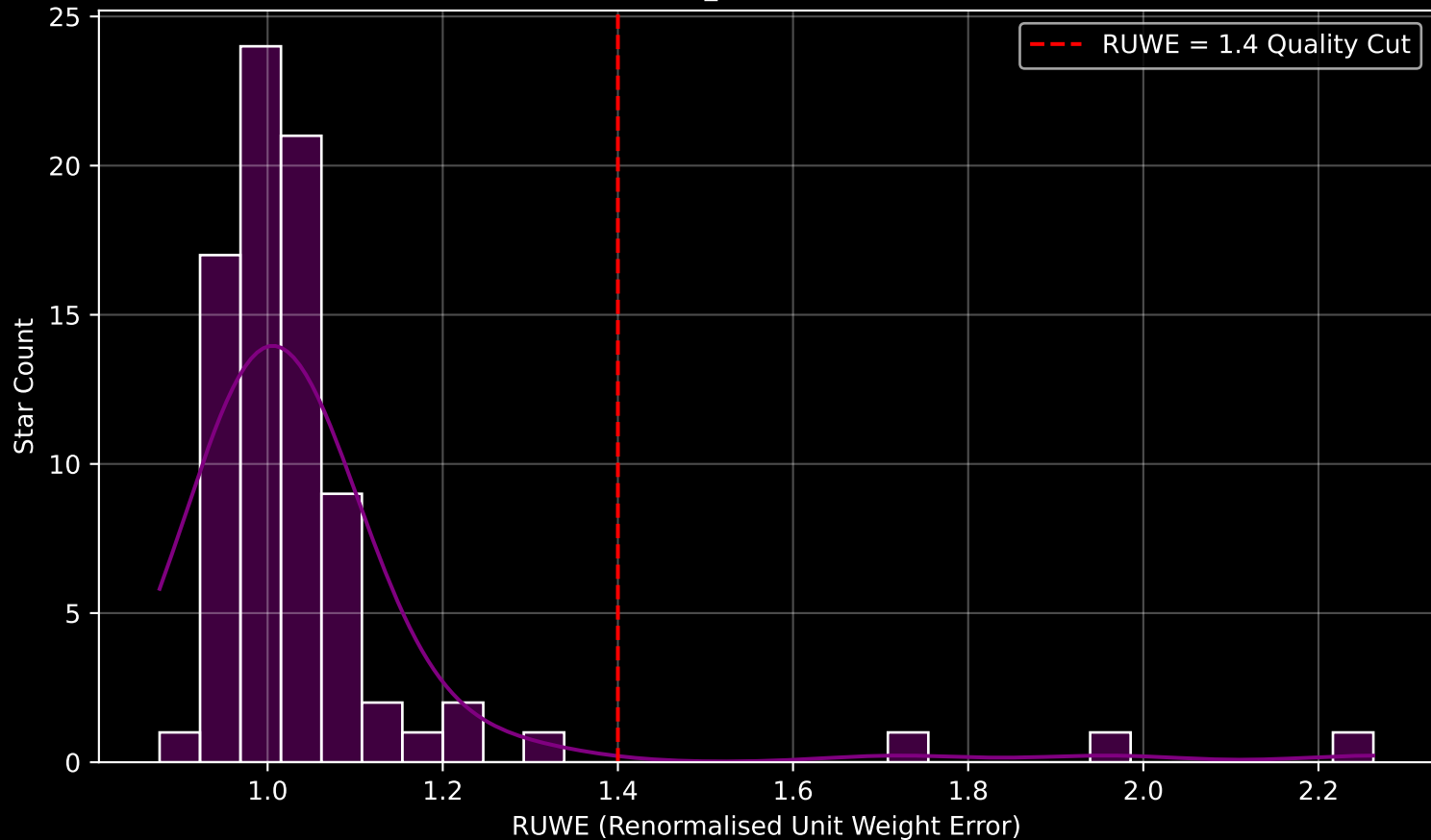
Gaia Cluster: [Gulliver_32] RUWE Distribution (n= 81)
