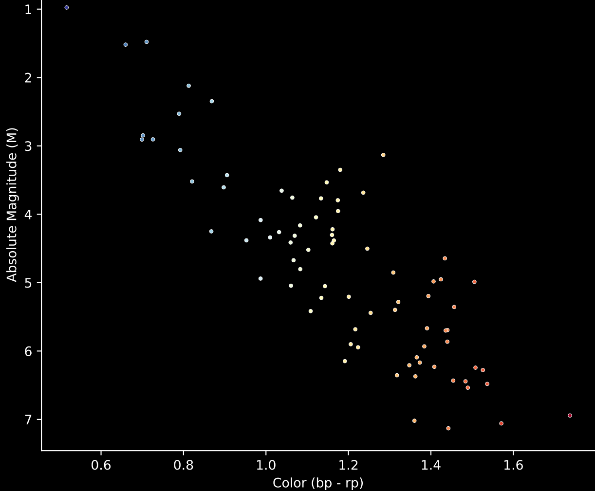
Gaia Cluster: [Gulliver_32] Stars (n= 81) Hertzprung-Russel Diagram
