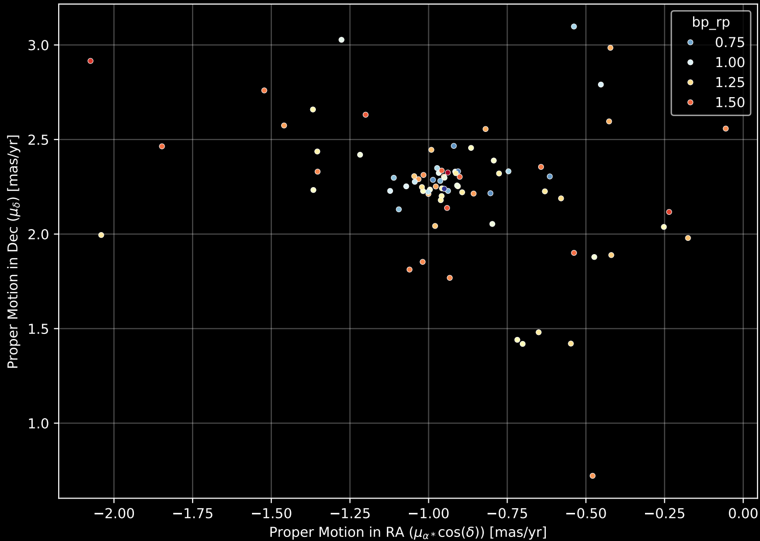
Gaia Cluster: [Gulliver_32] Proper Motion Diagram (n= 81)
