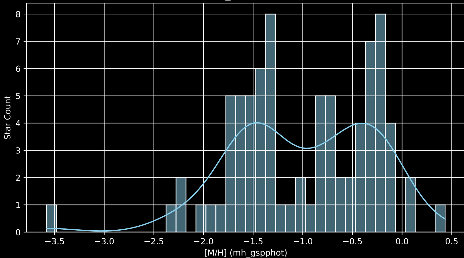
Gaia Cluster: [Gulliver_32 [M/H] (mh_gspphot) (n= 81)
