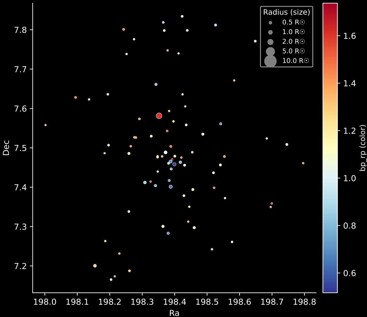
Gaia Cluster: [Gulliver_32] Stars: 81
