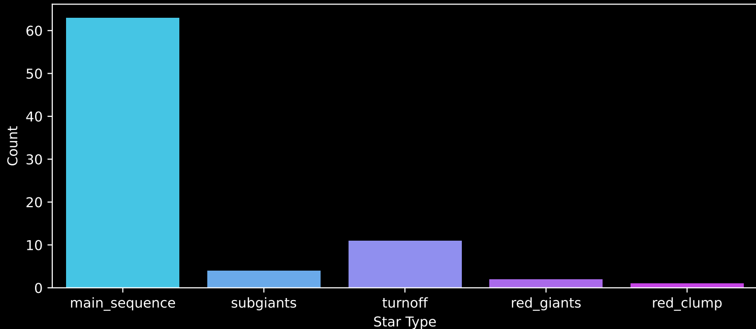
Gaia Cluster: [Gulliver_32] Count plot of Star Type
