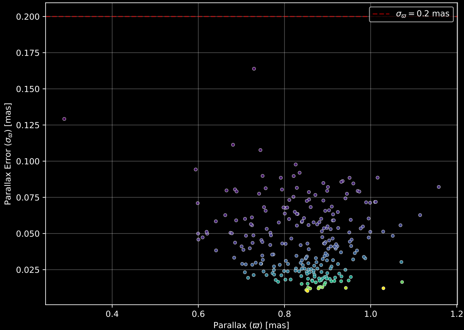
Gaia Cluster: [Gulliver_33] Parallax Quality (n= 249)
