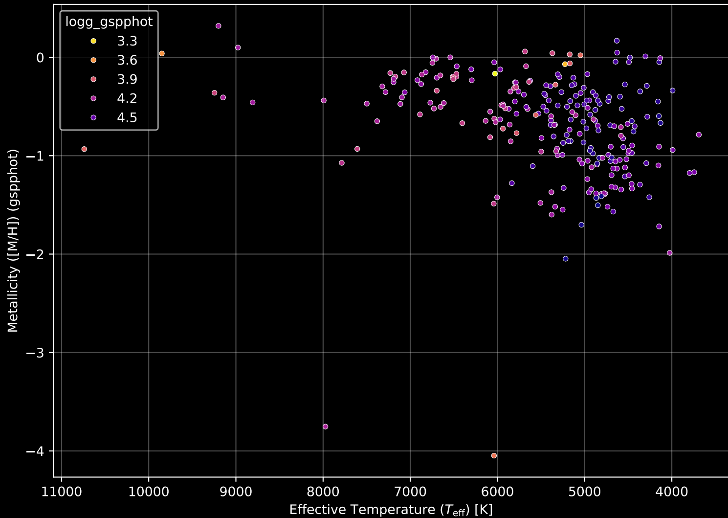
Gaia Cluster: [Gulliver_33] Stellar Population Parameters (n= 249)
