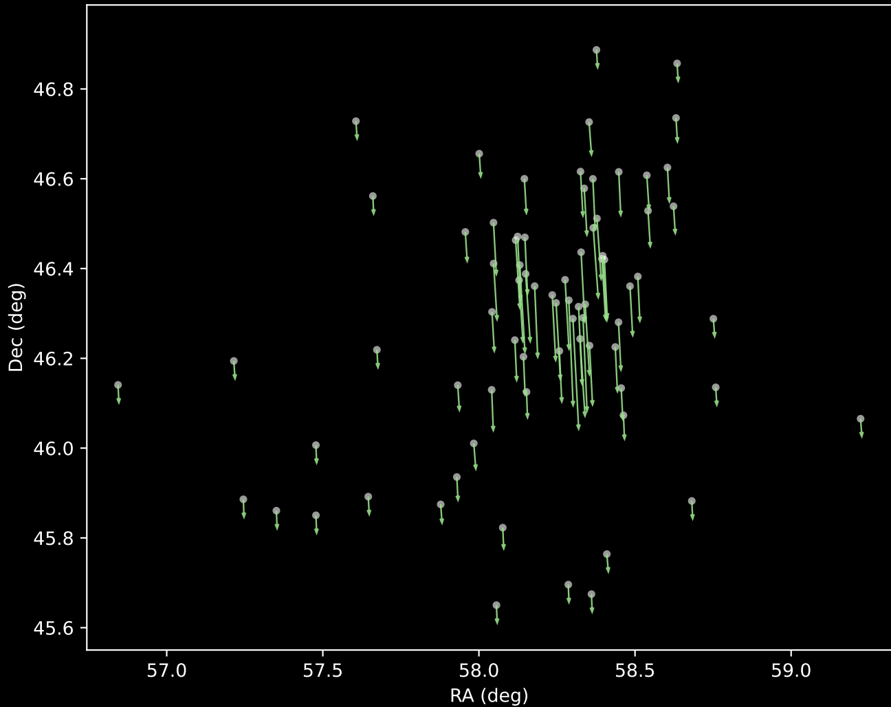
Gaia DR3 Cluster 5 Proper Motion Vectors (n=75)
