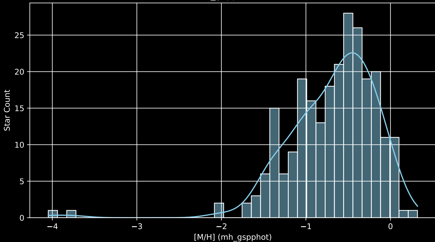
Gaia Cluster: [Gulliver_33 [M/H] (mh_gspphot) (n= 249)
