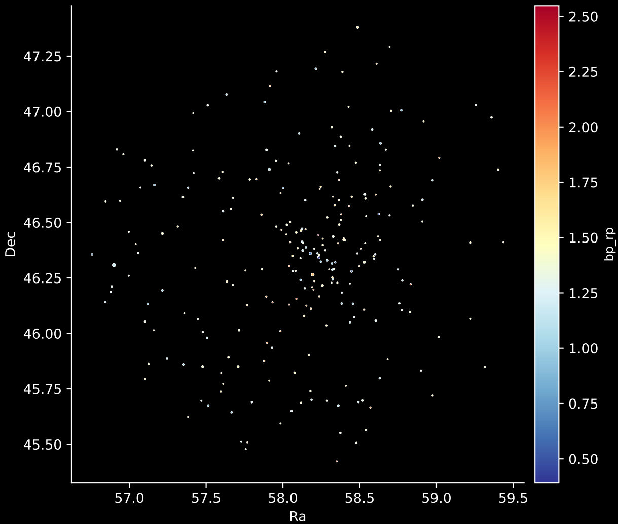
Gaia Cluster: [Gulliver_33] Stars: 249
