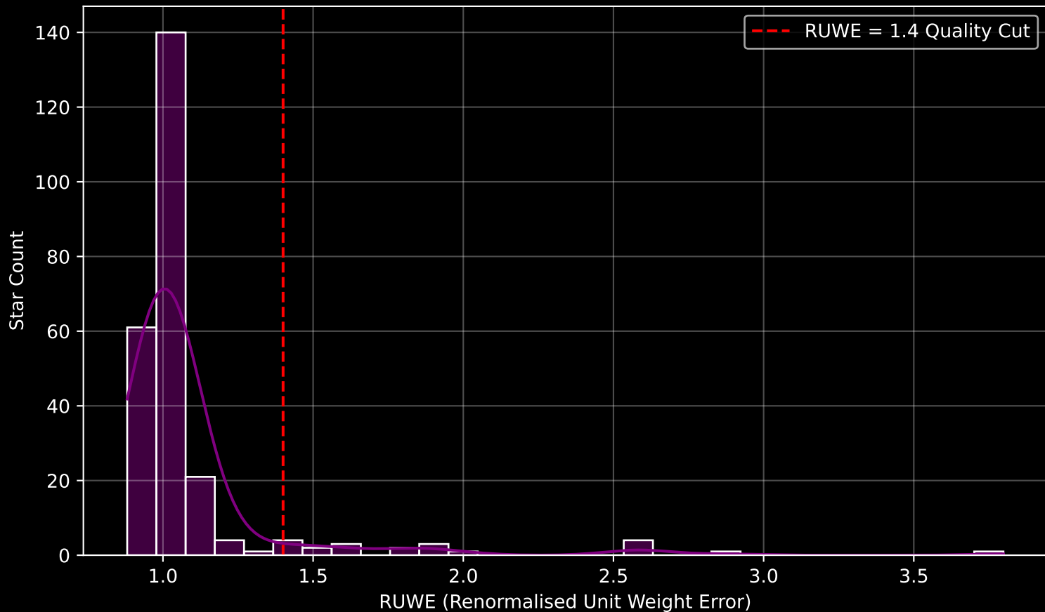
Gaia Cluster: [Gulliver_33] RUWE Distribution (n= 248)
