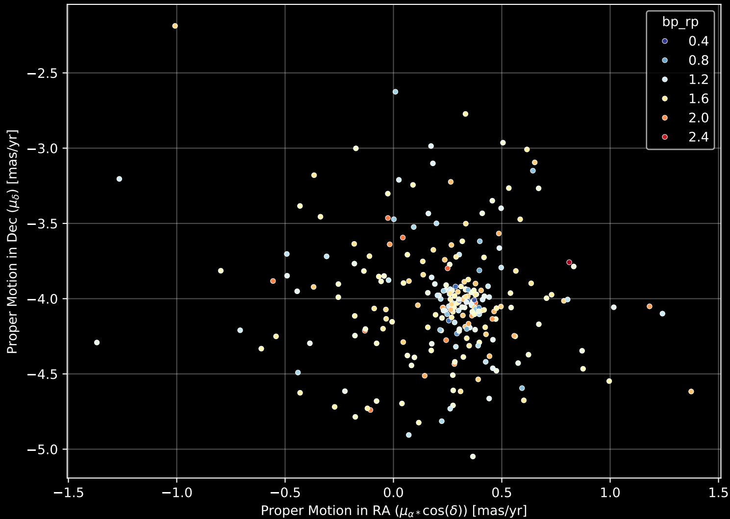
Gaia Cluster: [Gulliver_33] Proper Motion Diagram (n= 249)
