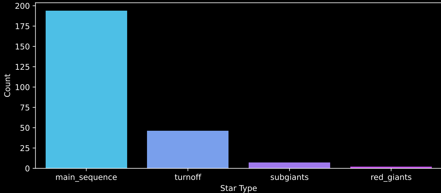
Gaia Cluster: [Gulliver_33] Count plot of Star Type
