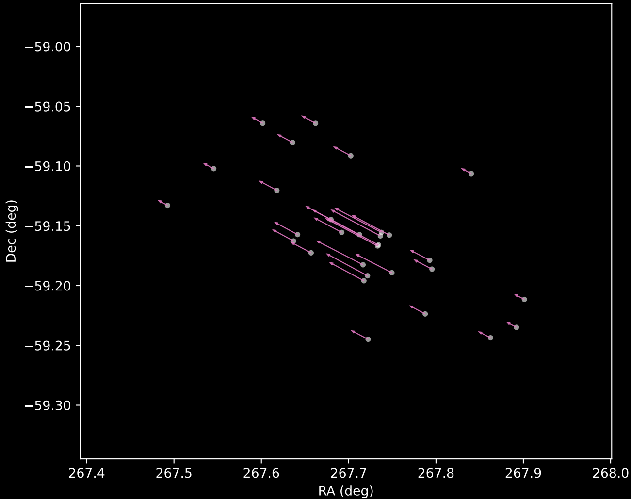
Gaia DR3 Cluster 12 Proper Motion Vectors (n=30)
