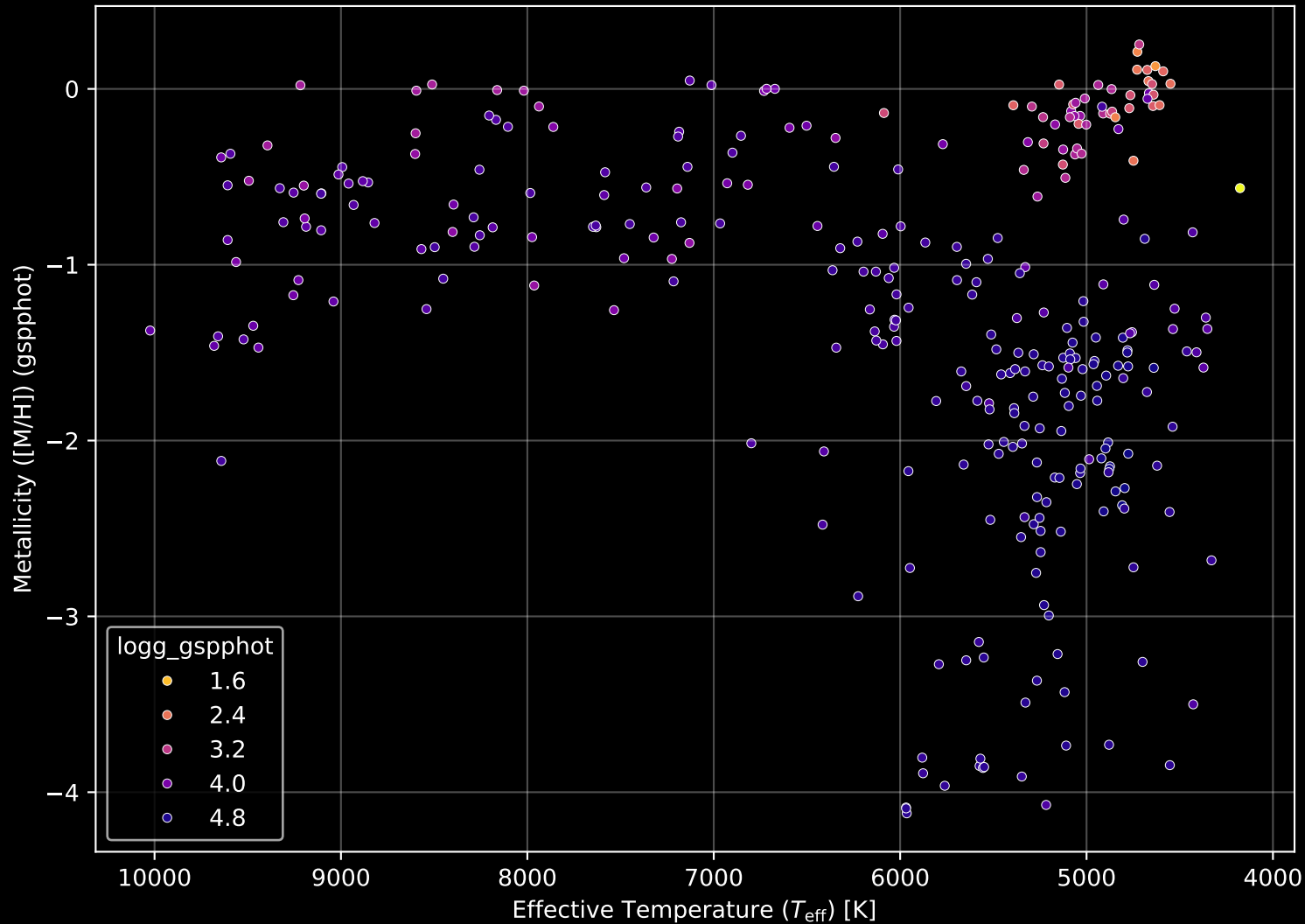
Gaia Cluster: [Gulliver_34] Stellar Population Parameters (n= 315)
