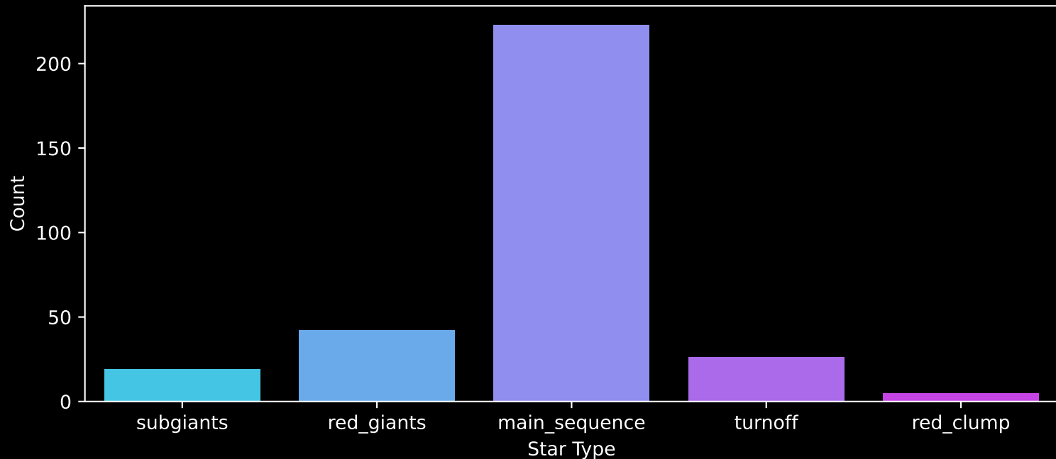
Gaia Cluster: [Gulliver_34] Count plot of Star Type
