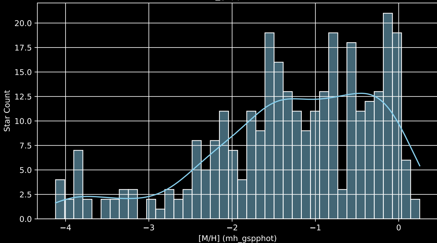
Gaia Cluster: [Gulliver_34 [M/H] (mh_gspphot) (n= 315)
