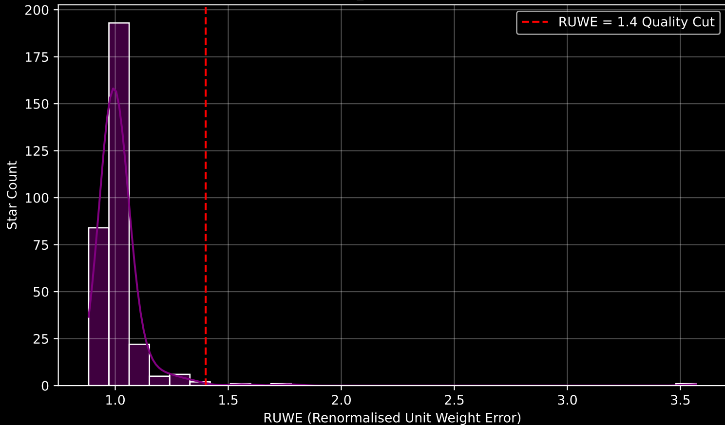
Gaia Cluster: [Gulliver_34] RUWE Distribution (n= 315)
