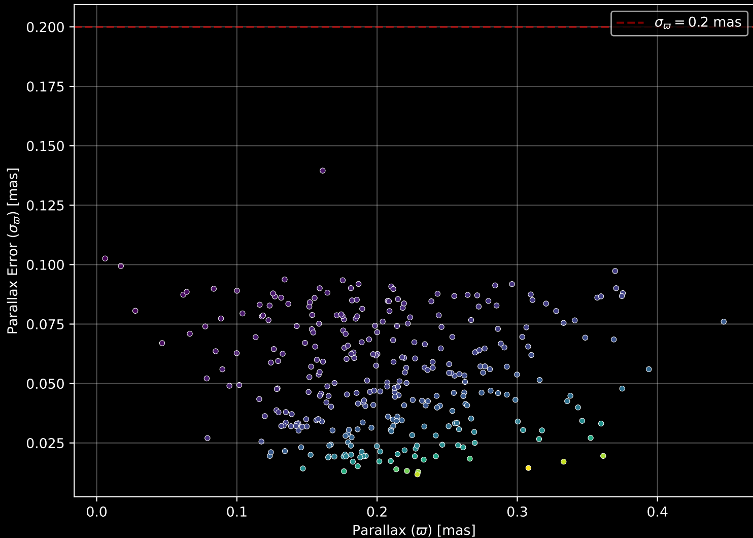
Gaia Cluster: [Gulliver_34] Parallax Quality (n= 315)
