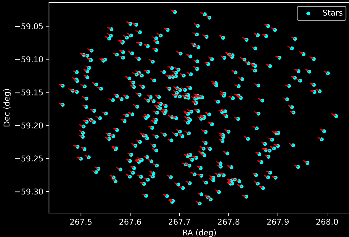
Gaia Cluster: [Gulliver_34] Proper Motion Vectors for Gaia Star Field (n= 315)
