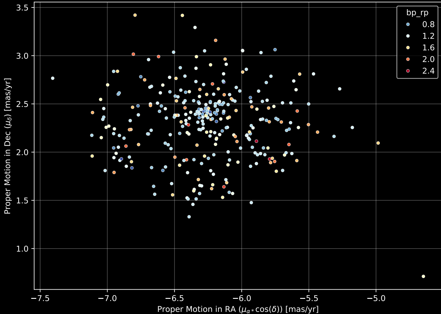
Gaia Cluster: [Gulliver_34] Proper Motion Diagram (n= 315)
