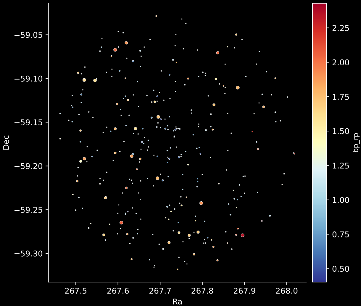
Gaia Cluster: [Gulliver_34] Stars: 315
