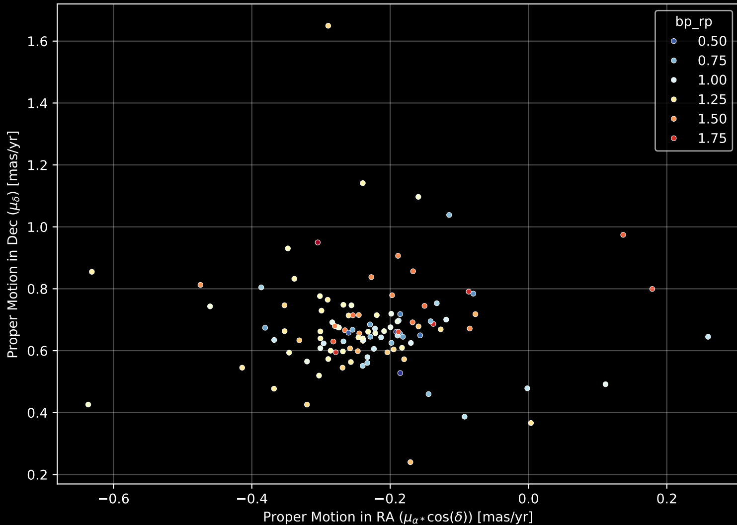
Gaia Cluster: [Gulliver_36] Proper Motion Diagram (n= 112)
