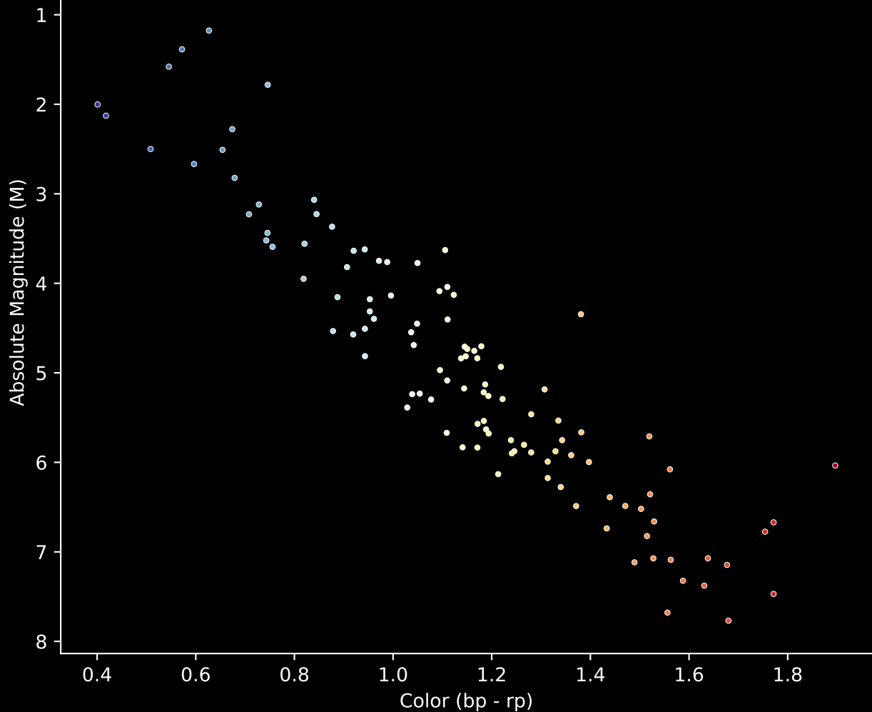
Gaia Cluster: [Gulliver_36] Stars (n= 112) Hertzsprung-Russel Diagram
