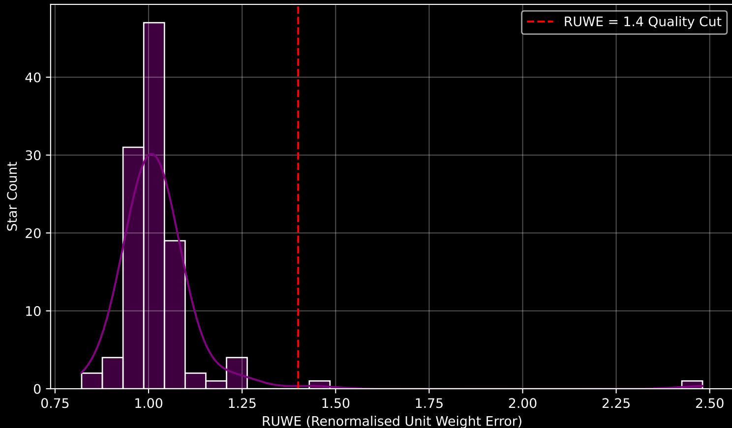
Gaia Cluster: [Gulliver_36] RUWE Distribution (n= 112)
