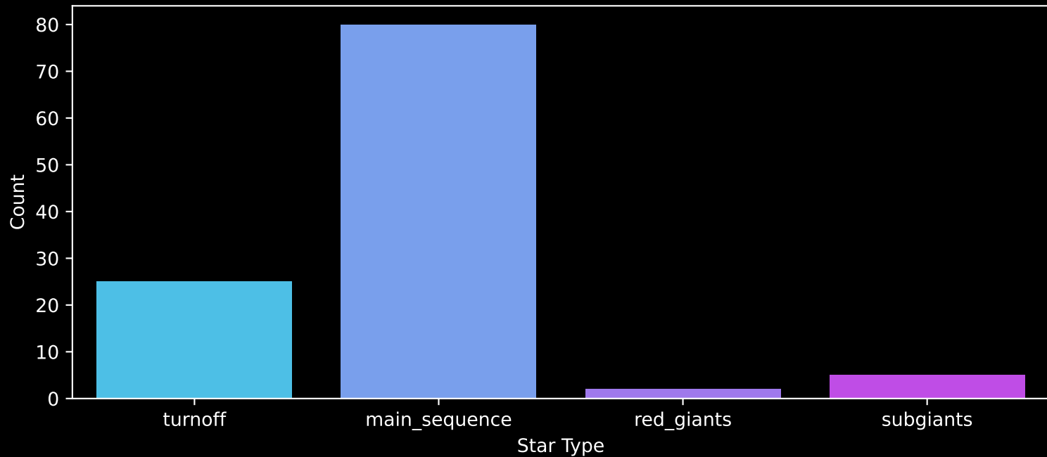
Gaia Cluster: [Gulliver_36] Count plot of Star Type
