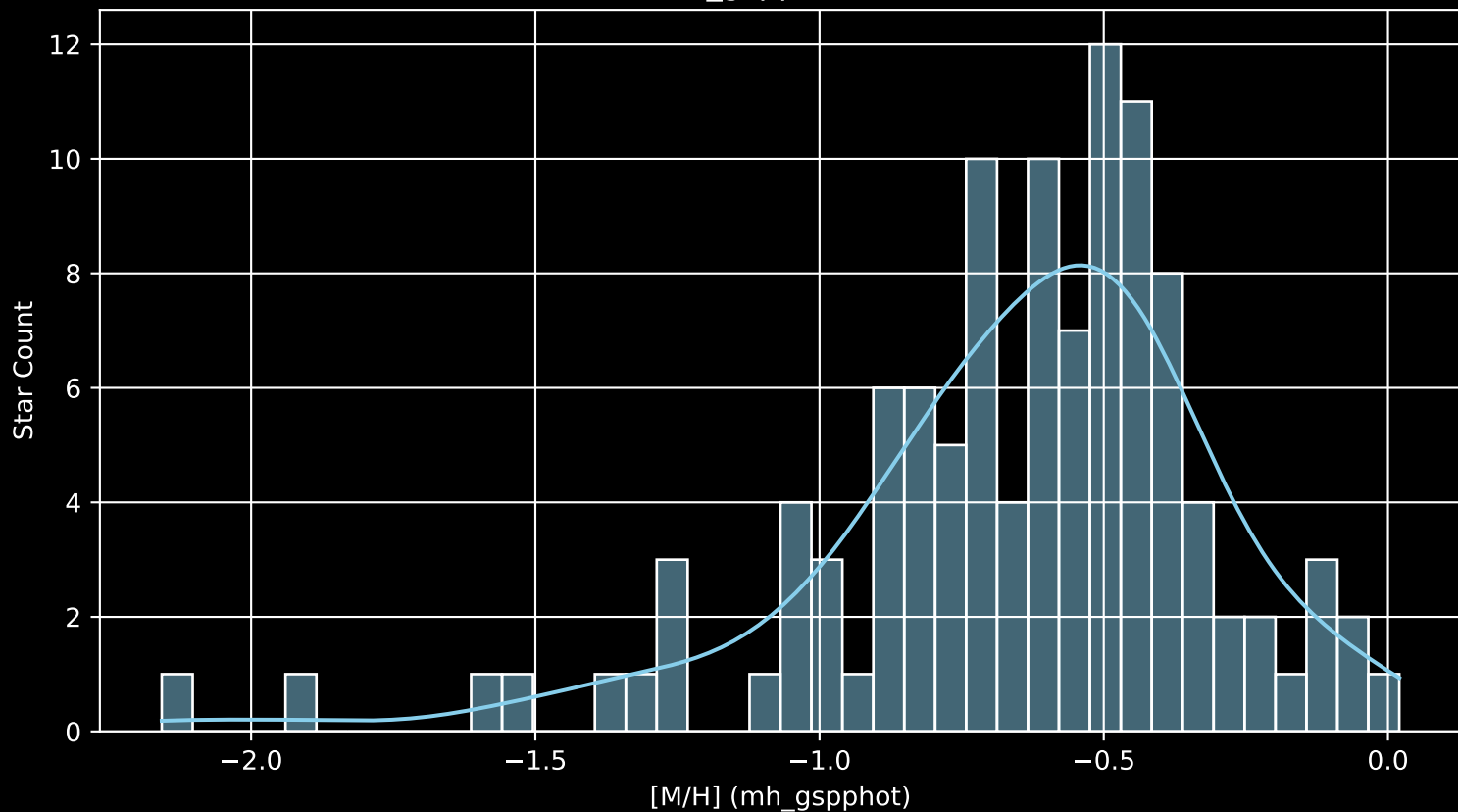
Gaia Cluster: [Gulliver_36 [M/H] (mh_gspphot) (n= 112)
