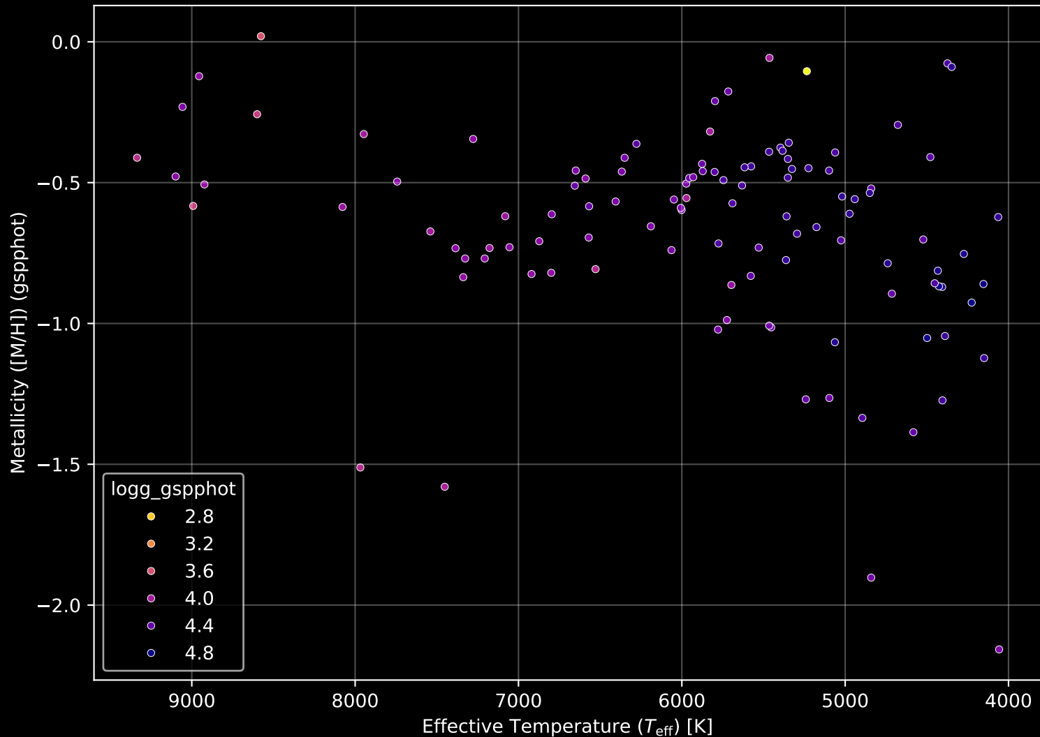
Gaia Cluster: [Gulliver_36] Stellar Population Parameters (n= 112)
