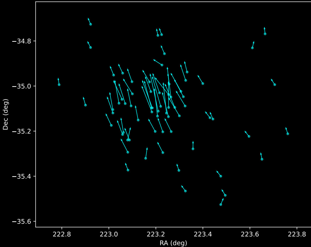
Gaia DR3 Noise Stream Proper Motion Vectors (n=68)
