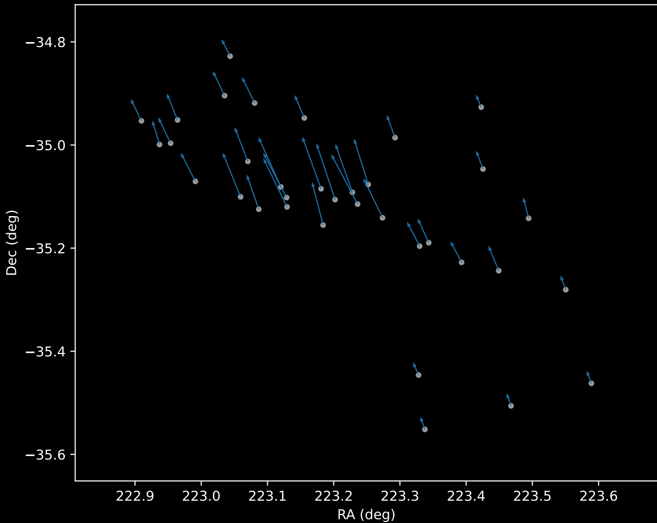
Gaia DR3 Cluster 0 Proper Motion Vectors (n=35)
