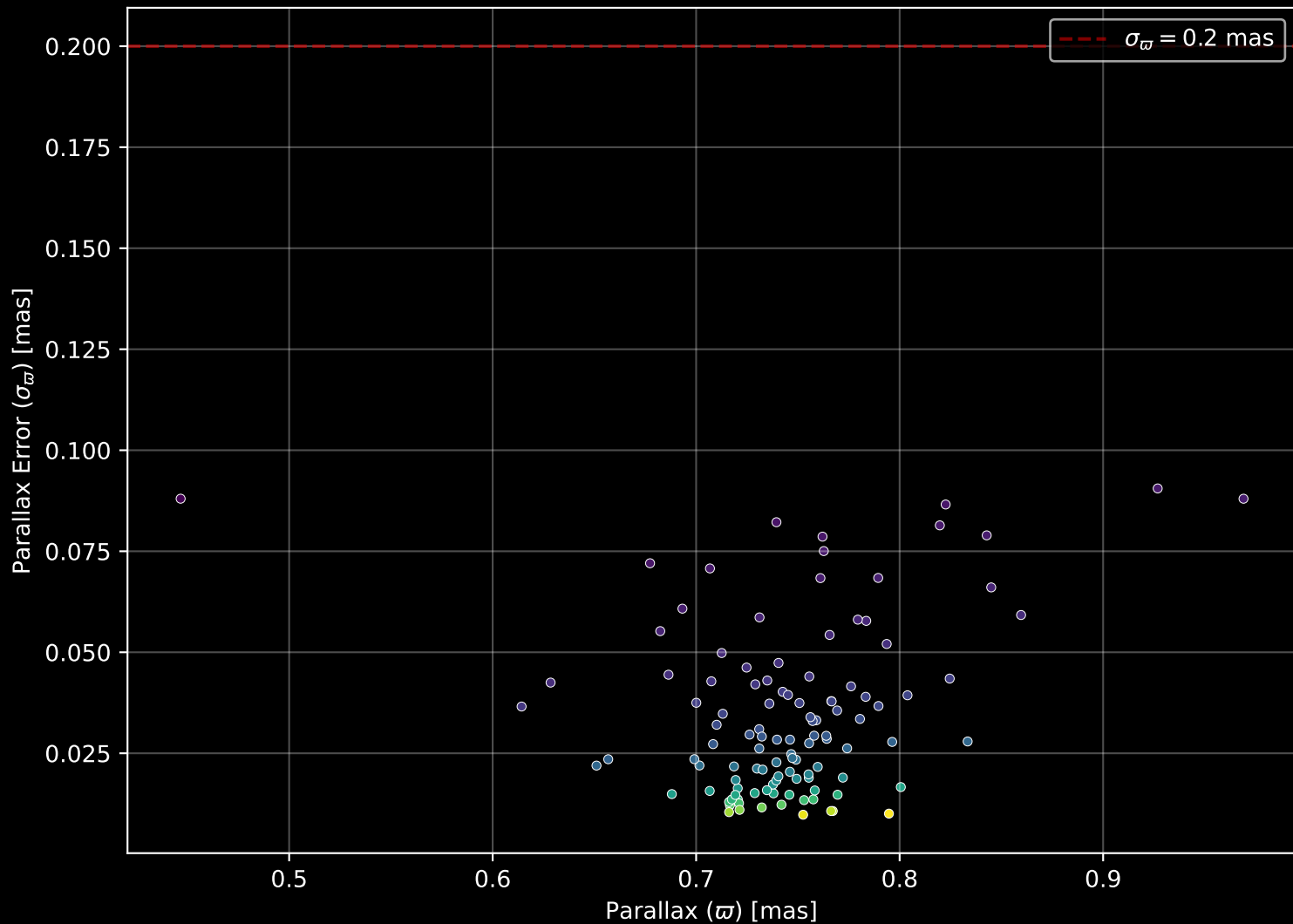
Gaia Cluster: [Gulliver_36] Parallax Quality (n= 112)
